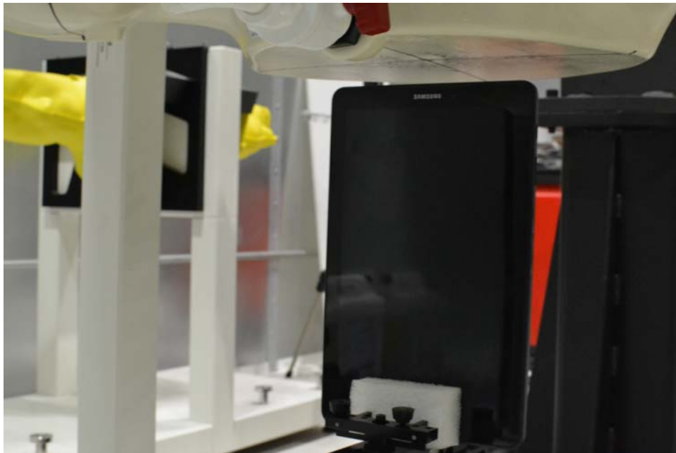
SAR Test Setup Photo 4: Top Edge at 1.5 cm
