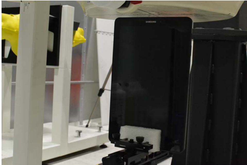
SAR Test Setup Photo 5: Top Edge at 0.4 cm
