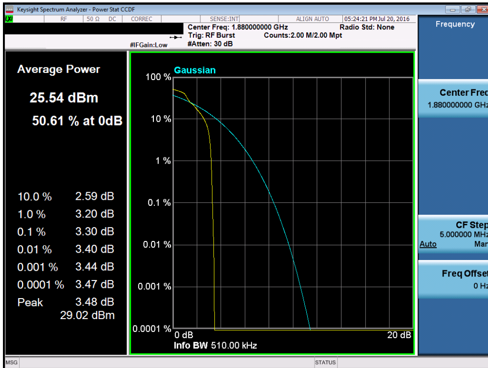
Plot 7-56. Peak-Average Ratio Plot (PCS EDGE Mode – Ch. 661)
