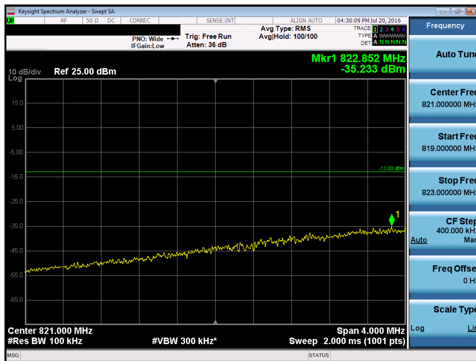
Plot 7-23. Lower Extended Band Edge Plot (Band 5 – 3.0MHz QPSK – RB Size 15)
