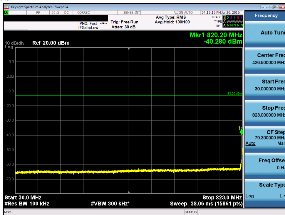
Plot 7-9. Conducted Spurious Plot (Band 5 – 10.0MHz QPSK – RB Size 1, RB Offset 0– Low Channel)
