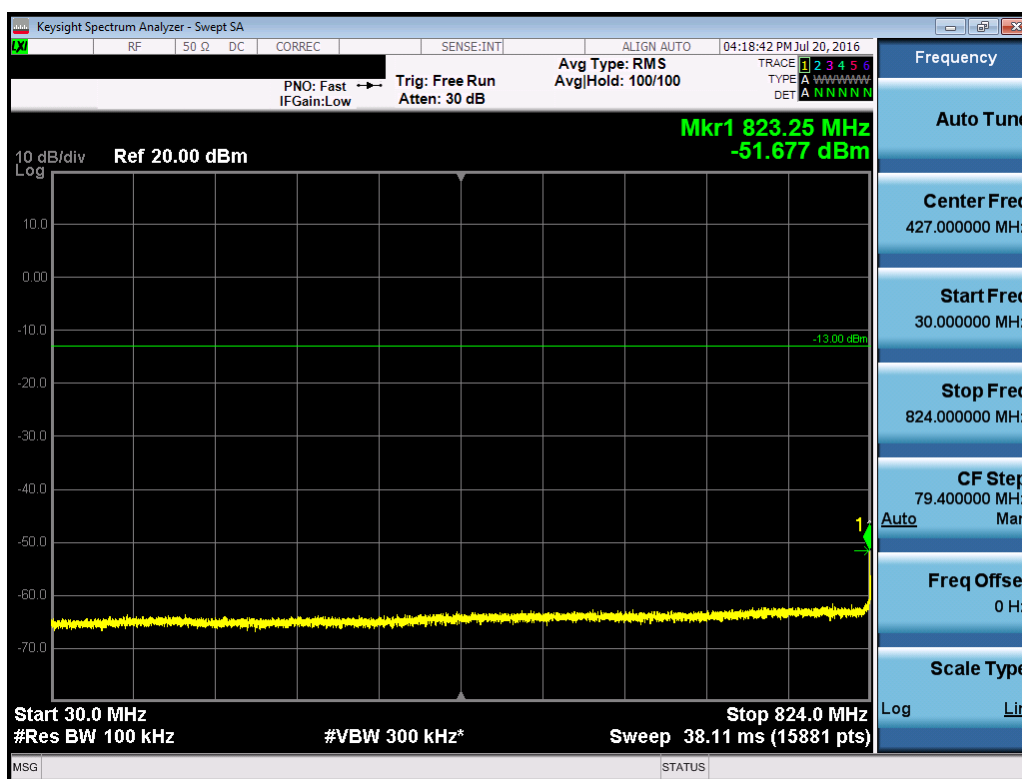
Plot 7-12. Conducted Spurious Plot (Band 5 – 10.0MHz QPSK – RB Size 1, RB Offset 0 – Mid Channel)
