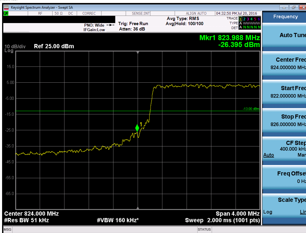
Plot 7-26. Lower Band Edge Plot (Band 5 – 5.0MHz QPSK – RB Size 25)
