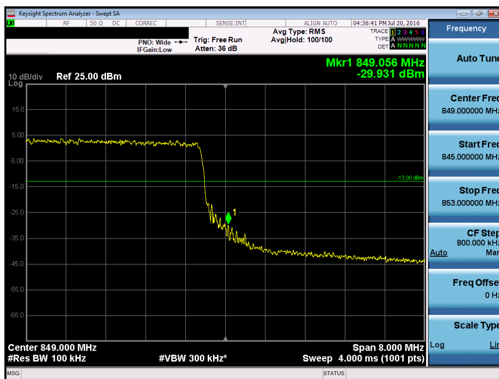
Plot 7-31. Upper Band Edge Plot (Band 5 - 10.0MHz QPSK - RB Size 50)
