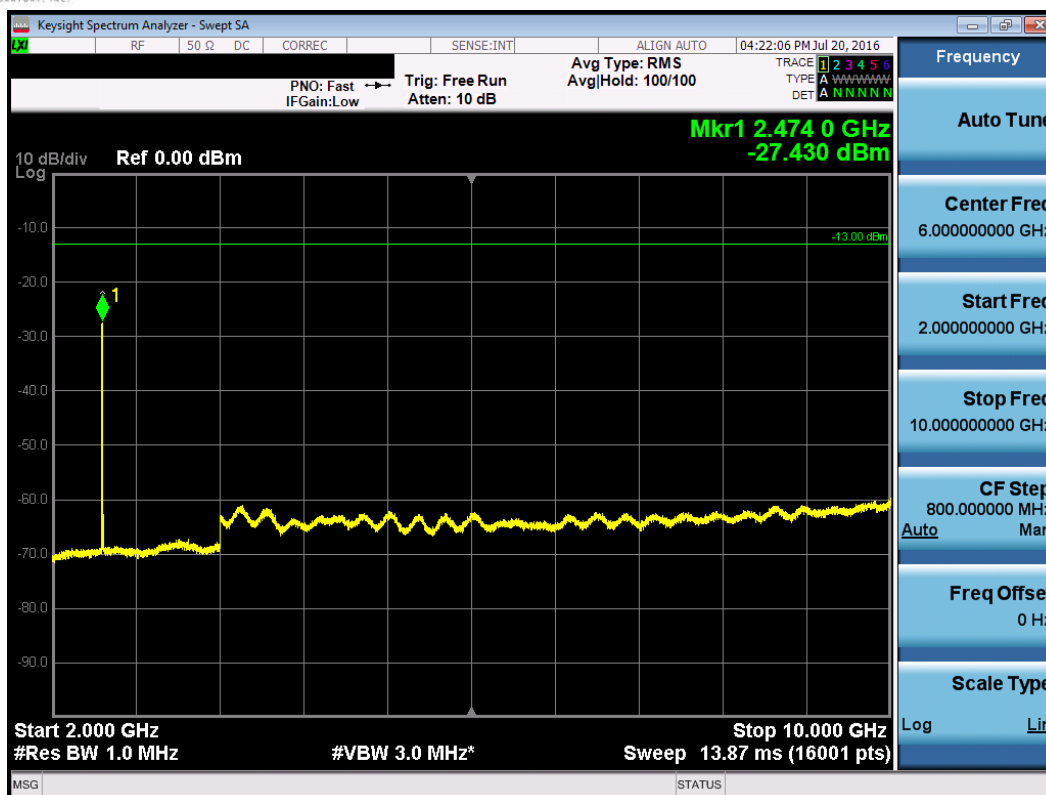
Plot 7-11. Conducted Spurious Plot (Band 5 – 10.0MHz QPSK – RB Size 1, RB Offset 0 – Low Channel)
