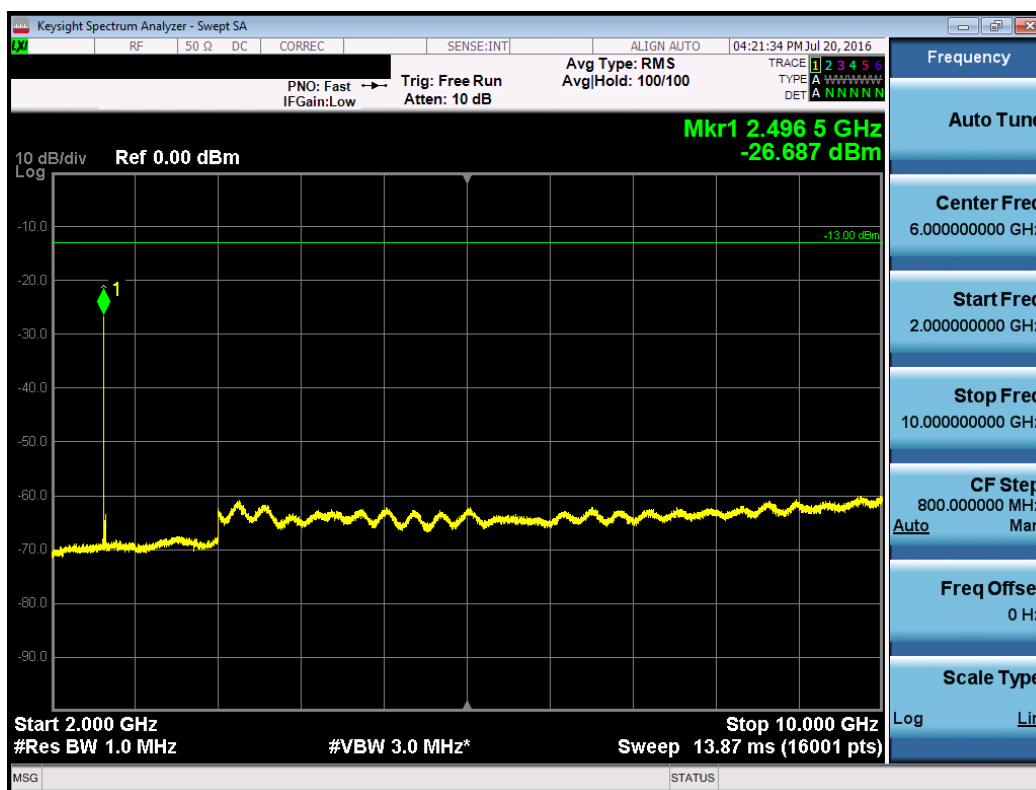
Plot 7-14. Conducted Spurious Plot (Band 5 – 10.0MHz QPSK – RB Size 1, RB Offset 0 – Mid Channel)
