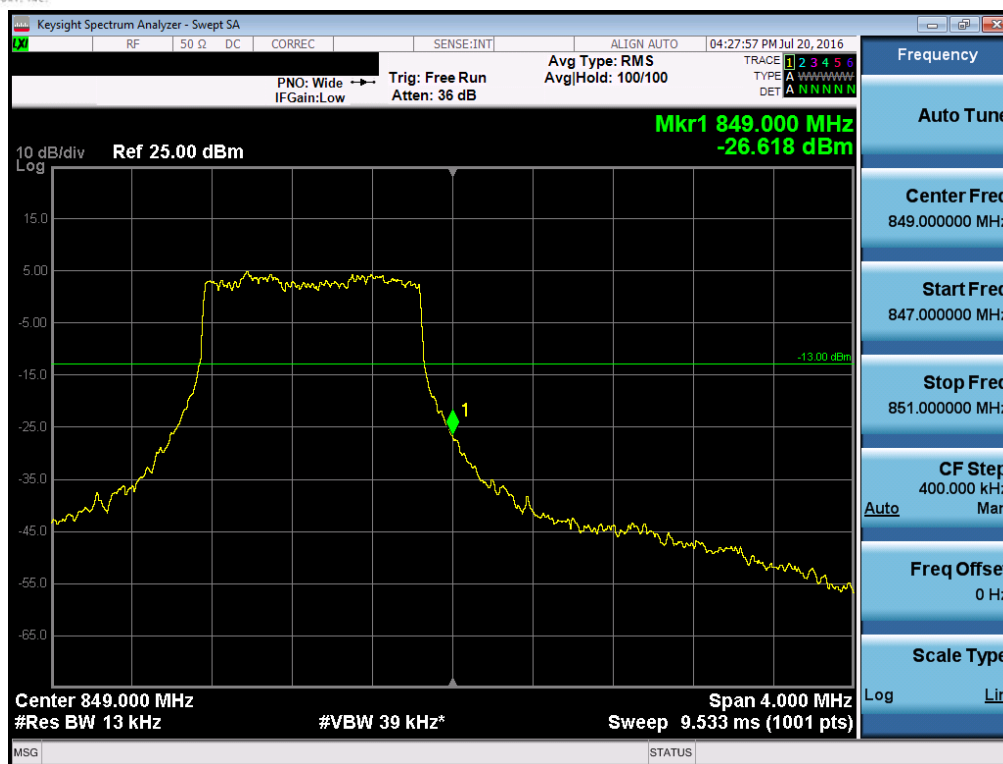
Plot 7-20. Upper Band Edge Plot (Band 5 – 1.4MHz QPSK – RB Size 6)
