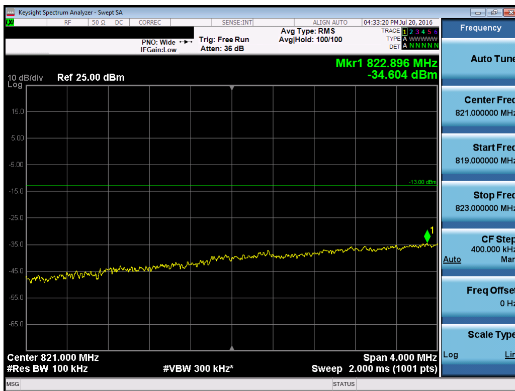
Plot 7-27. Lower Extended Band Edge Plot (Band 5 – 5.0MHz QPSK – RB Size 25)
