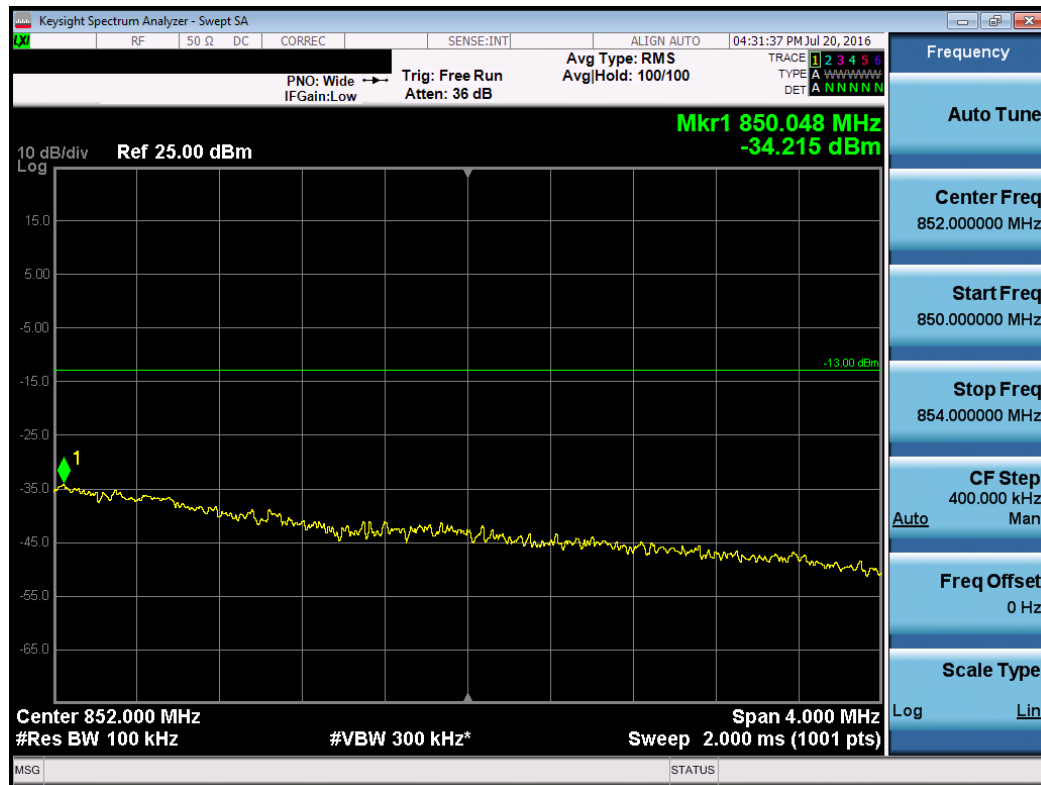
Plot 7-25. Upper Extended Band Edge Plot (Band 5 – Band 5 – 3.0MHz QPSK – RB Size 15)
