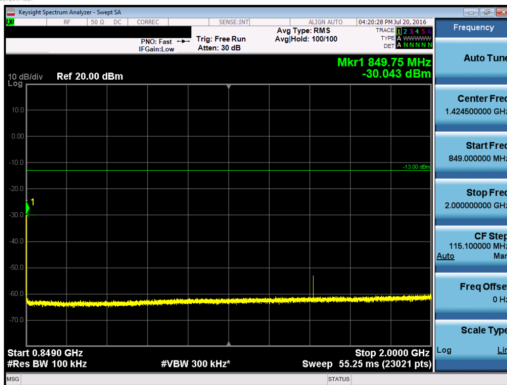
Plot 7-13. Conducted Spurious Plot (Band 5 – 10.0MHz QPSK – RB Size 1, RB Offset 0 – Mid Channel)
