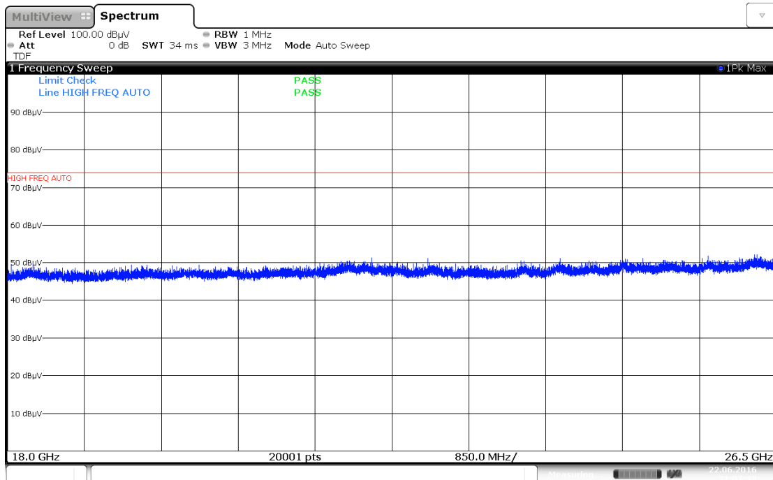
Plot 7-88. Radiated Spurious Plot above 18GHz (802.11a – Ant. Pol. V)
