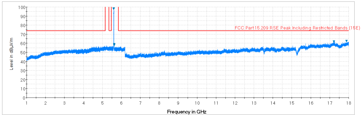
Plot 7-84. Radiated Spurious Plot above 1GHz (802.11a – U2C Ch. 116, Ant. Pol. V)
