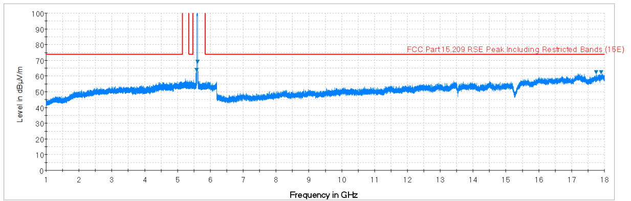
Plot 7-83. Radiated Spurious Plot above 1GHz (802.11a – U2C Ch. 116, Ant. Pol. H)
