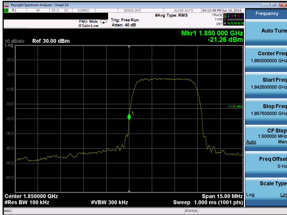
Plot 7-51. Band Edge Plot (PCS WCDMA Mode – Ch. 9262)
