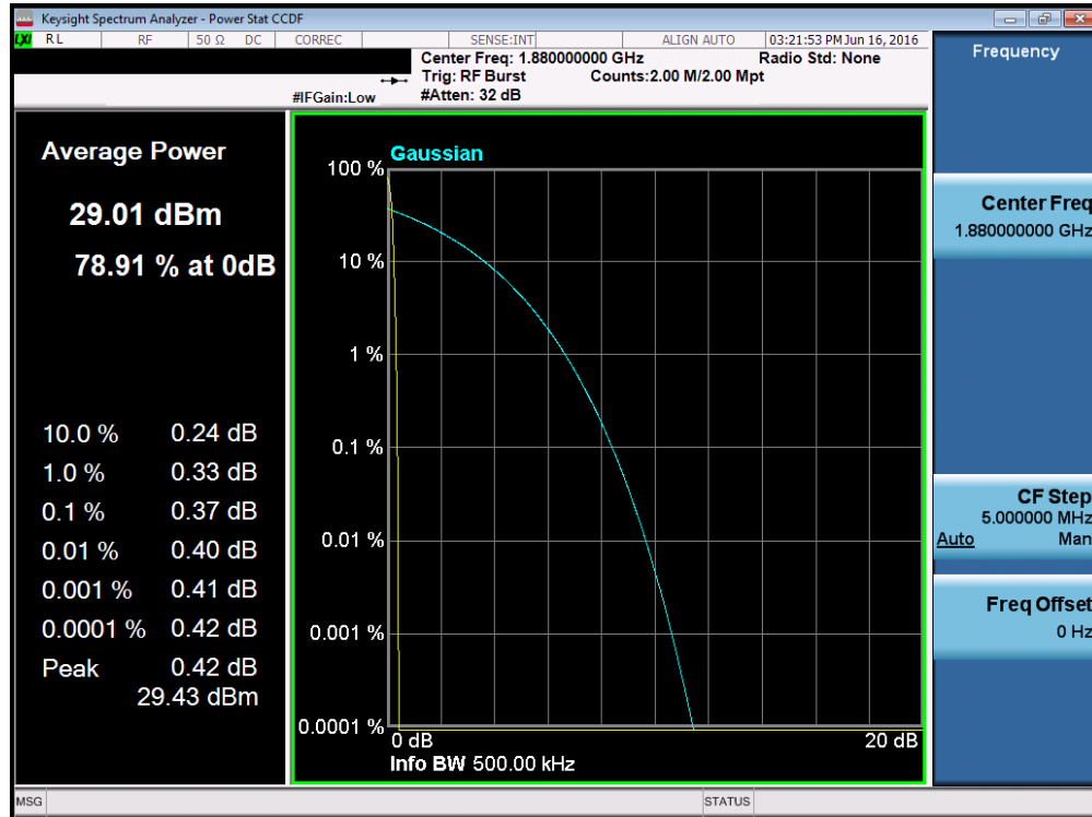
Plot 7-55. Peak-Average Ratio Plot (PCS GPRS Mode – Ch. 661)
