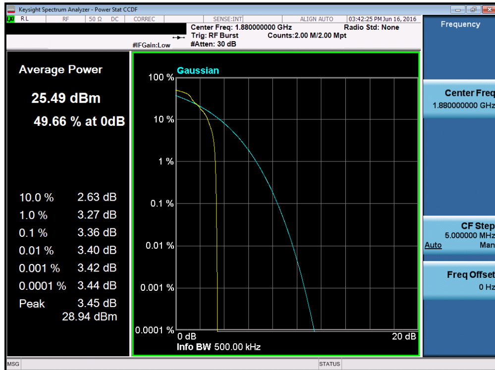
Plot 7-56. Peak-Average Ratio Plot (EDGE1900 Mode – Ch. 661)
