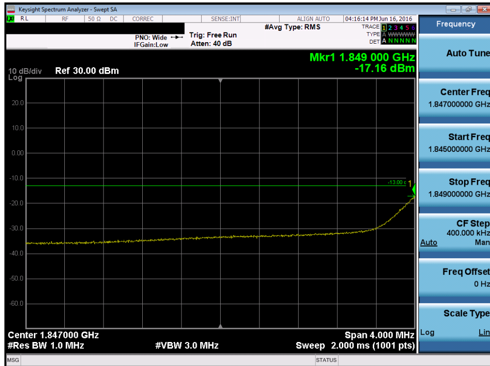
Plot 7-52. 4MHz Span Plot (PCS WCDMA Mode – Ch. 9262)
