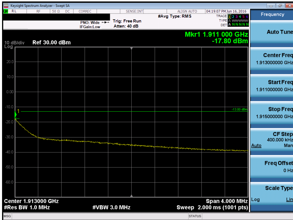
Plot 7-54. 4MHz Span Plot (PCS WCDMA Mode – Ch. 9538)
