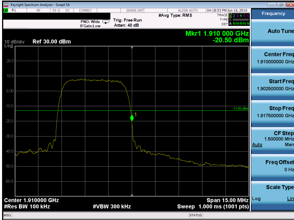
Plot 7-53. Band Edge Plot (PCS WCDMA Mode – Ch. 9538)
