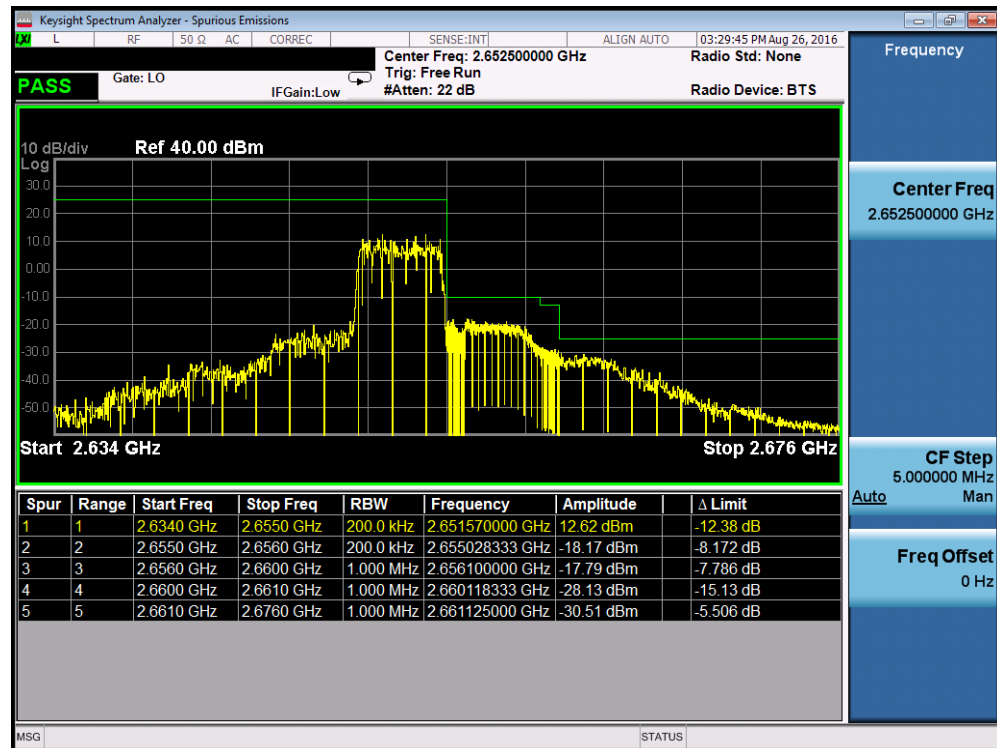
Plot 7-19. Upper ACP Plot (Band 41 – 5.0MHz QPSK – RB Size 25)
