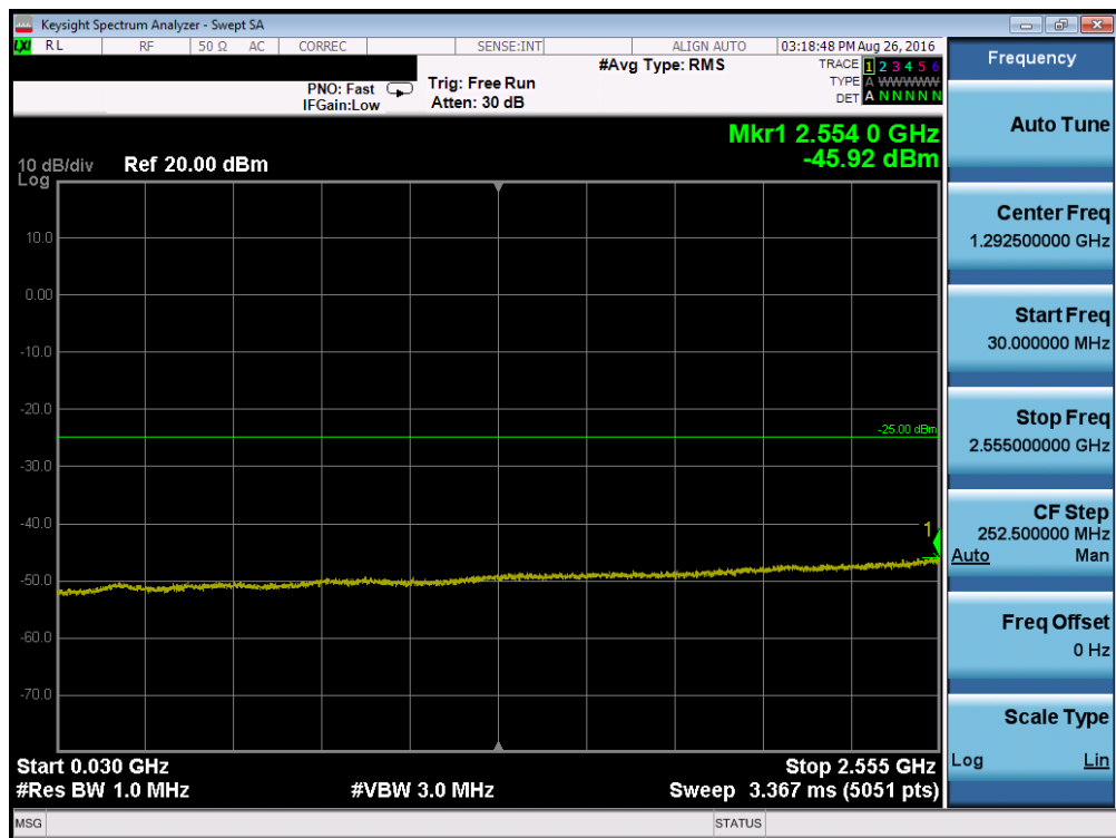
Plot 7-12. Conducted Spurious Plot (Band 41 – 5.0MHz QPSK – RB Size 1, RB Offset 0 – Mid Channel)
