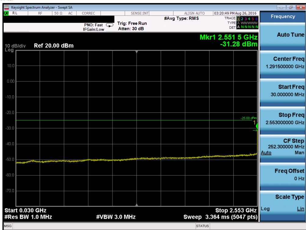
Plot 7-9. Conducted Spurious Plot (Band 41 – 5.0MHz QPSK – RB Size 1, RB Offset 0 – Low Channel)
