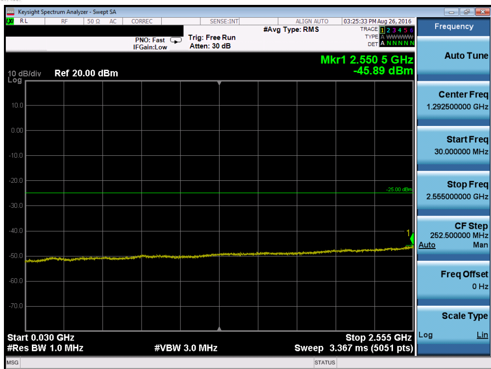
Plot 7-15. Conducted Spurious Plot (Band 41 – 5.0MHz QPSK – RB Size 1, RB Offset 0 – High Channel)
