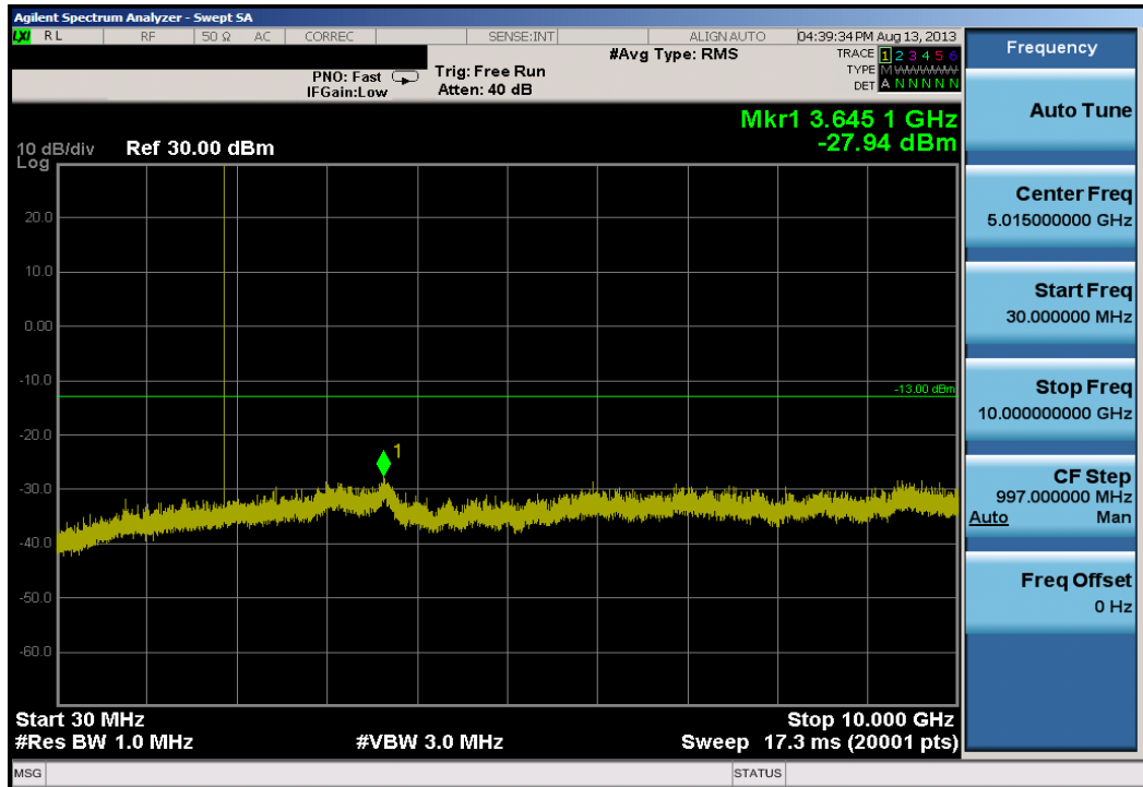
Plot 6-18. Conducted Spurious Plot (PCS GSM Mode – Ch. 661)
