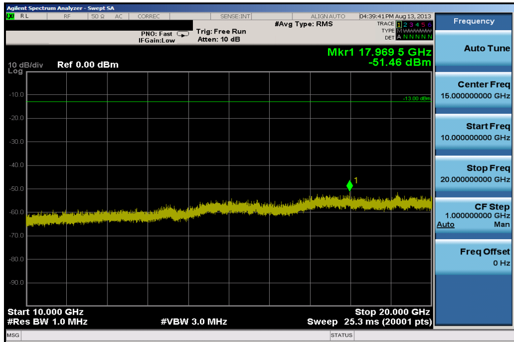
Plot 6-19. Conducted Spurious Plot (PCS GSM Mode – Ch. 661)
