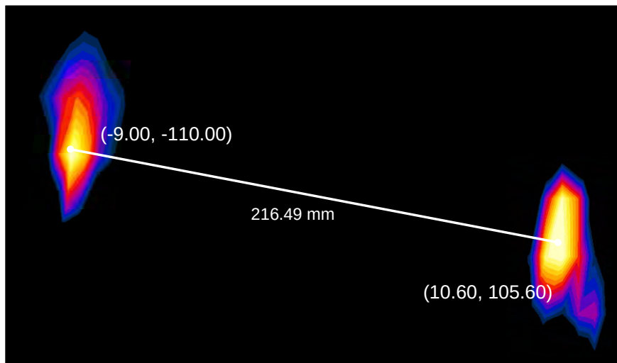
Figure 11-8 Peak SAR Locations of 5 GHz WLAN and GPRS 1900 MHz
