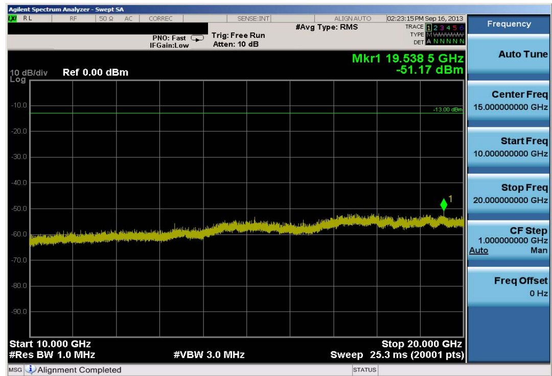
Plot 6-17. Conducted Spurious Plot (PCS WCDMA Mode – Ch. 9262)
