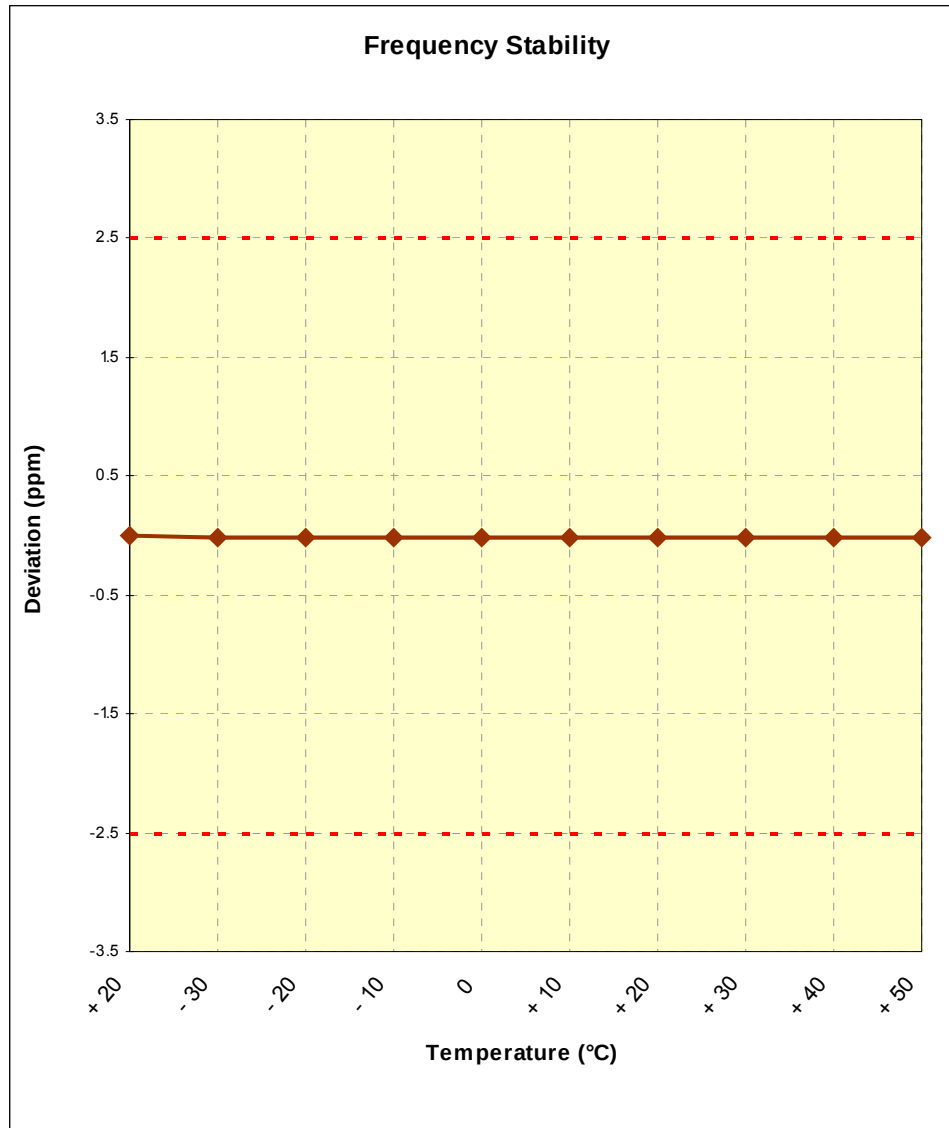
Figure 6-7. Frequency Stability Graph (Cellular WCDMA Mode – Ch. 4183)
