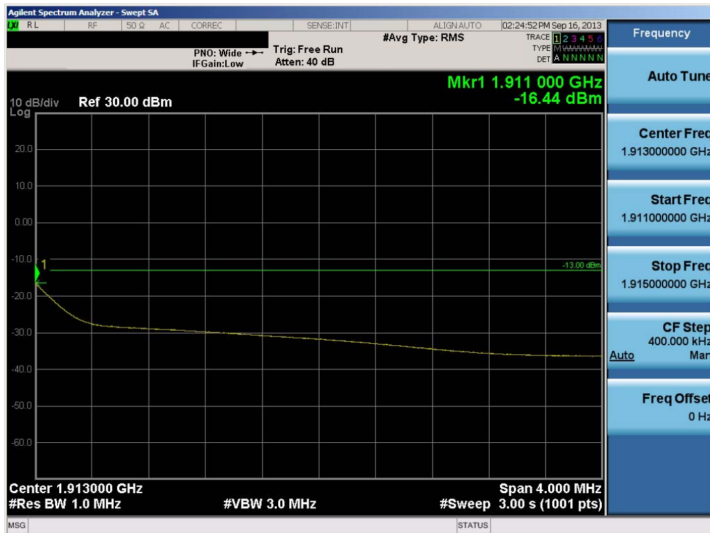
Plot 6-29. 4MHz Span Plot (PCS WCDMA Mode – Ch. 9538)
