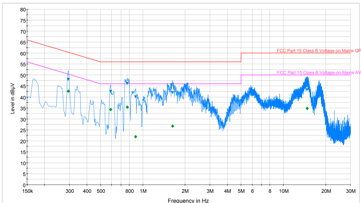
Plot 6-6. Line-Conducted Test Plot (L1)
