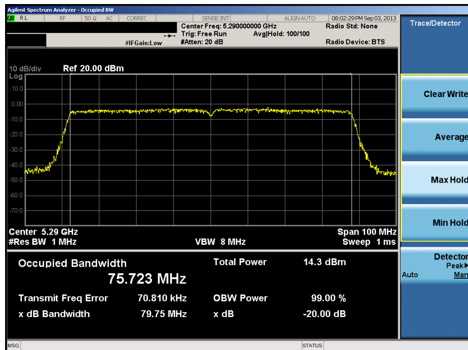
Plot 6-30. 20dB Bandwidth Plot (80MHz BW 802.11ac (UNII Band 2) – Ch. 58)
