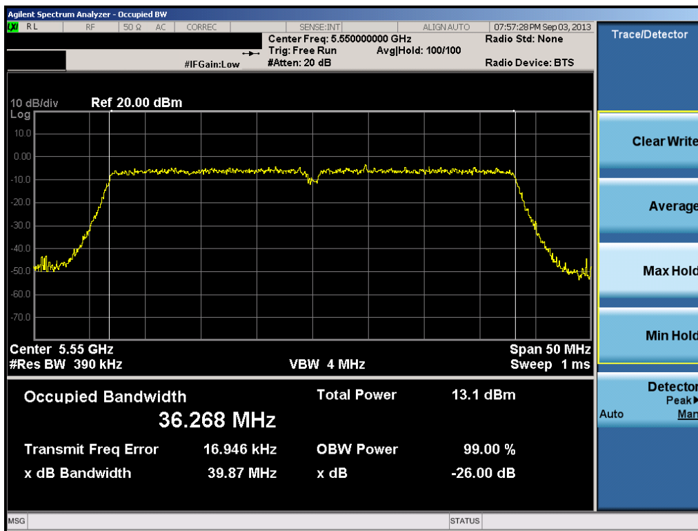
Plot 6-26. 26dB Bandwidth Plot (40MHz BW 802.11n (UNII Band 3) – Ch. 110)
