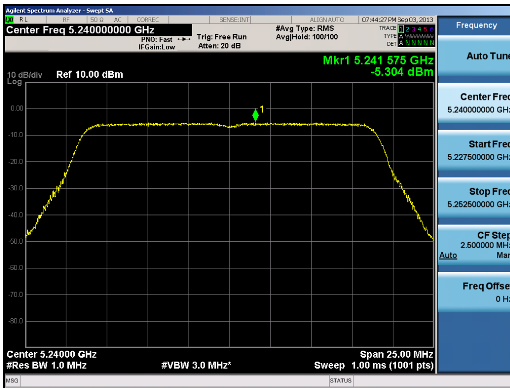
Plot 6-36. Peak Power Spectral Density Plot (20MHz BW 802.11n (UNII Band 1) – Ch. 48)
