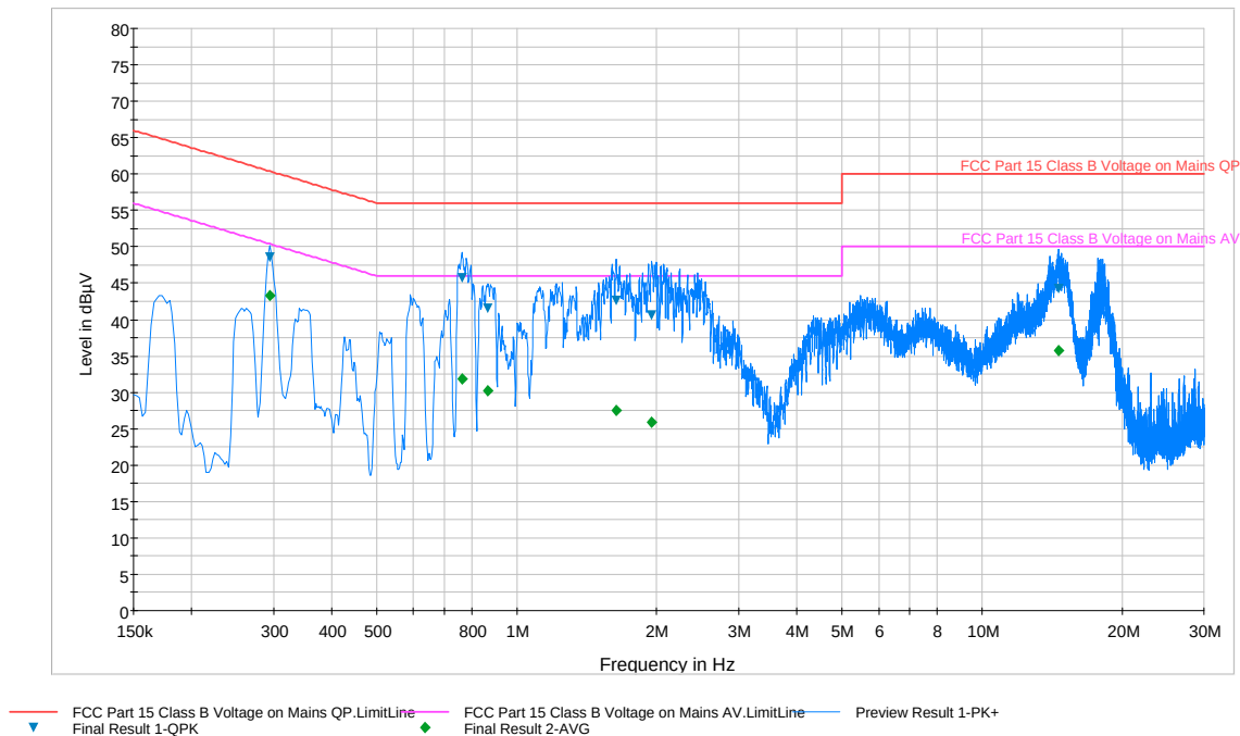
Plot 6-87. Line Conducted Plot with 802.11a UNII Band 3 (L1)
