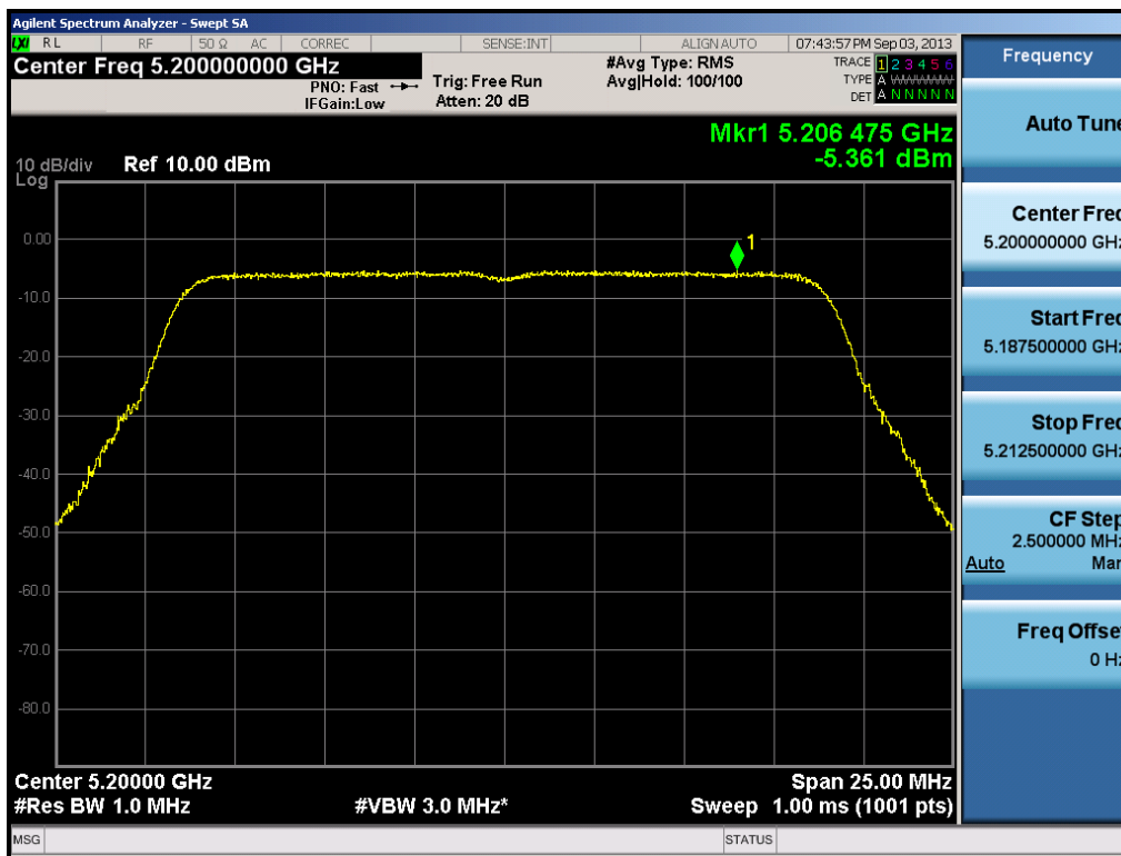
Plot 6-35. Peak Power Spectral Density Plot (20MHz BW 802.11n (UNII Band 1) – Ch. 40)
