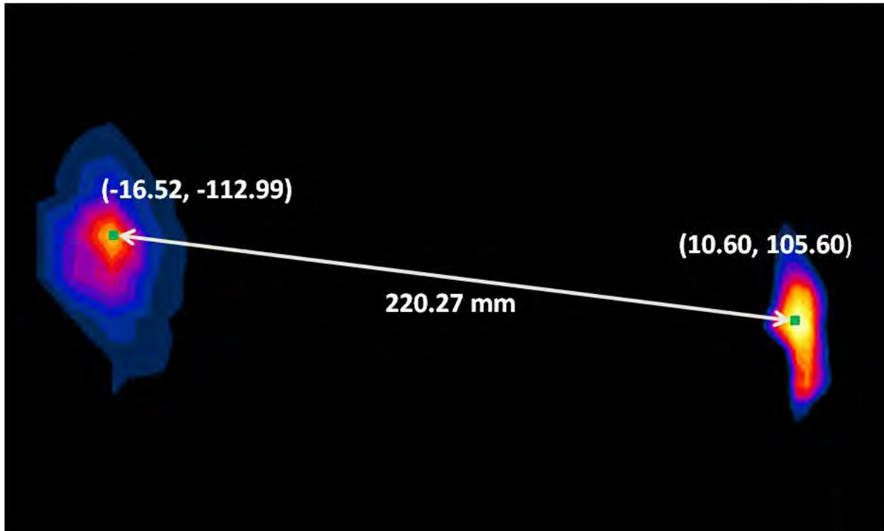
Figure 11-13 Peak SAR Location Plot of LTE Band 4 and 5 GHz WLAN
