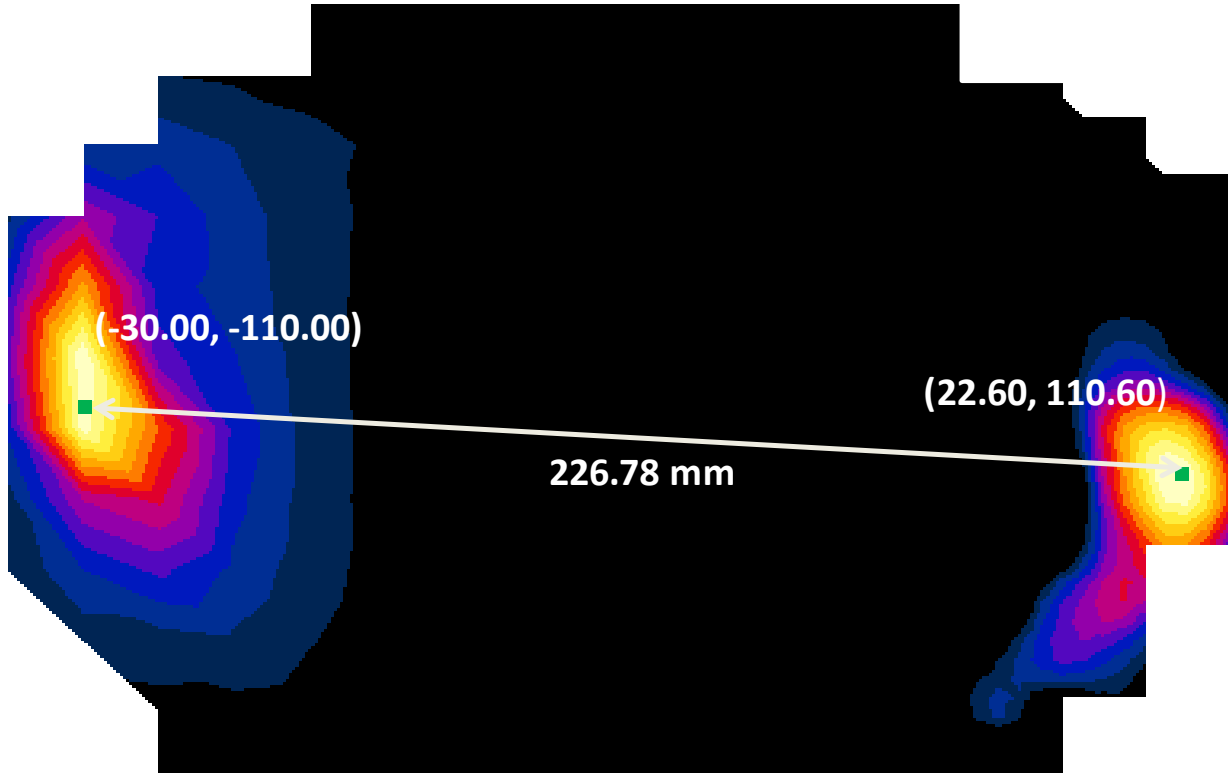
Figure 11-4 Peak SAR Location Plot of LTE Band 17 and 2.4 GHz WLAN
