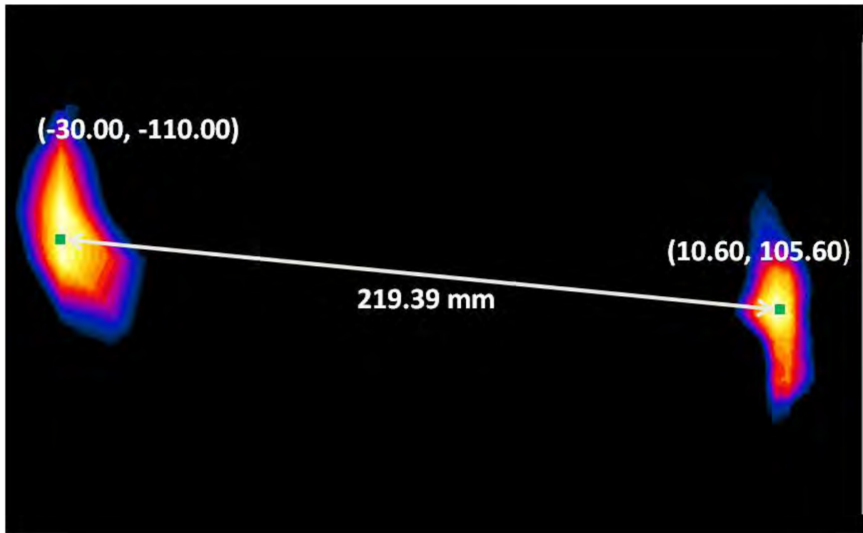
Figure 11-11 Peak SAR Location Plot of LTE Band 17 and 5 GHz WLAN
