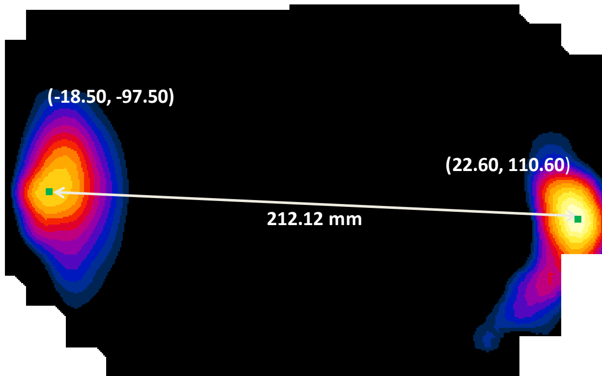
Figure 11-3 Peak SAR Location Plot of UMTS 1900 MHz and 2.4 GHz WLAN
