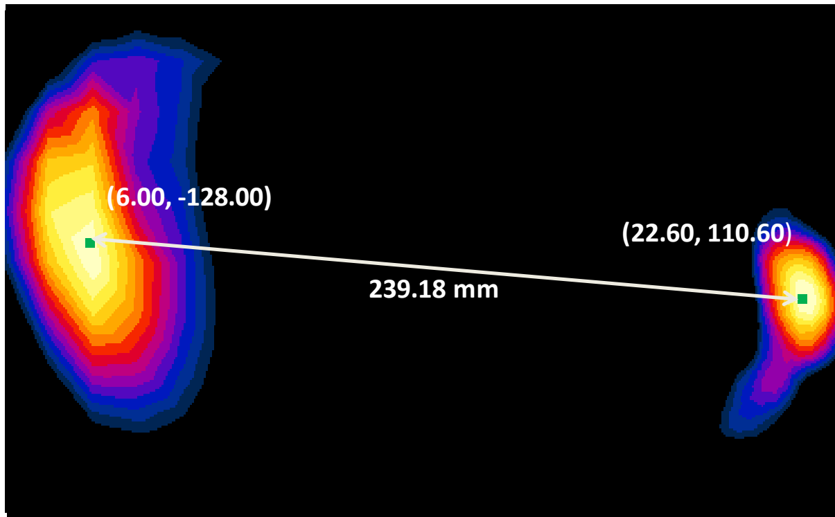
Figure 11-5 Peak SAR Location Plot of LTE Band 5 and 2.4 GHz WLAN
