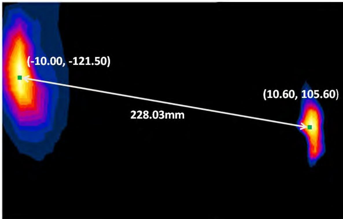
Figure 11-8 Peak SAR Location Plot of UMTS 850 MHz and 5 GHz WLAN
