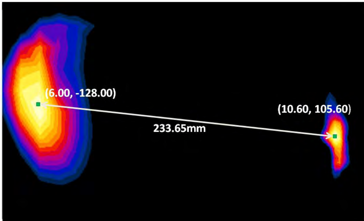
Figure 11-12 Peak SAR Location Plot of LTE Band 5 and 5 GHz WLAN
