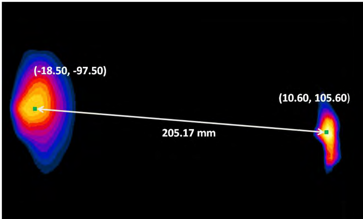
Figure 11-10 Peak SAR Location Plot of UMTS 1900 MHz and 5 GHz WLAN
