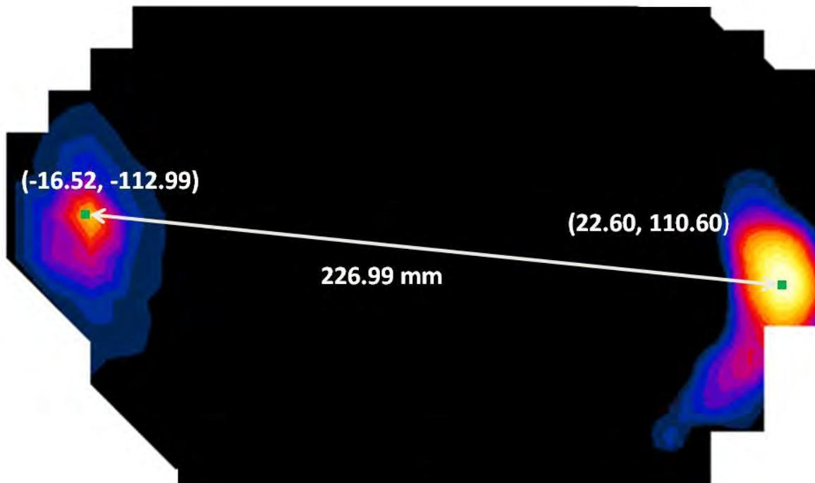
Figure 11-6 Peak SAR Location Plot of LTE Band 4 and 2.4 GHz WLAN
