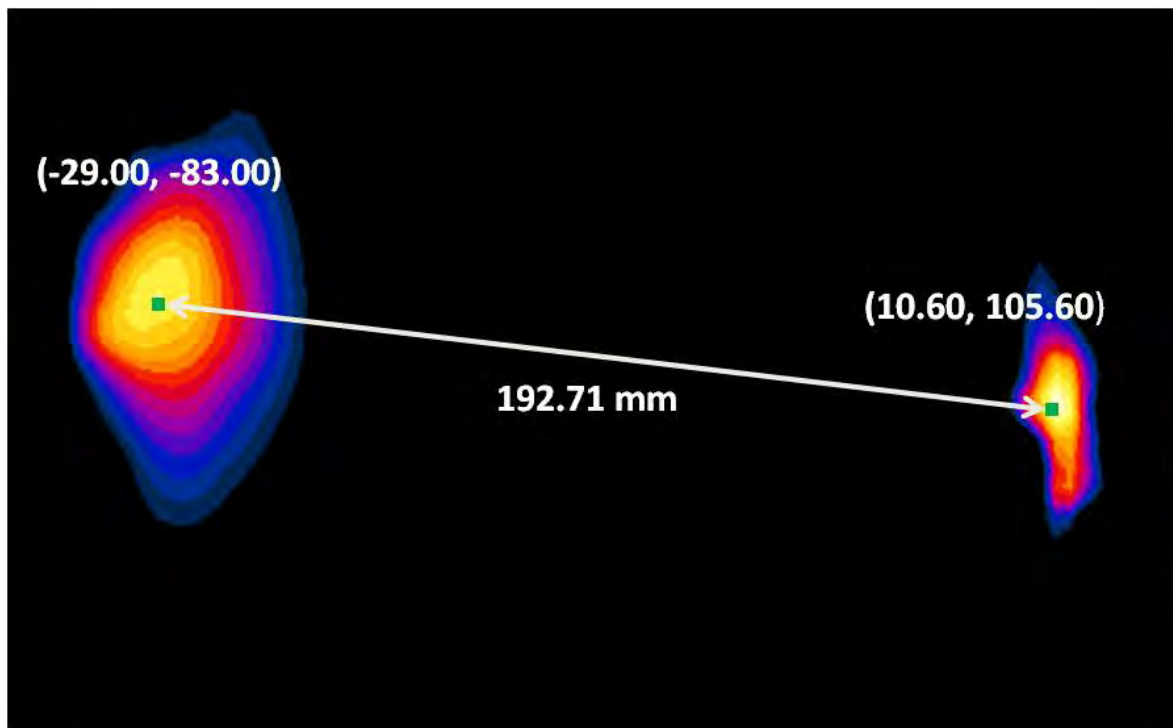
Figure 11-9 Peak SAR Location Plot of GPRS 1900 MHz and 5 GHz WLAN
