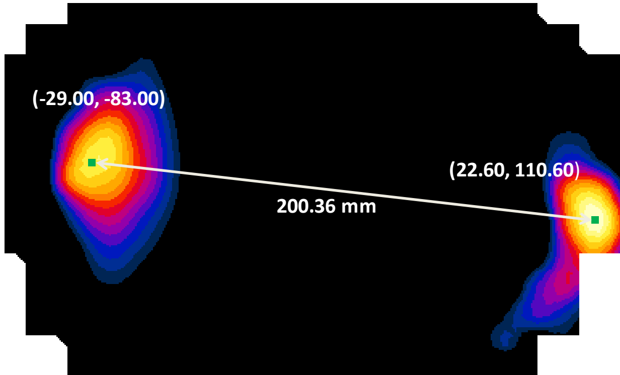
Figure 11-2 Peak SAR Location Plot of GPRS 1900 MHz and 2.4 GHz WLAN
