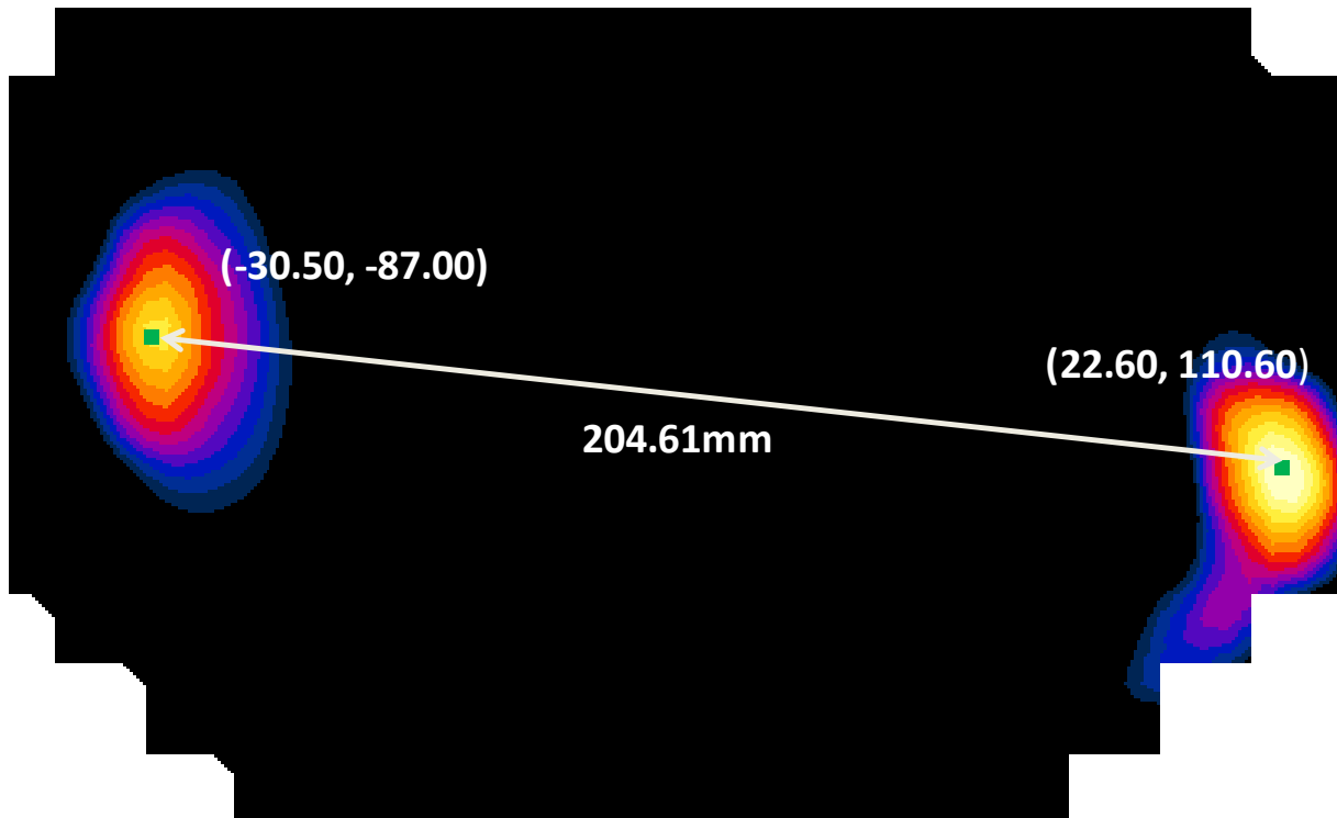
Figure 11-7 Peak SAR Location Plot of LTE Band 2 and 2.4 GHz WLAN
