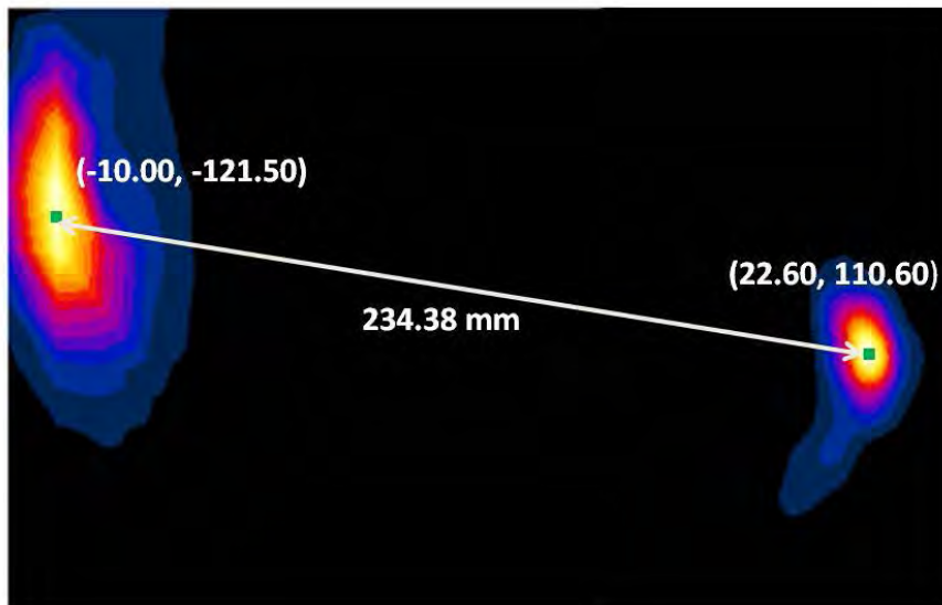
Figure 11-1 Peak SAR Location Plot of UMTS 850 MHz and 2.4 GHz WLAN
