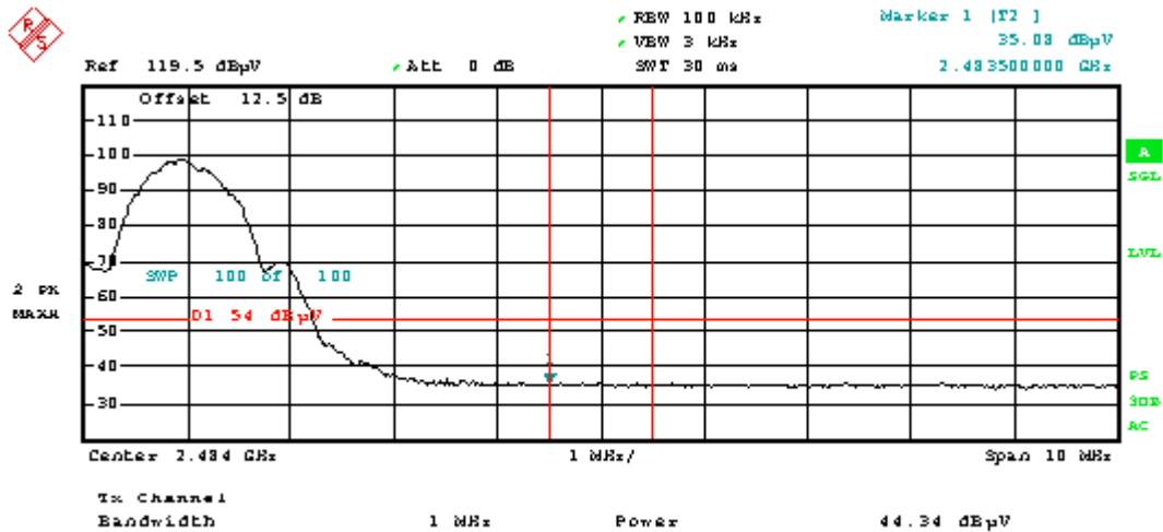
Plot 6-18. Radiated Restricted Band Edge Measurements (Average)
