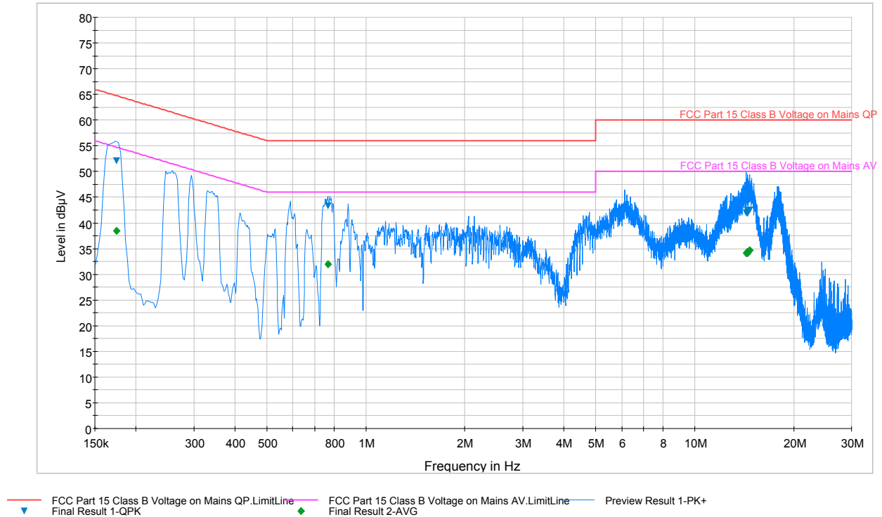
Plot 6-7. Line-Conducted Test Plot (N)
