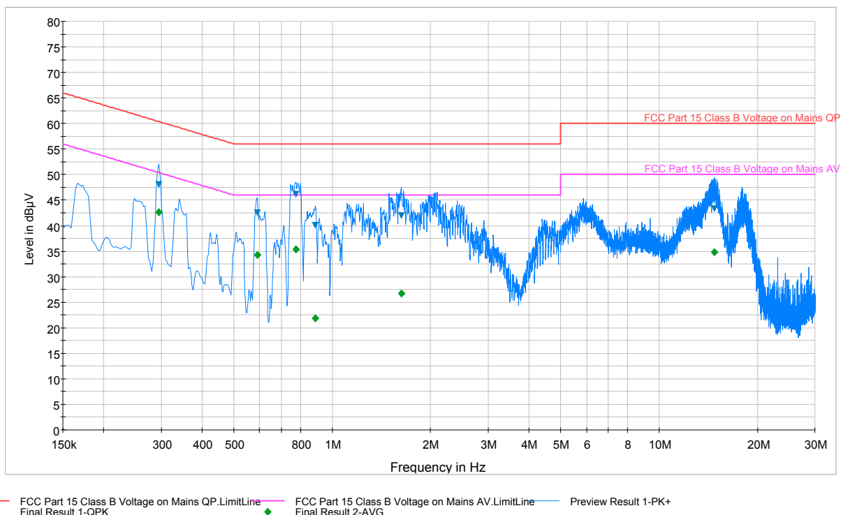
Plot 6-6. Line-Conducted Test Plot (L1)
