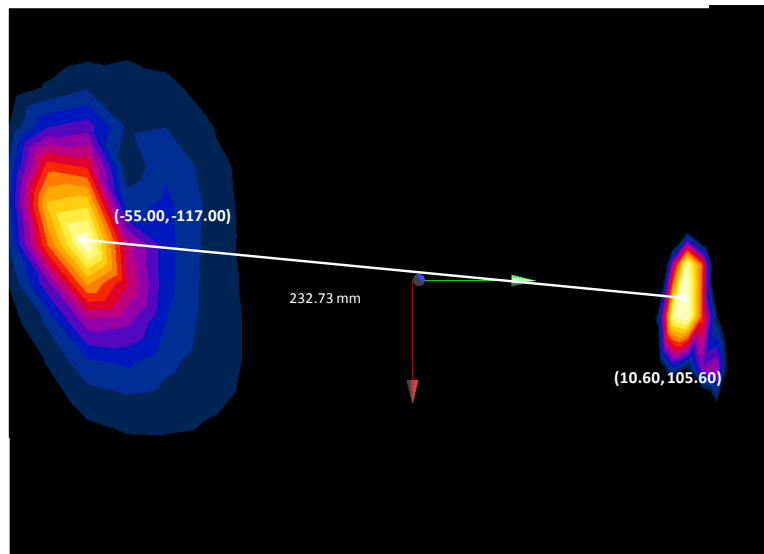
Figure 11-14 Peak SAR Locations of 5 GHz WLAN and GPRS 850 MHz
