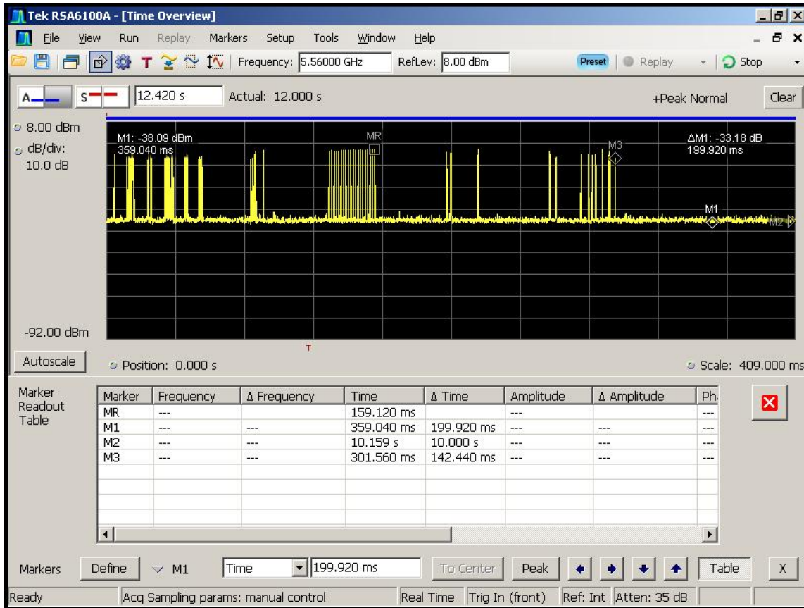
Figure 6-6. Zoomed channel move time
