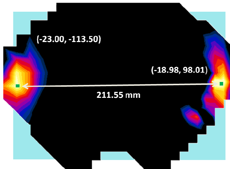
Figure 11-6 Peak SAR Location Plot of UMTS 1900 MHz and 5 GHz WLAN
