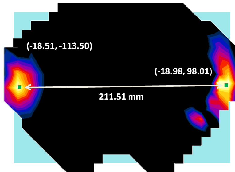
Figure 11-5 Peak SAR Location Plot of UMTS 1750 MHz and 5 GHz WLAN
