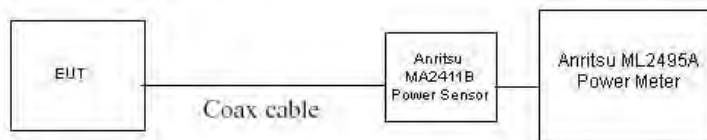
Figure 8-2 Power Measurement Setup for Signal < 50 MHz
