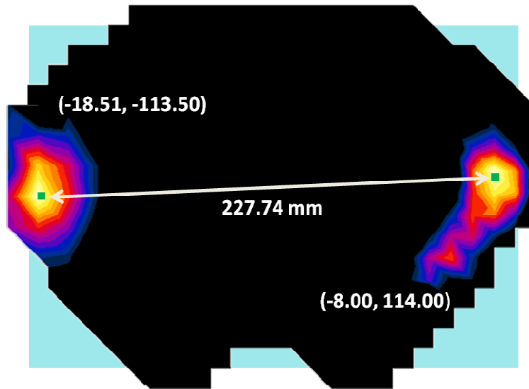
Figure 11-1 Peak SAR Location Plot of UMTS 1750 MHz and 2.4 GHz WLAN
