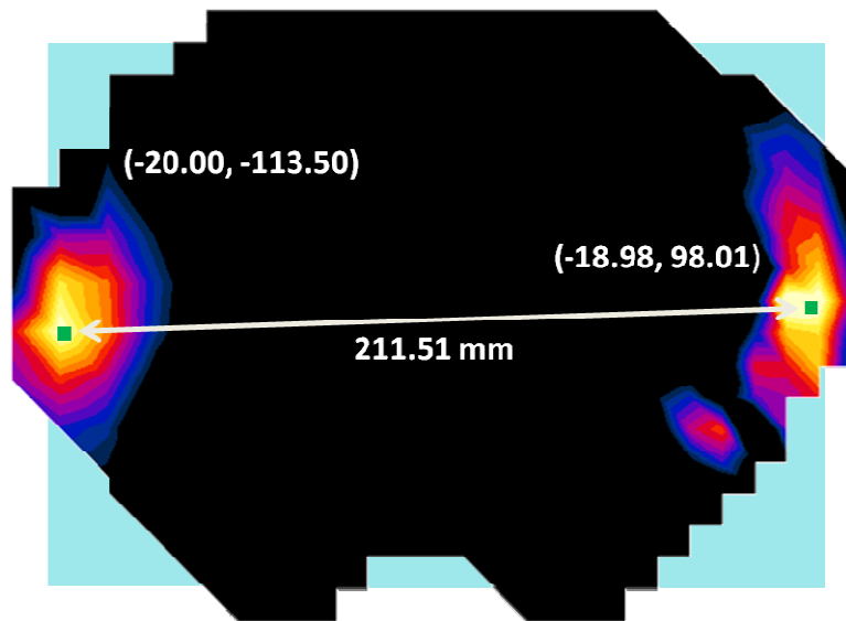
Figure 11-8 Peak SAR Location Plot of LTE Band 2 and 5 GHz WLAN
