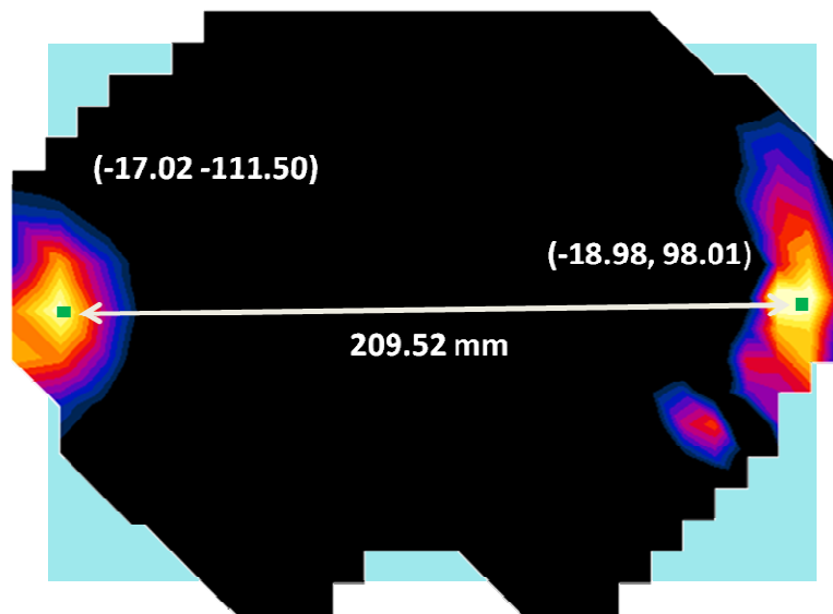
Figure 11-7 Peak SAR Location Plot of LTE Band 4 and 5 GHz WLAN
