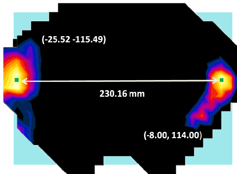
Figure 11-9 Peak SAR Location Plot of UMTS 1750 MHz and 2.4 GHz WLAN
