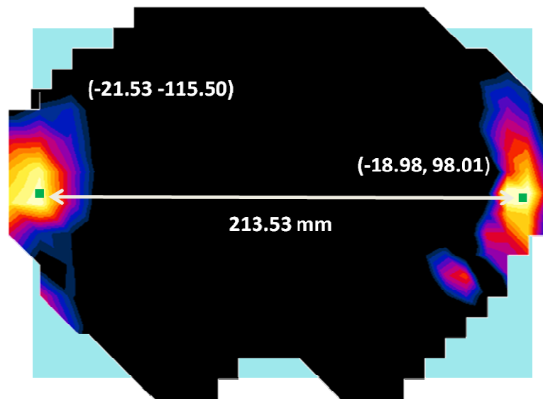
Figure 11-11 Peak SAR Location Plot of LTE Band 4 and 5 GHz WLAN
