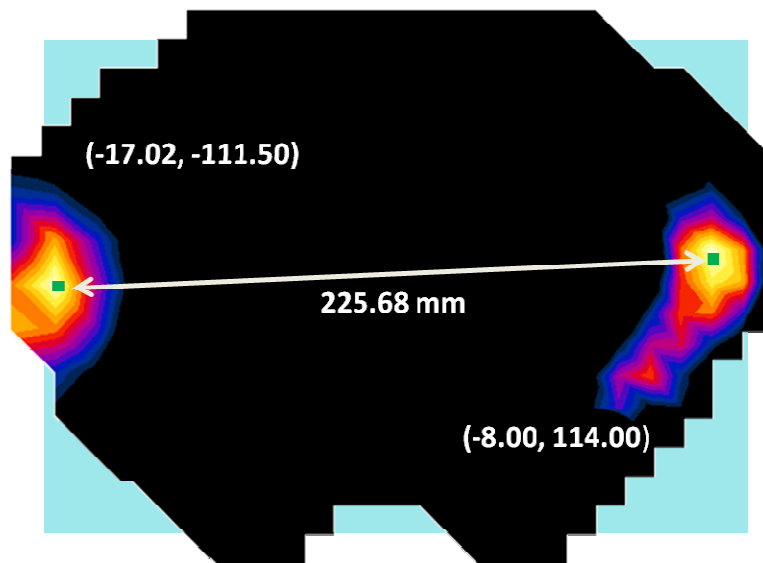
Figure 11-3 Peak SAR Location Plot of LTE Band 4 and 2.4 GHz WLAN
