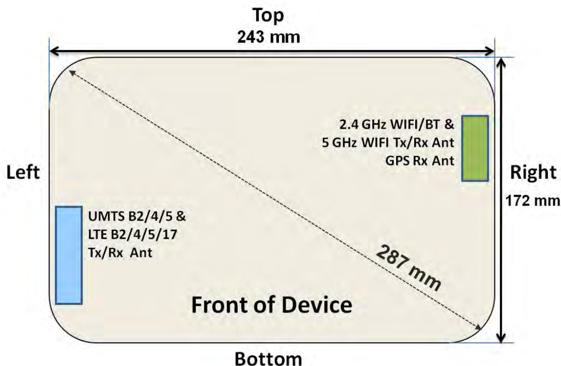
Figure 1-1 DUT Antenna Locations
