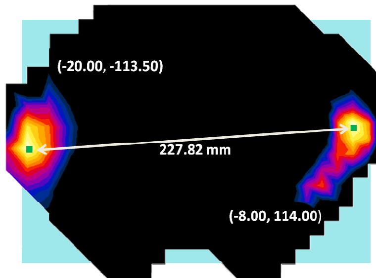
Figure 11-4 Peak SAR Location Plot of LTE Band 2 and 2.4 GHz WLAN
