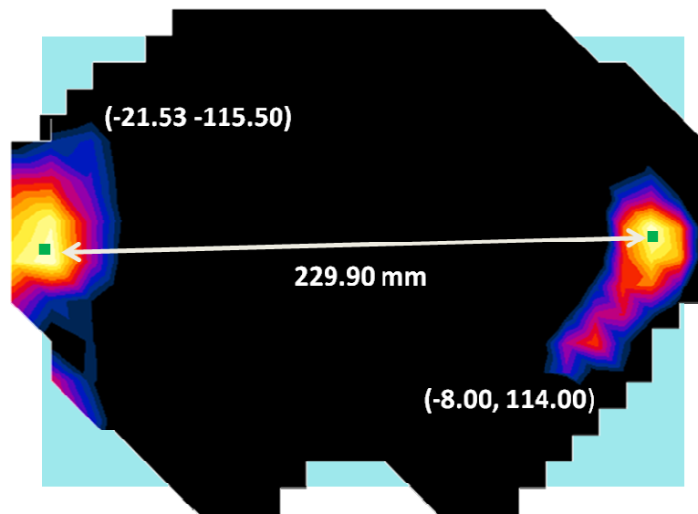
Figure 11-10 Peak SAR Location Plot of LTE Band 4 and 2.4 GHz WLAN
