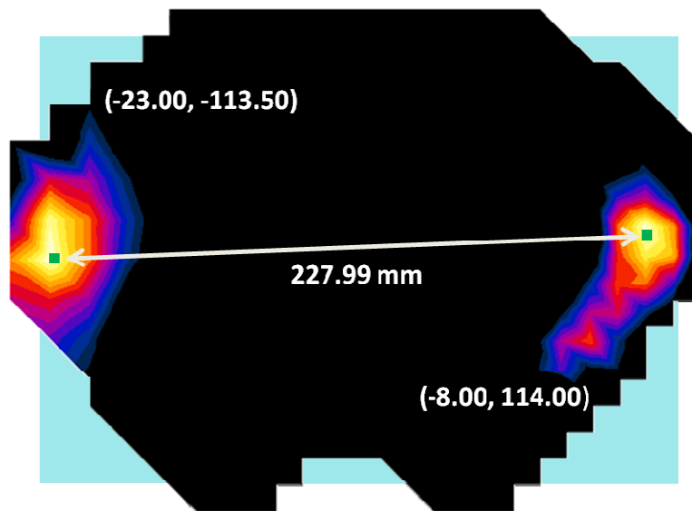
Figure 11-2 Peak SAR Location Plot of UMTS 1900 MHz and 2.4 GHz WLAN
