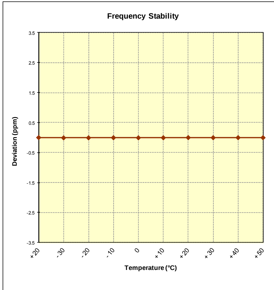
Figure 6-8. Frequency Stability Graph (AWS WCDMA Mode – Ch. 1413)
