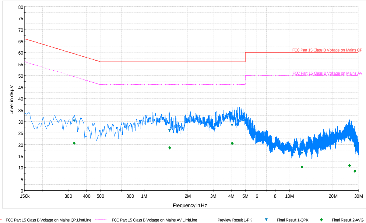
Plot 6-6. Line Conducted Plot with ANT+ (L1)
