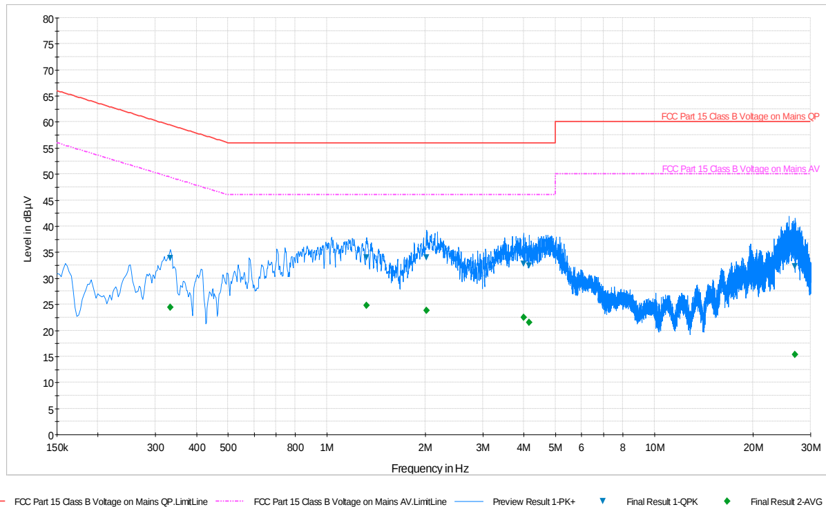
Plot 6-7. Line Conducted Plot with ANT+ (N)
