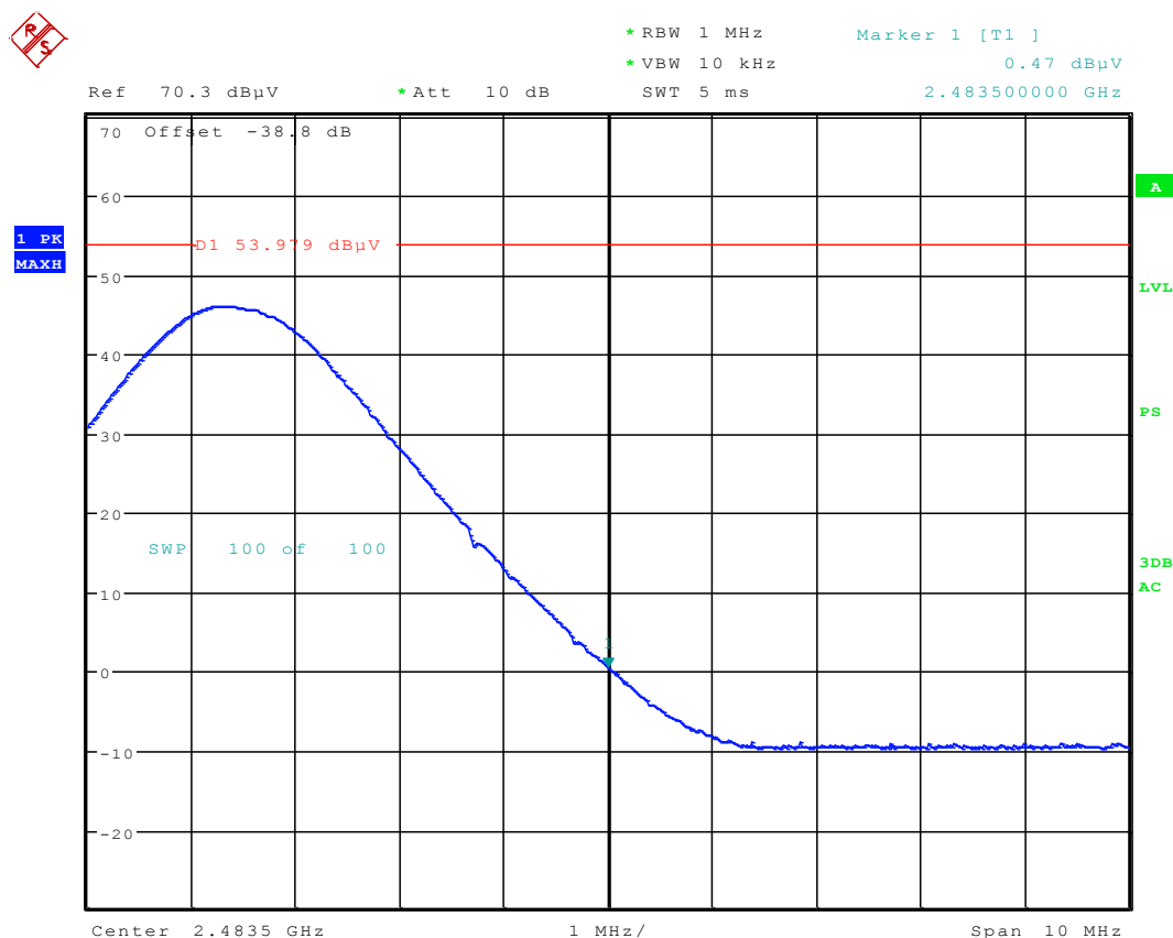
Plot 6-4. Radiated Restricted Upper Band Edge Measurement (Average)
