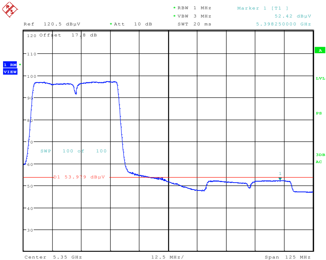
Plot 6-77. Radiated Restricted Upper Band Edge Plot (Average – UNII Band 2A)
