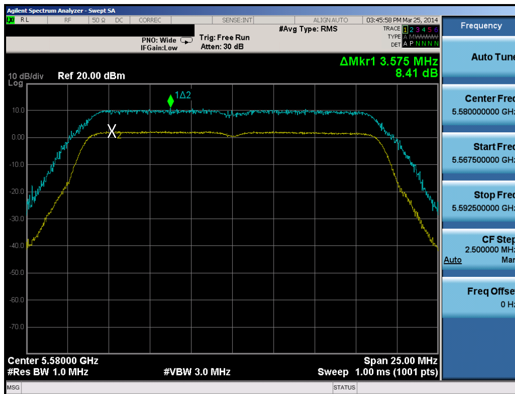
Plot 6-64. Peak Excursion Ratio Plot (20MHz BW 802.11n)
