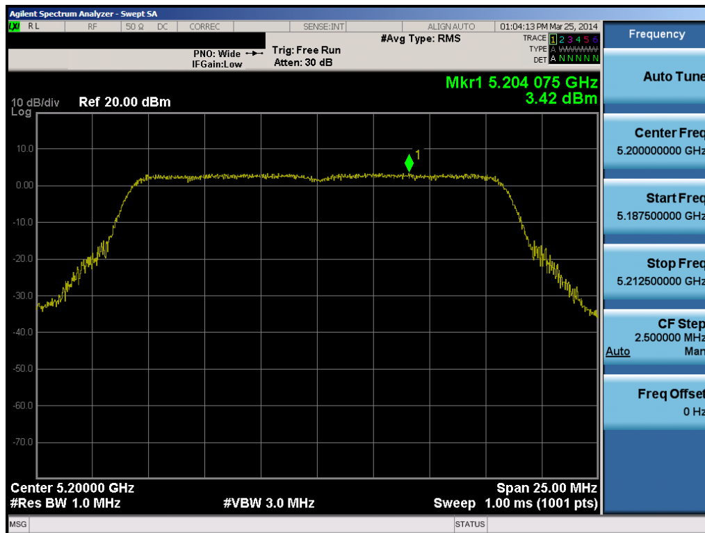
Plot 6-36. Peak Power Spectral Density Plot (802.11a (UNII Band 1) – Ch. 40)
