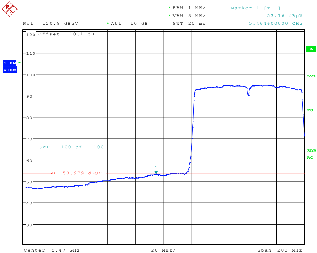
Plot 6-86. Radiated Restricted Lower Band Edge Plot (Average – UNII Band 2C)
