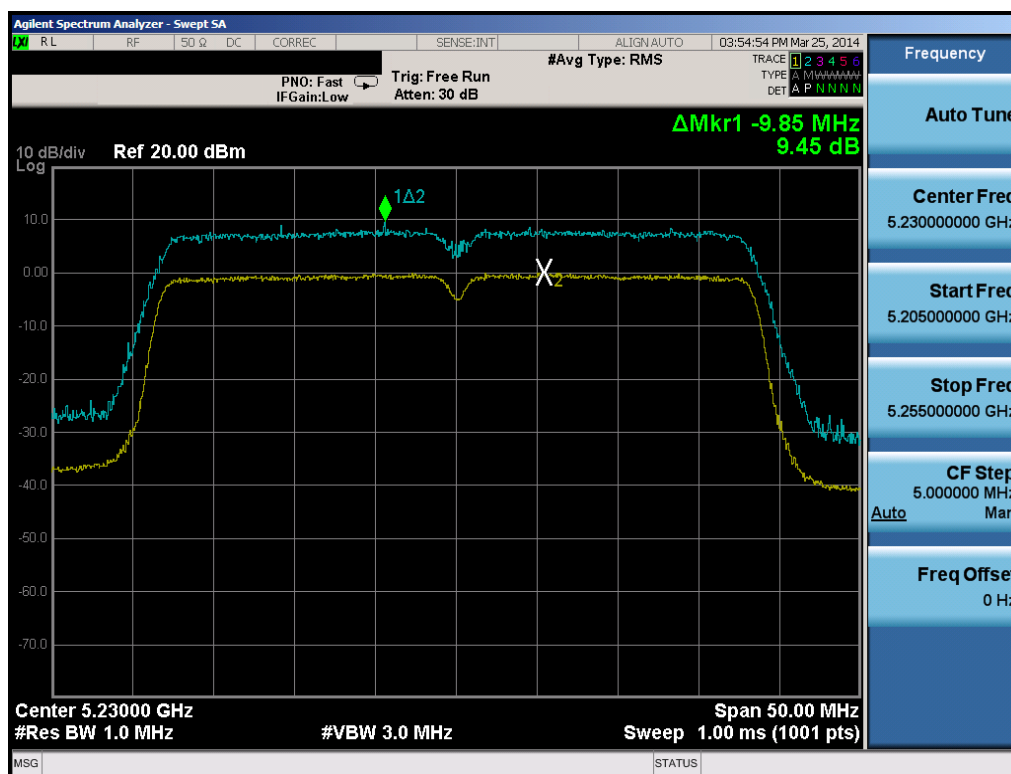
Plot 6-65. Peak Excursion Ratio Plot (40MHz BW 802.11n)
