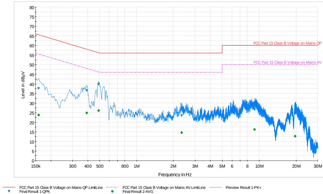
Plot 6-92. Line Conducted Plot with 802.11a UNII Band 2C (L1)
