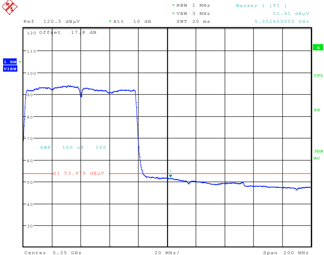
Plot 6-84. Radiated Restricted Upper Band Edge Plot (Average – UNII Band 2A)
