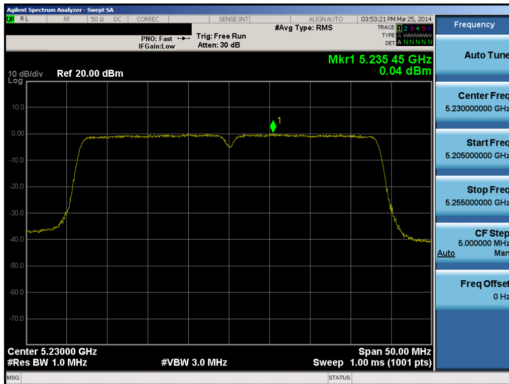
Plot 6-42. Peak Power Spectral Density Plot (40MHz BW 802.11n (UNII Band 1) – Ch. 46)
