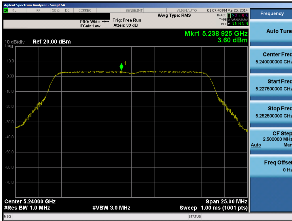
Plot 6-37. Peak Power Spectral Density Plot (802.11a (UNII Band 1) – Ch. 48)
