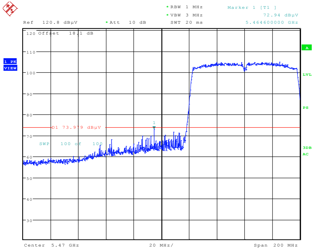
Plot 6-87. Radiated Restricted Lower Band Edge Plot (Peak – UNII Band 2C)
