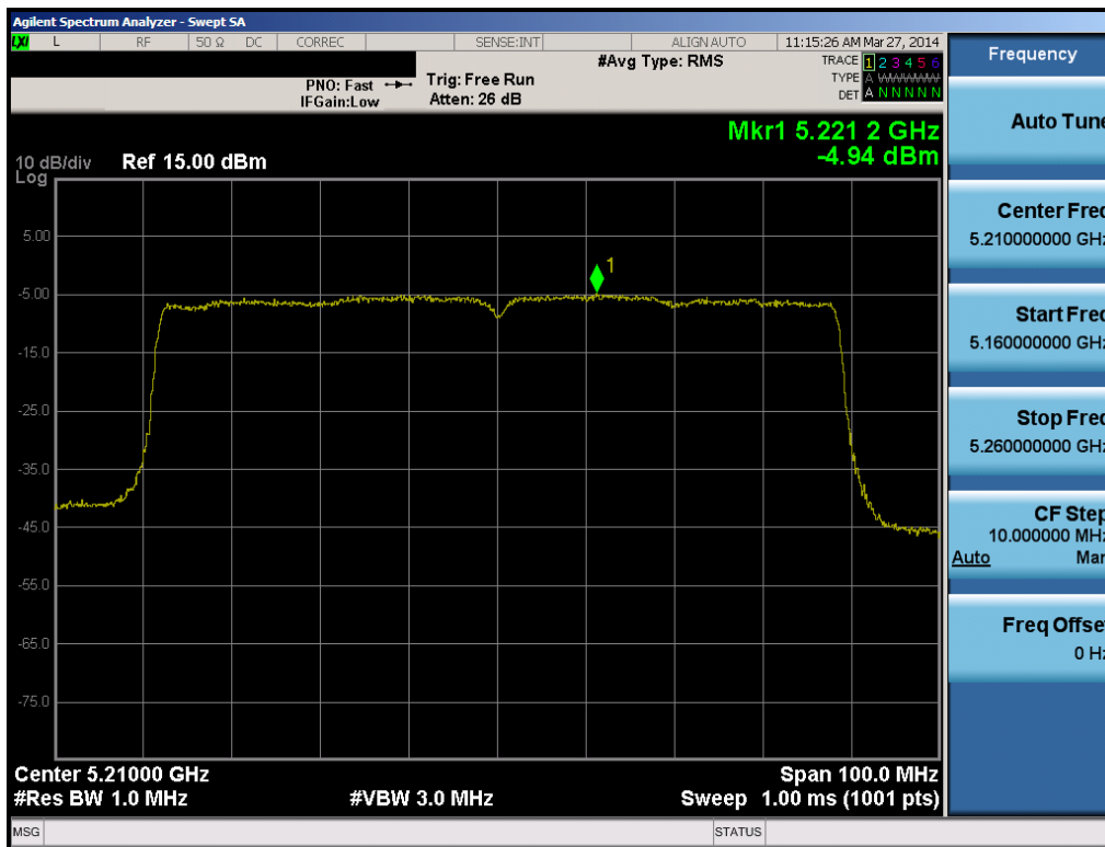
Plot 6-43. Peak Power Spectral Density Plot (80MHz BW 802.11ac (UNII Band 1) – Ch. 42)
