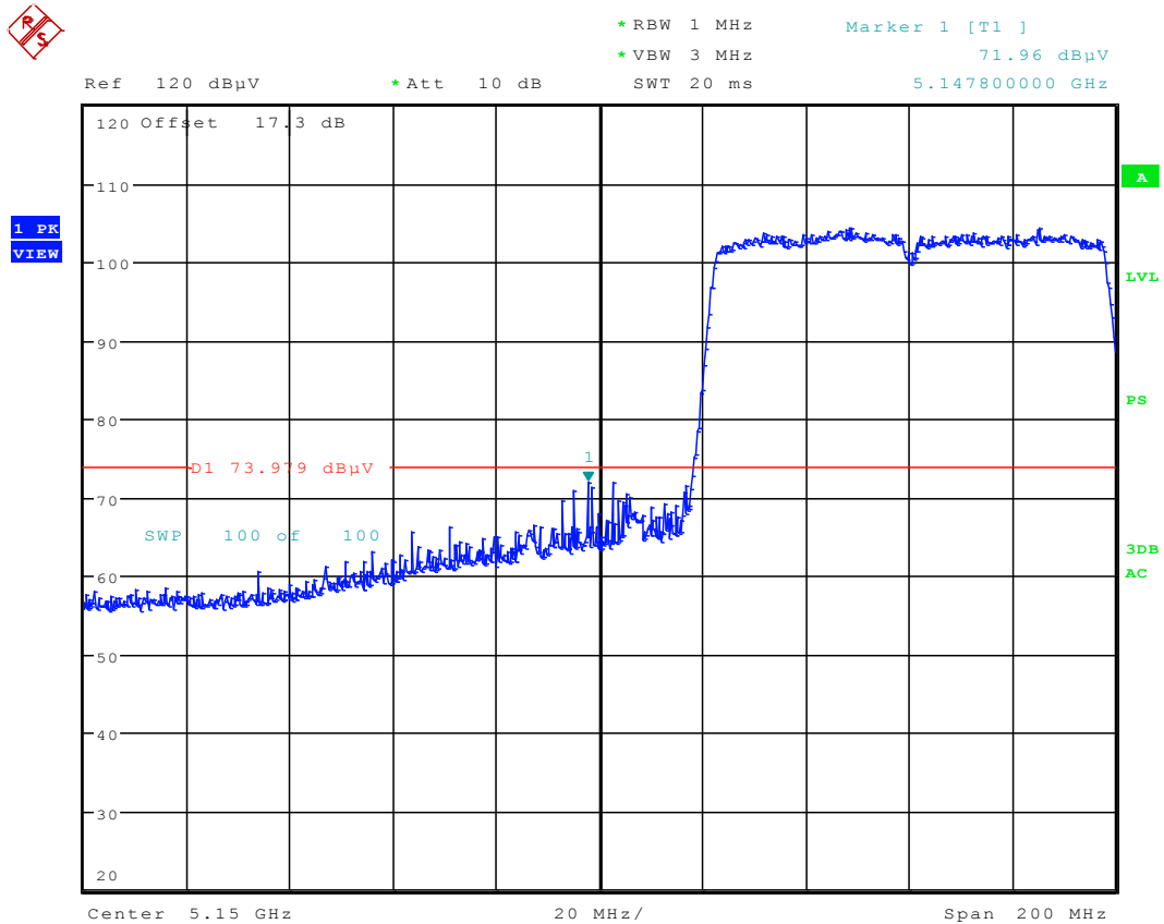
Plot 6-83. Radiated Restricted Lower Band Edge Plot (Peak - UNII Band 1)
