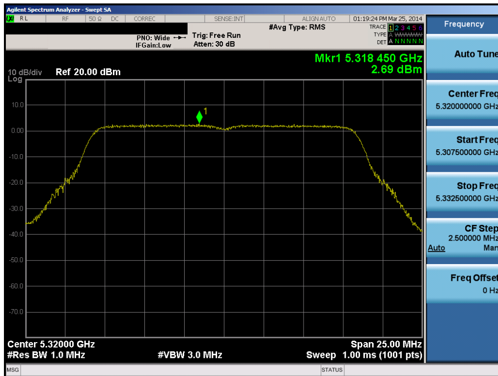
Plot 6-46. Peak Power Spectral Density Plot (802.11a (UNII Band 2A) – Ch. 64)
