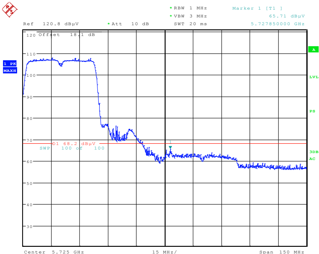
Plot 6-81. Radiated Upper Band Edge Plot (Peak – UNII Band 2C)
