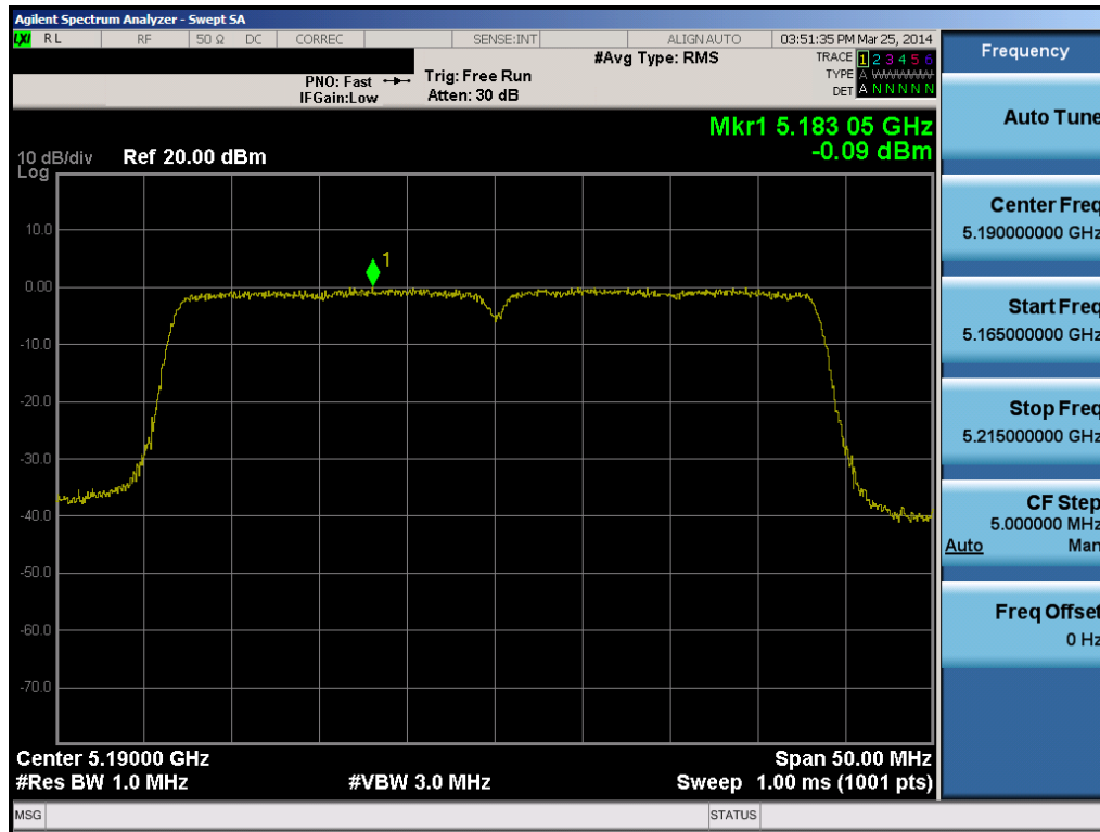
Plot 6-41. Peak Power Spectral Density Plot (40MHz BW 802.11n (UNII Band 1) – Ch. 38)
