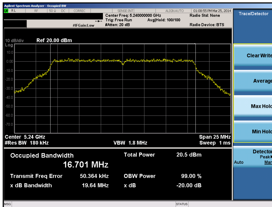
Plot 6-29. 20dB Bandwidth Plot (20MHz BW 802.11a (UNII Band 1) – Ch. 48)
