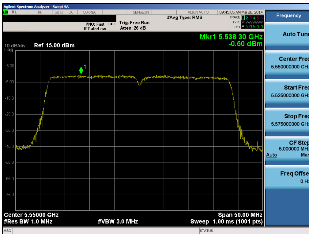
Plot 6-60. Peak Power Spectral Density Plot (40MHz BW 802.11n (UNII Band 2C) – Ch. 110)
