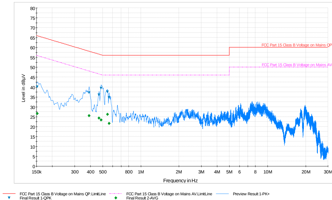
Plot 6-91. Line Conducted Plot with 802.11a UNII Band 2A (N)
