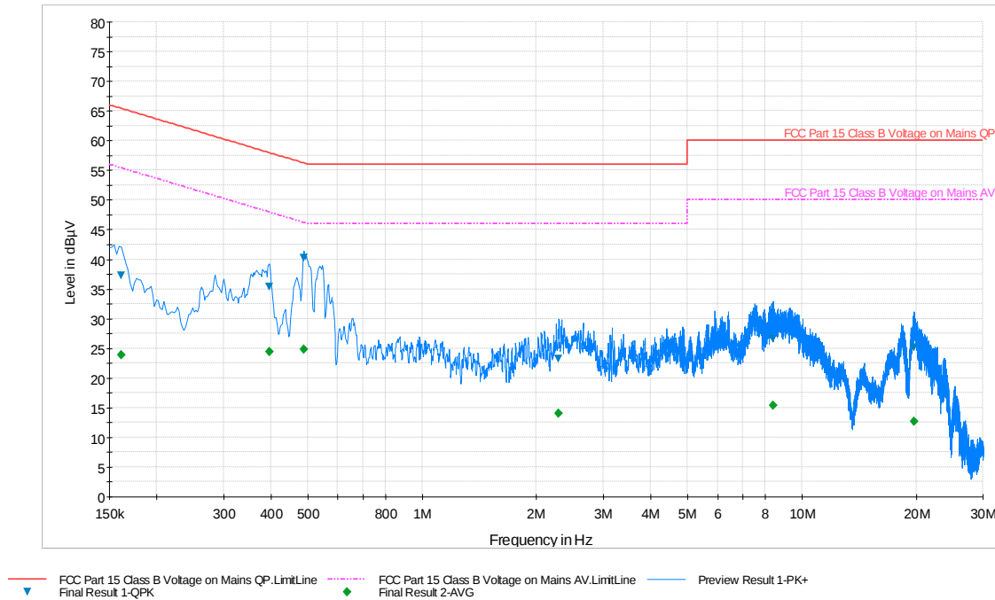
Plot 6-88. Line Conducted Plot with 802.11a UNII Band 1 (L1)
