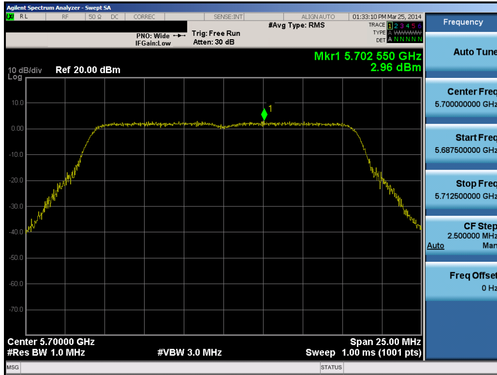
Plot 6-55. Peak Power Spectral Density Plot (802.11a (UNII Band 2C) – Ch. 140)
