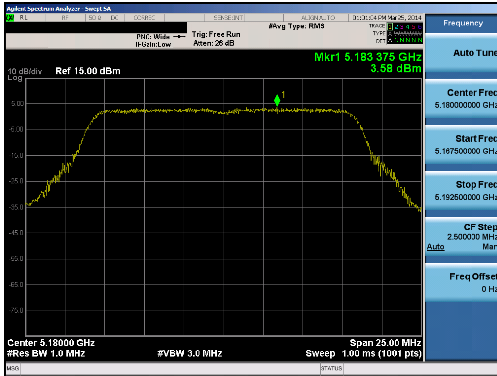
Plot 6-35. Peak Power Spectral Density Plot (802.11a (UNII Band 1) – Ch. 36)
