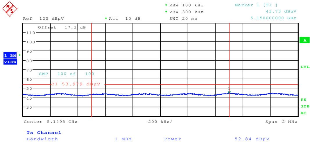
Plot 6-75. Radiated Restricted Lower Band Edge Plot (Average - UNII Band 1)
