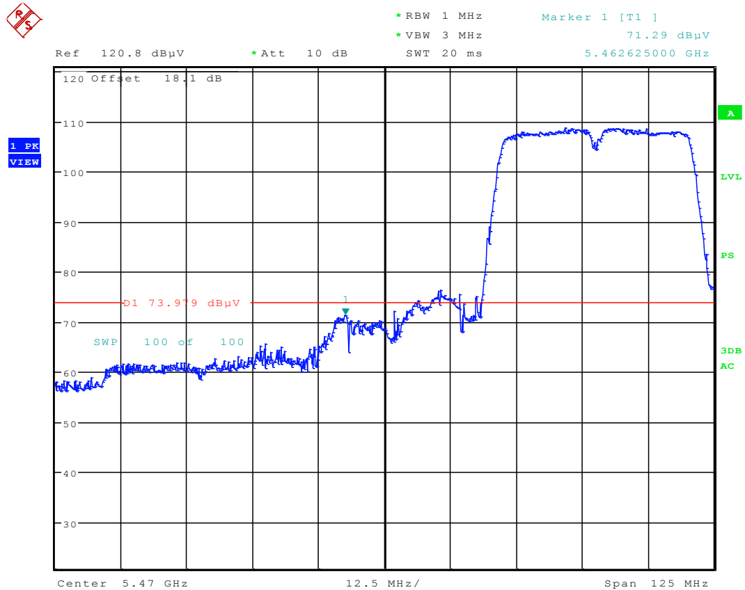
Plot 6-80. Radiated Restricted Lower Band Edge Plot (Peak – UNII Band 2C)
