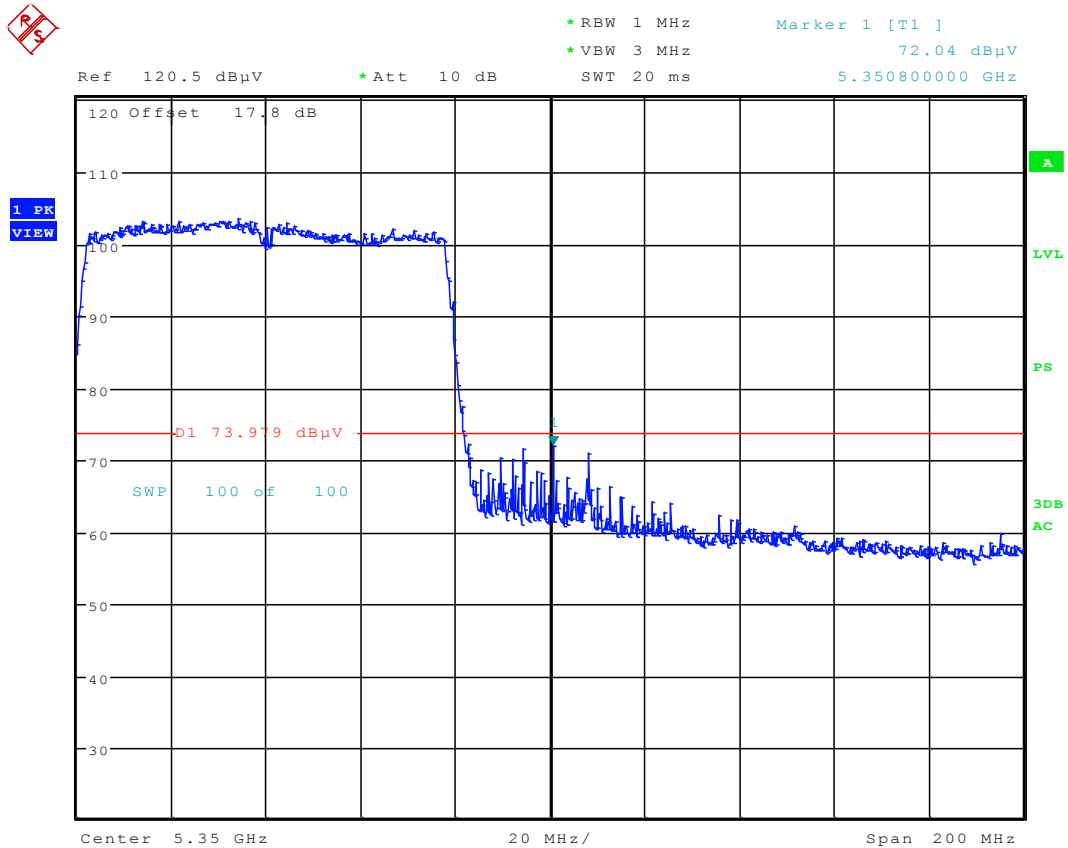
Plot 6-85. Radiated Restricted Upper Band Edge Plot (Peak – UNII Band 2A)
