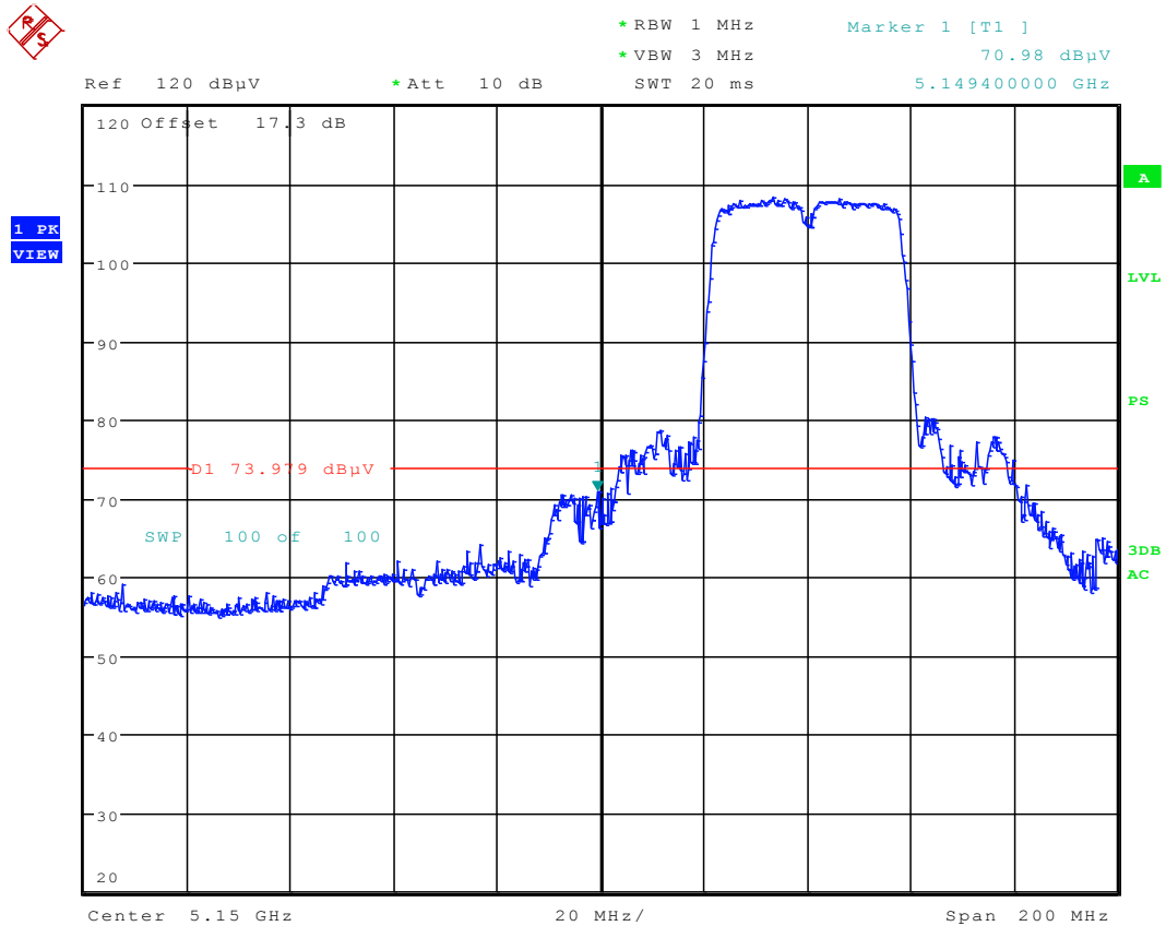
Plot 6-76. Radiated Restricted Lower Band Edge Plot (Peak – UNII Band 1)
