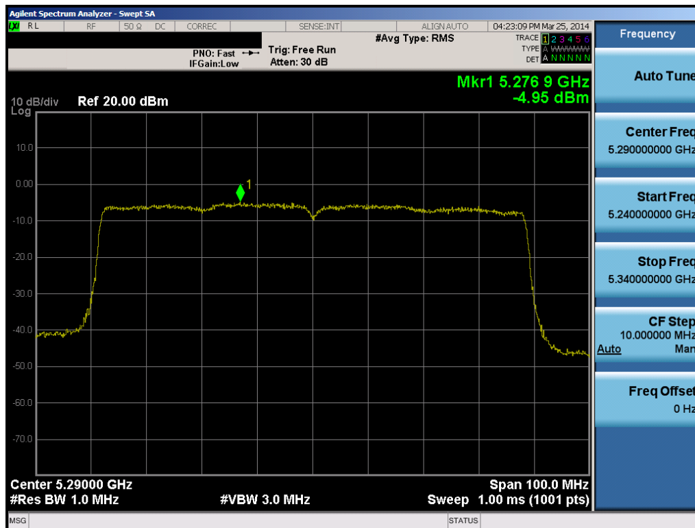
Plot 6-52. Peak Power Spectral Density Plot (80MHz BW 802.11ac (UNII Band 2A) – Ch. 58)
