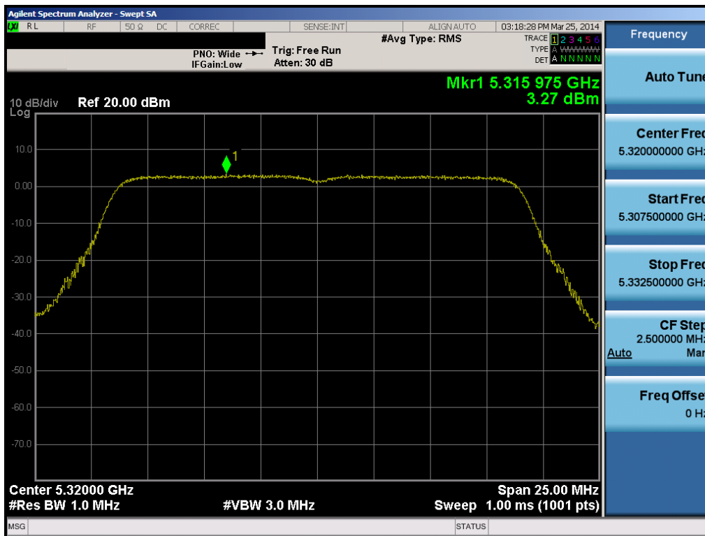
Plot 6-49. Peak Power Spectral Density Plot (20MHz BW 802.11n (UNII Band 2A) – Ch. 64)
