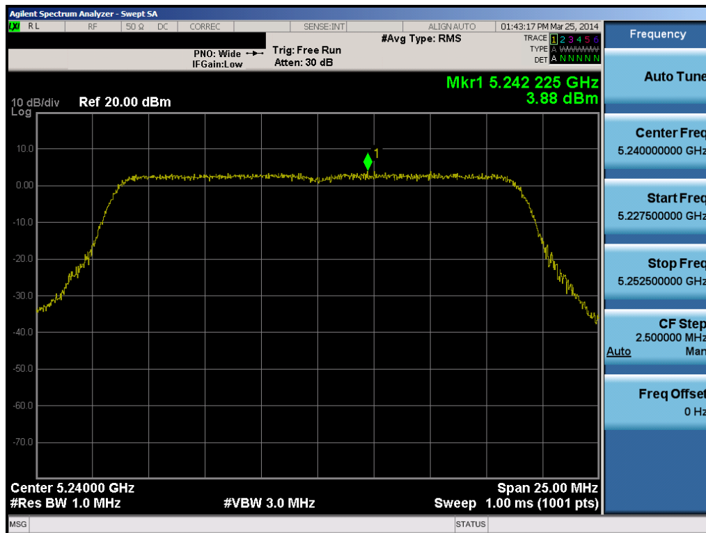
Plot 6-40. Peak Power Spectral Density Plot (20MHz BW 802.11n (UNII Band 1) – Ch. 48)
