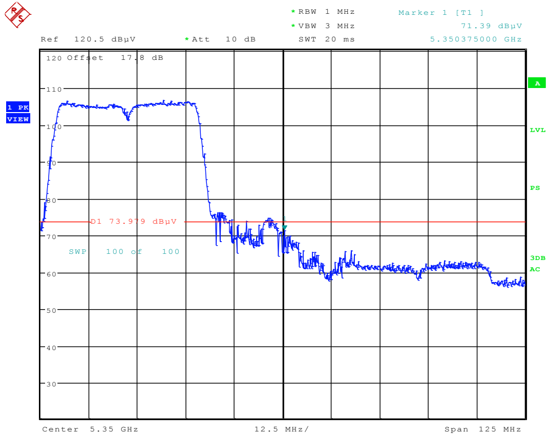
Plot 6-78. Radiated Restricted Upper Band Edge Plot (Peak – UNII Band 2A)
