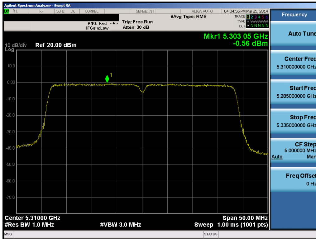
Plot 6-51. Peak Power Spectral Density Plot (40MHz BW 802.11n (UNII Band 2A) – Ch. 62)
