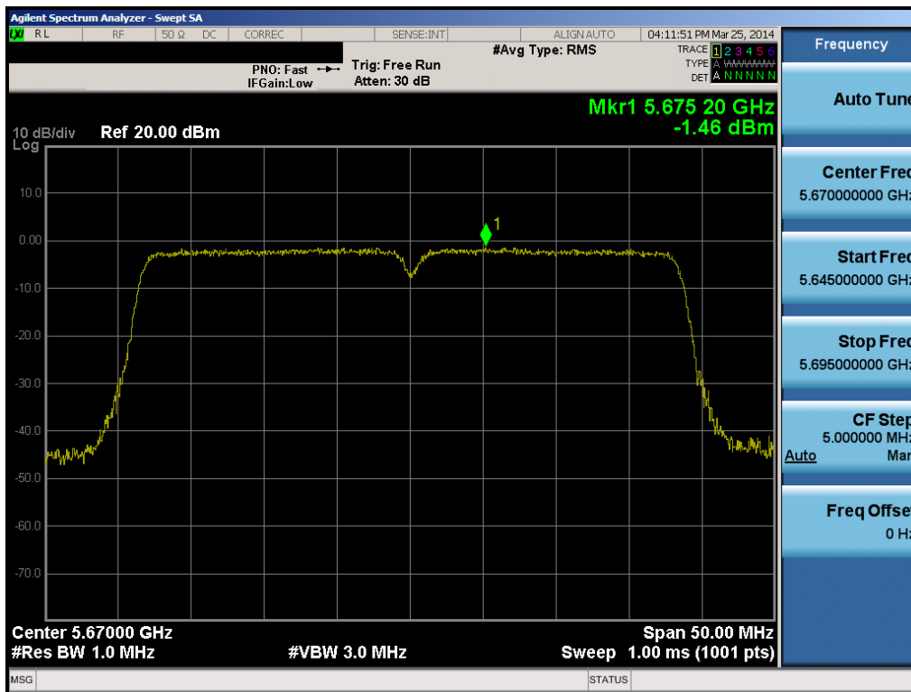
Plot 6-61. Peak Power Spectral Density Plot (40MHz BW 802.11n (UNII Band 2C) – Ch. 134)
