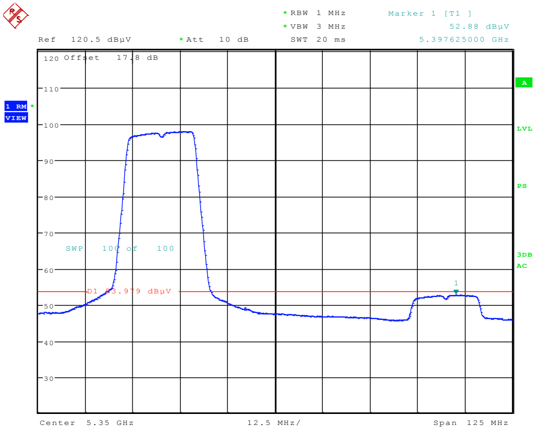
Plot 6-69. Radiated Restricted Upper Band Edge Plot (Average – UNII Band 2A)
