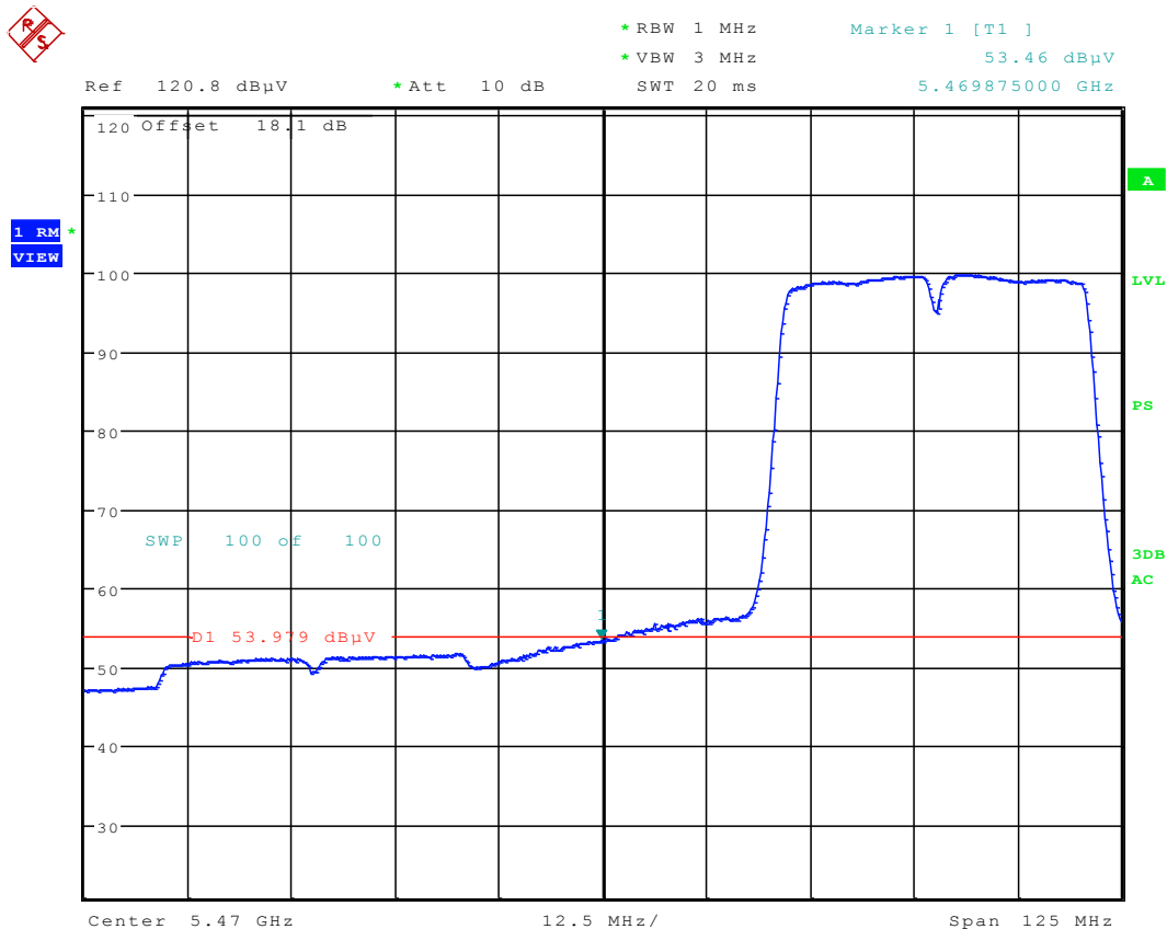
Plot 6-79. Radiated Restricted Lower Band Edge Plot (Average – UNII Band 2C)
