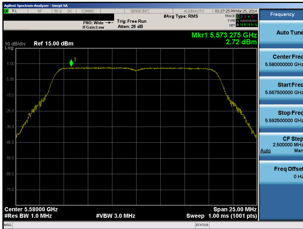
Plot 6-54. Peak Power Spectral Density Plot (802.11a (UNII Band 2C) – Ch. 116)
