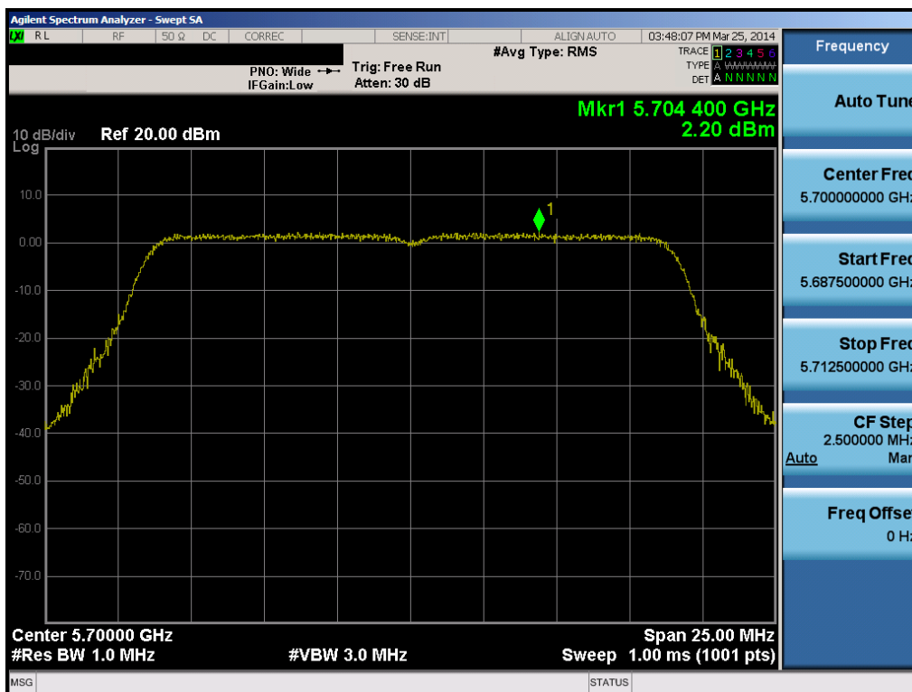
Plot 6-58. Peak Power Spectral Density Plot (20MHz BW 802.11n (UNII Band 2C) – Ch. 140)
