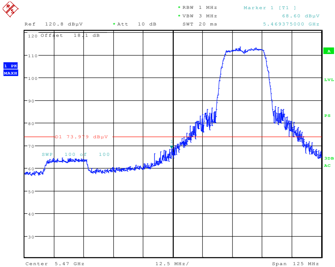
Plot 6-72. Radiated Restricted Lower Band Edge Plot (Peak – UNII Band 2C)
