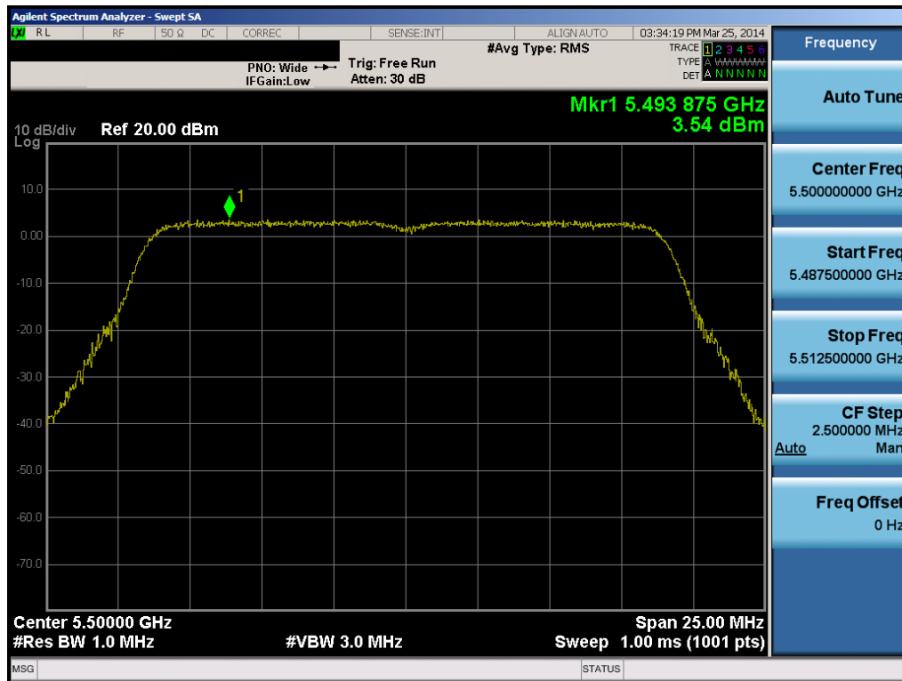
Plot 6-56. Peak Power Spectral Density Plot (20MHz BW 802.11n (UNII Band 2C) – Ch. 100)
