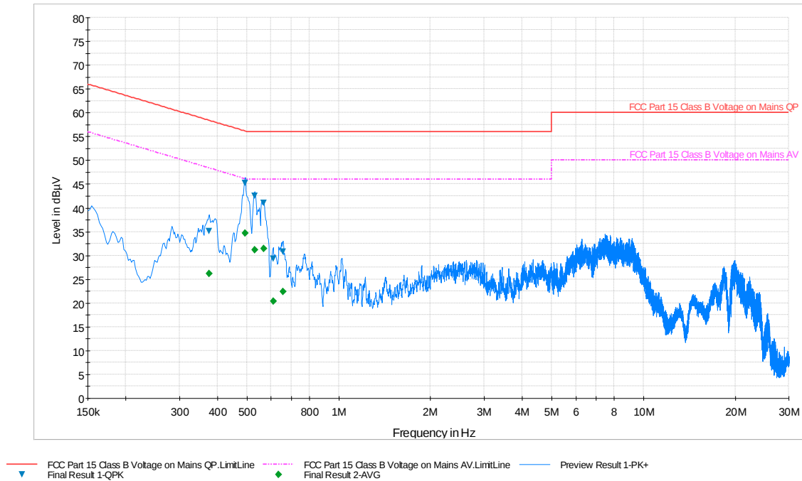
Plot 6-93. Line Conducted Plot with 802.11a UNII Band 2C (N)
