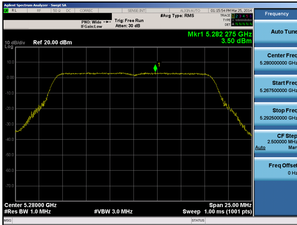
Plot 6-45. Peak Power Spectral Density Plot (802.11a (UNII Band 2A) – Ch. 56)
