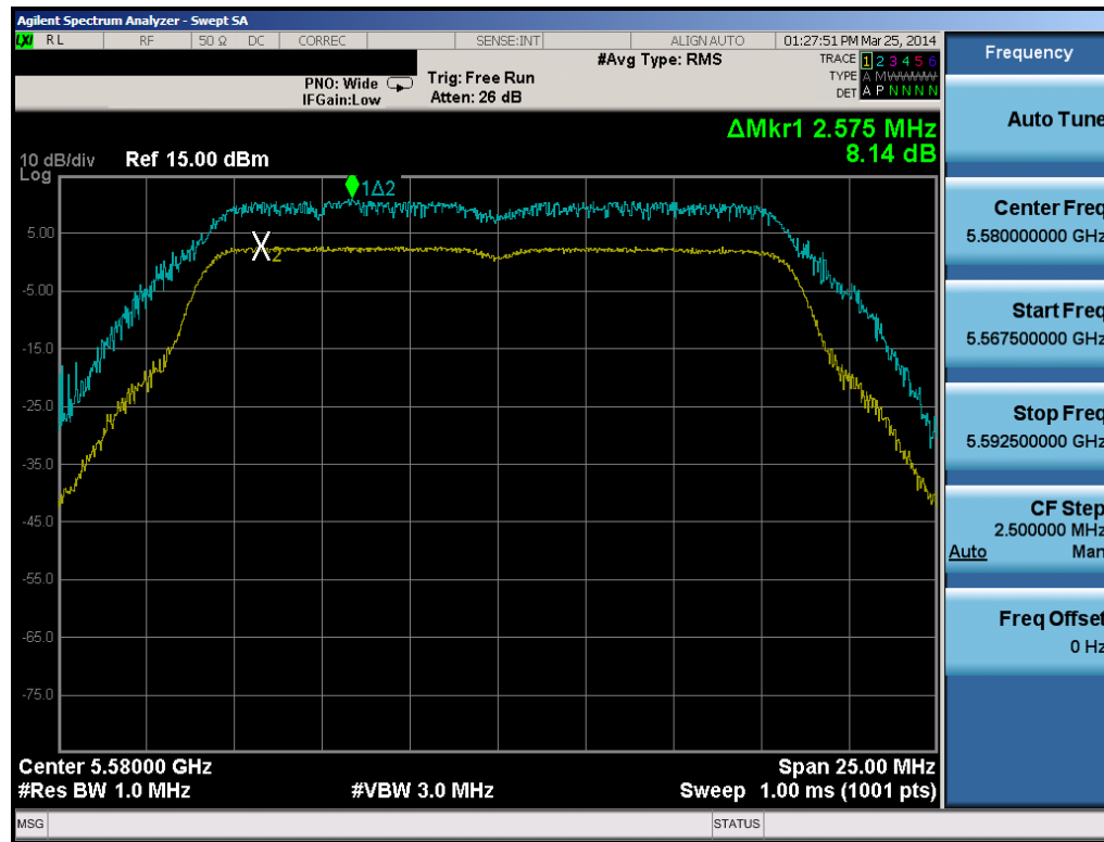
Plot 6-63. Peak Excursion Ratio Plot (802.11a)
