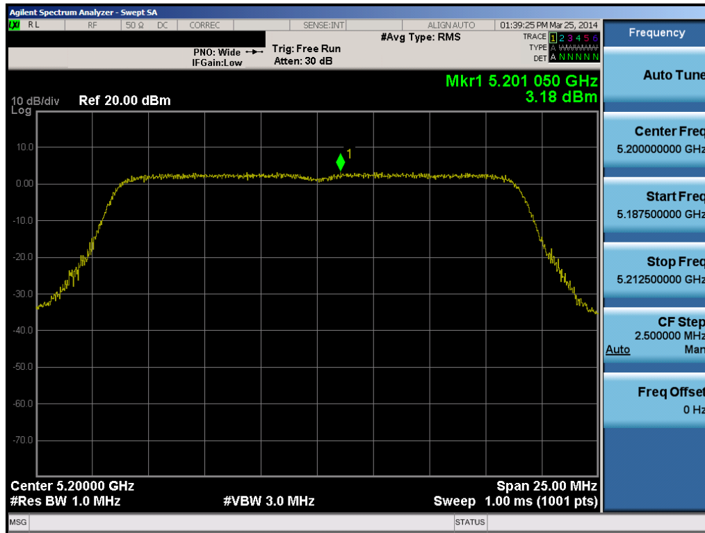
Plot 6-39. Peak Power Spectral Density Plot (20MHz BW 802.11n (UNII Band 1) – Ch. 40)
