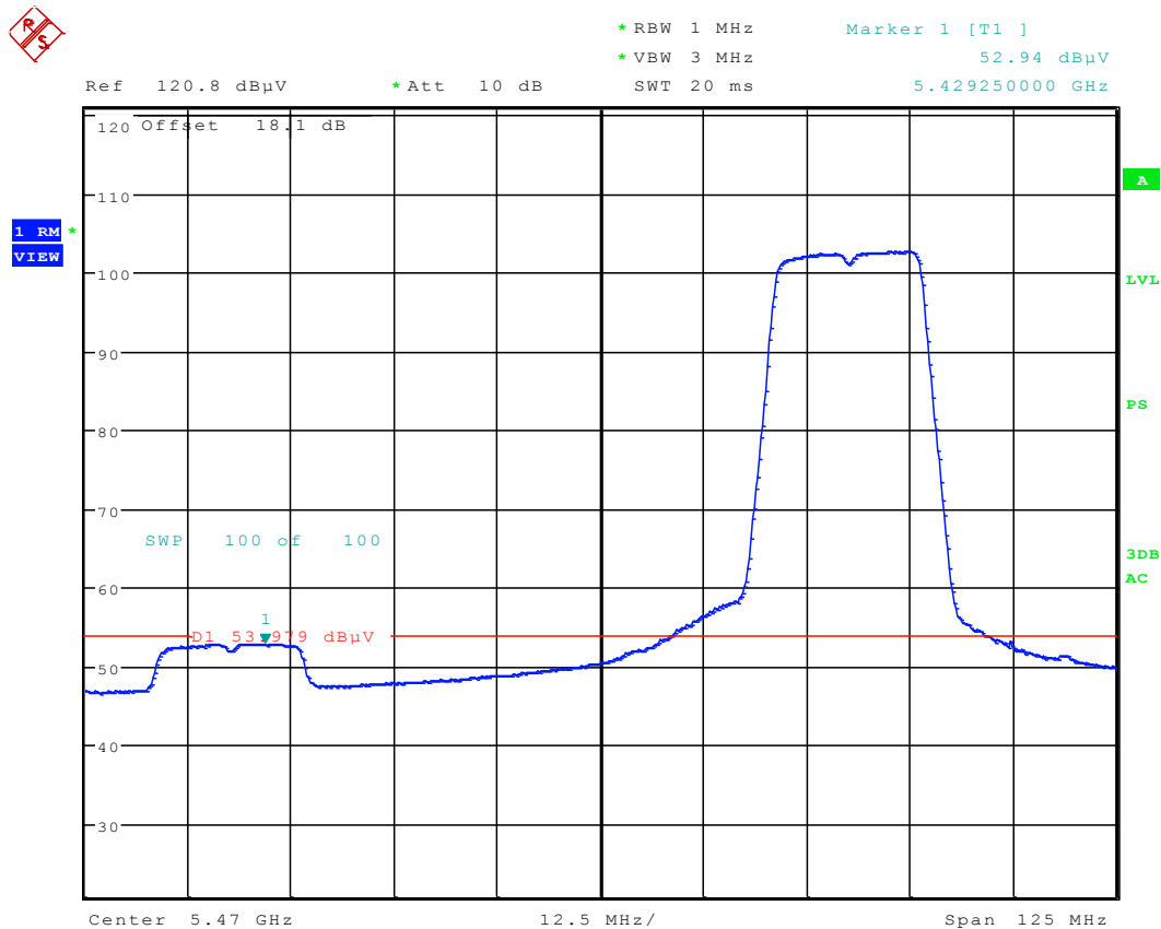
Plot 6-71. Radiated Restricted Lower Band Edge Plot (Average – UNII Band 2C)
