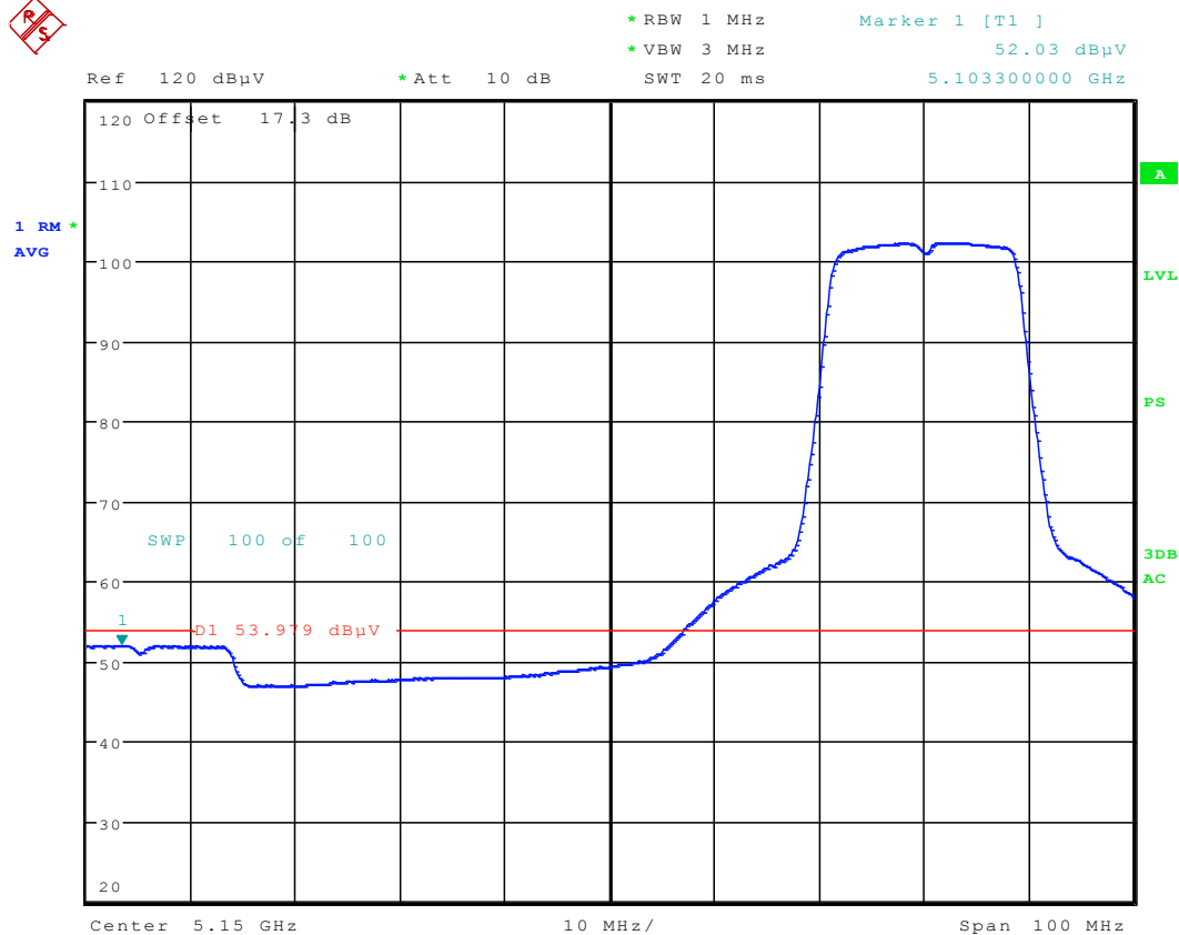
Plot 6-67. Radiated Restricted Lower Band Edge Plot (Average – UNII Band 1)
