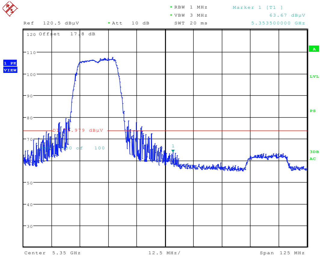
Plot 6-70. Radiated Restricted Upper Band Edge Plot (Peak – UNII Band 2A)
