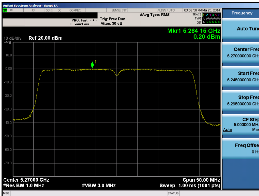
Plot 6-50. Peak Power Spectral Density Plot (40MHz BW 802.11n (UNII Band 2A) – Ch. 54)
