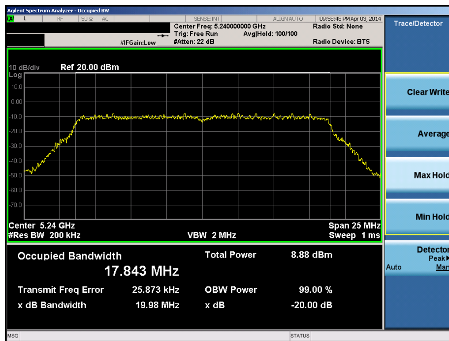
Plot 6-30. 20dB Bandwidth Plot (20MHz BW 802.11n (UNII Band 1) – Ch. 48)
