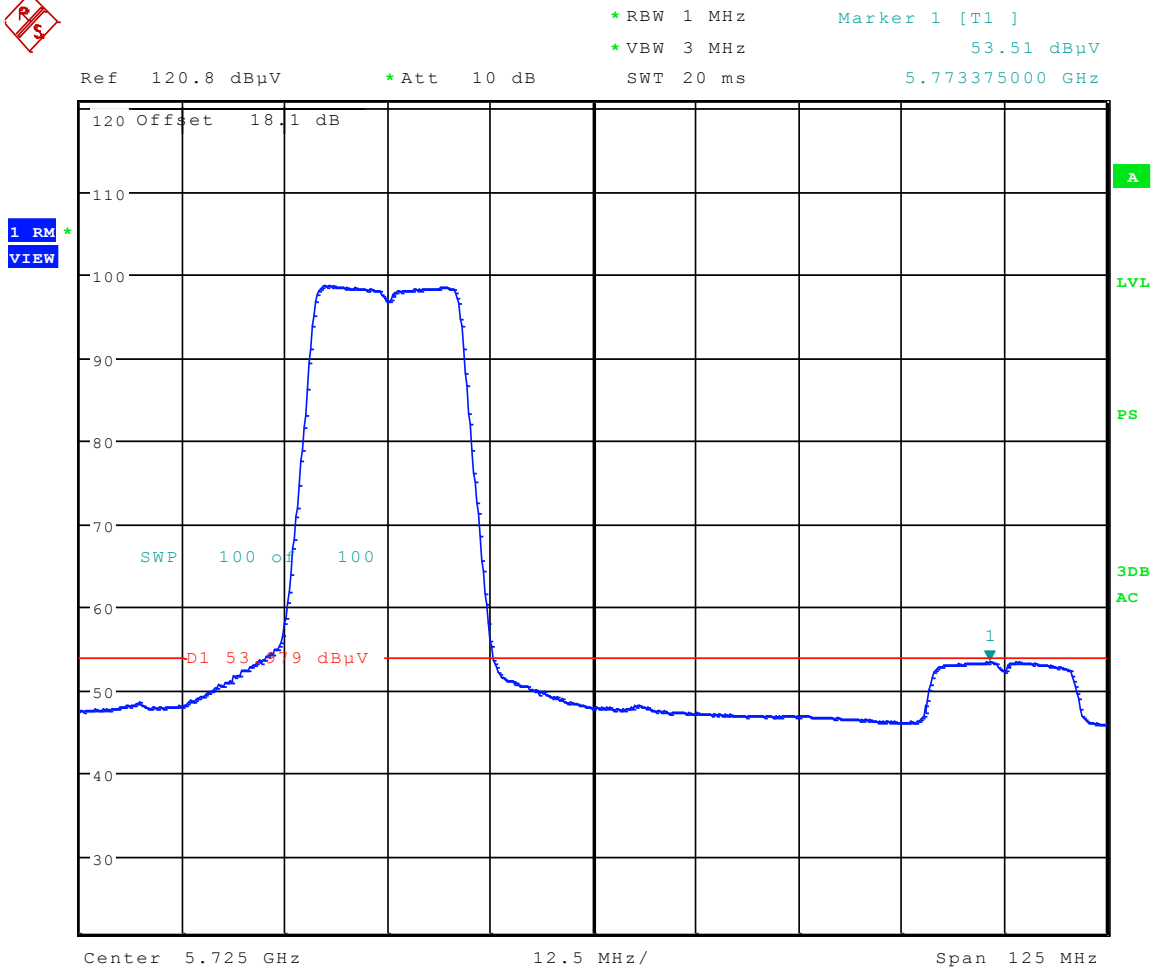
Plot 6-73. Radiated Upper Band Edge Plot (Average – UNII Band 2C)
