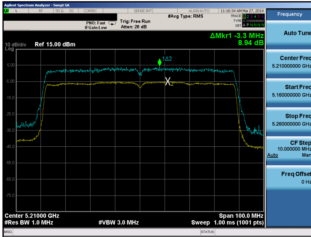
Plot 6-66. Peak Excursion Ratio Plot (80MHz BW 802.11ac)
