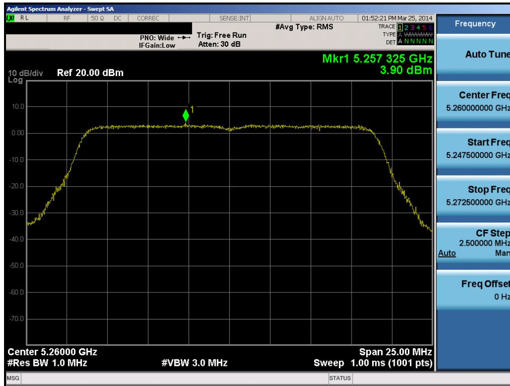
Plot 6-47. Peak Power Spectral Density Plot (20MHz BW 802.11n (UNII Band 2A) – Ch. 52)
