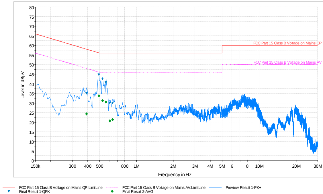
Plot 6-89. Line Conducted Plot with 802.11a UNII Band 1 (N)
