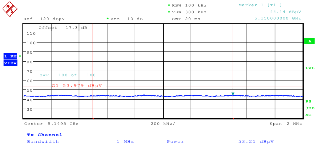
Plot 6-82. Radiated Restricted Lower Band Edge Plot (Average – UNII Band 1)
