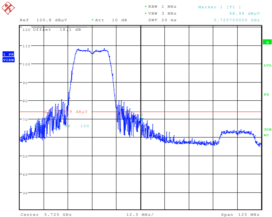
Plot 6-74. Radiated Upper Band Edge Plot (Peak – UNII Band 2C)
