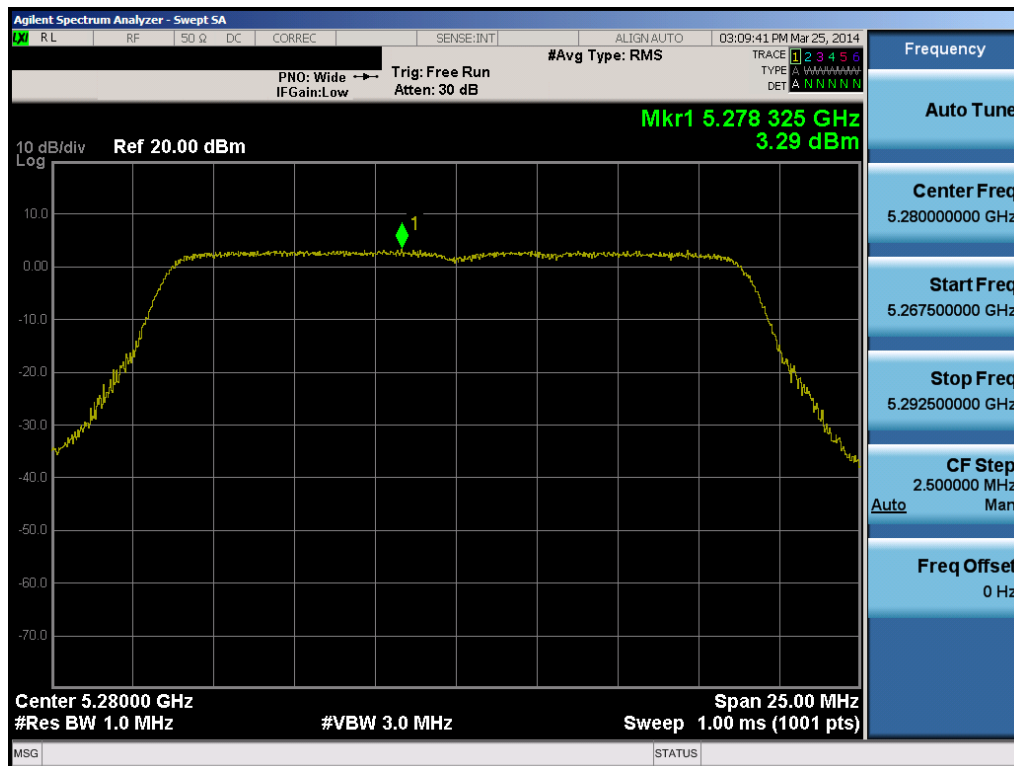
Plot 6-48. Peak Power Spectral Density Plot (20MHz BW 802.11n (UNII Band 2A) – Ch. 56)
