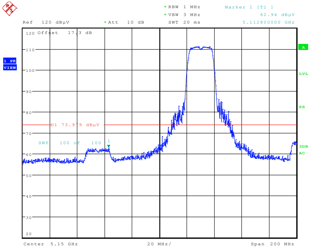
Plot 6-68. Radiated Restricted Lower Band Edge Plot (Peak – UNII Band 1)
