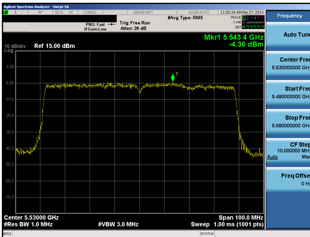
Plot 6-62. Peak Power Spectral Density Plot (80MHz BW 802.11ac (UNII Band 2C) – Ch. 106)
