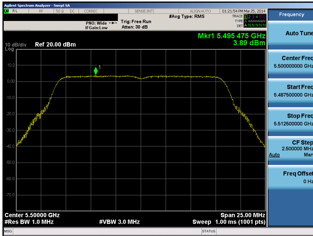
Plot 6-53. Peak Power Spectral Density Plot (802.11a (UNII Band 2C) – Ch. 100)
