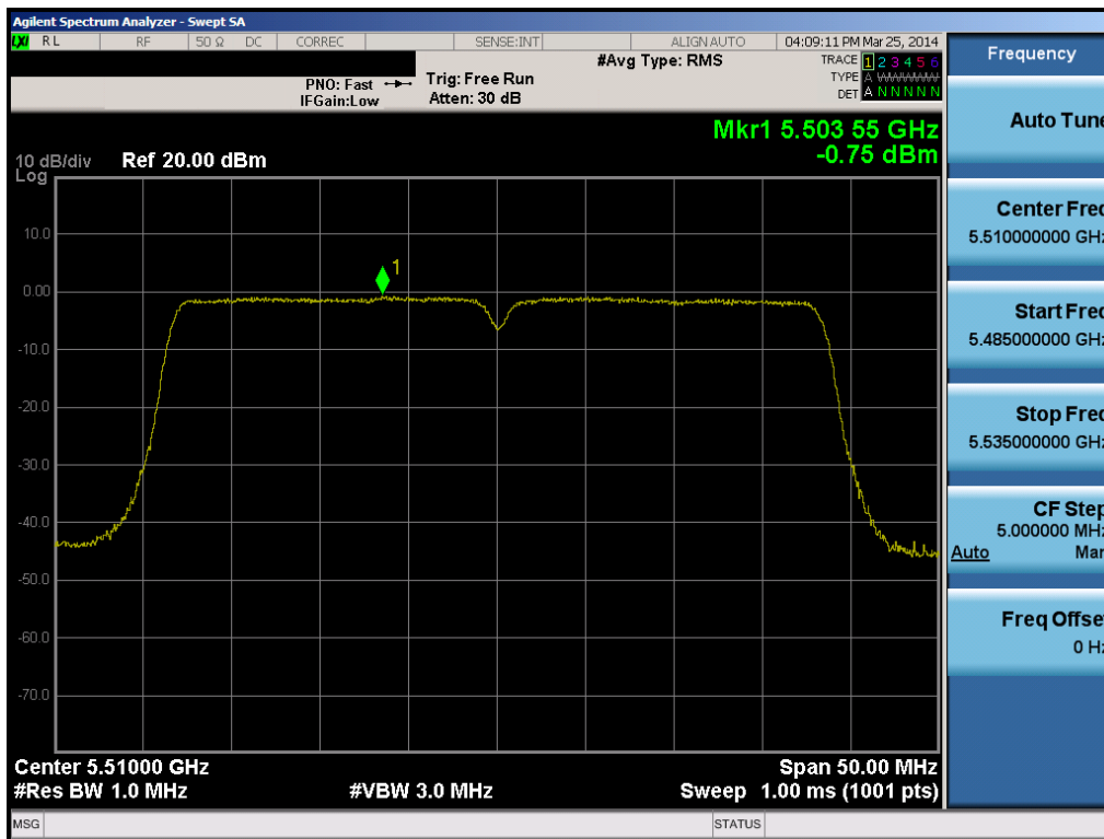
Plot 6-59. Peak Power Spectral Density Plot (40MHz BW 802.11n (UNII Band 2C) – Ch. 102)
