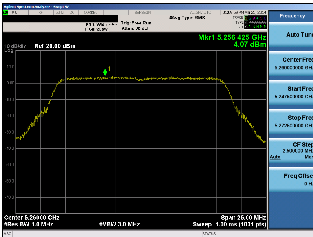
Plot 6-44. Peak Power Spectral Density Plot (802.11a (UNII Band 2A) – Ch. 52)
