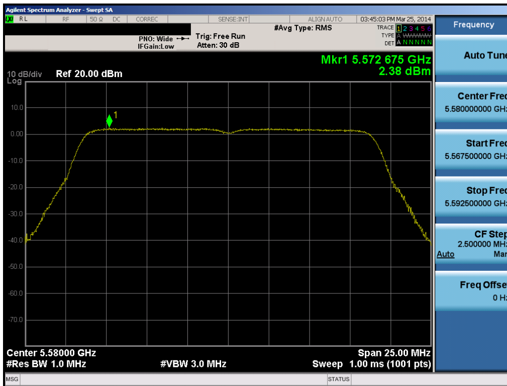
Plot 6-57. Peak Power Spectral Density Plot (20MHz BW 802.11n (UNII Band 2C) – Ch. 116)
