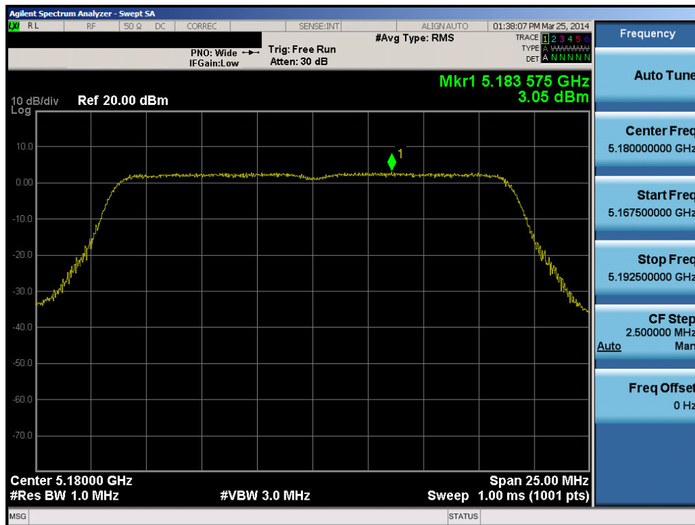
Plot 6-38. Peak Power Spectral Density Plot (20MHz BW 802.11n (UNII Band 1) – Ch. 36)
