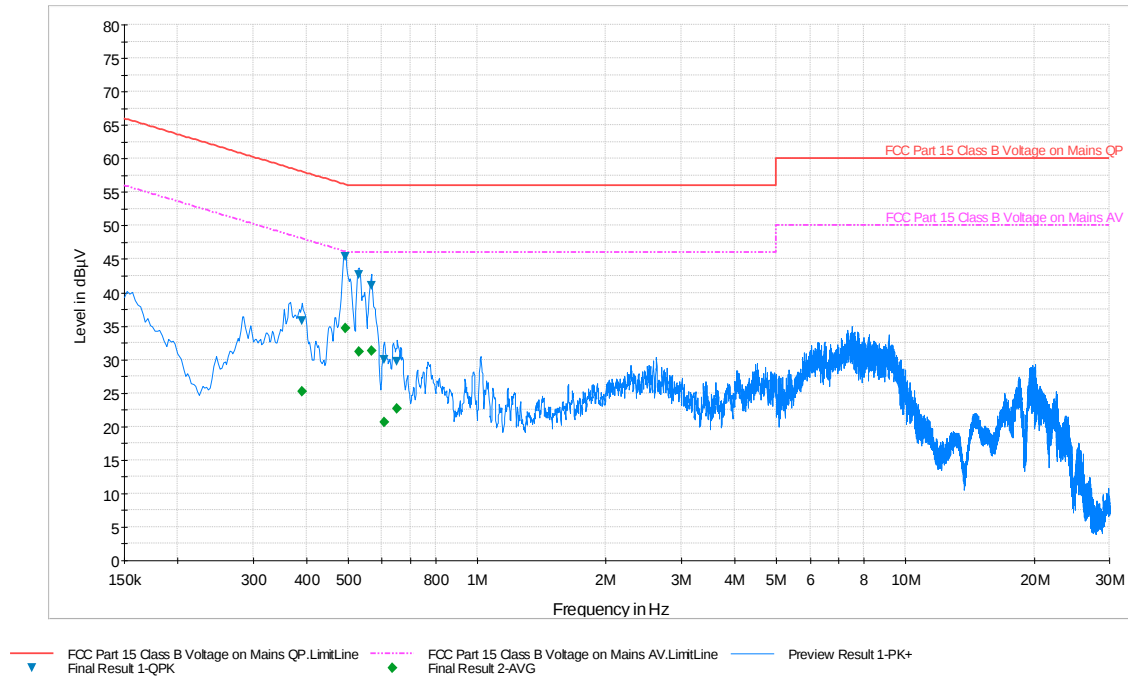
Plot 6-90. Line Conducted Plot with 802.11a UNII Band 2A (L1)
