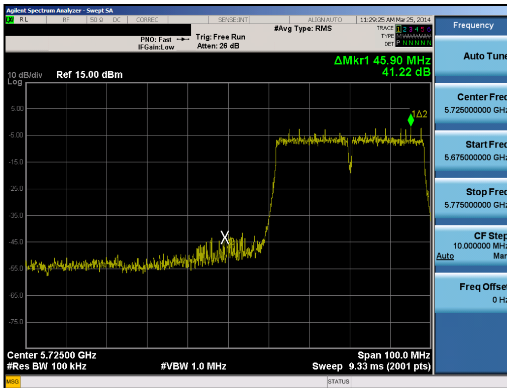
Plot 6-47. Band Edge Plot (40MHz BW 802.11n (5.8GHz) – Ch. 151)
