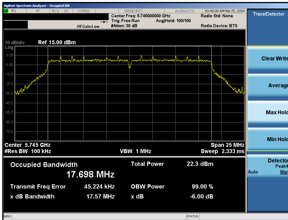
Plot 6-13. 6dB Bandwidth Plot (20MHz BW 802.11n (5.8GHz) – Ch. 149)
