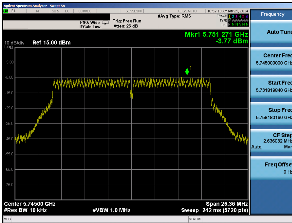
Plot 6-31. Power Spectral Density Plot (20MHz BW 802.11n (5.8GHz) – Ch. 149)
