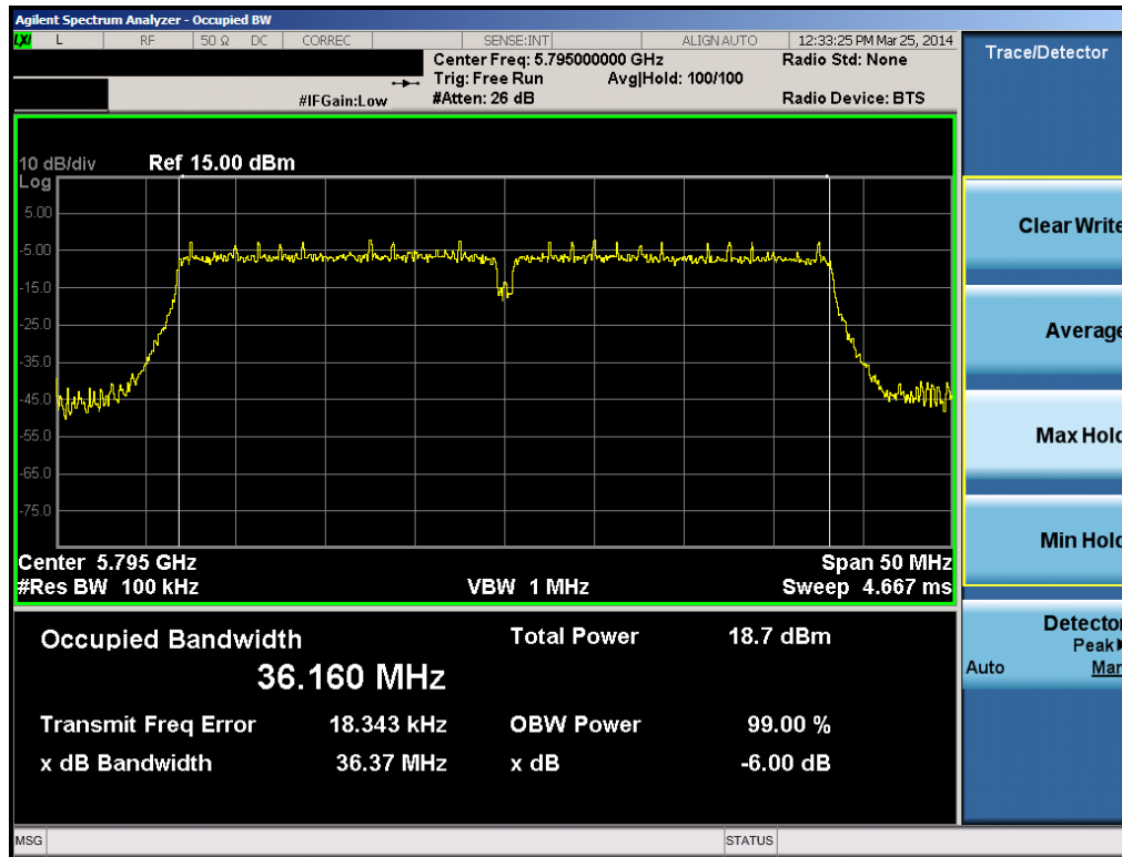
Plot 6-17. 6dB Bandwidth Plot (40MHz BW 802.11n (5.8GHz) – Ch. 159)
