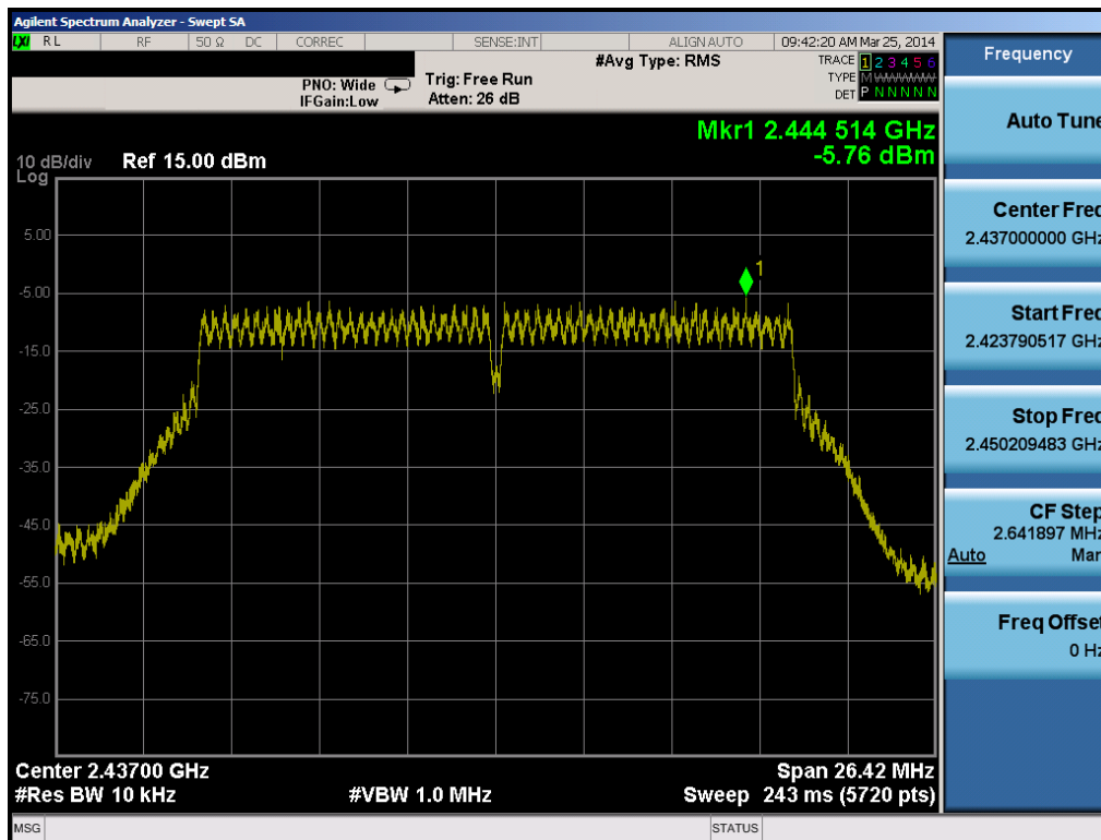
Plot 6-26. Power Spectral Density Plot (802.11n (2.4GHz) – Ch. 6)
