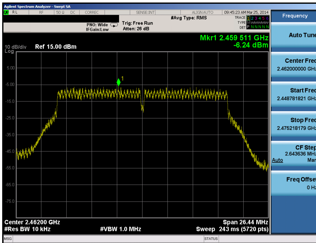
Plot 6-27. Power Spectral Density Plot (802.11n (2.4GHz) – Ch. 11)
