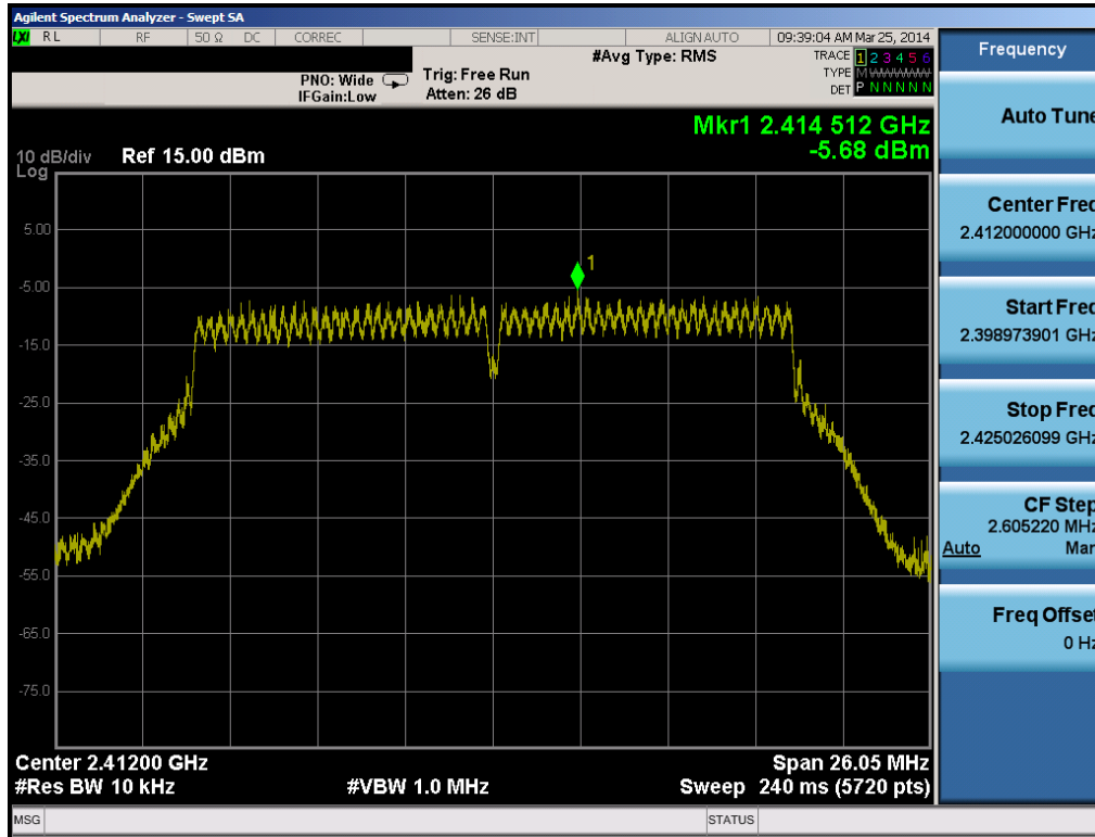
Plot 6-25. Power Spectral Density Plot (802.11n (2.4GHz) – Ch. 1)
