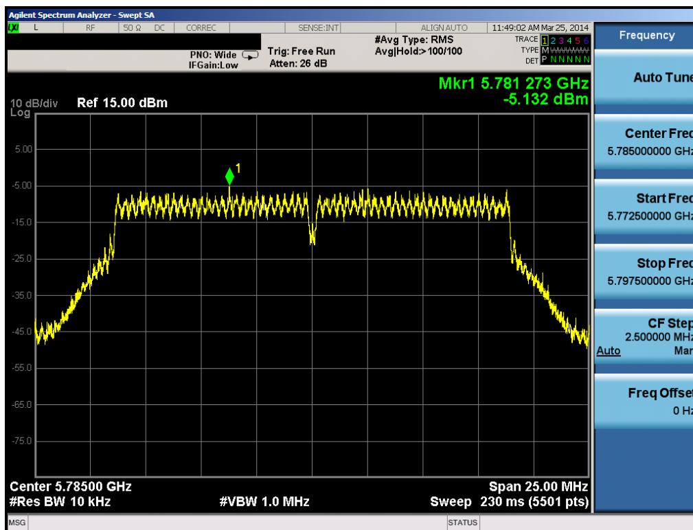
Plot 6-32. Power Spectral Density Plot (20MHz BW 802.11n (5.8GHz) – Ch. 157)
