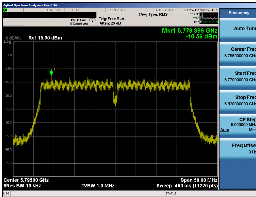
Plot 6-35. Power Spectral Density Plot (40MHz BW 802.11n (5.8GHz) – Ch. 159)
