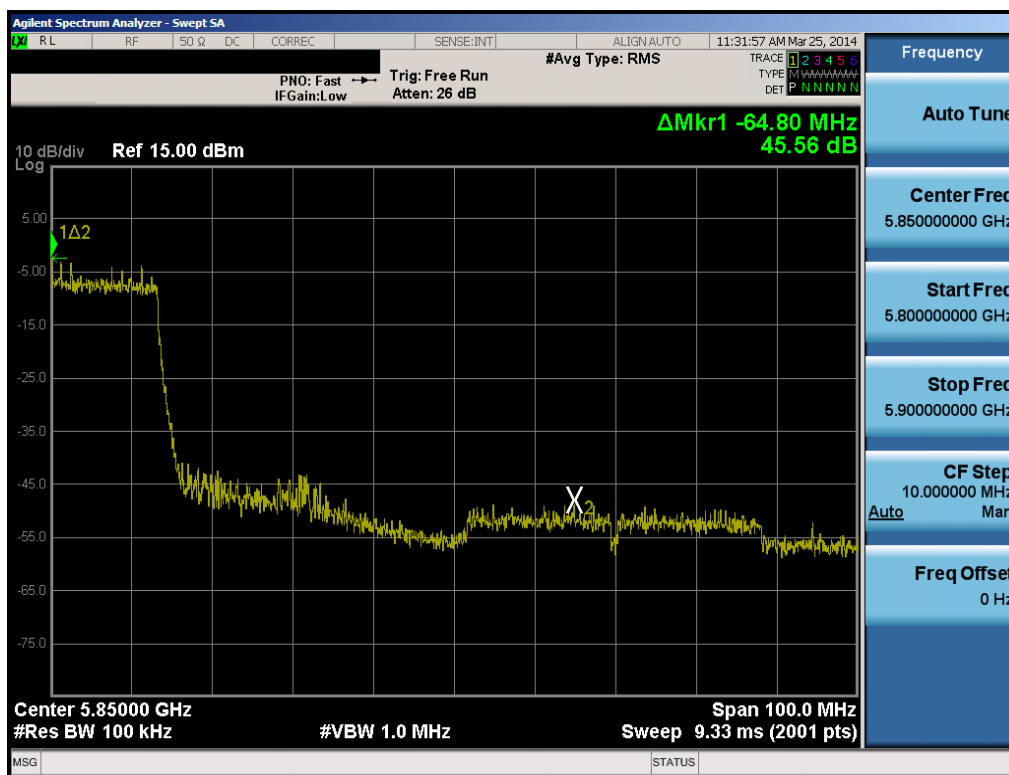
Plot 6-48. Band Edge Plot (40MHz BW 802.11n (5.8GHz) – Ch. 159)
