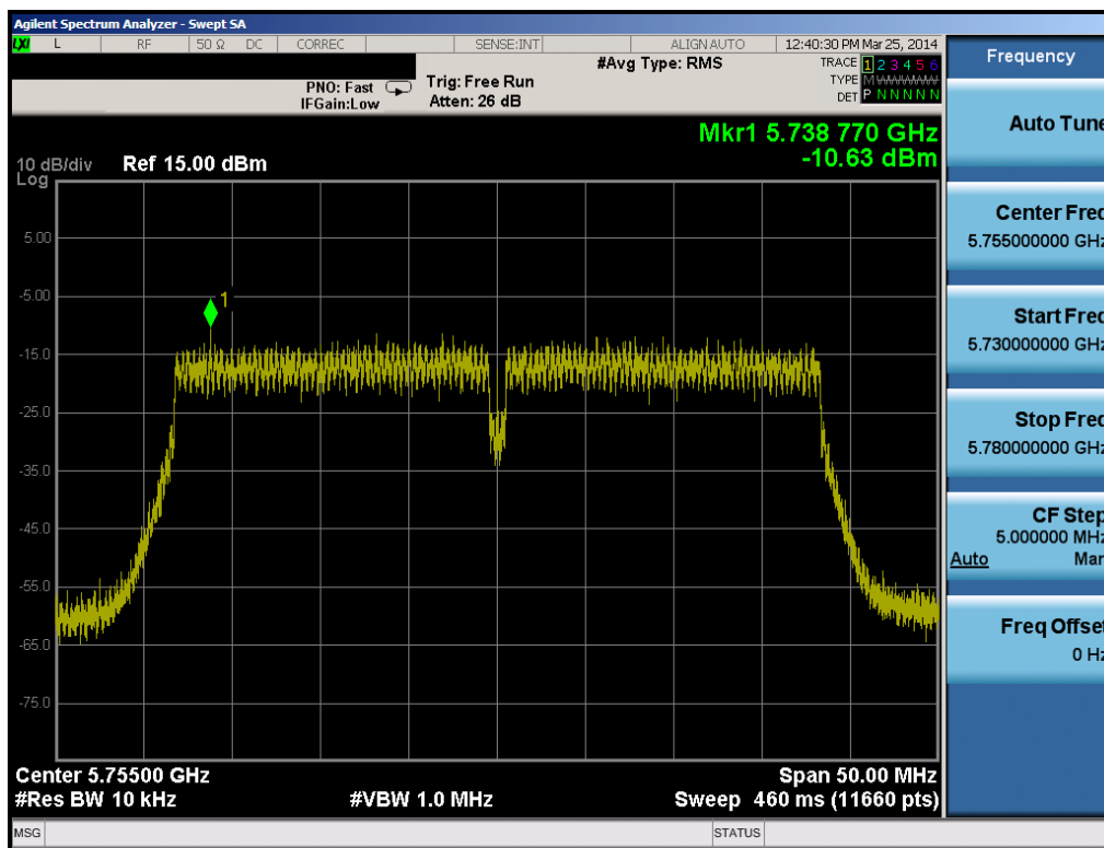
Plot 6-34. Power Spectral Density Plot (40MHz BW 802.11n (5.8GHz) – Ch. 151)
