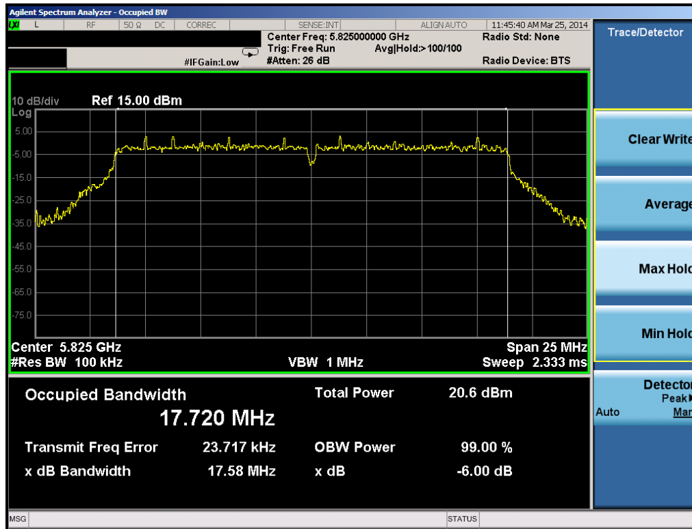
Plot 6-15. 6dB Bandwidth Plot (20MHz BW 802.11n (5.8GHz) – Ch. 165)
