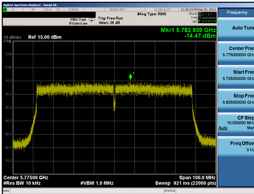
Plot 6-36. Power Spectral Density Plot (80MHz BW 802.11ac (5.8GHz) – Ch. 155)
