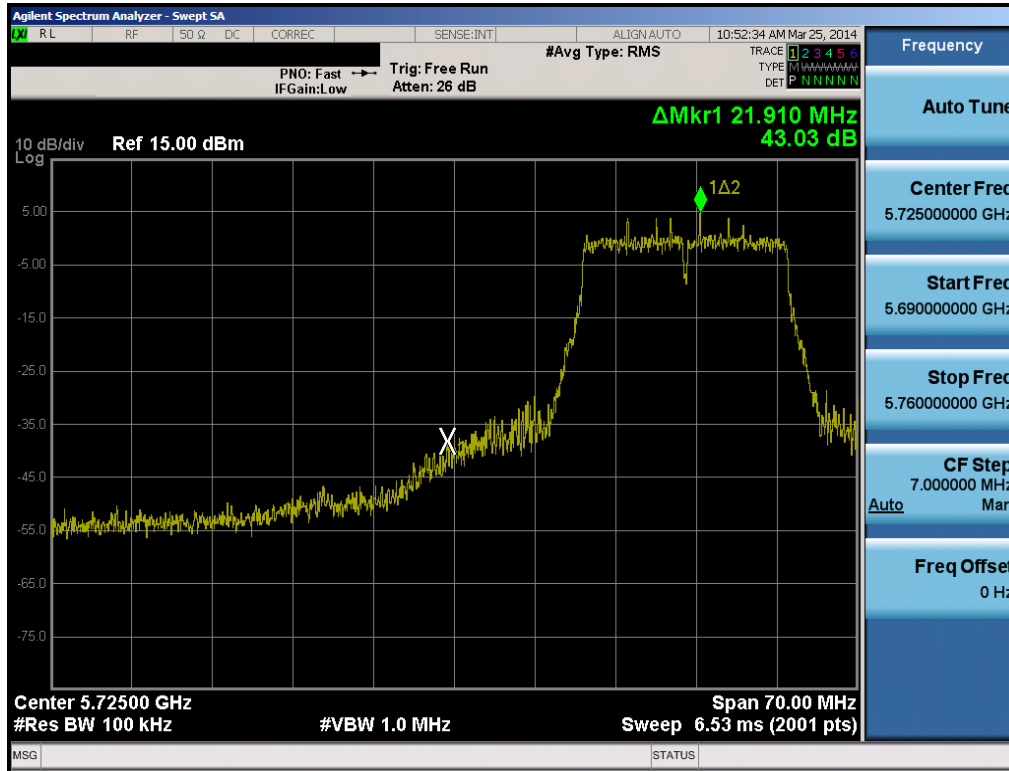
Plot 6-45. Band Edge Plot (20MHz BW 802.11n (5.8GHz) – Ch. 149)
