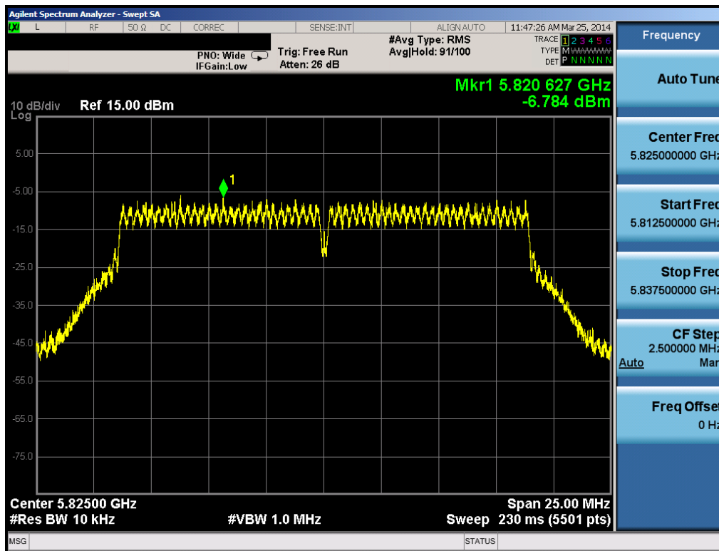
Plot 6-33. Power Spectral Density Plot (20MHz BW 802.11n (5.8GHz) – Ch. 165)
