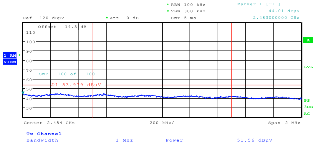
Plot 6-65. Radiated Restricted Upper Band Edge Measurement (Average)
