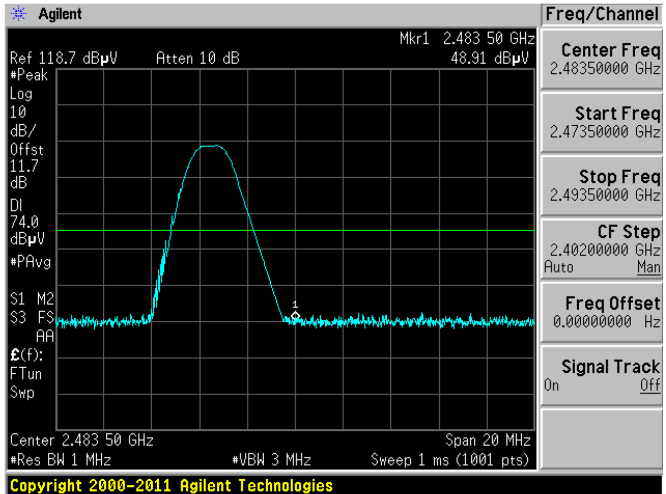
Plot 6-19. Radiated Restricted Upper Band Edge Measurement (Peak)
