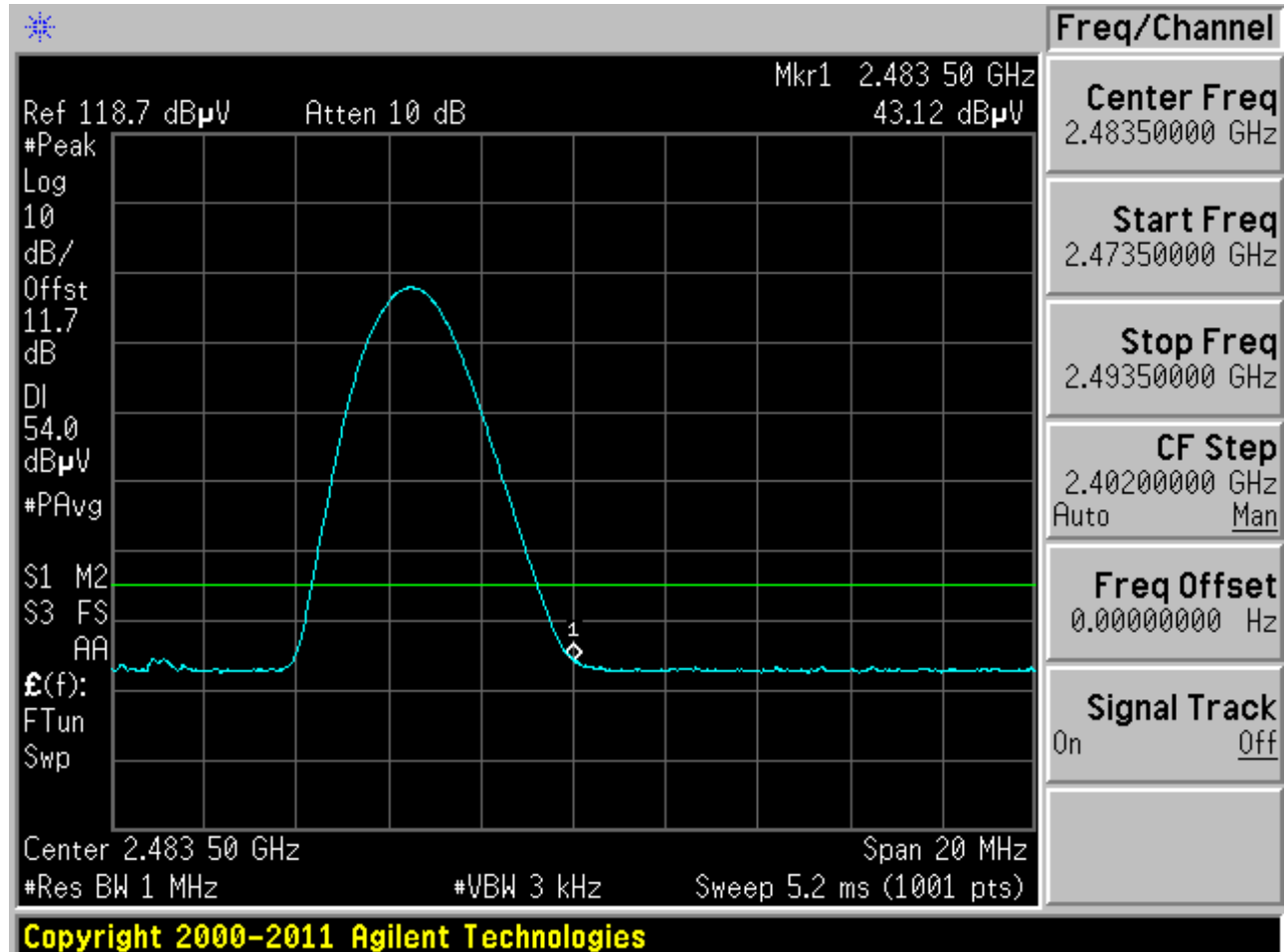
Plot 6-18. Radiated Restricted Upper Band Edge Measurement (Average)
