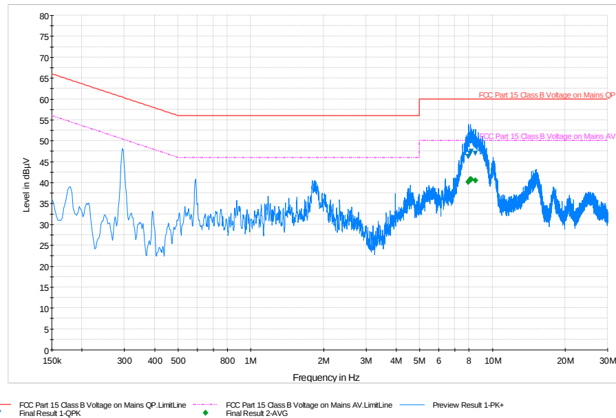
Plot 6-45. Line-Conducted Test Plot (N)
