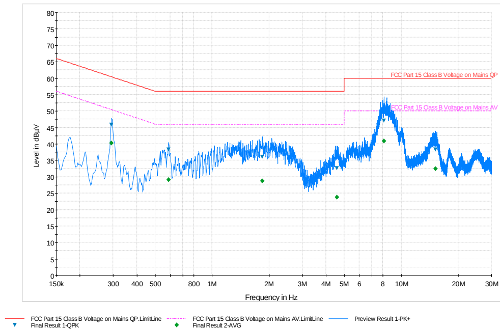
Plot 6-44. Line-Conducted Test Plot (L1)
