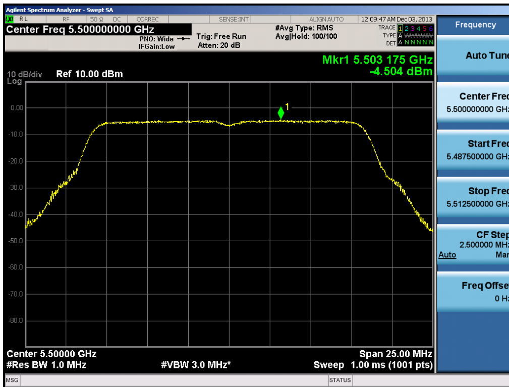
Plot 6-83. Peak Power Spectral Density Plot (802.11a (UNII Band 2C) – Ch. 100)
