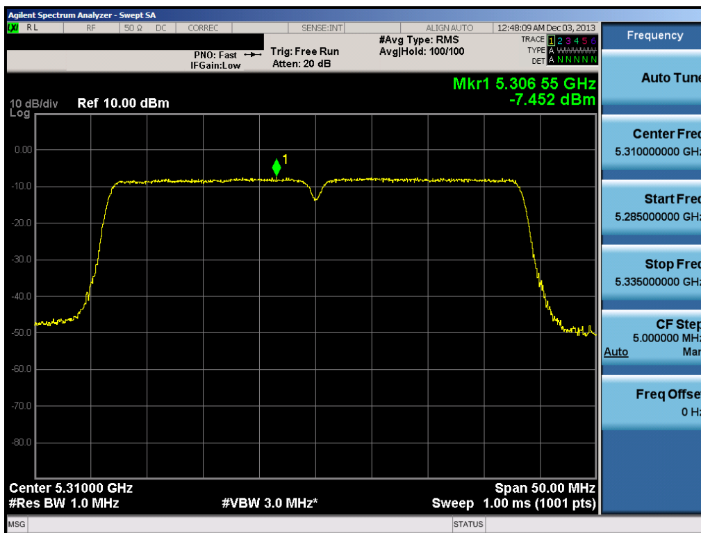
Plot 6-81. Peak Power Spectral Density Plot (40MHz BW 802.11n (UNII Band 2A) – Ch. 62)
