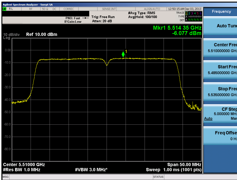
Plot 6-89. Peak Power Spectral Density Plot (40MHz BW 802.11n (UNII Band 2C) – Ch. 102)
