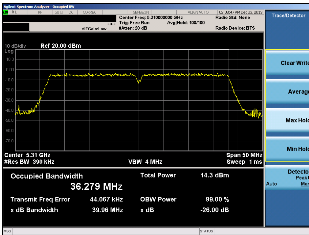
Plot 6-50. 26dB Bandwidth Plot (40MHz BW 802.11n (UNII Band 2A) – Ch. 62)
