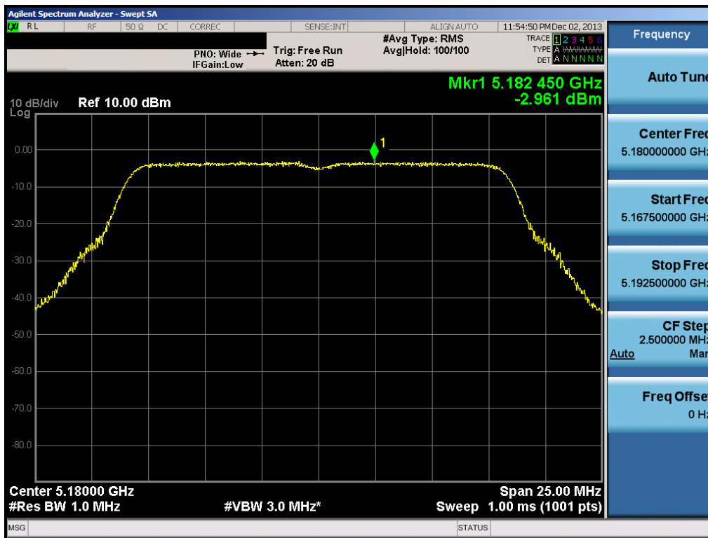
Plot 6-65. Peak Power Spectral Density Plot (802.11a (UNII Band 1) – Ch. 36)
