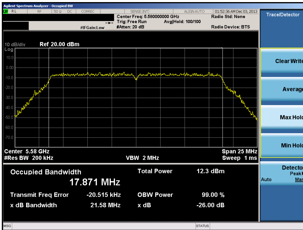
Plot 6-56. 26dB Bandwidth Plot (20MHz BW 802.11n (UNII Band 2C) – Ch. 116)
