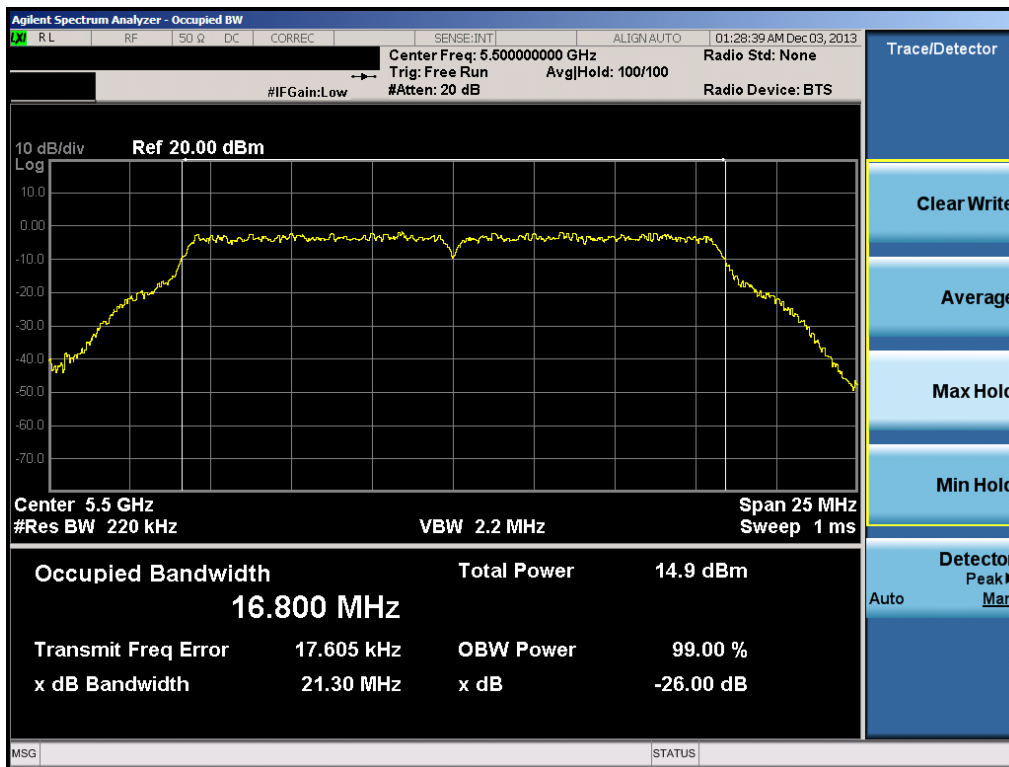
Plot 6-52. 26dB Bandwidth Plot (802.11a (UNII Band 2C) – Ch. 100)
