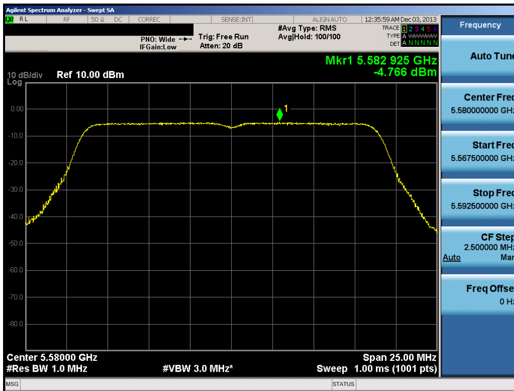
Plot 6-87. Peak Power Spectral Density Plot (20MHz BW 802.11n (UNII Band 2C) – Ch. 116)
