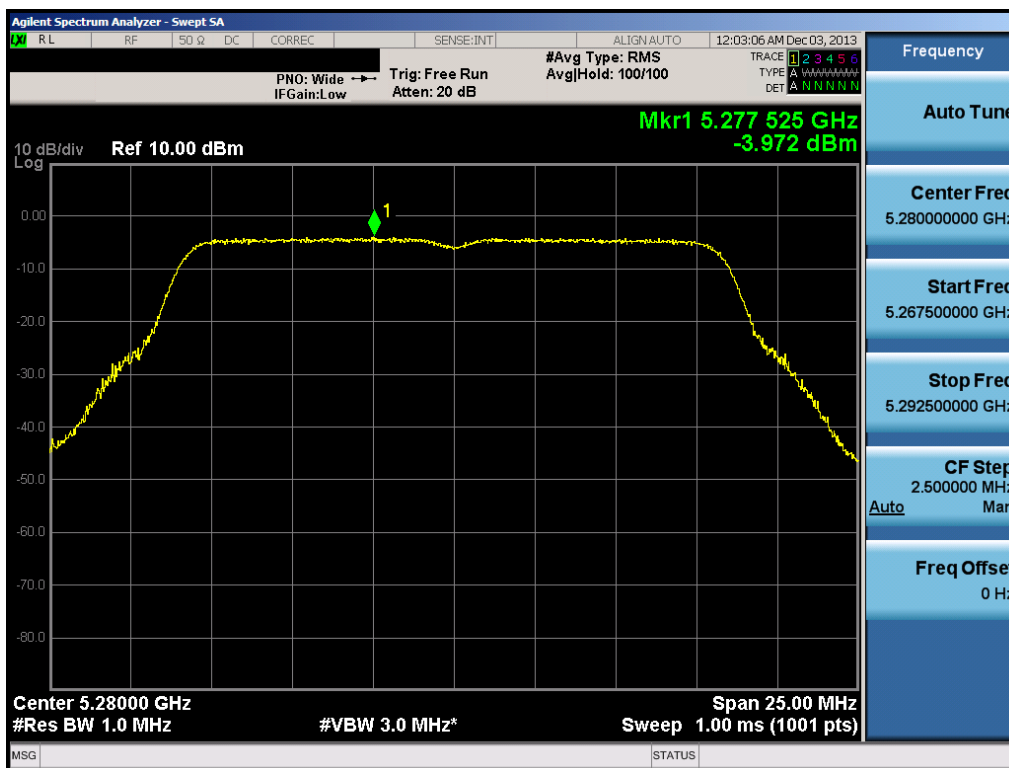
Plot 6-75. Peak Power Spectral Density Plot (802.11a (UNII Band 2A) – Ch. 56)
