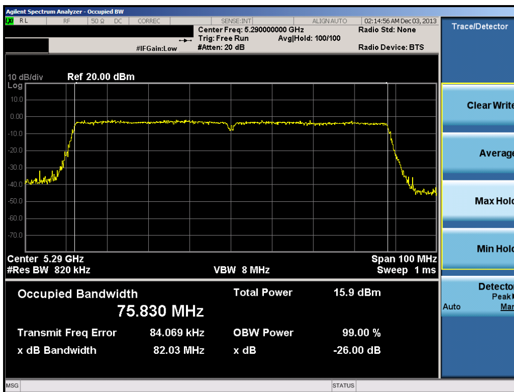
Plot 6-51. 26dB Bandwidth Plot (80MHz BW 802.11ac (UNII Band 2A) – Ch. 58)
