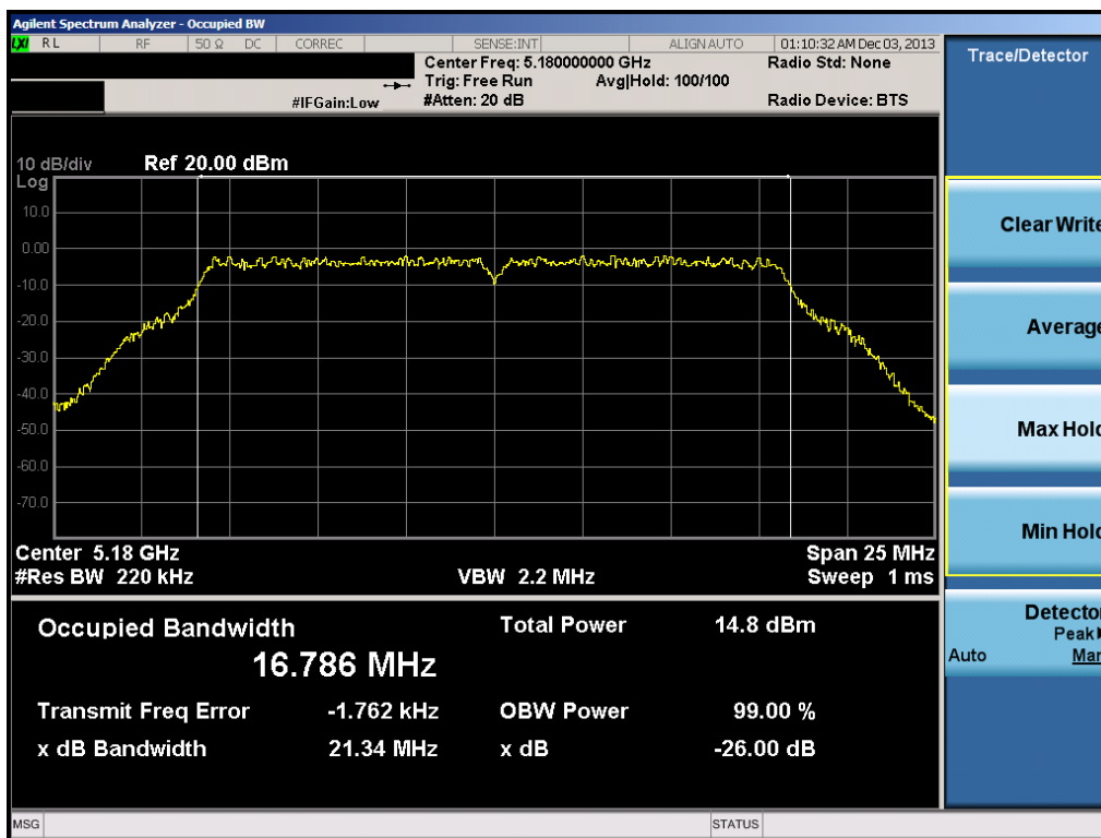
Plot 6-33. 26dB Bandwidth Plot (802.11a (UNII Band 1) – Ch. 36)
