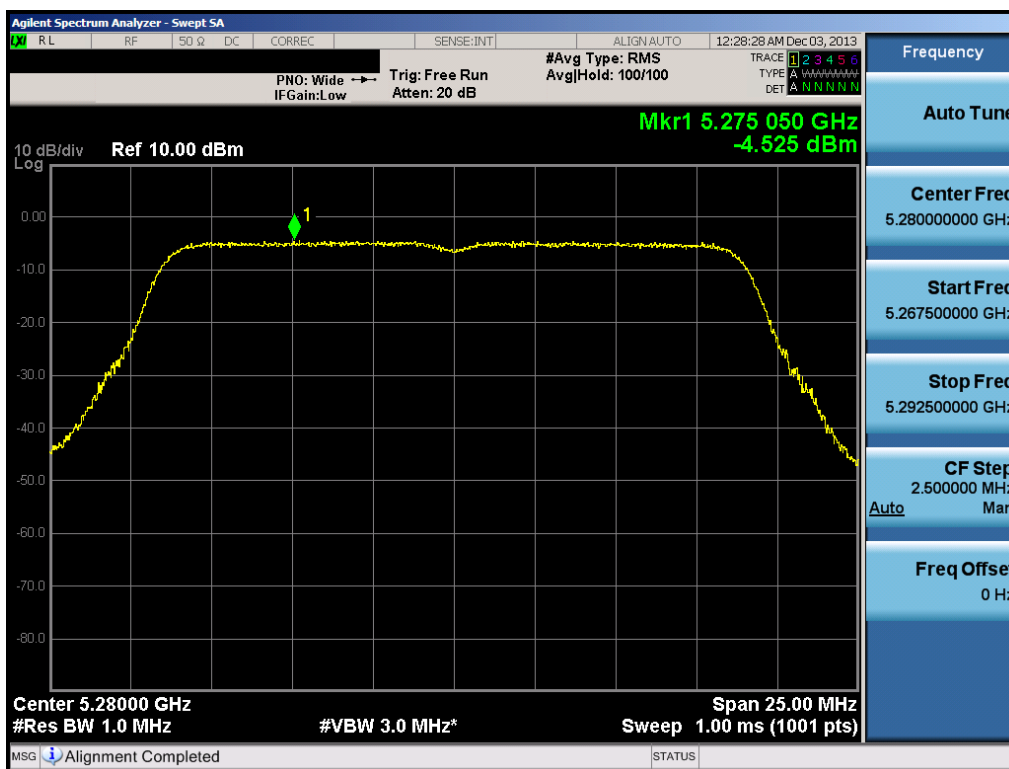
Plot 6-78. Peak Power Spectral Density Plot (20MHz BW 802.11n (UNII Band 2A) – Ch. 56)
