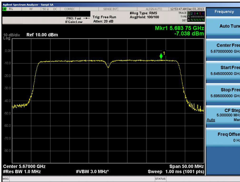
Plot 6-91. Peak Power Spectral Density Plot (40MHz BW 802.11n (UNII Band 2C) – Ch. 134)
