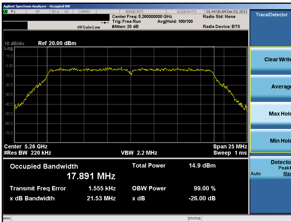
Plot 6-46. 26dB Bandwidth Plot (20MHz BW 802.11n (UNII Band 2A) – Ch. 52)
