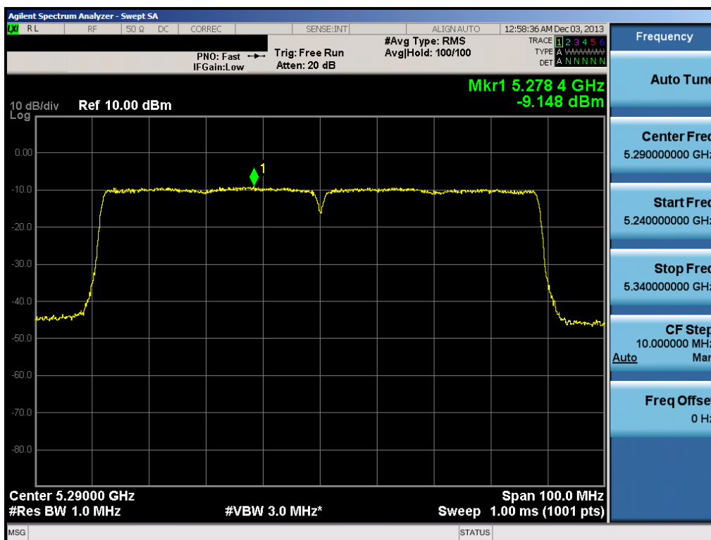
Plot 6-82. Peak Power Spectral Density Plot (80MHz BW 802.11ac (UNII Band 2A) – Ch. 58)
