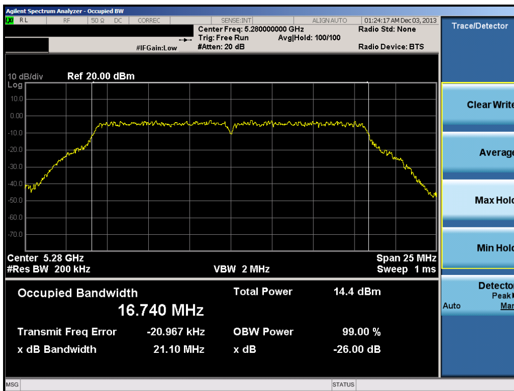
Plot 6-44. 26dB Bandwidth Plot (802.11a (UNII Band 2A) – Ch. 56)
