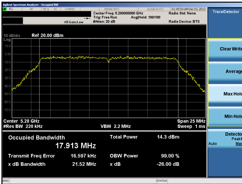
Plot 6-47. 26dB Bandwidth Plot (20MHz BW 802.11n (UNII Band 2A) – Ch. 56)
