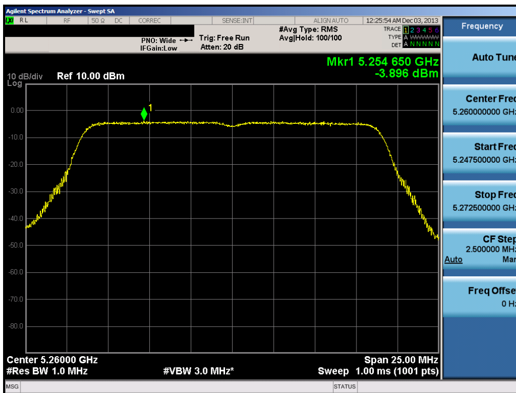
Plot 6-77. Peak Power Spectral Density Plot (20MHz BW 802.11n (UNII Band 2A) – Ch. 52)
