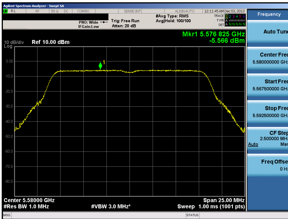
Plot 6-84. Peak Power Spectral Density Plot (802.11a (UNII Band 2C) – Ch. 116)
