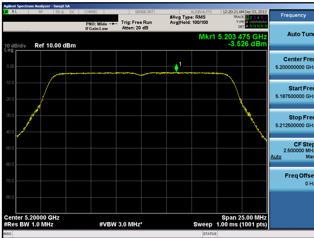
Plot 6-69. Peak Power Spectral Density Plot (20MHz BW 802.11n (UNII Band 1) – Ch. 40)
