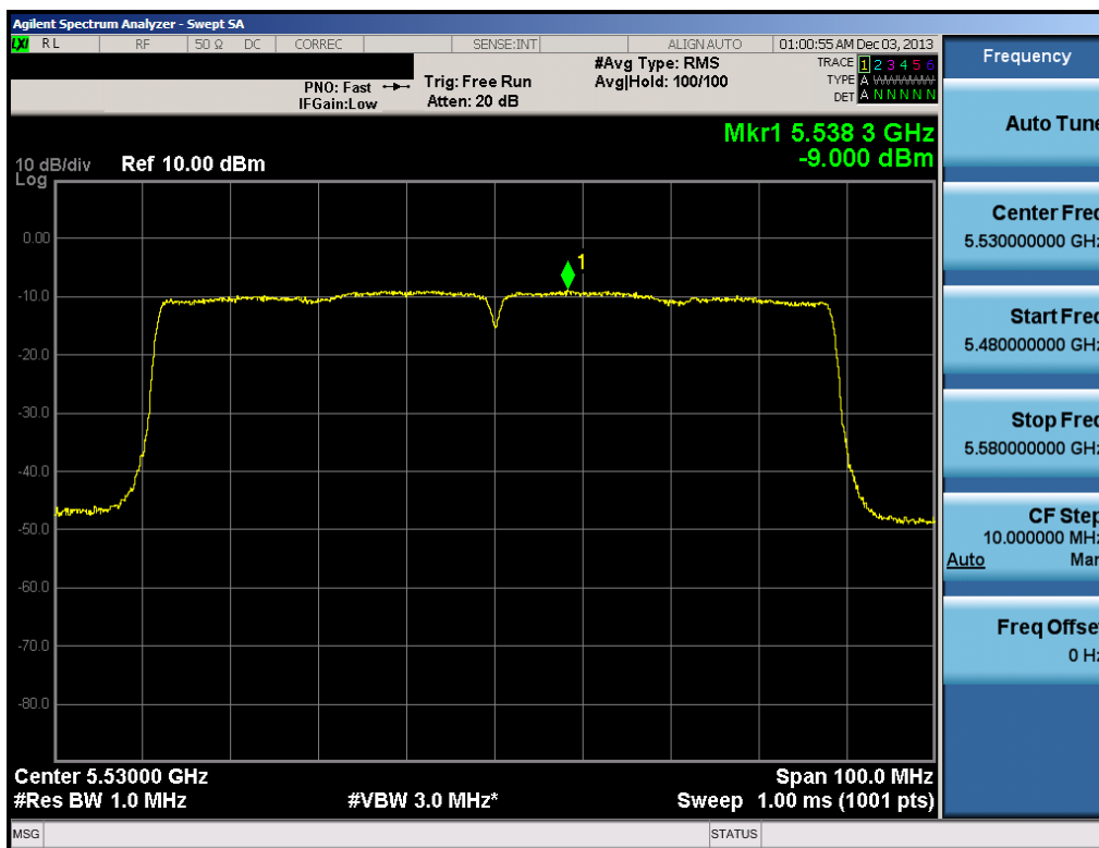
Plot 6-92. Peak Power Spectral Density Plot (80MHz BW 802.11ac (UNII Band 2C) – Ch. 106)
