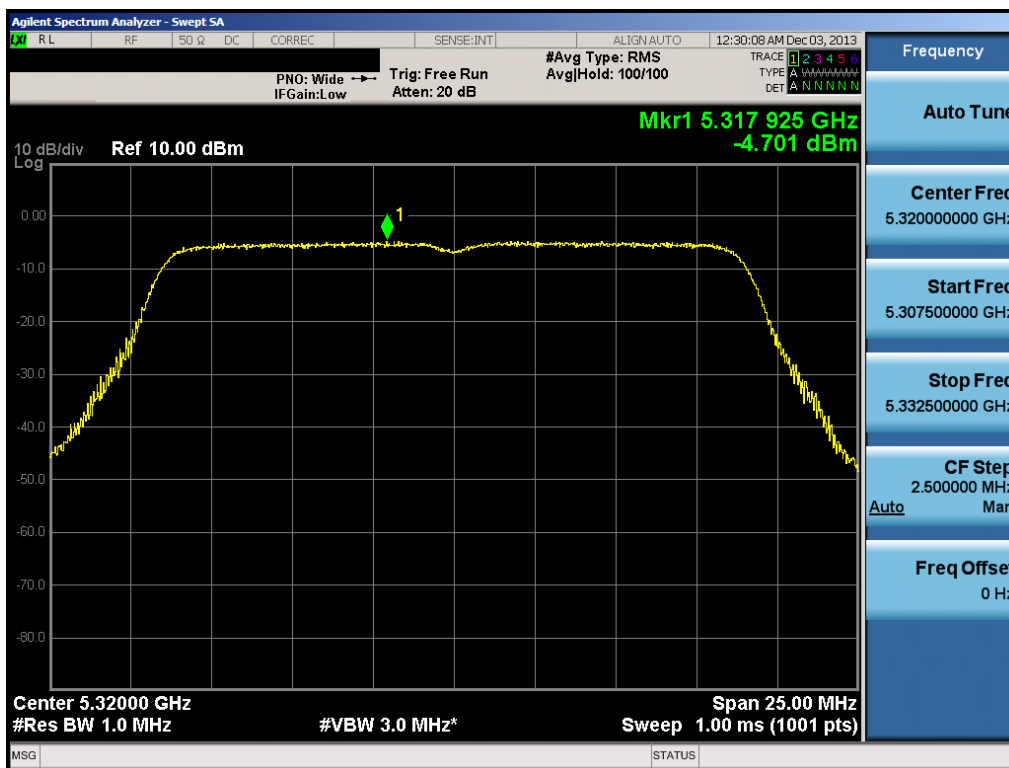
Plot 6-79. Peak Power Spectral Density Plot (20MHz BW 802.11n (UNII Band 2A) – Ch. 64)
