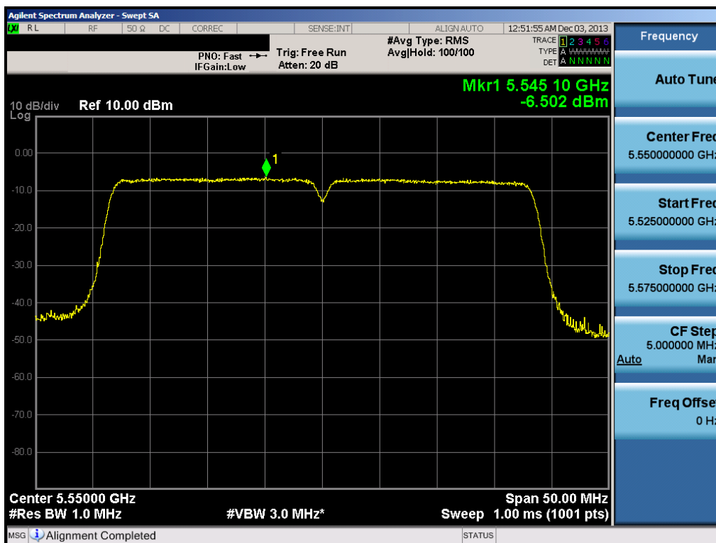
Plot 6-90. Peak Power Spectral Density Plot (40MHz BW 802.11n (UNII Band 2C) – Ch. 110)
