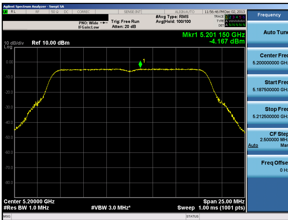
Plot 6-66. Peak Power Spectral Density Plot (802.11a (UNII Band 1) – Ch. 40)
