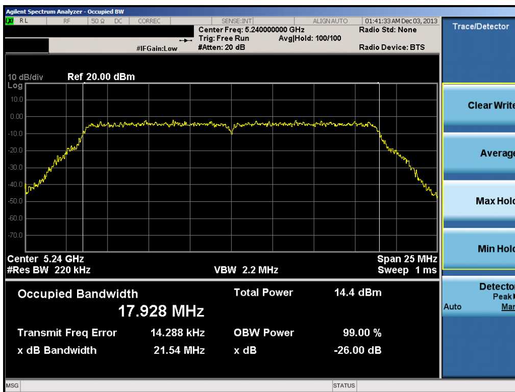
Plot 6-39. 26dB Bandwidth Plot (20MHz BW 802.11n (UNII Band 1) – Ch. 48)
