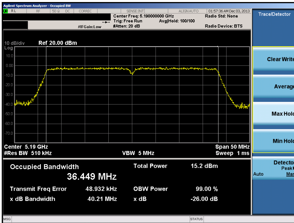
Plot 6-40. 26dB Bandwidth Plot (40MHz BW 802.11n (UNII Band 1) – Ch. 38)
