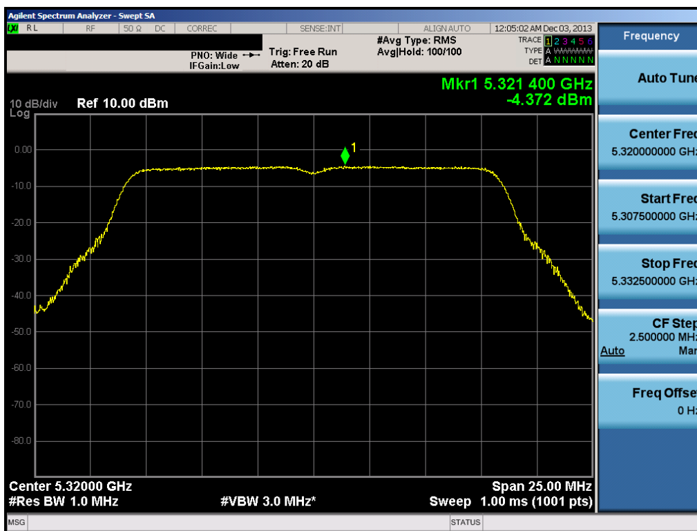
Plot 6-76. Peak Power Spectral Density Plot (802.11a (UNII Band 2A) – Ch. 64)
