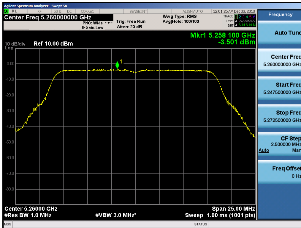
Plot 6-74. Peak Power Spectral Density Plot (802.11a (UNII Band 2A) – Ch. 52)
