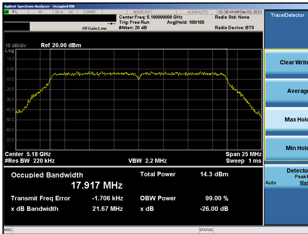
Plot 6-37. 26dB Bandwidth Plot (20MHz BW 802.11n (UNII Band 1) – Ch. 36)
