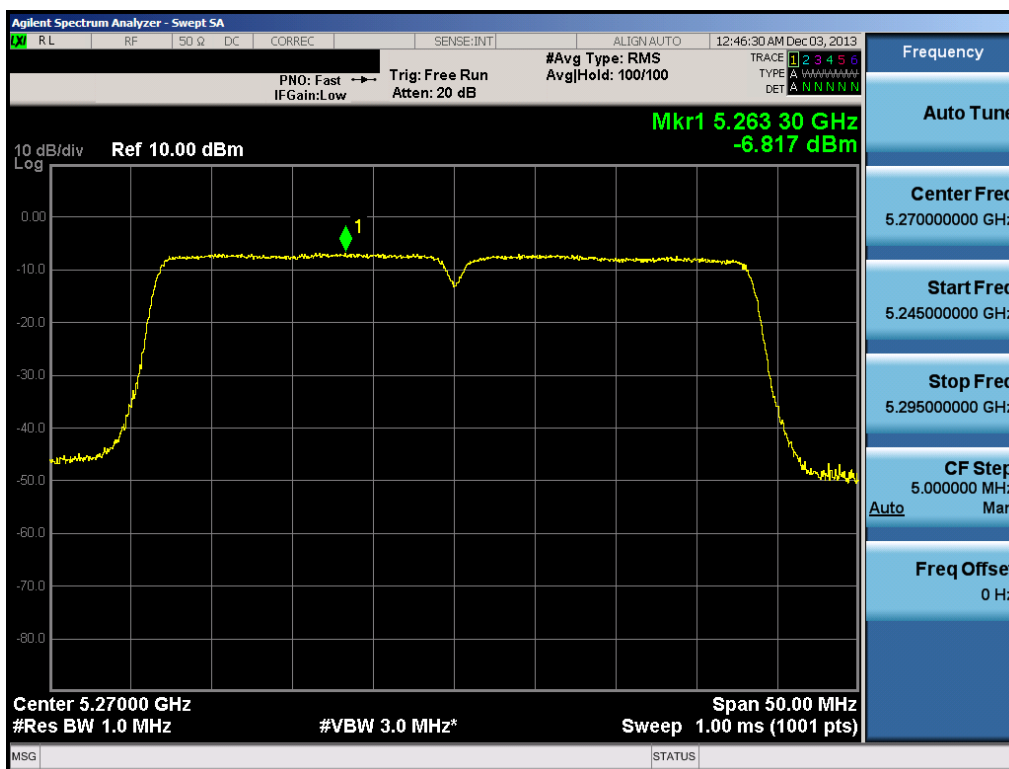
Plot 6-80. Peak Power Spectral Density Plot (40MHz BW 802.11n (UNII Band 2A) – Ch. 54)
