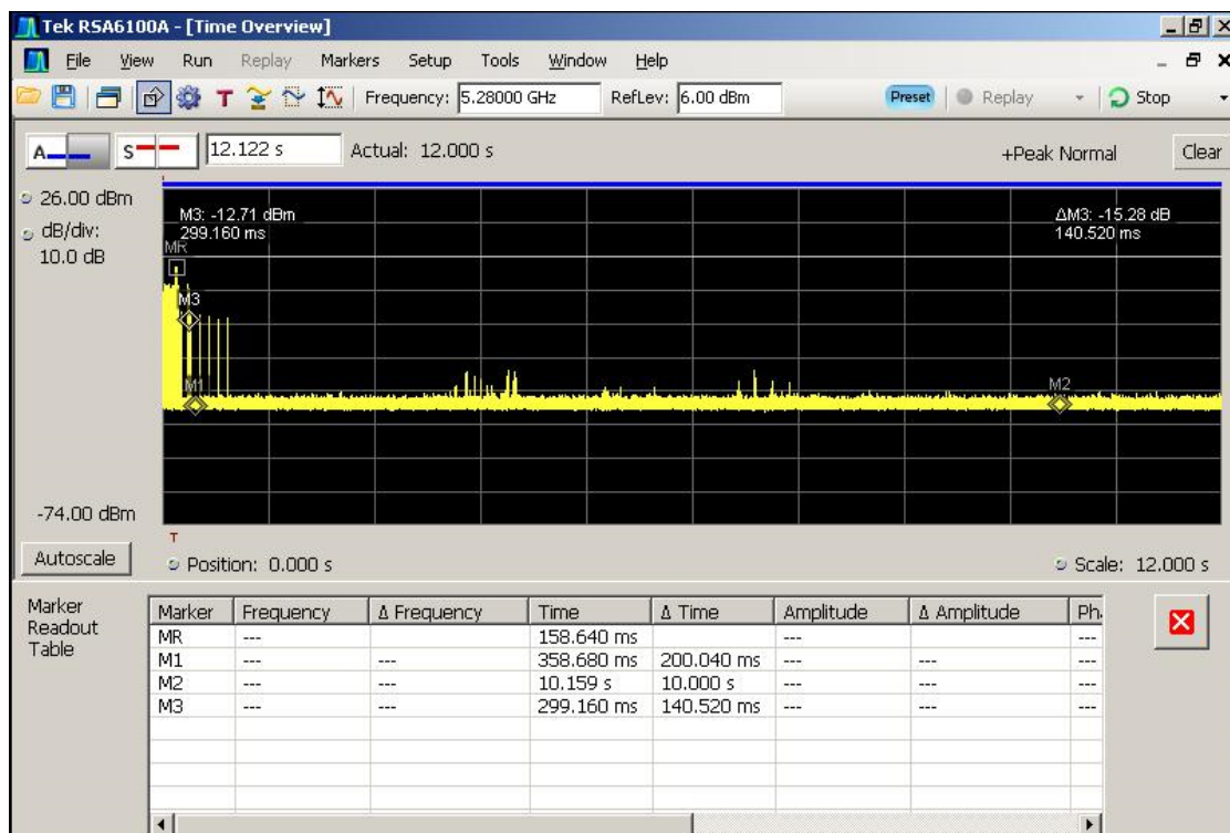
Figure 5-4. Channel Move Time (< 10sec)
