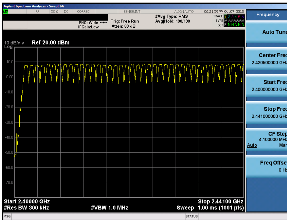
Plot 6-34. Low End Spectrum Channel Hopping Plot (Bluetooth)
