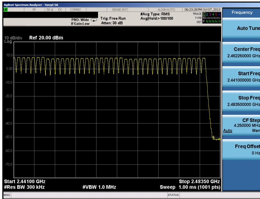
Plot 6-35. High End Spectrum Channel Hopping Plot (Bluetooth)
