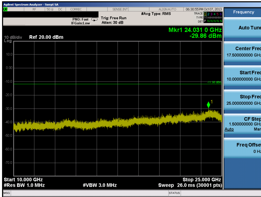
Plot 6-41. Conducted Spurious Plot (Bluetooth, 1Mbps – Ch. 78)
