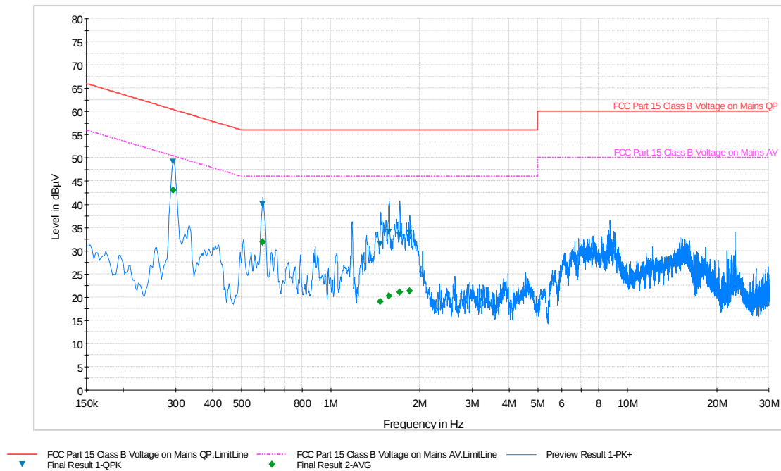
Plot 6-45. Line-Conducted Test Plot (N)
