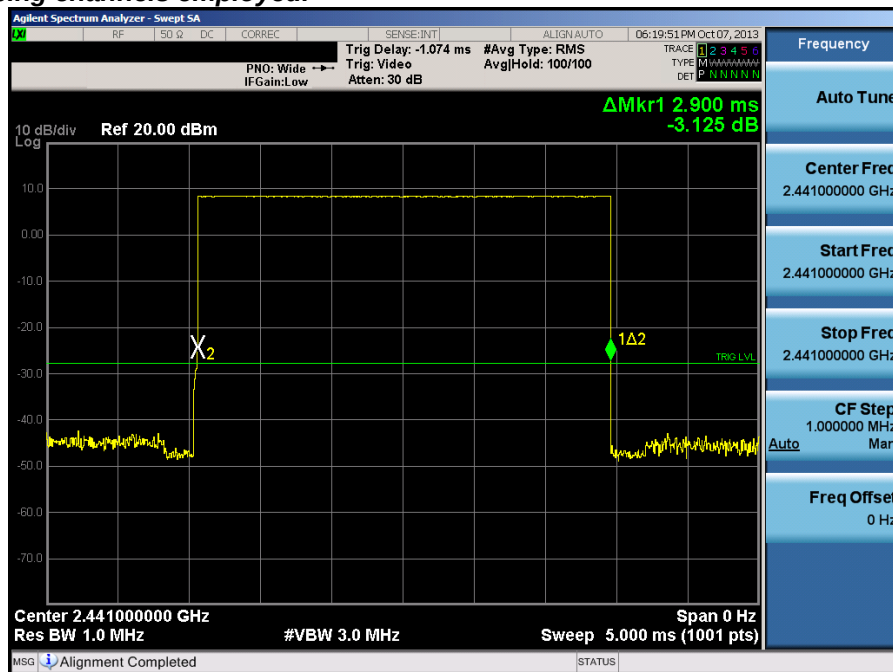
Plot 6-33. Time of Occupancy Plot (Bluetooth)
