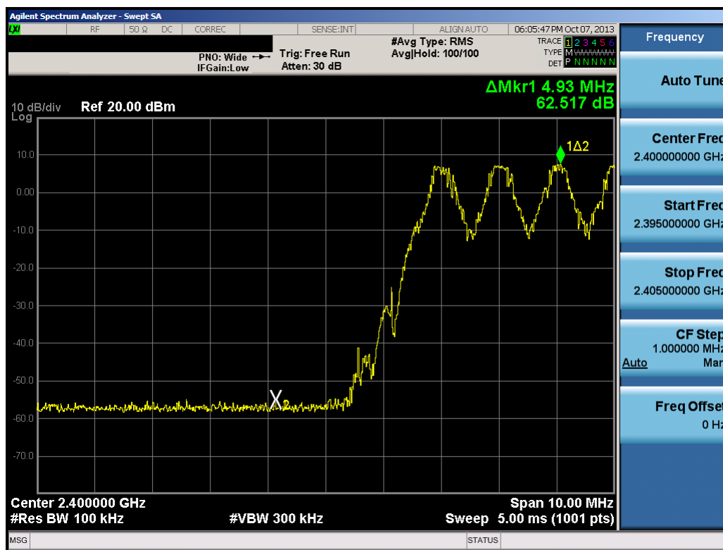
Plot 6-30. Band Edge Plot (Bluetooth with Hopping Enabled, 1Mbps)
