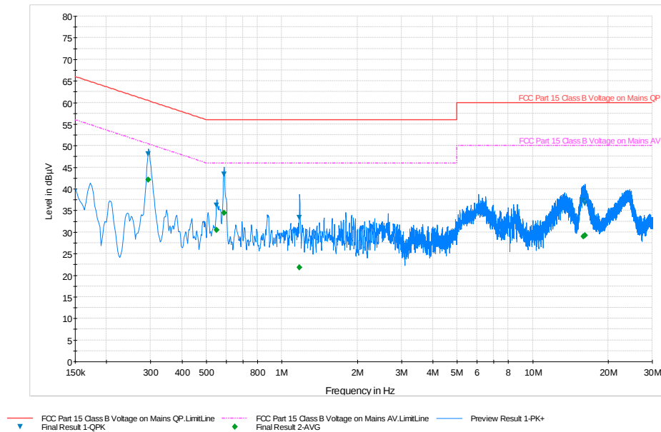
Plot 6-6. Line-Conducted Test Plot (N)
