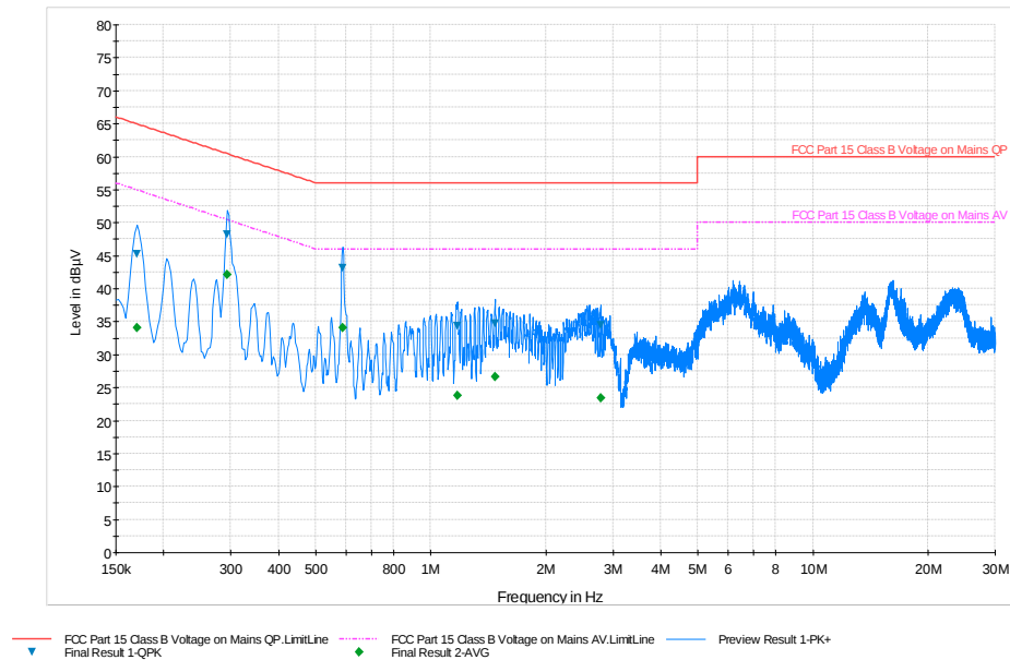
Plot 6-5. Line-Conducted Test Plot (L1)
