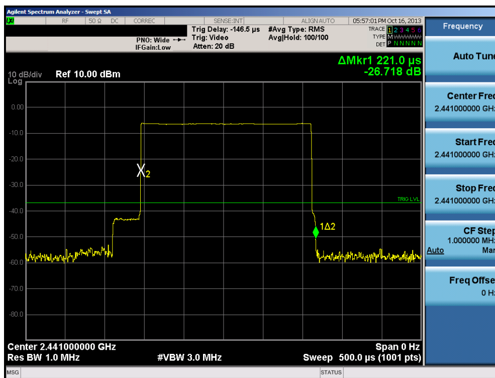
Plot 6-2. Pulse Width Measurement
