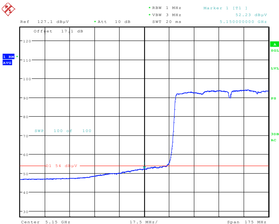
Plot 6-76. Radiated Restricted Lower Band Edge Plot (Average – UNII Band 1)
