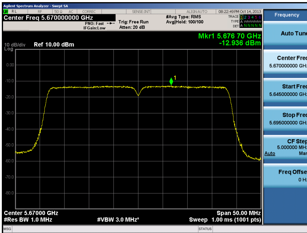
Plot 6-56. Peak Power Spectral Density Plot (40MHz BW 802.11n (UNII Band 3) – Ch. 134)
