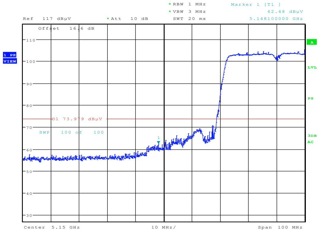
Plot 6-70. Radiated Restricted Lower Band Edge Plot (Peak – UNII Band 1)
