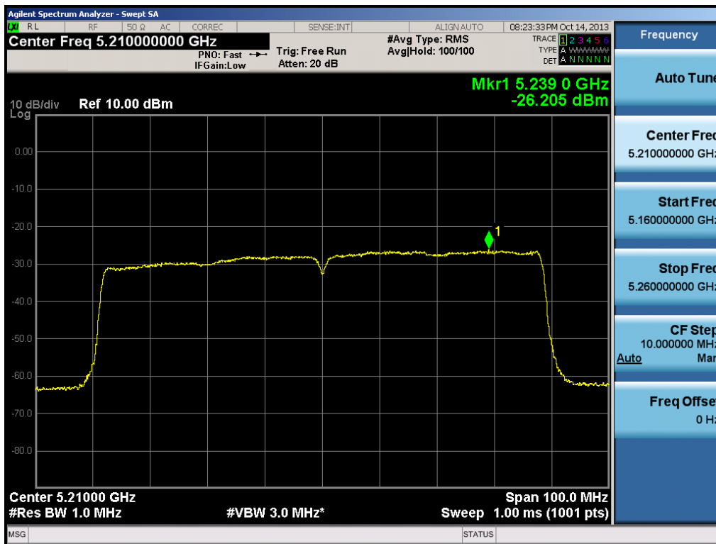
Plot 6-38. Peak Power Spectral Density Plot (80MHz BW 802.11ac (UNII Band 1) – Ch. 42)
