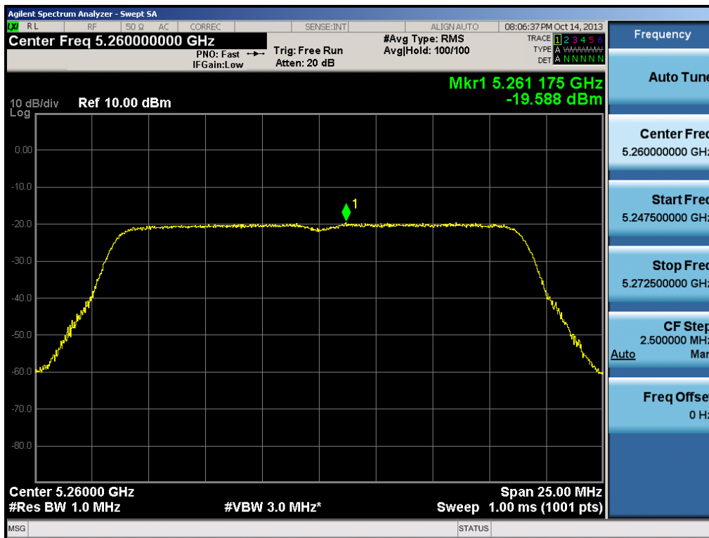
Plot 6-42. Peak Power Spectral Density Plot (20MHz BW 802.11n (UNII Band 2) – Ch. 52)
