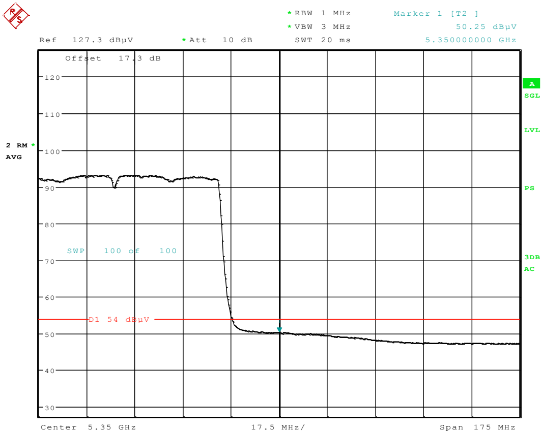
Plot 6-78. Radiated Restricted Upper Band Edge Plot (Average – UNII Band 2)
