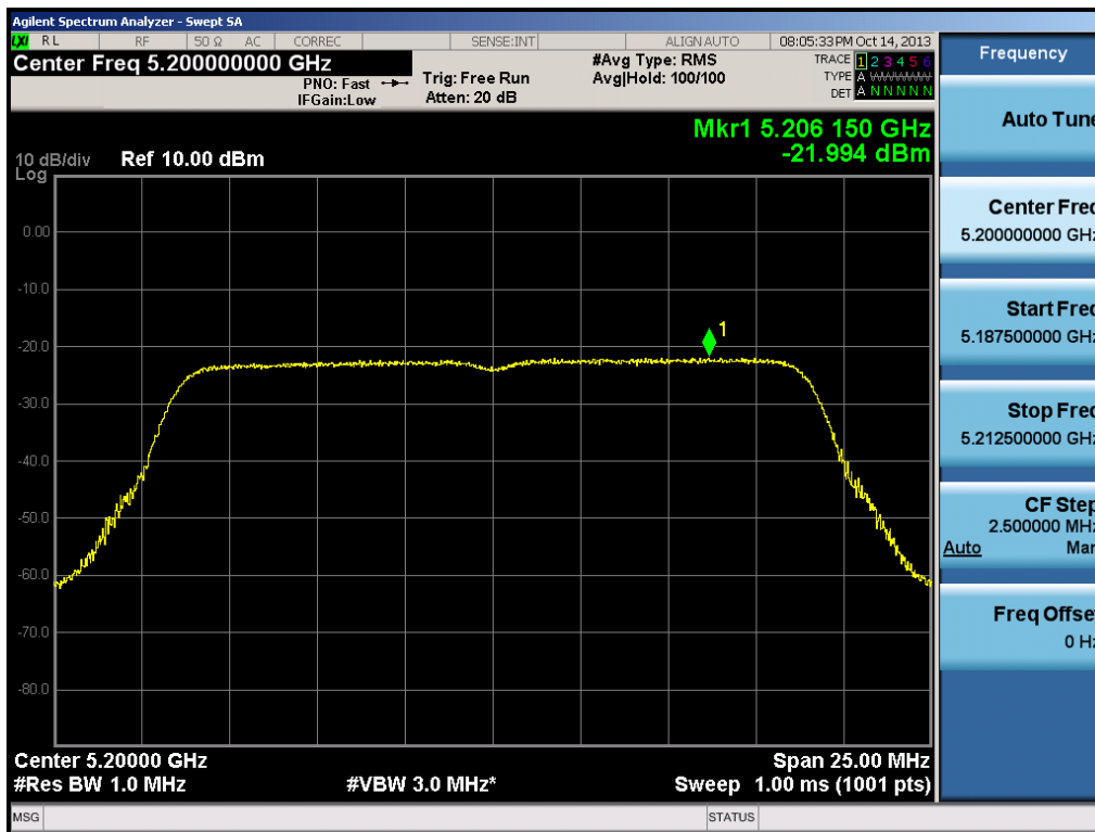
Plot 6-34. Peak Power Spectral Density Plot (20MHz BW 802.11n (UNII Band 1) – Ch. 40)
