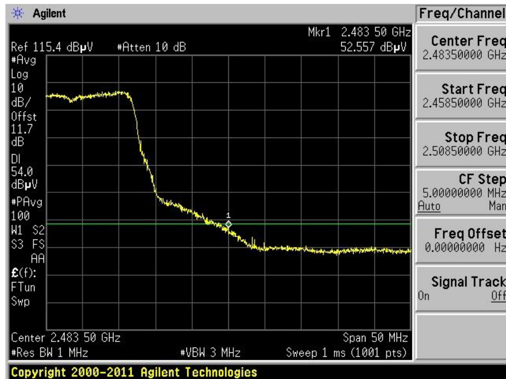
Plot 6-65. Radiated Restricted Upper Band Edge Measurement (Average)
