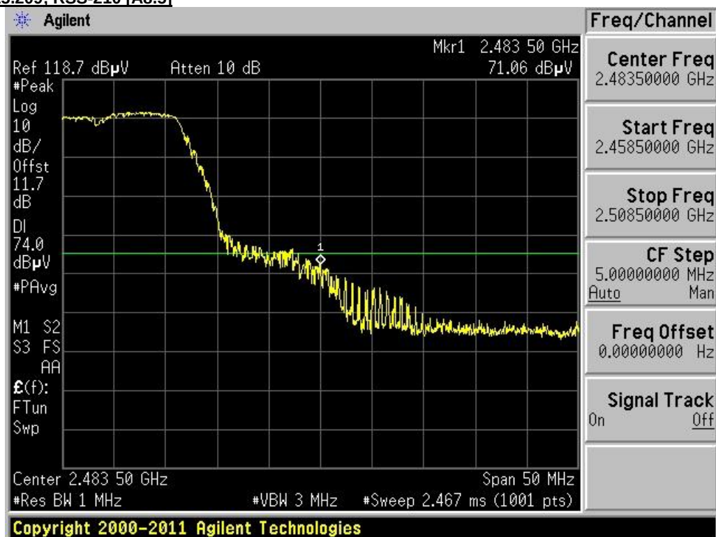
Plot 6-66. Radiated Restricted Upper Band Edge Measurement (Peak)
