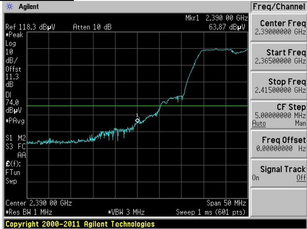
Plot 6-64. Radiated Restricted Lower Band Edge Measurement (Peak)
