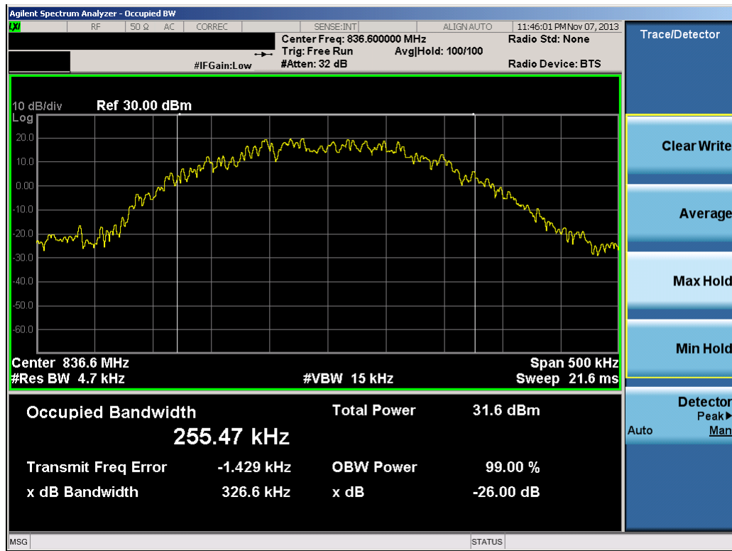
Plot 6-2. Occupied Bandwidth Plot (EDGE850 Mode – Ch. 190)
