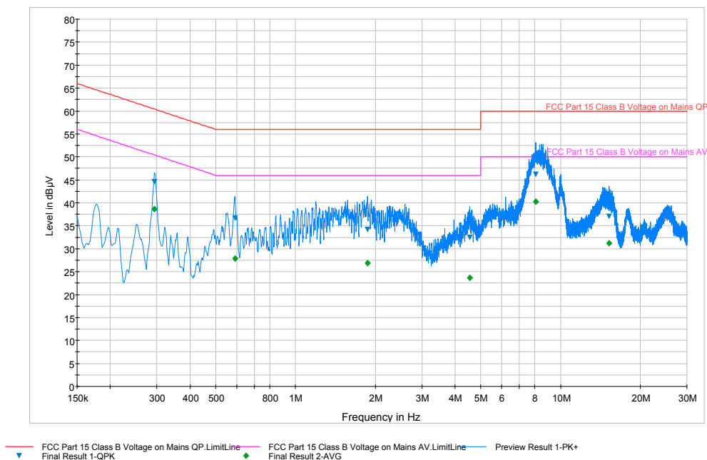
Plot 6-6. Line Conducted Plot with ANT+ (L1)
