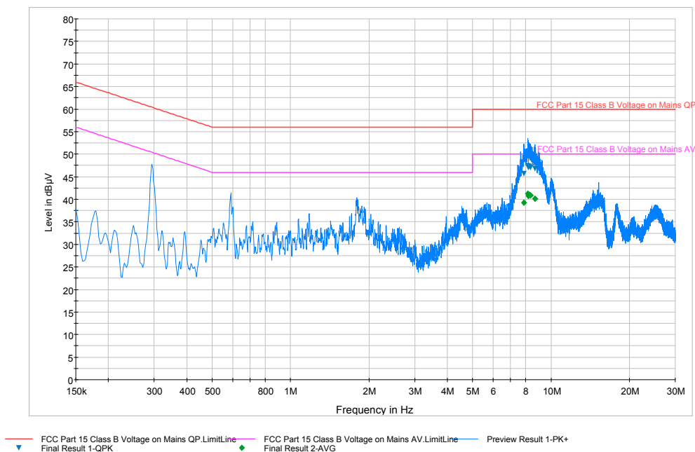
Plot 6-7. Line Conducted Plot with ANT+ (N)
