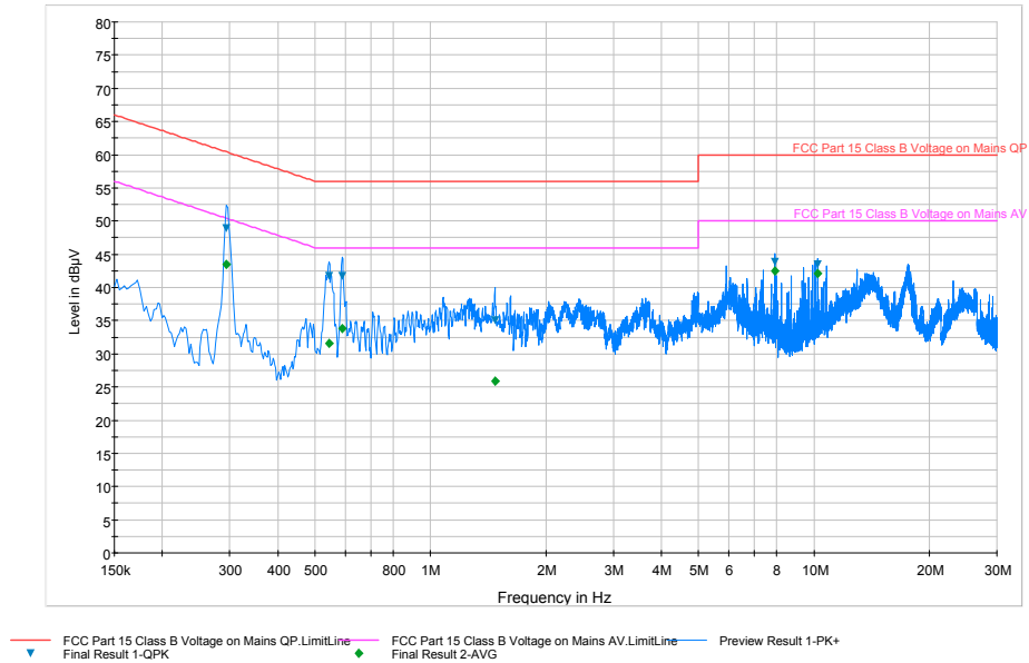
Plot 6-139. Line Conducted Plot with 802.11a (L1)
