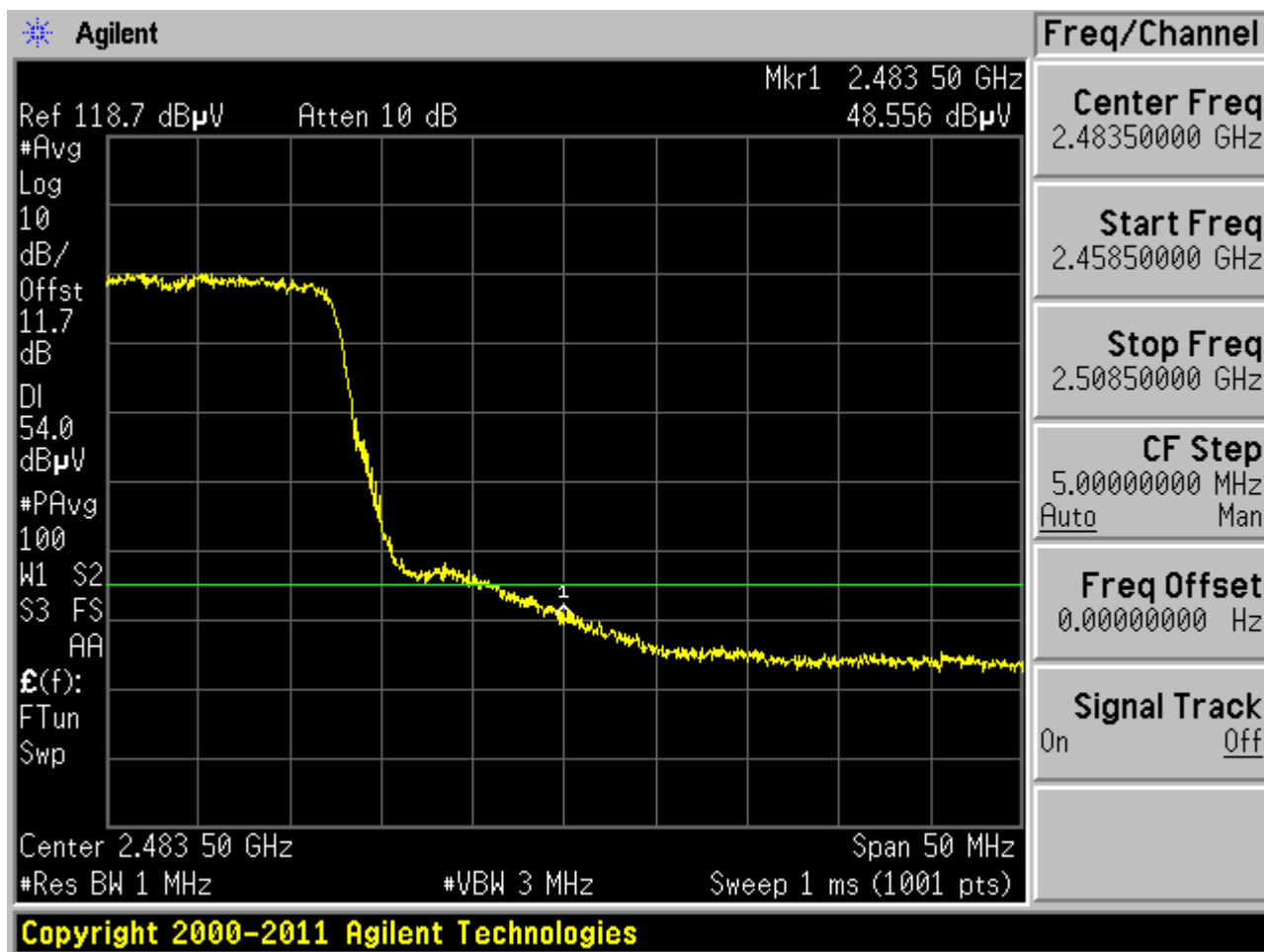
Plot 6-135. Radiated Restricted Upper Band Edge Measurement (Average)
