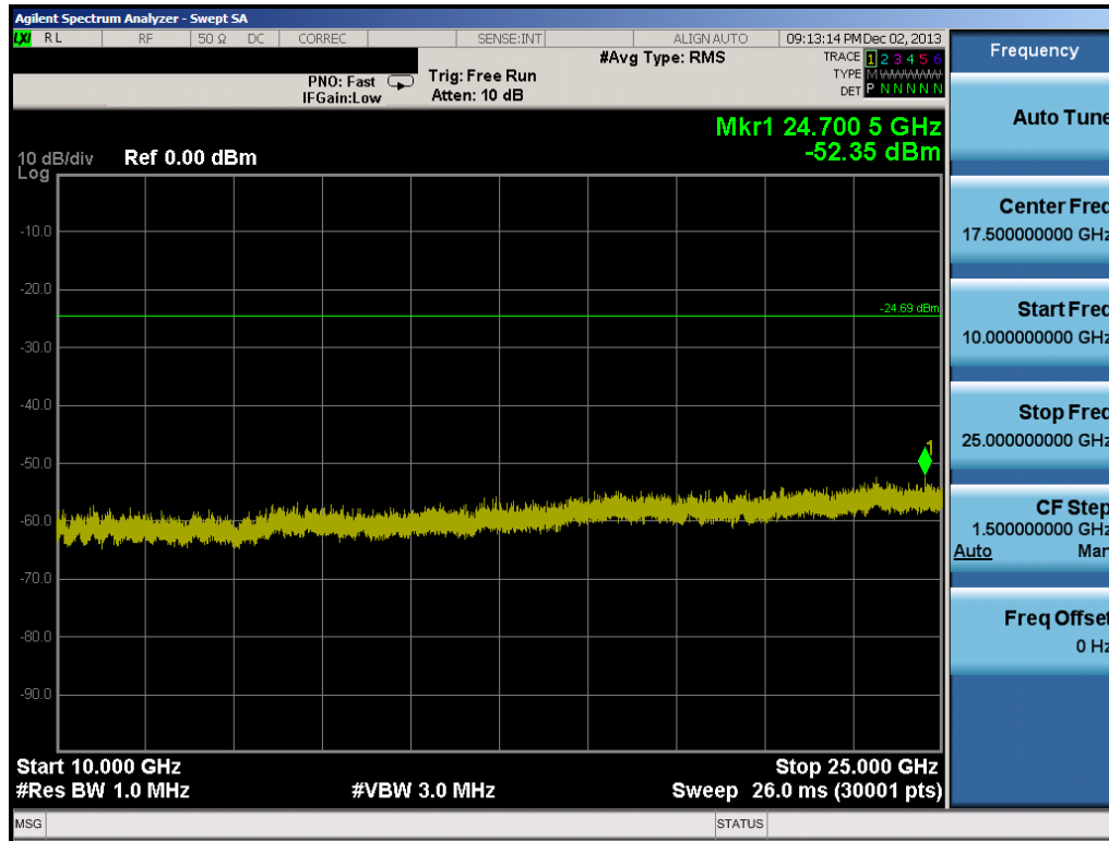
Plot 6-114. Conducted Spurious Plot (802.11b – Ch. 1)
