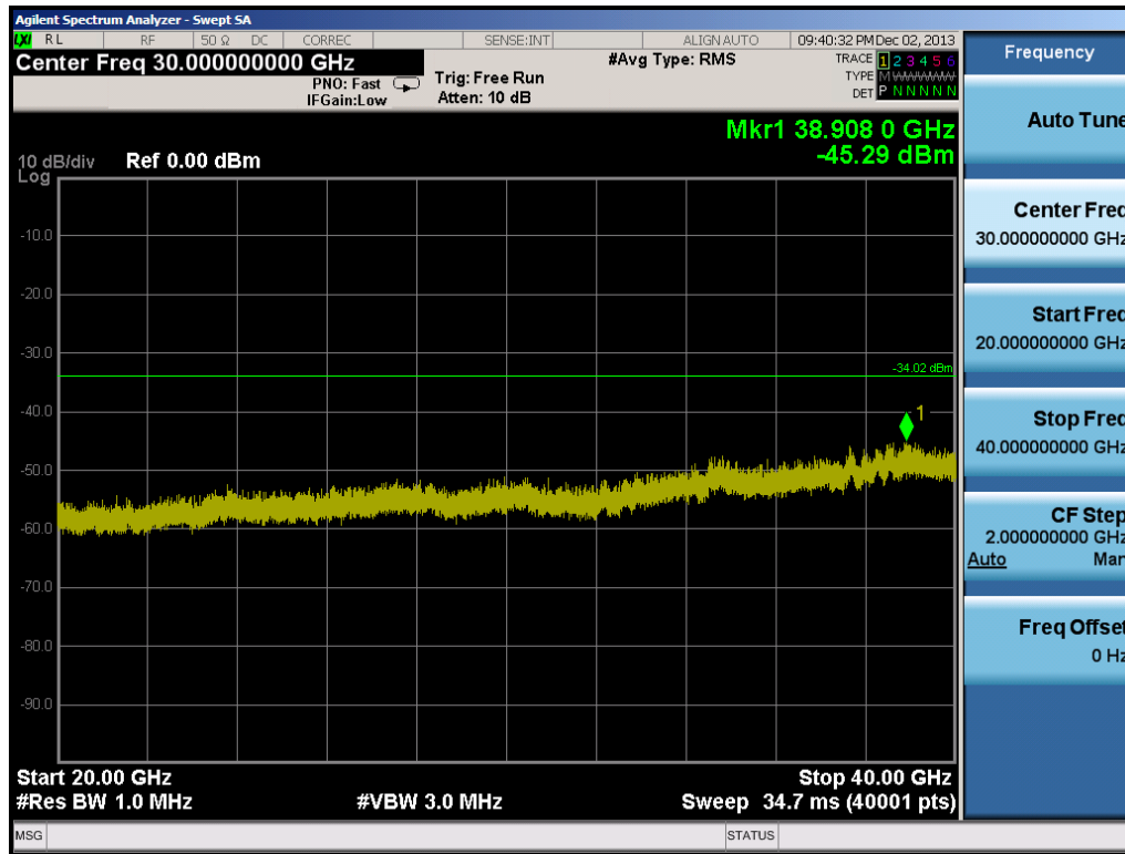
Plot 6-108. Conducted Spurious Plot (802.11a – Ch. 149)
