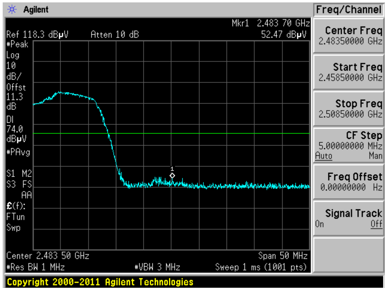
Plot 6-128. Radiated Restricted Upper Band Edge Measurement (Peak)
