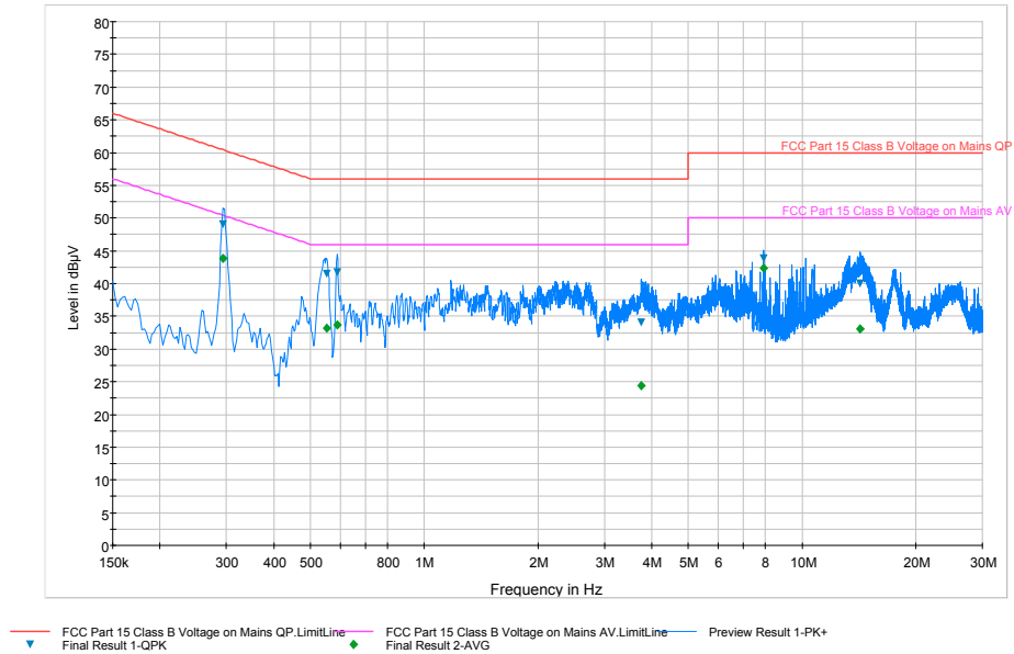
Plot 6-137. Line Conducted Plot with 802.11b (L1)
