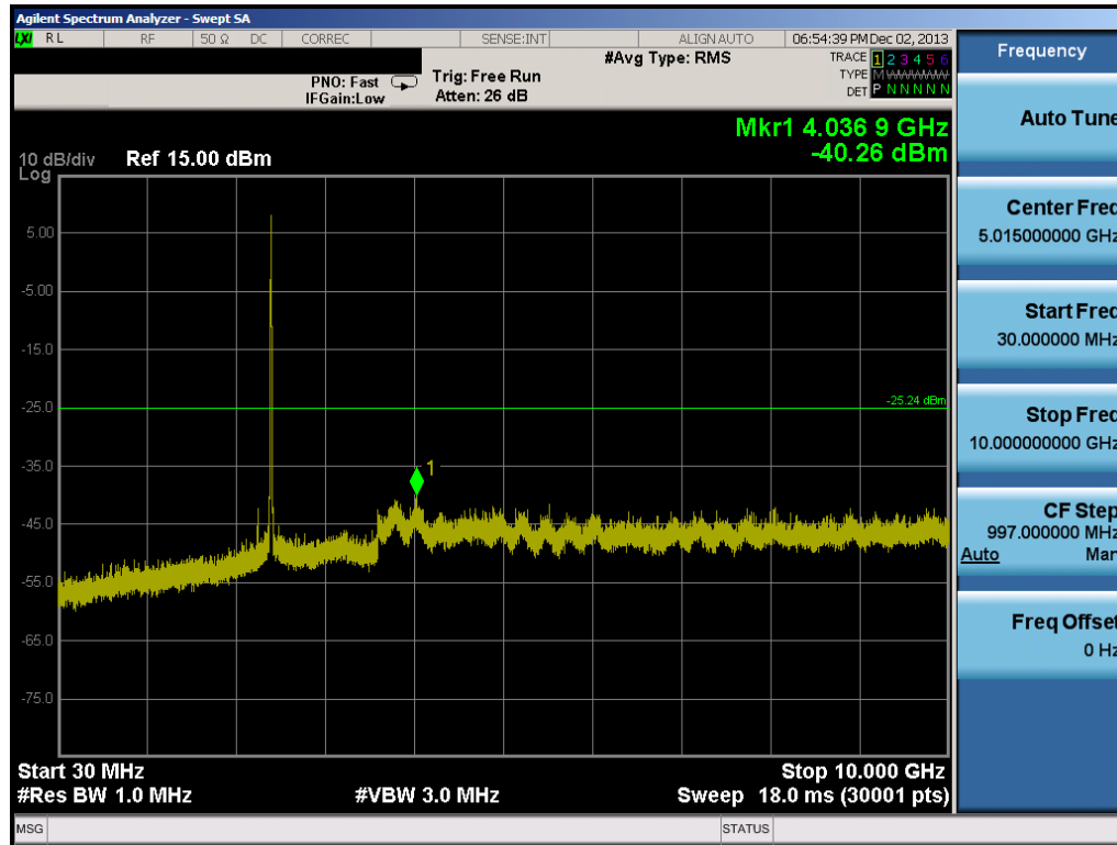
Plot 6-101. Conducted Spurious Plot (802.11b – Ch. 1)
