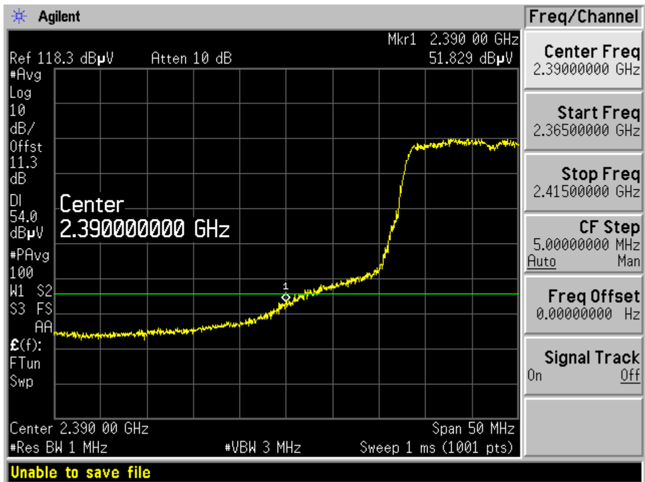
Plot 6-133. Radiated Restricted Lower Band Edge Measurement (Average)
