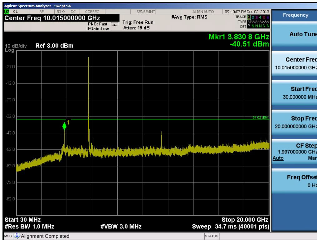
Plot 6-107. Conducted Spurious Plot (802.11a – Ch. 149)
