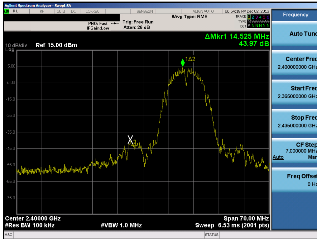
Plot 6-73. Band Edge Plot (802.11b – Ch. 1)
