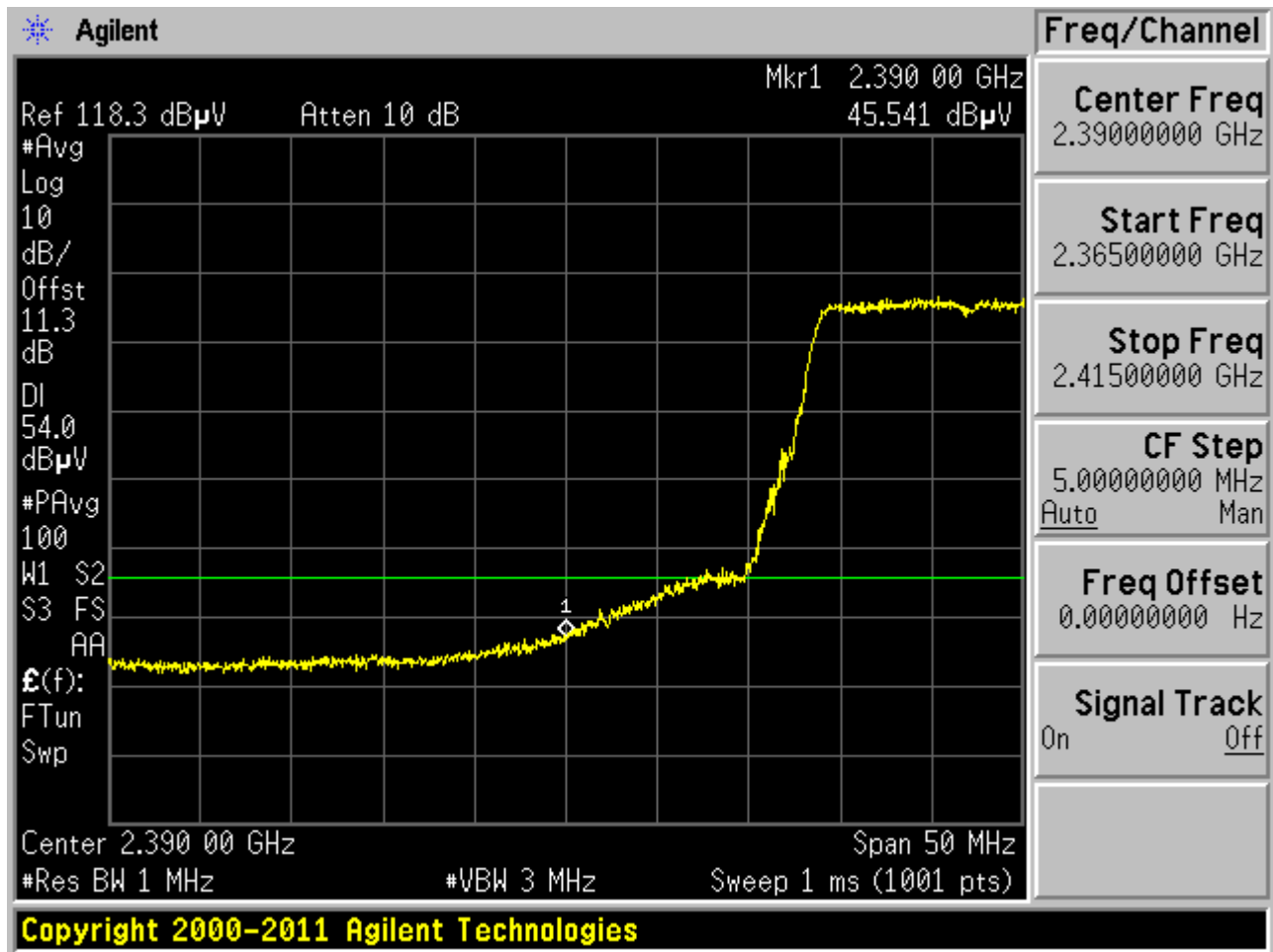
Plot 6-129. Radiated Restricted Lower Band Edge Measurement (Average)
