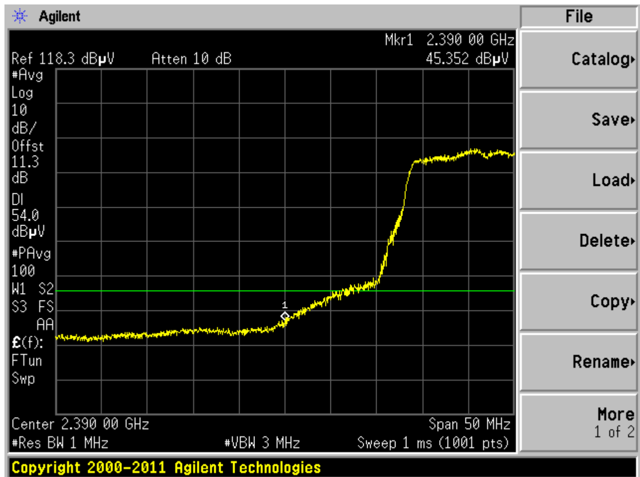
Plot 6-125. Radiated Restricted Lower Band Edge Measurement (Average)
