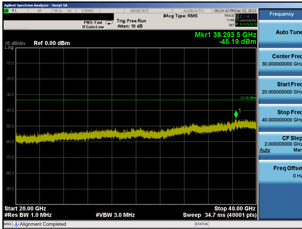
Plot 6-120. Conducted Spurious Plot (802.11a – Ch. 149)
