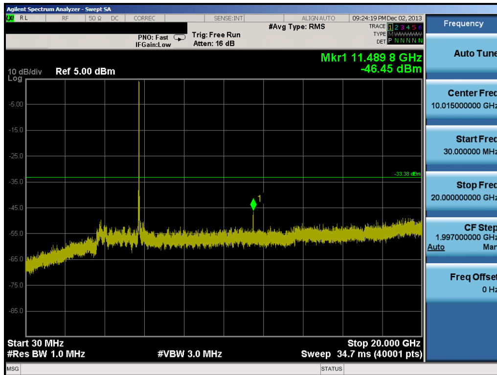
Plot 6-119. Conducted Spurious Plot (802.11a – Ch. 149)
