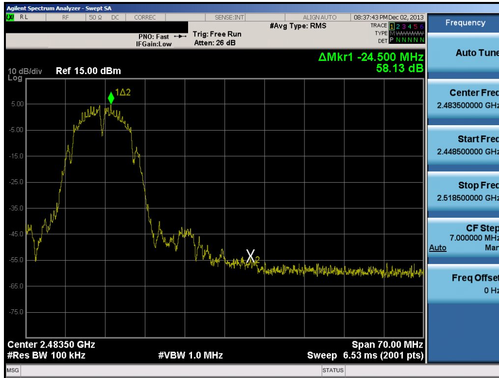
Plot 6-88. Band Edge Plot (802.11b - Ch. 11)
