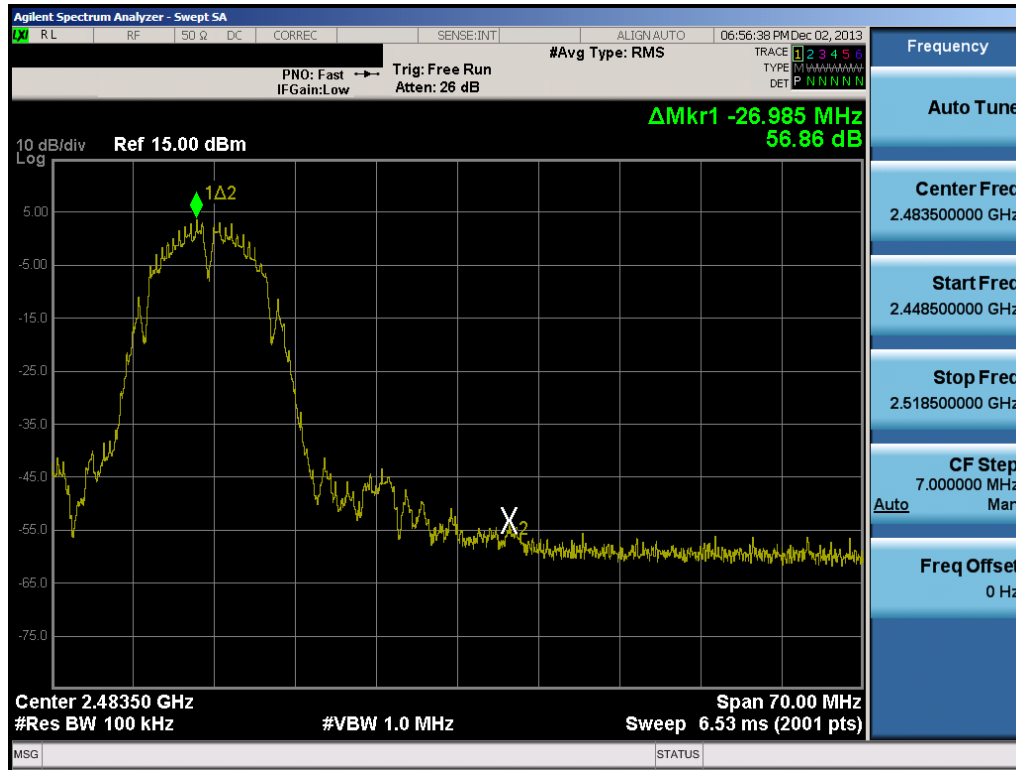
Plot 6-74. Band Edge Plot (802.11b – Ch. 11)
