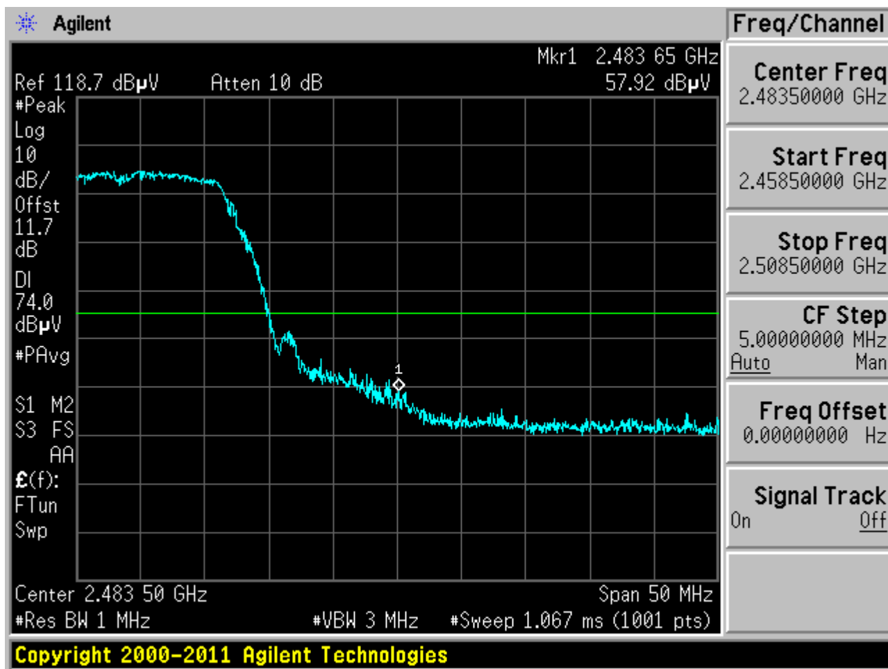
Plot 6-132. Radiated Restricted Upper Band Edge Measurement (Peak)
