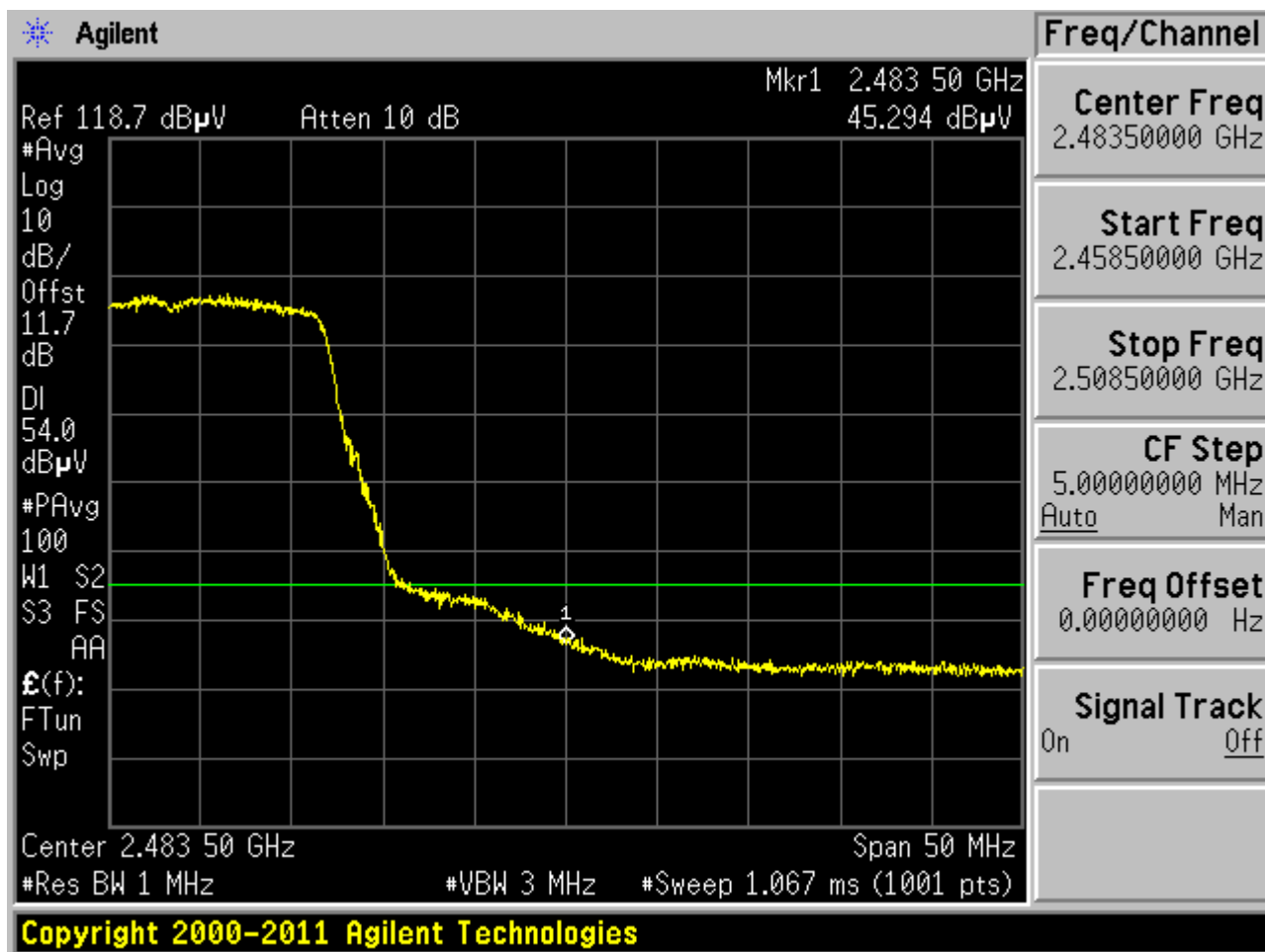
Plot 6-131. Radiated Restricted Upper Band Edge Measurement (Average)
