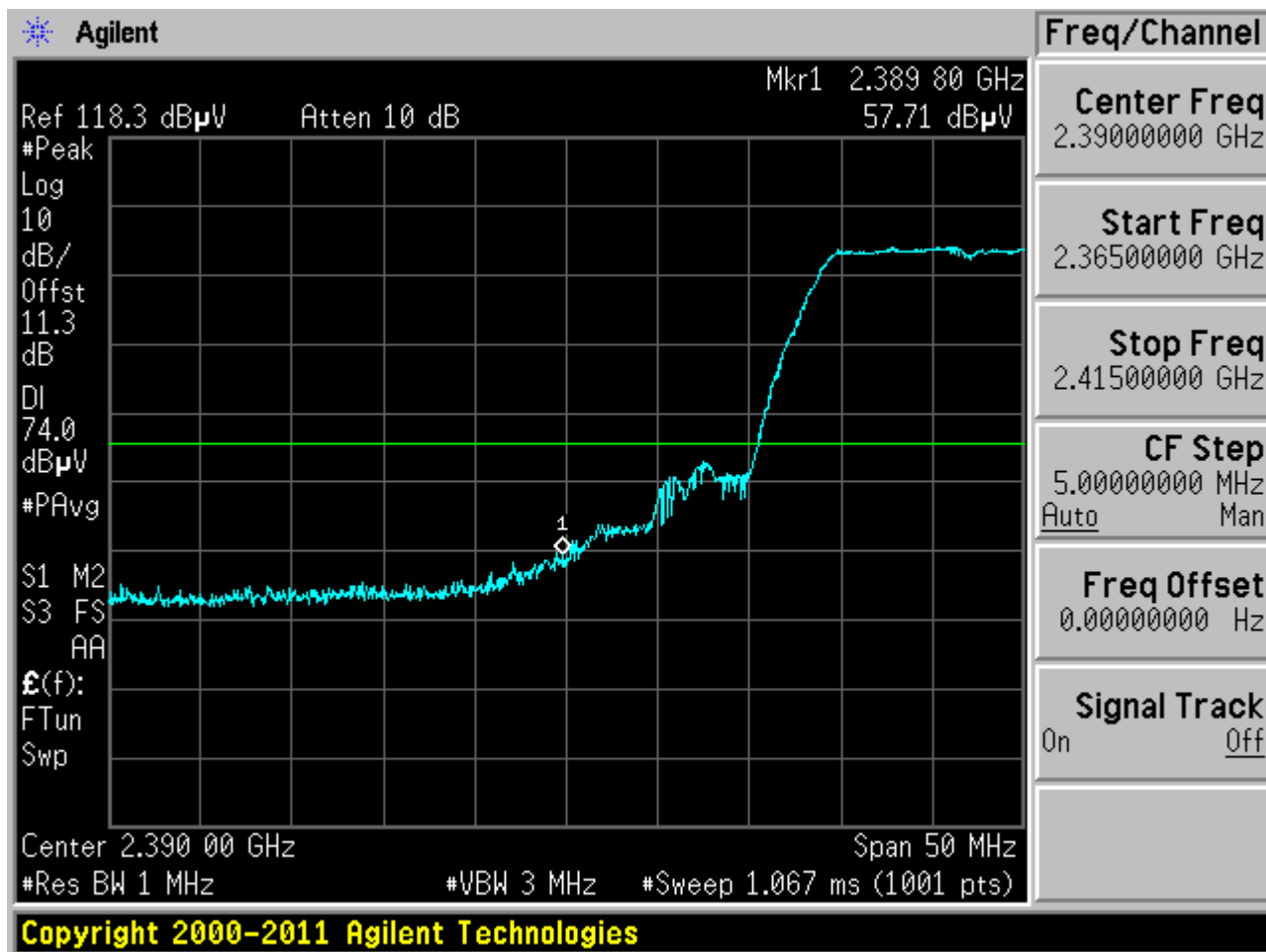
Plot 6-130. Radiated Restricted Lower Band Edge Measurement (Peak)
