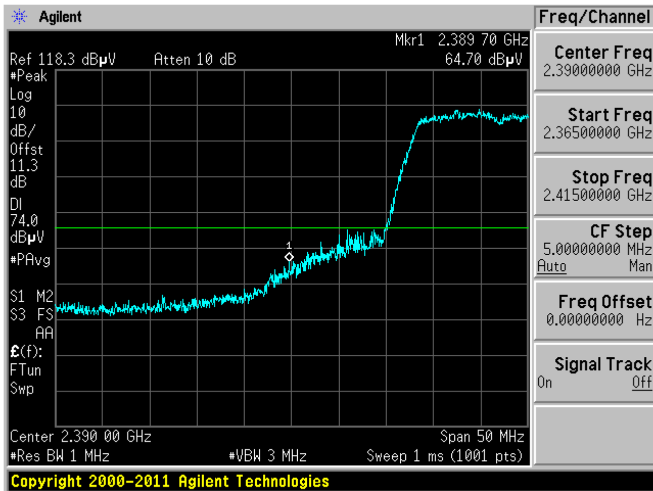
Plot 6-134. Radiated Restricted Lower Band Edge Measurement (Peak)
