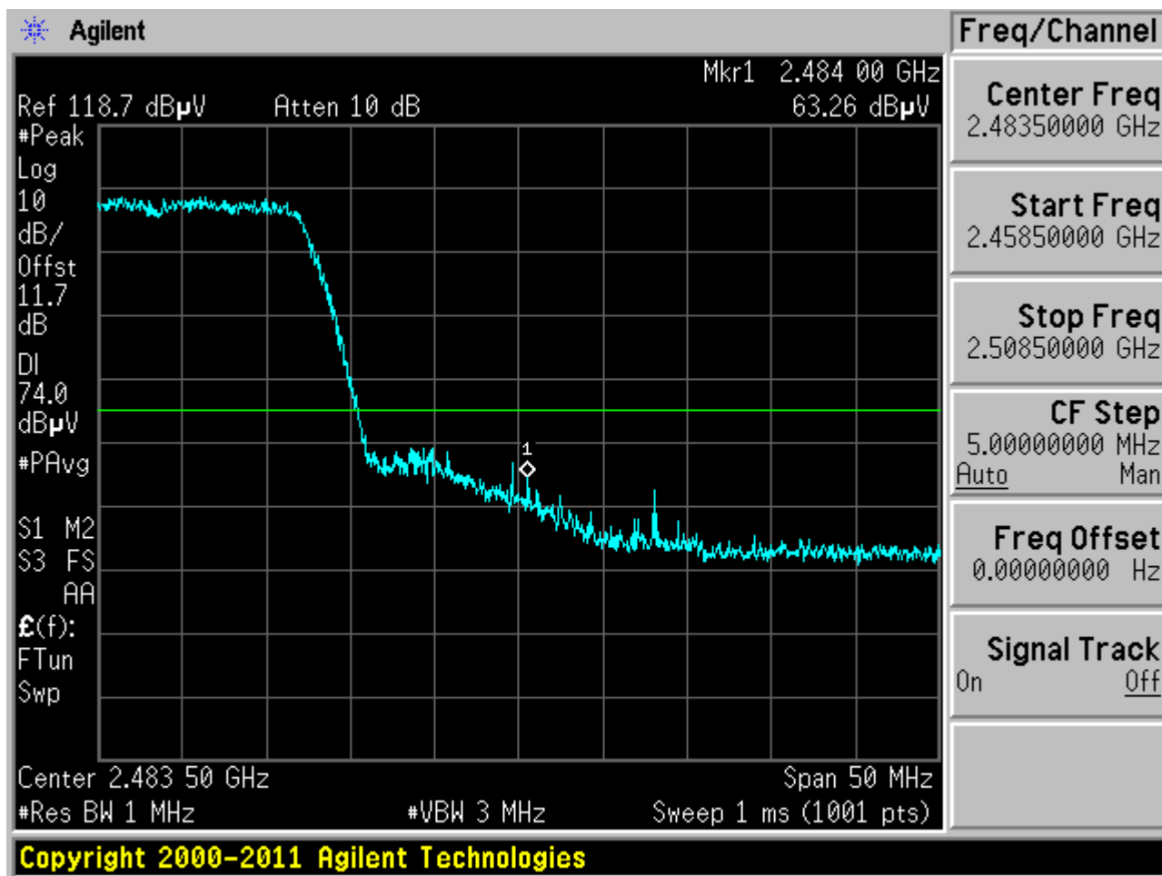
Plot 6-136. Radiated Restricted Upper Band Edge Measurement (Peak)
