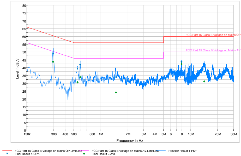
Plot 6-140. Line Conducted Plot with 802.11a (N)
