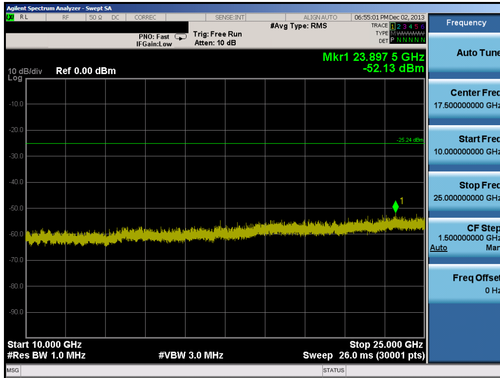
Plot 6-102. Conducted Spurious Plot (802.11b – Ch. 1)
