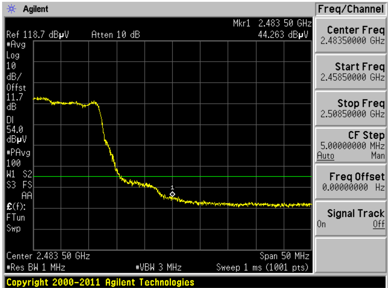
Plot 6-127. Radiated Restricted Upper Band Edge Measurement (Average)
