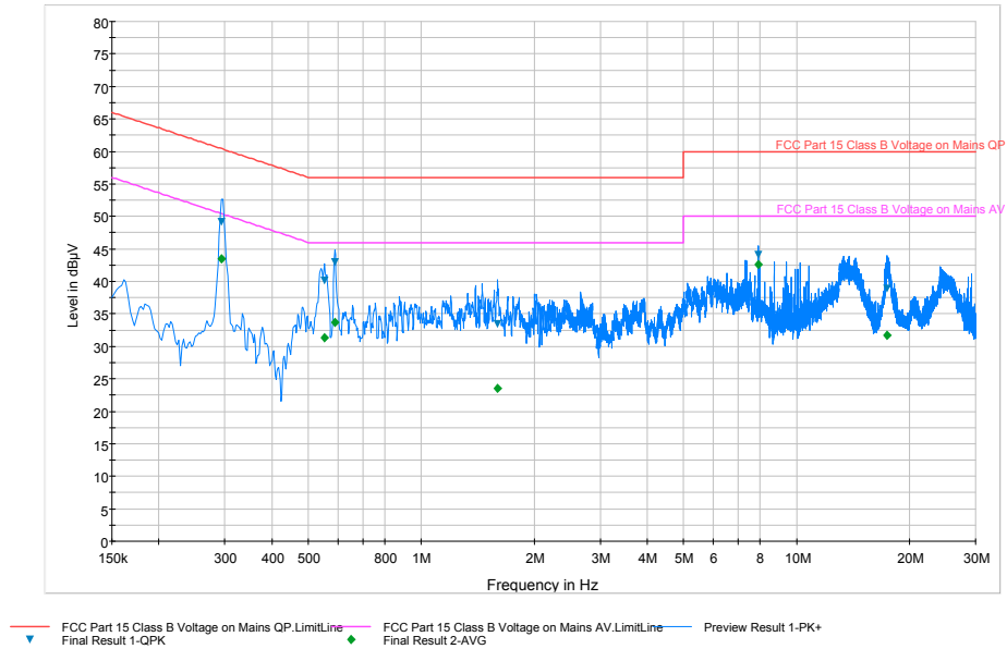
Plot 6-138. Line Conducted Plot with 802.11g (N)
