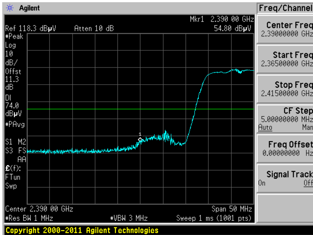
Plot 6-126. Radiated Restricted Lower Band Edge Measurement (Peak)
