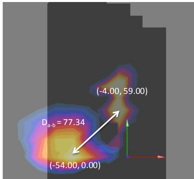
Figure 11-8 Peak SAR Location of 5 GHz WLAN and UMTS 1900 MHz
