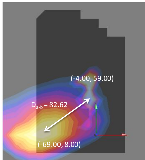
Figure 11-5 Peak SAR Location of 5 GHz WLAN and GRPS 850 MHz
