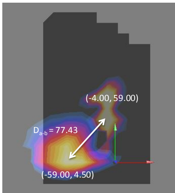
Figure 11-7 Peak SAR Location of 5 GHz WLAN and GPRS 1900 MHz
