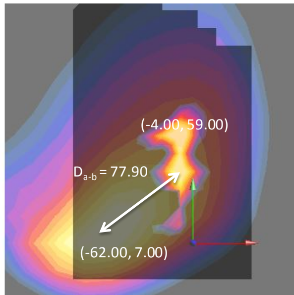
Figure 11-10 Peak SAR Location of 5 GHz WLAN and GPRS 850 MHz
