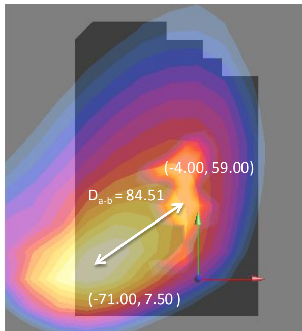
Figure 11-10 Peak SAR Location of 5 GHz WLAN and UMTS 850 MHz
