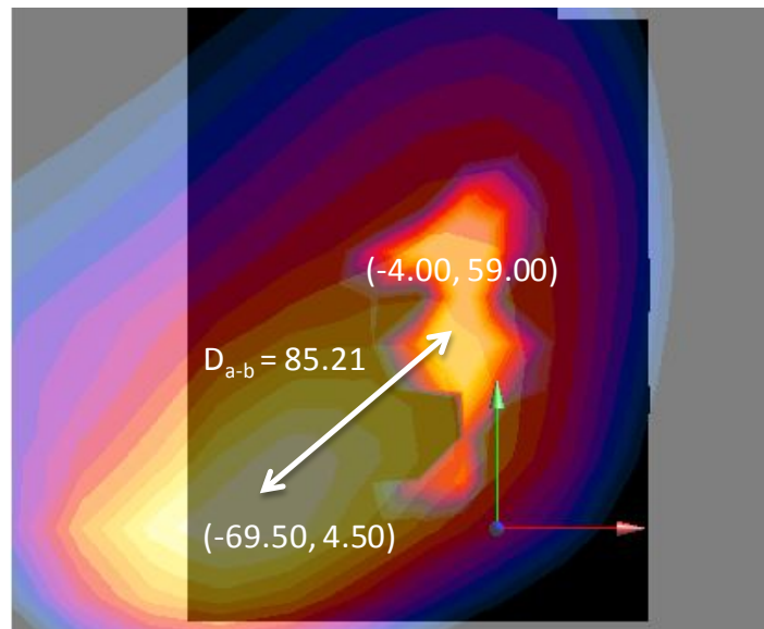
Figure 11-11 Peak SAR Location of 5 GHz WLAN and LTE Band 5 (Cell)
