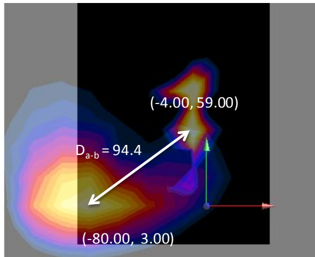
Figure 11-10 Peak SAR Location of 5 GHz WLAN and UMTS 1900 MHz
