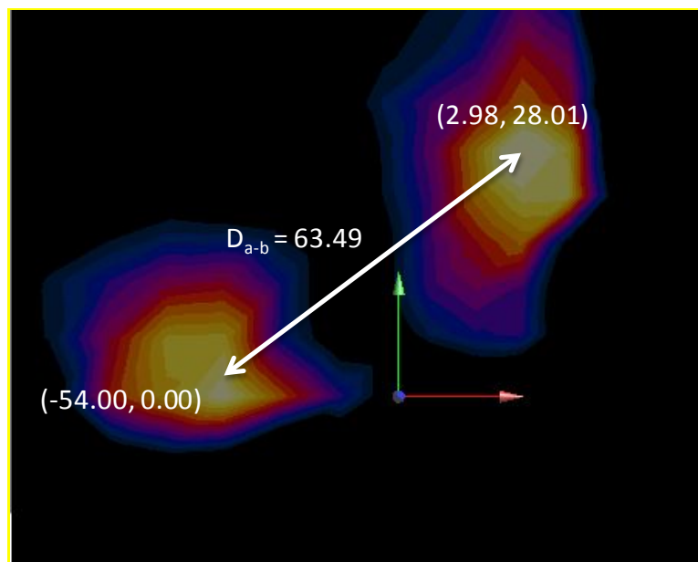
Figure 11-4 Peak SAR Locations of 2.4 GHz WLAN and UMTS 1900 MHz
