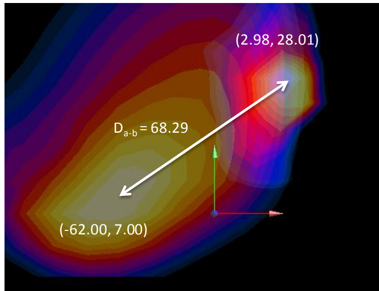
Figure 11-9 Peak SAR Location of 2.4 GHz WLAN and GPRS 850 MHz
