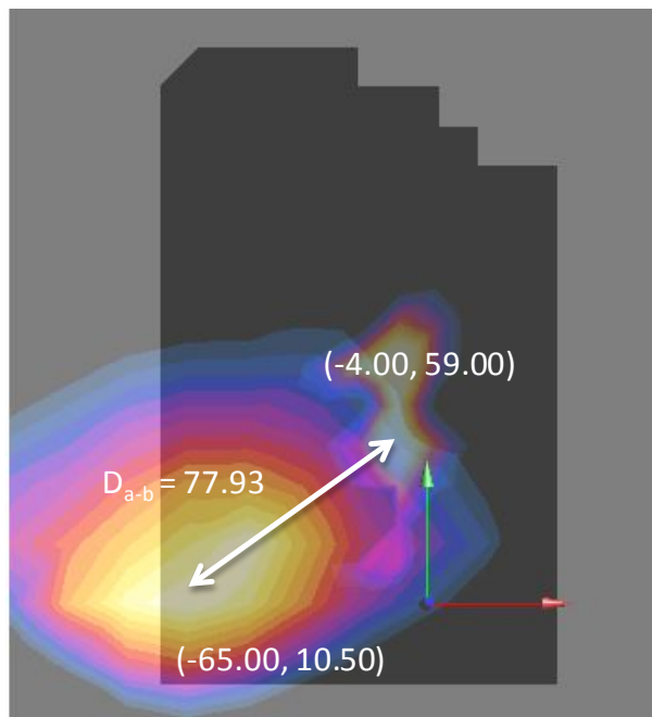
Figure 11-6 Peak SAR Location of 5 GHz WLAN and UMTS 850 MHz
