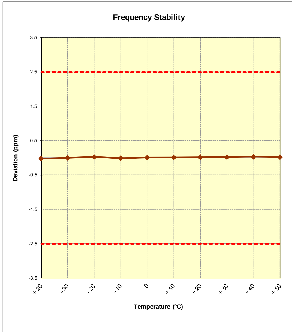
Figure 6-8. Frequency Stability Graph (Cellular WCDMA Mode – Ch. 4183)
