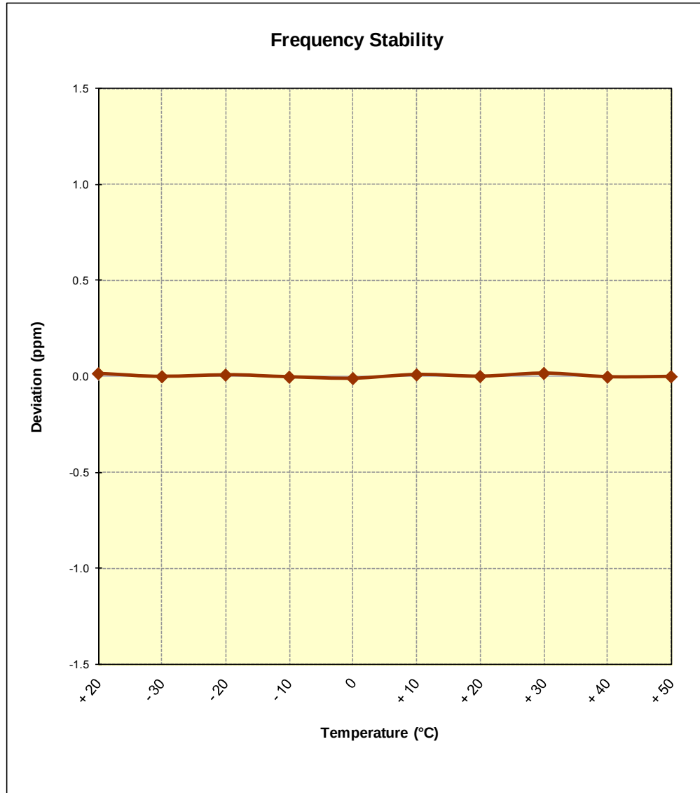
Figure 6-10. Frequency Stability Graph (PCS WCDMA Mode – Ch. 9400)
