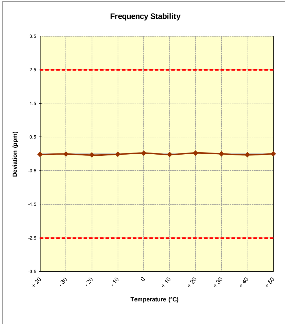
Figure 6-7. Frequency Stability Graph (Cellular GSM Mode – Ch. 190)
