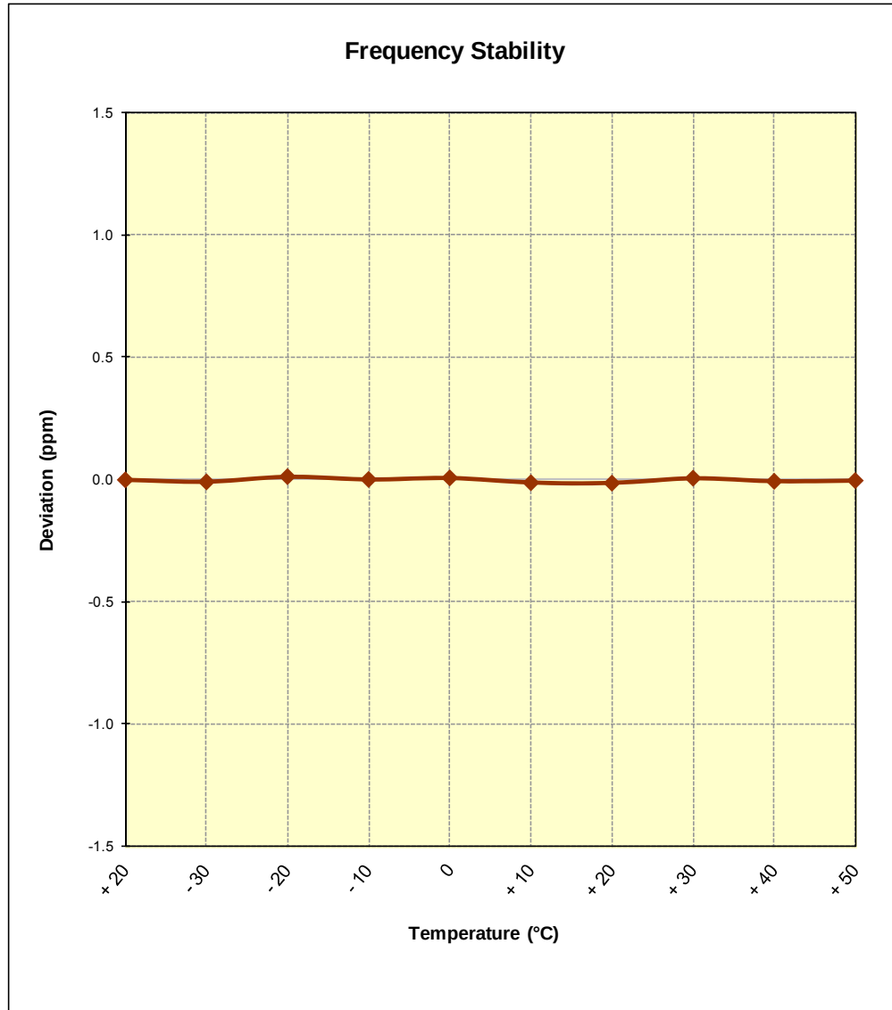
Figure 6-9. Frequency Stability Graph (PCS GSM Mode – Ch. 661)
