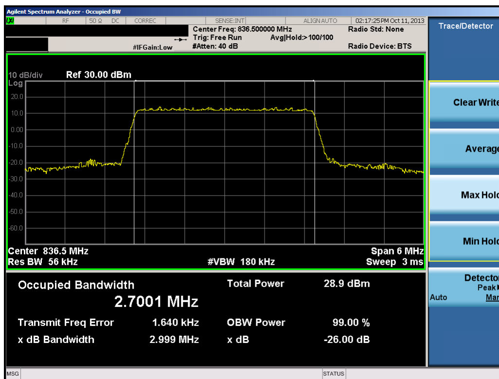
Plot 7-13. Occupied Bandwidth Plot (3.0MHz 16-QAM – RB Size 15)
