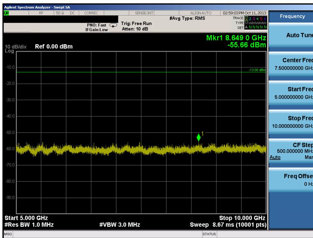
Plot 7-35. Conducted Spurious Plot (10.0MHz QPSK – RB Size 1, RB Offset 0 – Low Channel)
