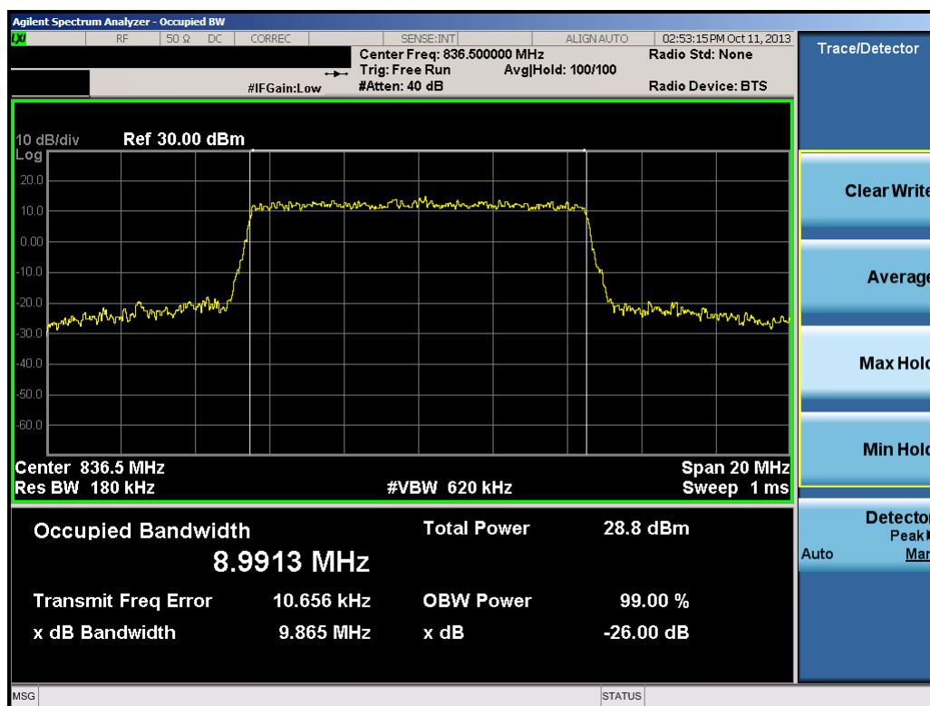
Plot 7-33. Occupied Bandwidth Plot (10.0MHz 16-QAM – RB Size 50)
