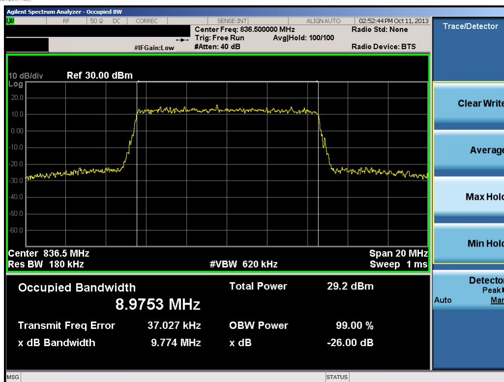
Plot 7-32. Occupied Bandwidth Plot (10.0MHz QPSK – RB Size 50)
