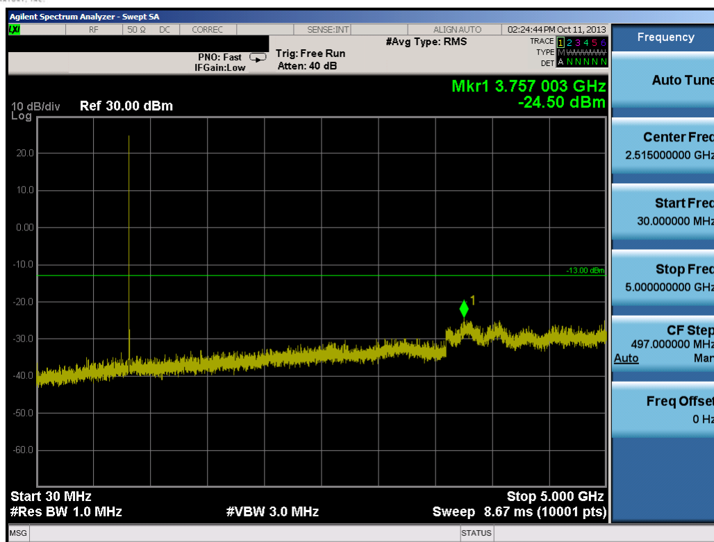
Plot 7-16. Conducted Spurious Plot (3.0MHz QPSK – RB Size 1, RB Offset 0 – Mid Channel)
