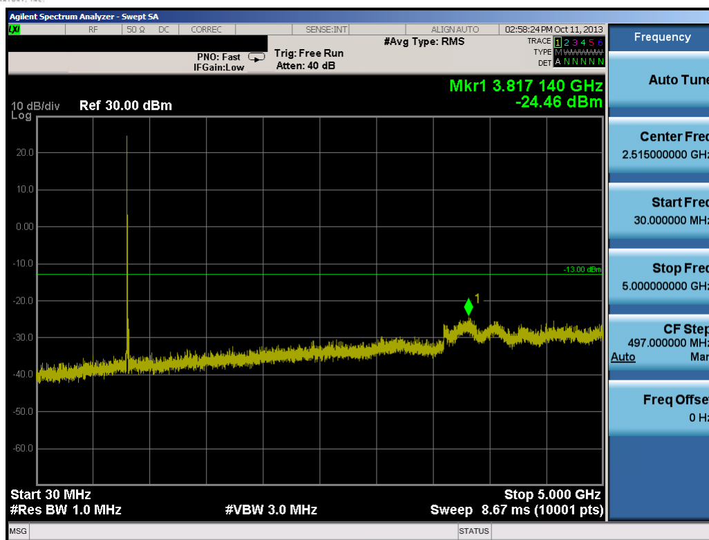
Plot 7-34. Conducted Spurious Plot (10.0MHz QPSK – RB Size 1, RB Offset 0– Low Channel)
