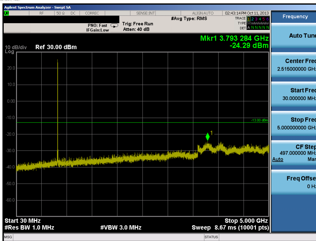
Plot 7-28. Conducted Spurious Plot (5.0MHz QPSK – RB Size 1, RB Offset 0 – High Channel)
