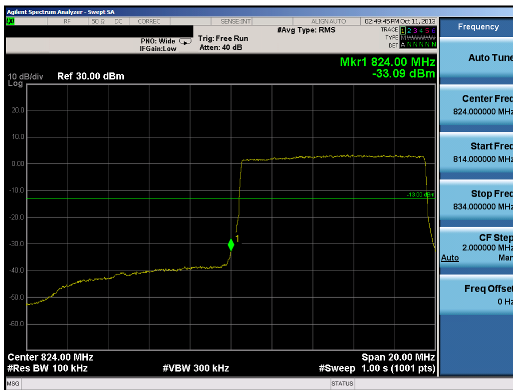
Plot 7-31. Lower Band Edge Plot (10.0MHz QPSK – RB Size 50)
