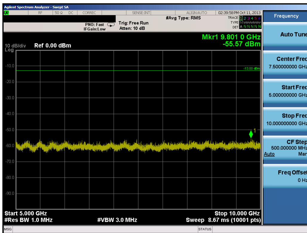
Plot 7-25. Conducted Spurious Plot (5.0MHz QPSK – RB Size 1, RB Offset 0 – Low Channel)
