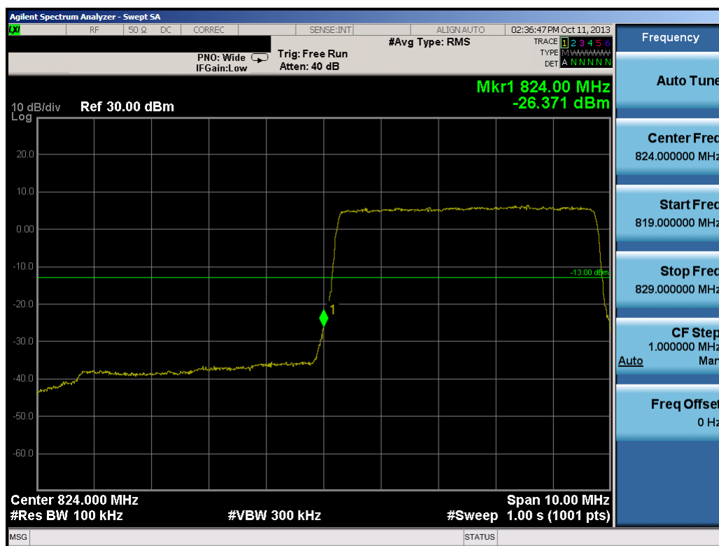
Plot 7-21. Lower Band Edge Plot (5.0MHz QPSK – RB Size 25)
