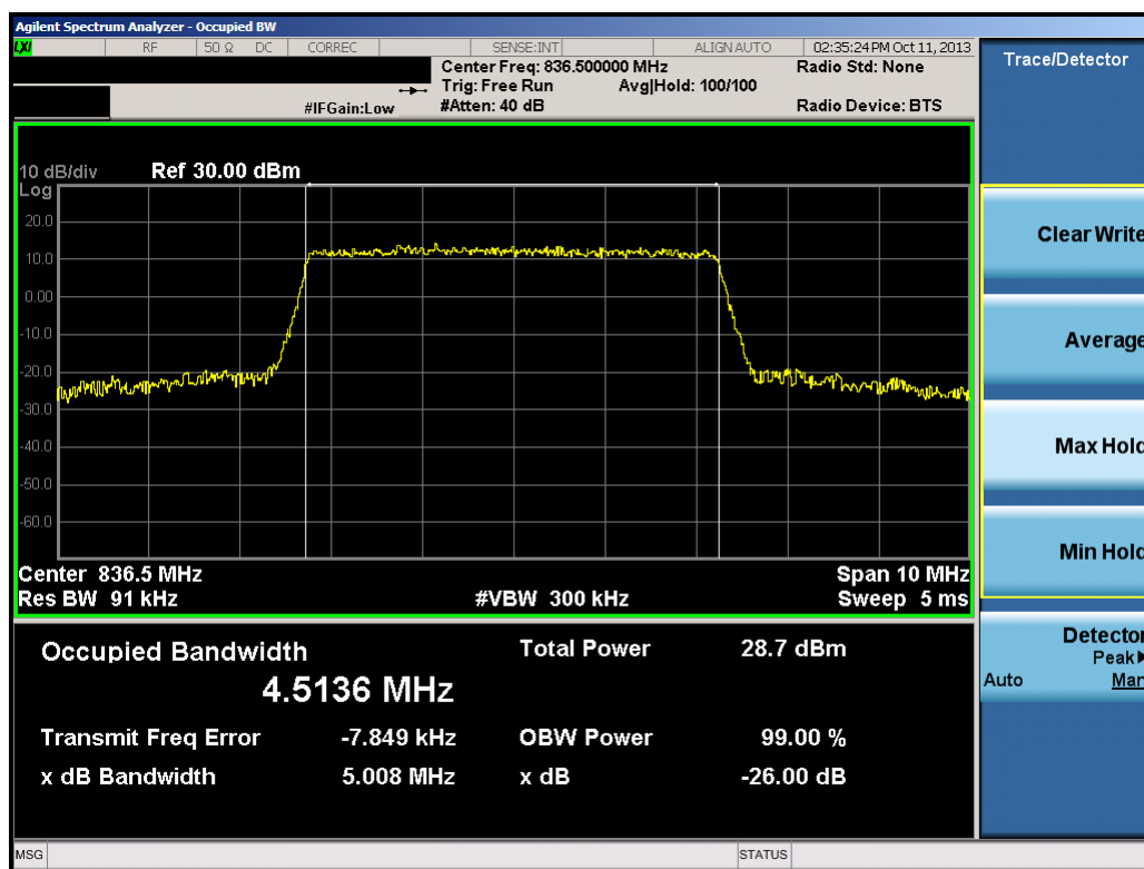
Plot 7-23. Occupied Bandwidth Plot (5.0MHz 16-QAM – RB Size 25)
