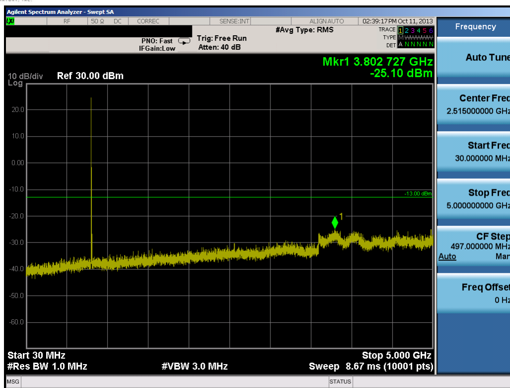
Plot 7-24. Conducted Spurious Plot (5.0MHz QPSK – RB Size 1, RB Offset 0 – Low Channel)
