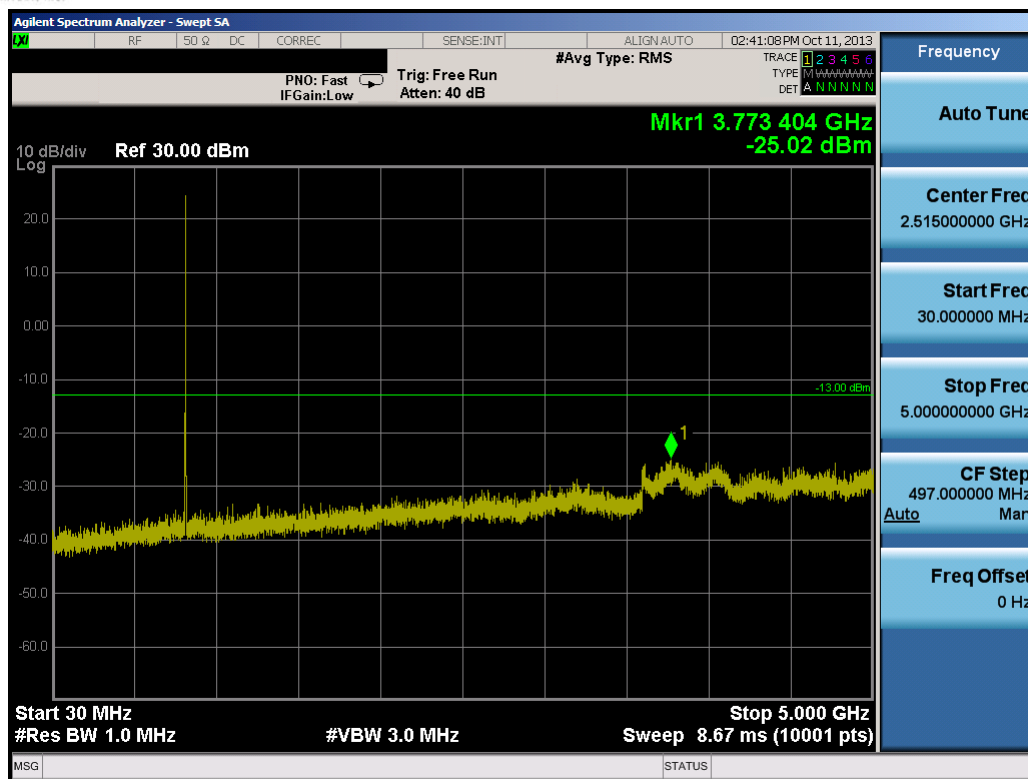
Plot 7-26. Conducted Spurious Plot (5.0MHz QPSK – RB Size 1, RB Offset 0 – Mid Channel)
