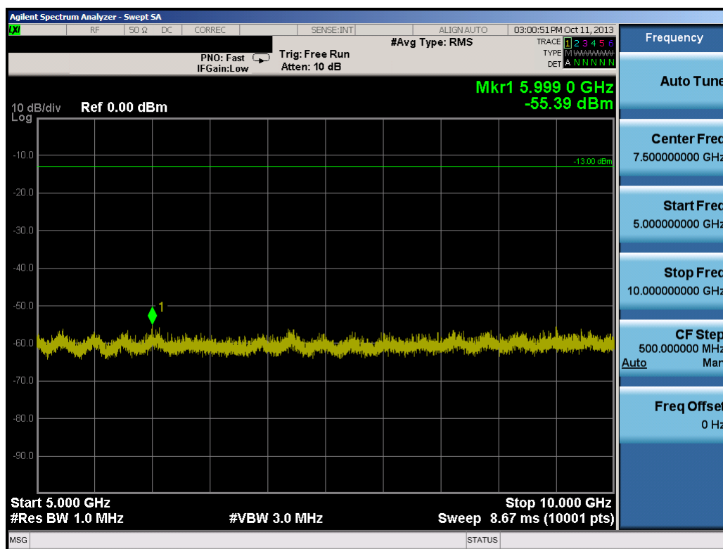
Plot 7-39. Conducted Spurious Plot (10.0MHz QPSK – RB Size 1, RB Offset 0 – High Channel)
