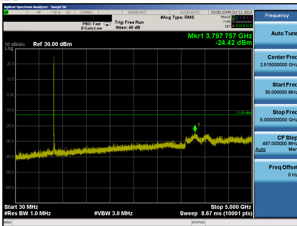
Plot 7-38. Conducted Spurious Plot (10.0MHz QPSK – RB Size 1, RB Offset 0 – High Channel)
