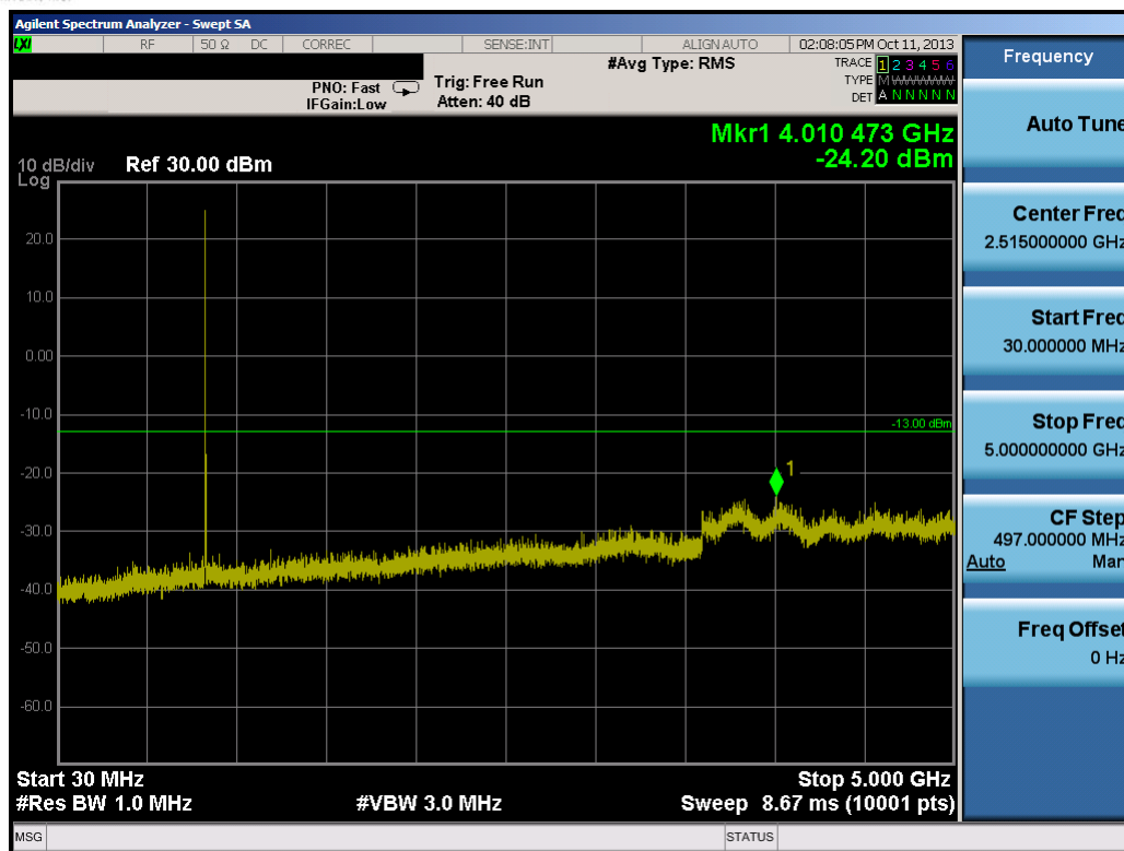
Plot 7-8. Conducted Spurious Plot (1.4MHz QPSK – RB Size 1, RB Offset 0 – High Channel)
