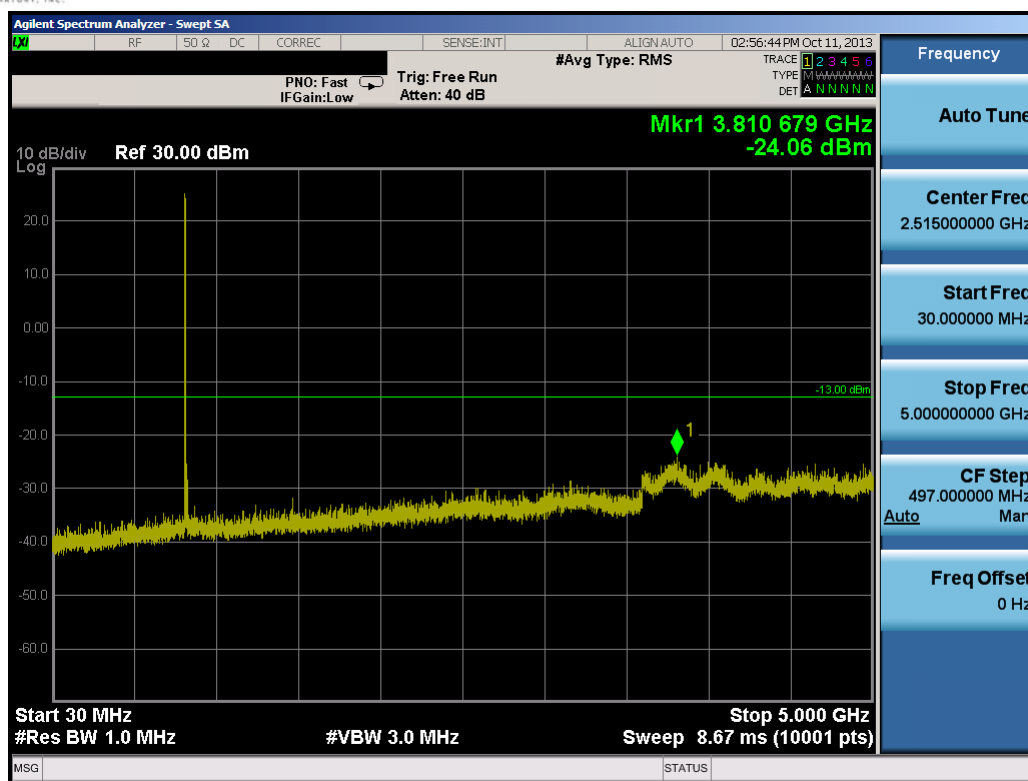
Plot 7-36. Conducted Spurious Plot (10.0MHz QPSK – RB Size 1, RB Offset 0 – Mid Channel)
