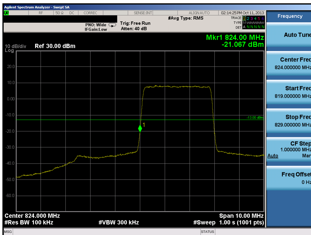
Plot 7-11. Lower Band Edge Plot (3.0MHz QPSK – RB Size 15)
