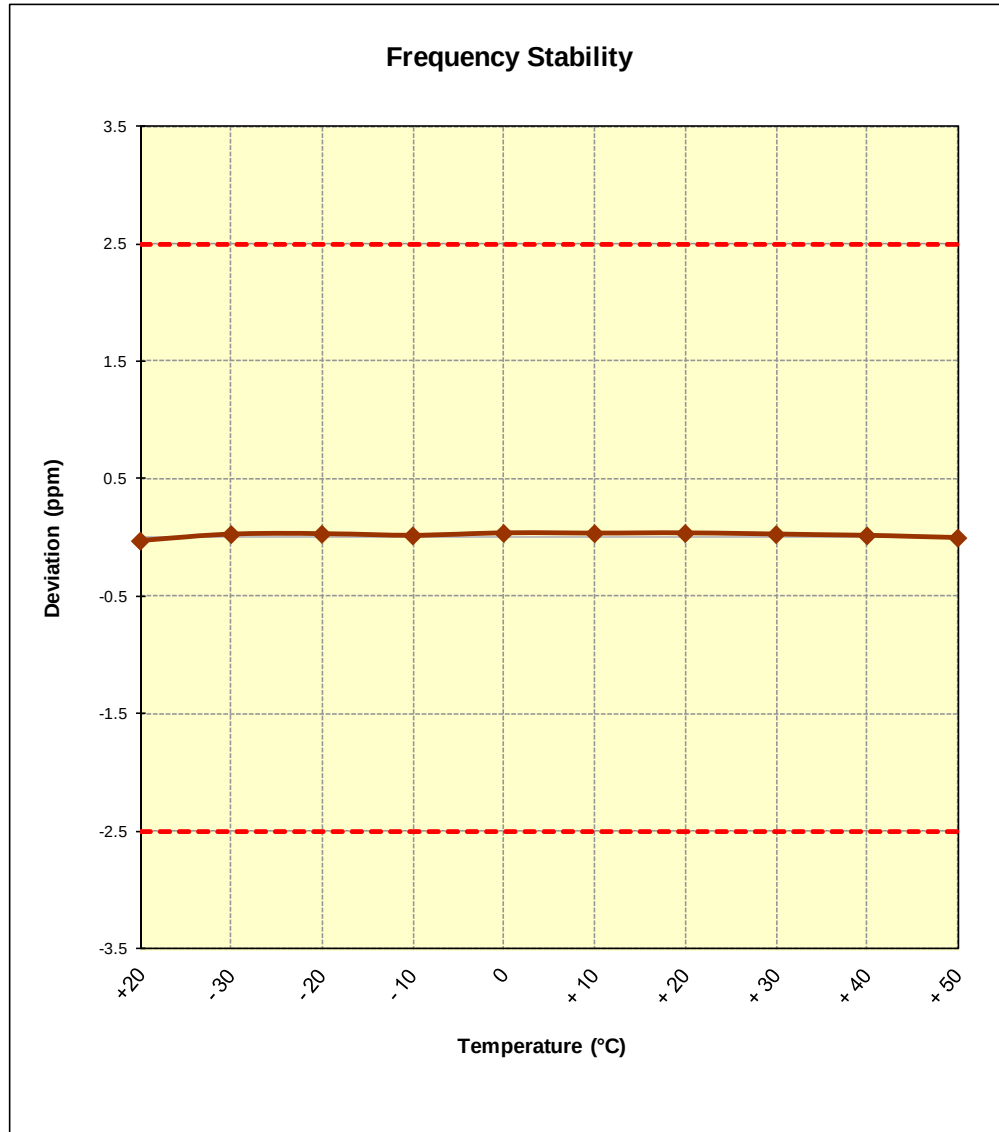
Figure 6-1. Frequency Stability Graph (Band 5)
