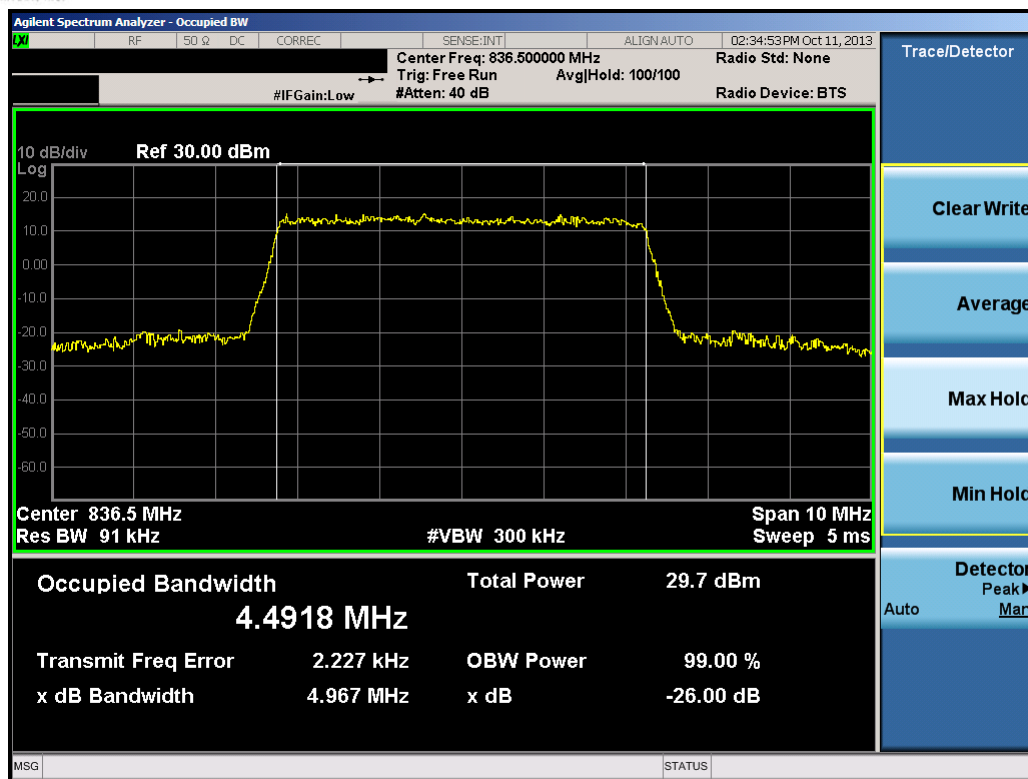
Plot 7-22. Occupied Bandwidth Plot (5.0MHz QPSK – RB Size 25)
