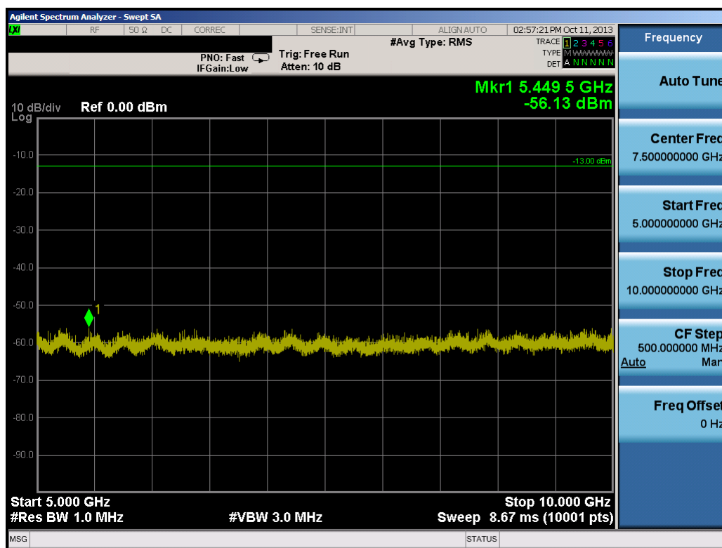
Plot 7-37. Conducted Spurious Plot (10.0MHz QPSK – RB Size 1, RB Offset 0 – Mid Channel)
