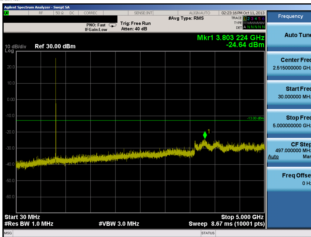
Plot 7-14. Conducted Spurious Plot (3.0MHz QPSK – RB Size 1, RB Offset 0 – Low Channel)
