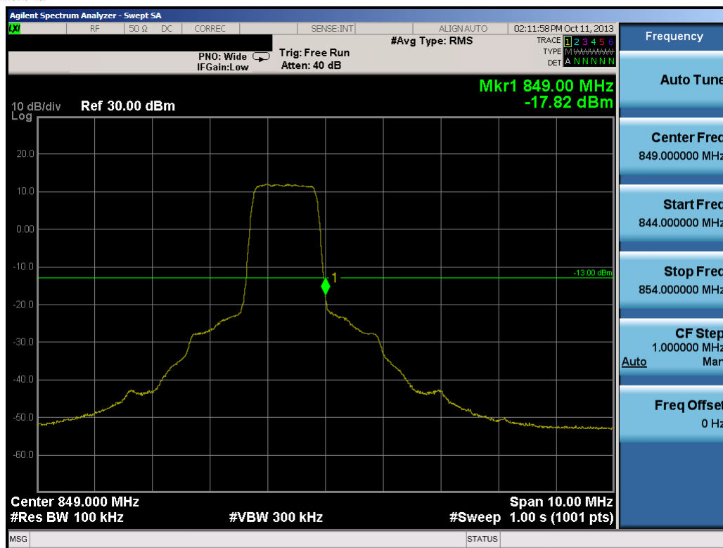
Plot 7-10. Upper Band Edge Plot (1.4MHz QPSK – RB Size 6)
