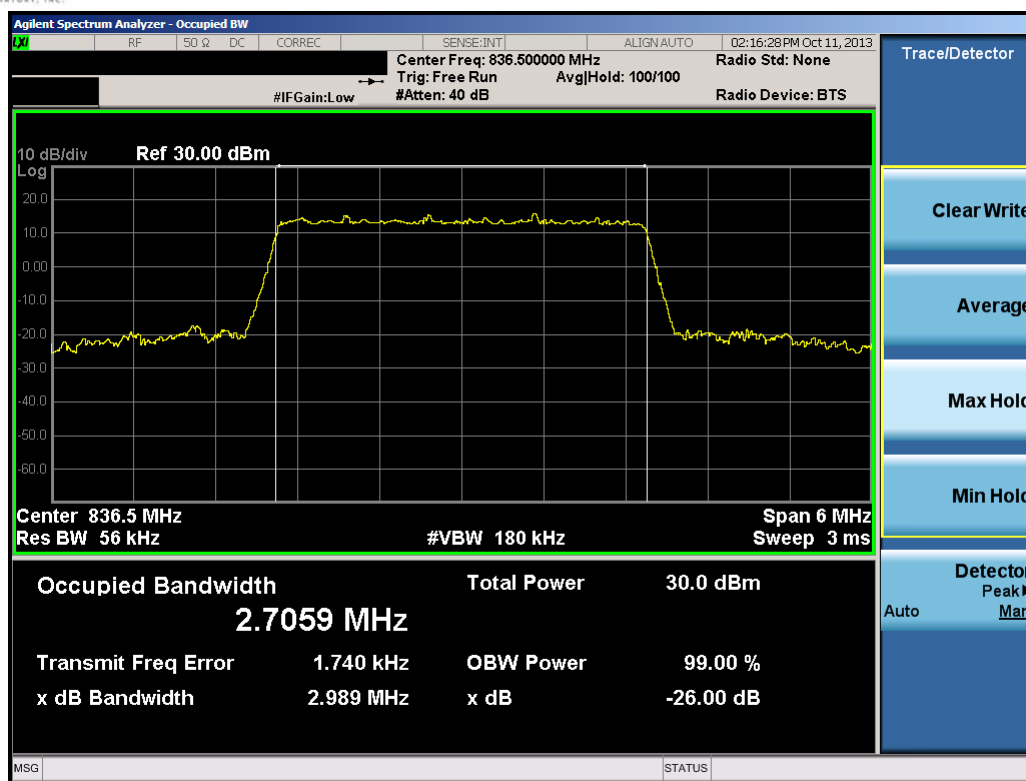
Plot 7-12. Occupied Bandwidth Plot (3.0MHz QPSK – RB Size 15)
