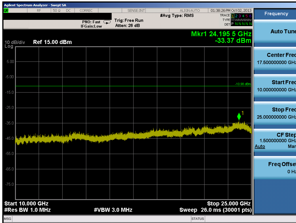
Plot 6-39. Conducted Spurious Plot (Bluetooth, 1Mbps – Ch. 39)
