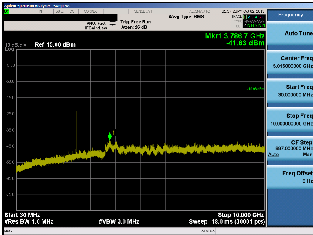
Plot 6-38. Conducted Spurious Plot (Bluetooth, 1Mbps – Ch. 39)
