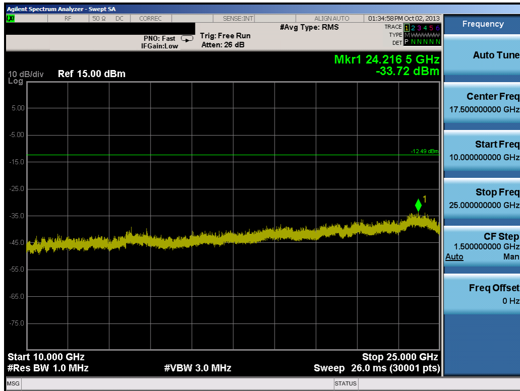
Plot 6-37. Conducted Spurious Plot (Bluetooth, 1Mbps – Ch. 0)
