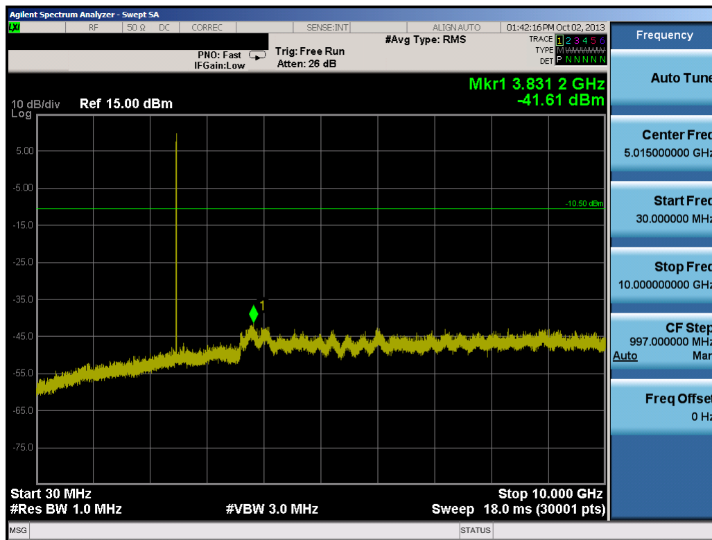
Plot 6-40. Conducted Spurious Plot (Bluetooth, 1Mbps – Ch. 78)
