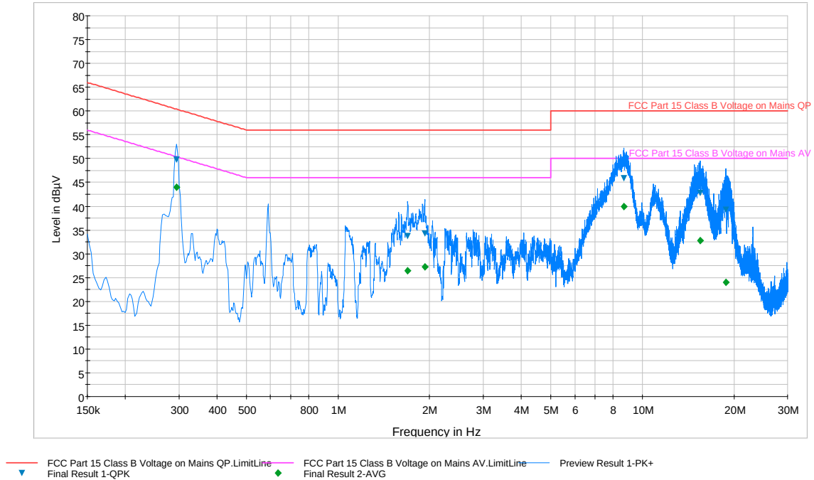
Plot 6-86. Line Conducted Plot with 802.11a UNII Band 1 (N)
