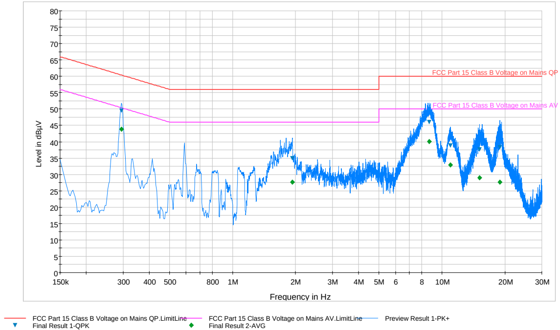
Plot 6-85. Line Conducted Plot with 802.11a UNII Band 1 (L1)
