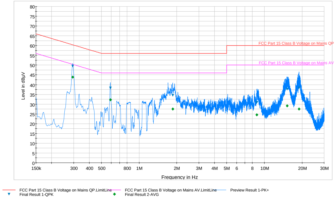
Plot 6-89. Line Conducted Plot with 802.11a UNII Band 3 (L1)
