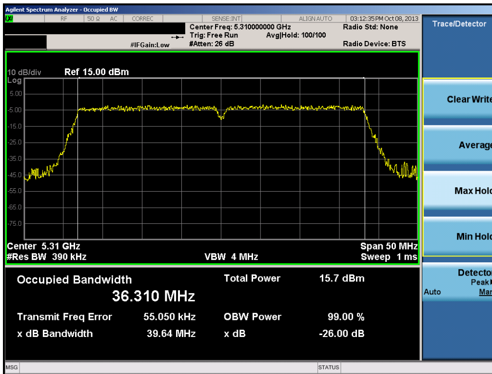
Plot 6-17. 26dB Bandwidth Plot (40MHz BW 802.11n (UNII Band 2) – Ch. 62)
