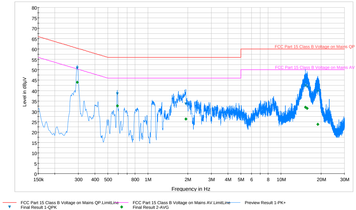
Plot 6-88. Line Conducted Plot with 802.11a UNII Band 2 (N)
