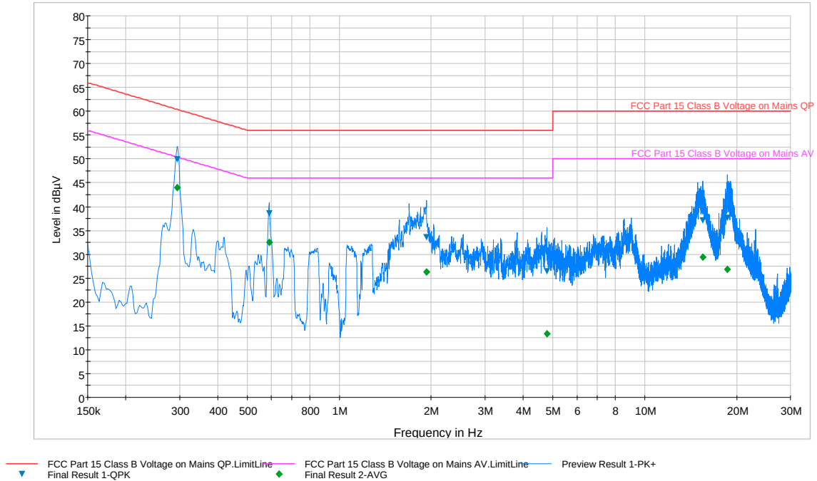
Plot 6-87. Line Conducted Plot with 802.11a UNII Band 2 (L1)
