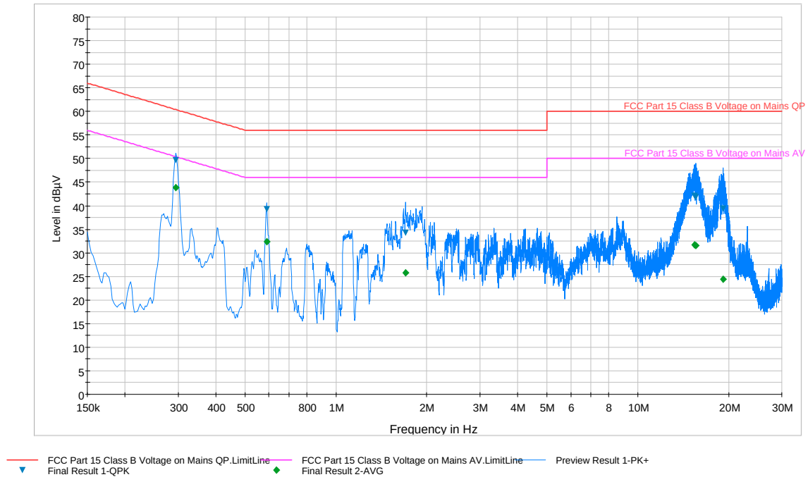
Plot 6-90. Line Conducted Plot with 802.11a UNII Band 3 (N)
