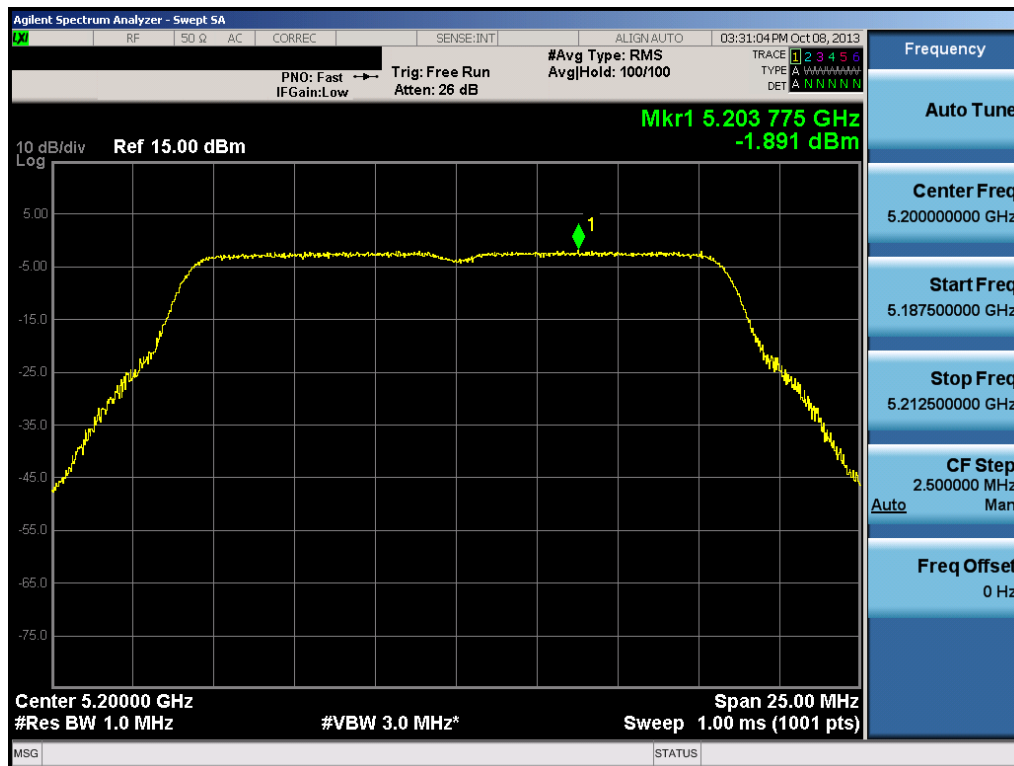
Plot 6-34. Peak Power Spectral Density Plot (802.11a (UNII Band 1) – Ch. 40)
