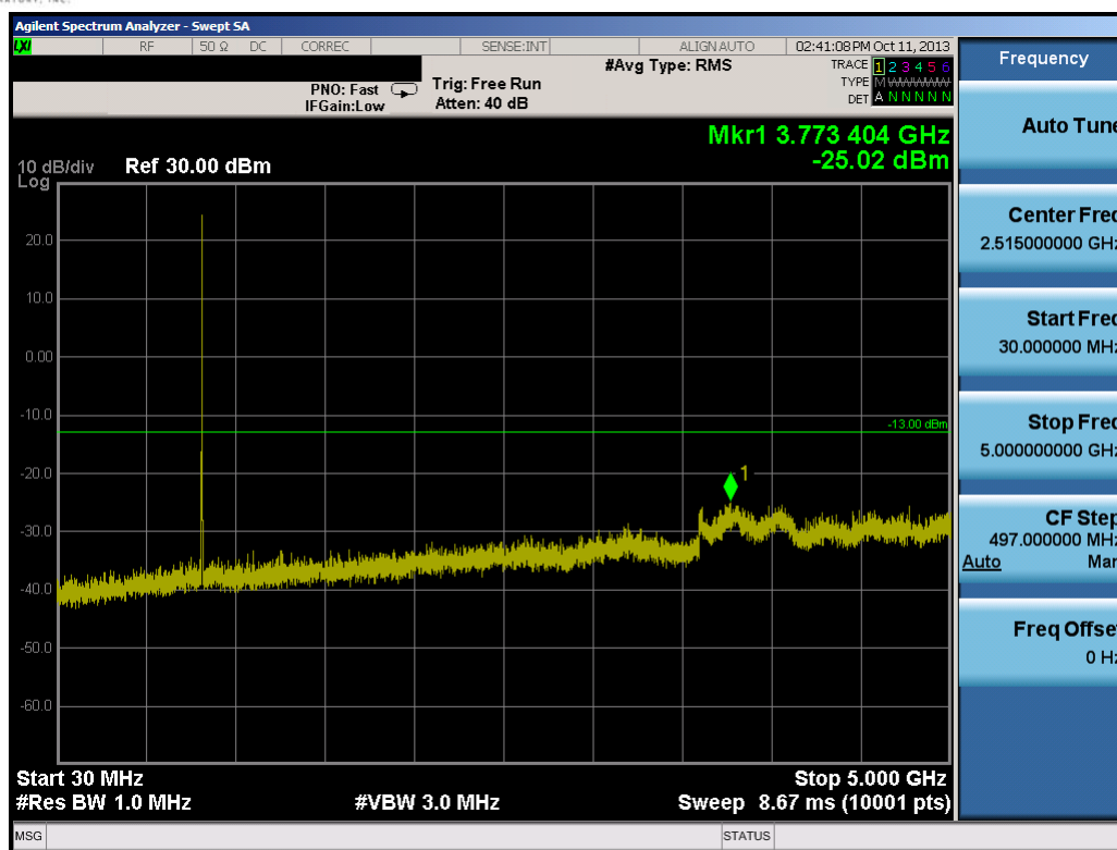
Plot 7-26. Conducted Spurious Plot (5.0MHz QPSK – RB Size 1, RB Offset 0 – Mid Channel)
