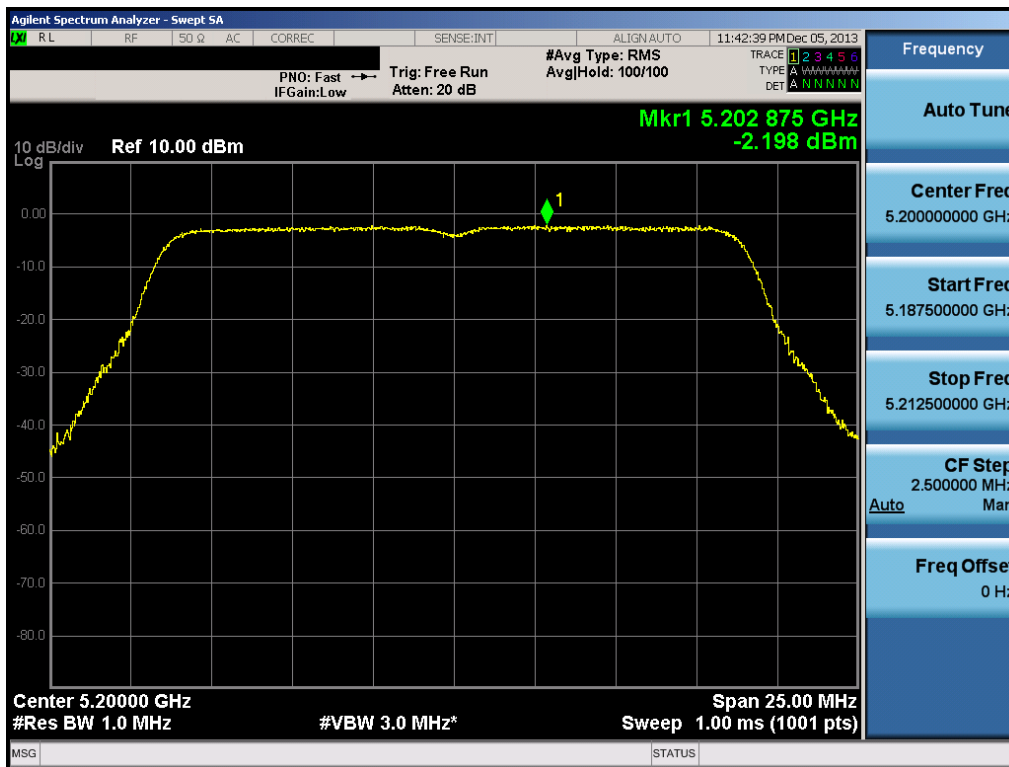
Plot 6-68. Peak Power Spectral Density Plot (20MHz BW 802.11n (UNII Band 1) – Ch. 40)
