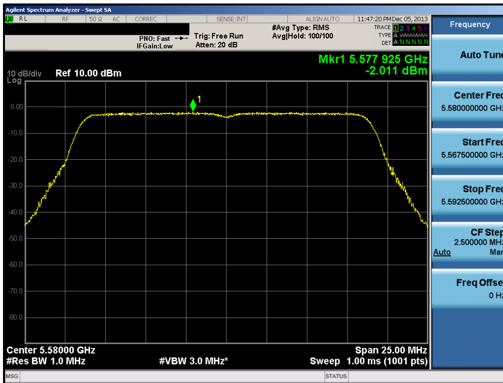
Plot 6-86. Peak Power Spectral Density Plot (20MHz BW 802.11n (UNII Band 2C) – Ch. 116)
