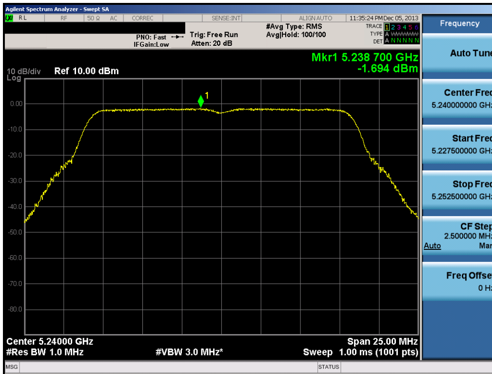
Plot 6-66. Peak Power Spectral Density Plot (802.11a (UNII Band 1) – Ch. 48)
