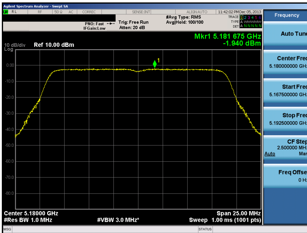
Plot 6-67. Peak Power Spectral Density Plot (20MHz BW 802.11n (UNII Band 1) – Ch. 36)
