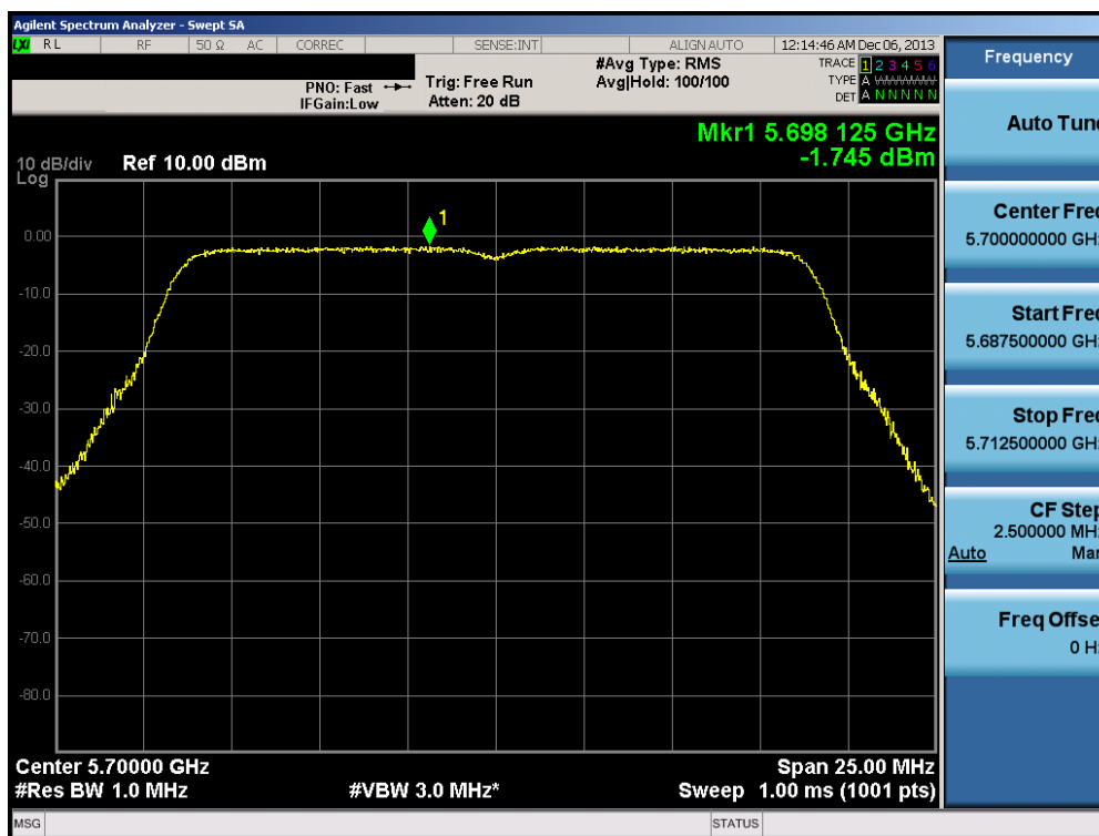
Plot 6-115. Peak Power Spectral Density Plot (20MHz BW 802.11n (UNII Band 2C) – Ch. 140)
