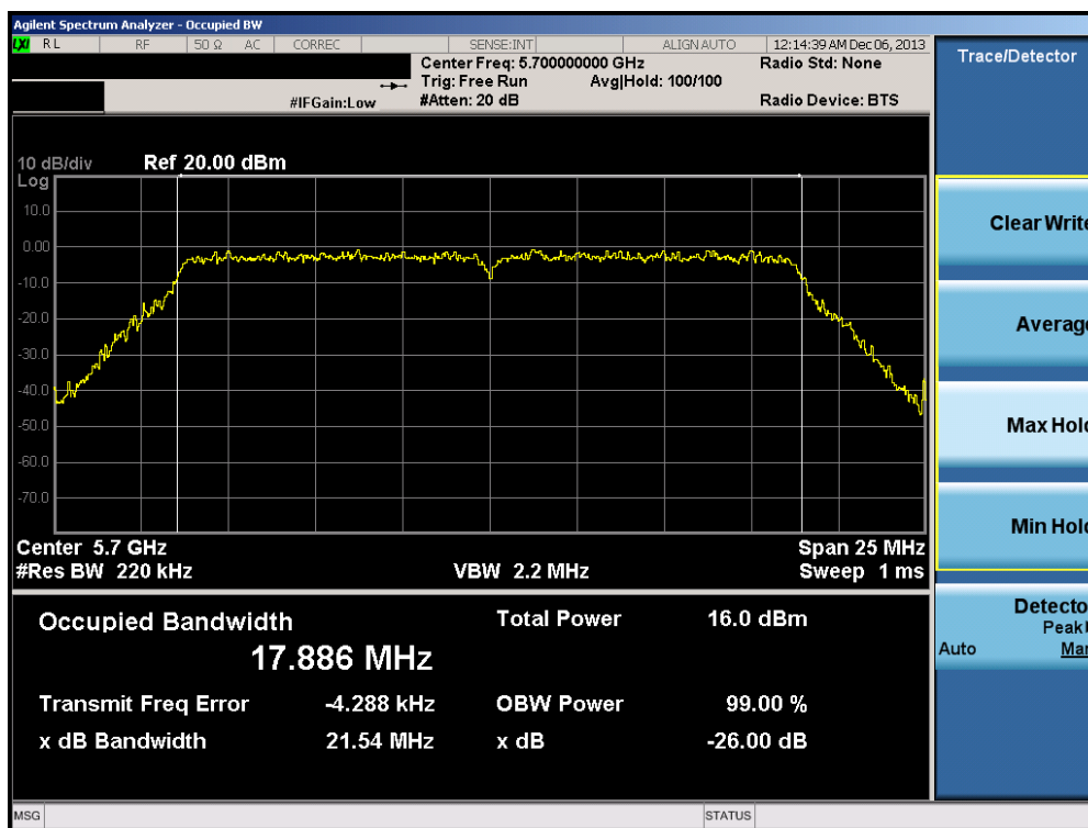
Plot 6-55. 26dB Bandwidth Plot (20MHz BW 802.11n (UNII Band 2C) – Ch. 140)
