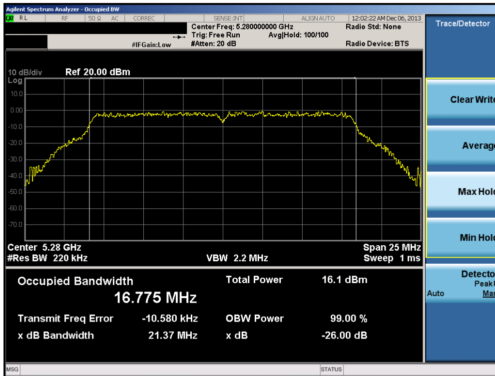
Plot 6-42. 26dB Bandwidth Plot (802.11a (UNII Band 2A) – Ch. 56)
