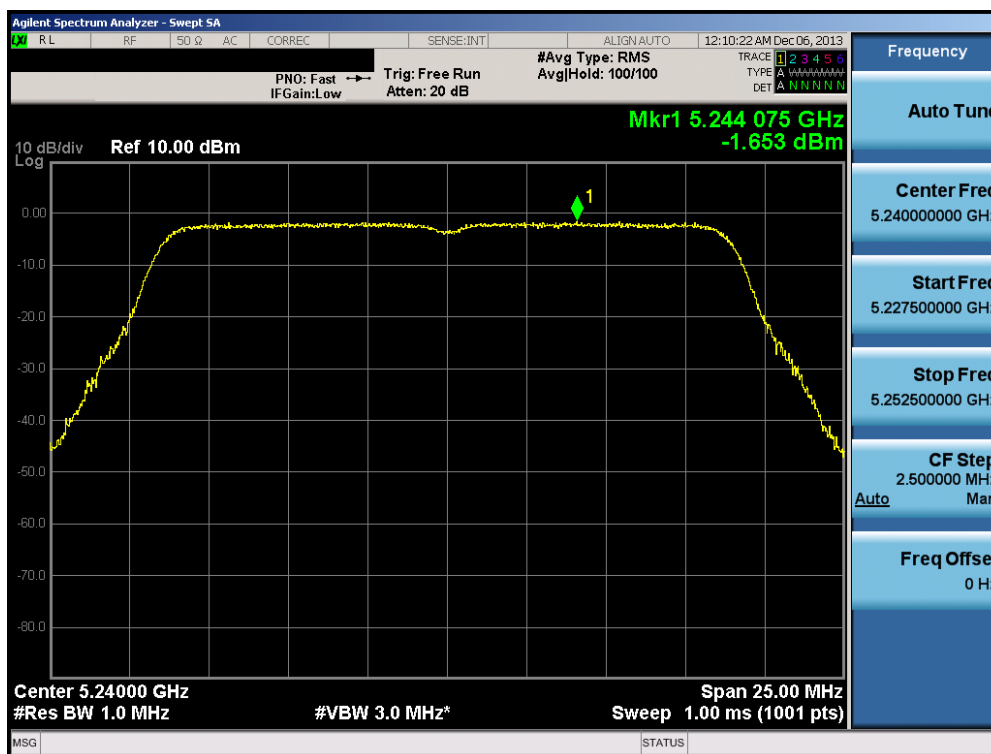
Plot 6-97. Peak Power Spectral Density Plot (20MHz BW 802.11n (UNII Band 1) – Ch. 48)
