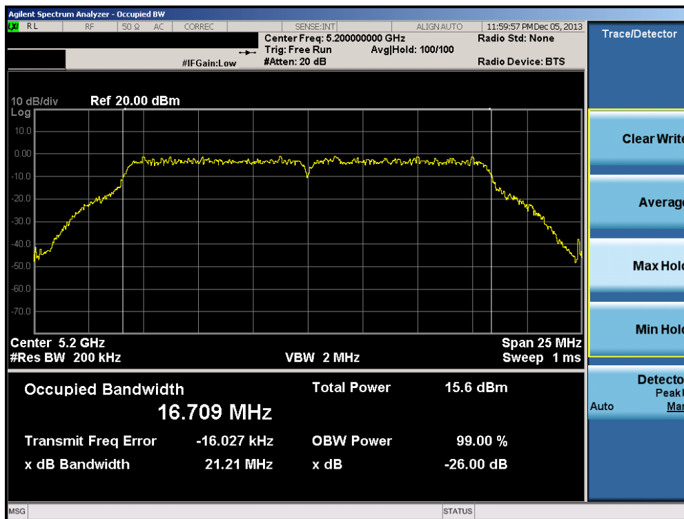
Plot 6-33. 26dB Bandwidth Plot (802.11a (UNII Band 1) – Ch. 40)
