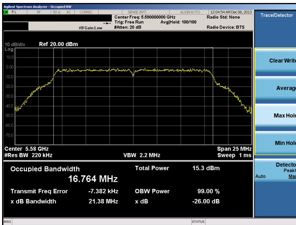
Plot 6-51. 26dB Bandwidth Plot (802.11a (UNII Band 2C) – Ch. 116)
