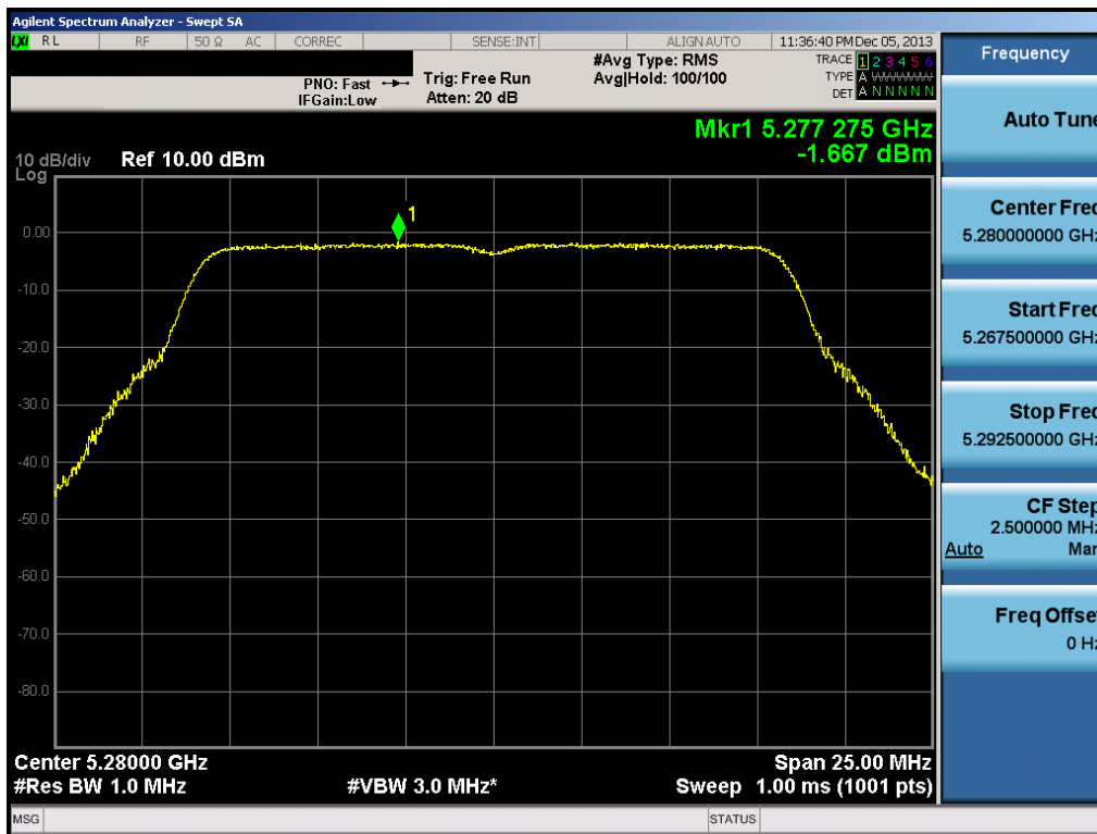
Plot 6-74. Peak Power Spectral Density Plot (802.11a (UNII Band 2A) – Ch. 56)
