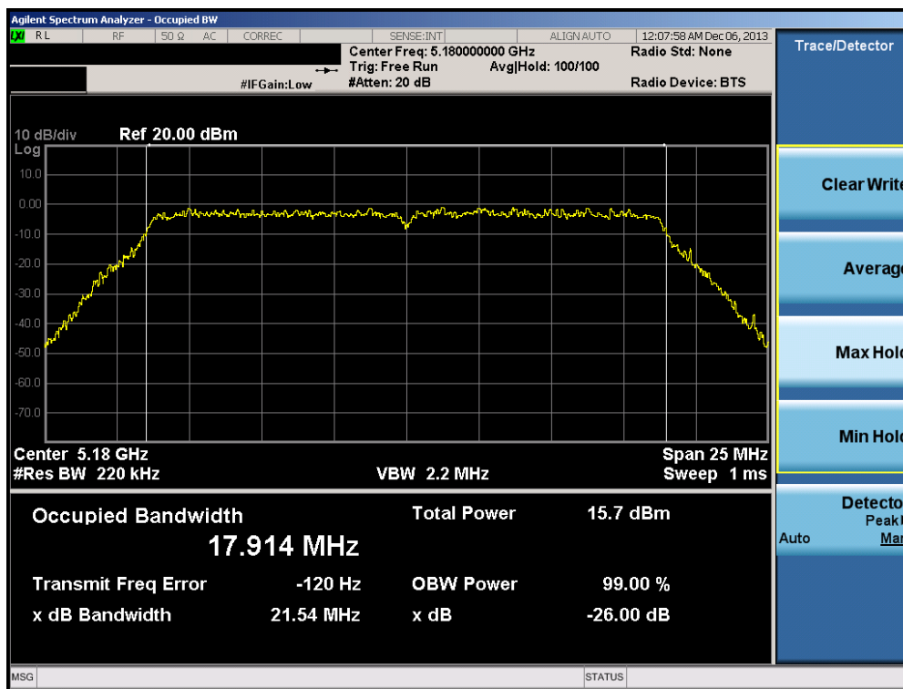
Plot 6-35. 26dB Bandwidth Plot (20MHz BW 802.11n (UNII Band 1) – Ch. 36)
