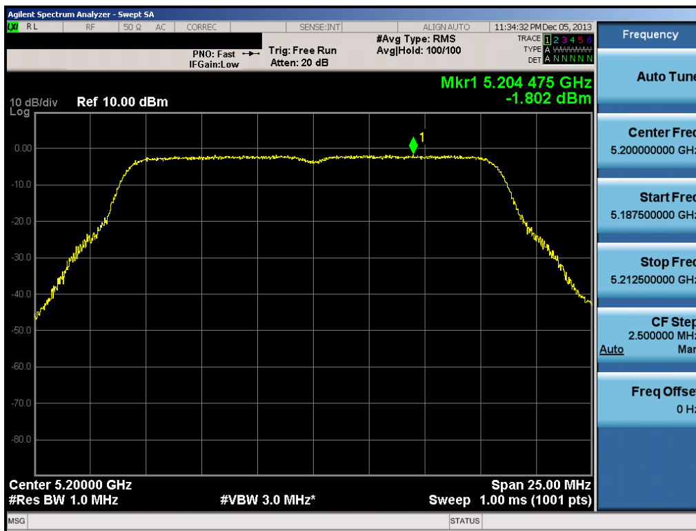
Plot 6-65. Peak Power Spectral Density Plot (802.11a (UNII Band 1) – Ch. 40)
