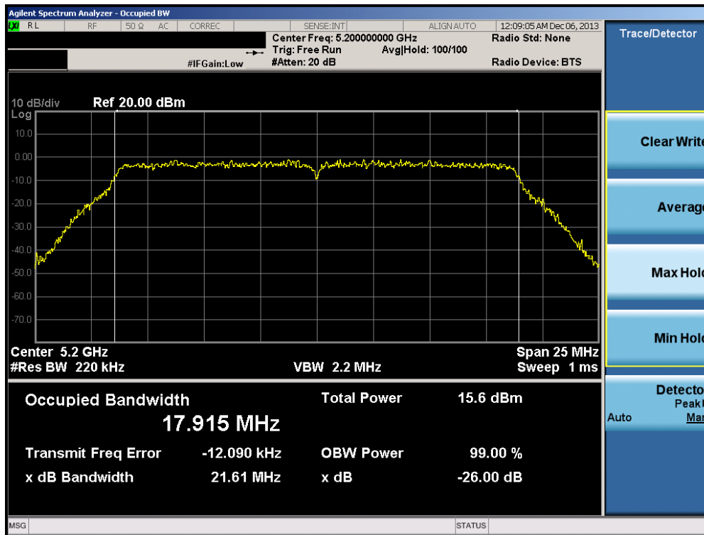
Plot 6-36. 26dB Bandwidth Plot (20MHz BW 802.11n (UNII Band 1) – Ch. 40)
