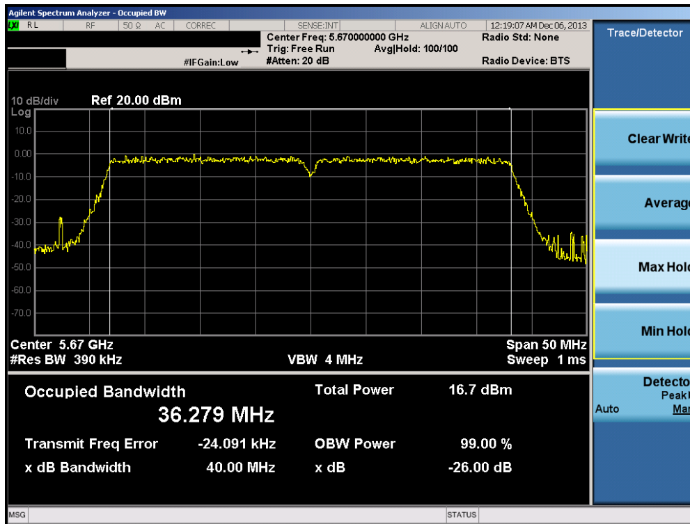
Plot 6-58. 26dB Bandwidth Plot (40MHz BW 802.11n (UNII Band 2C) – Ch. 134)
