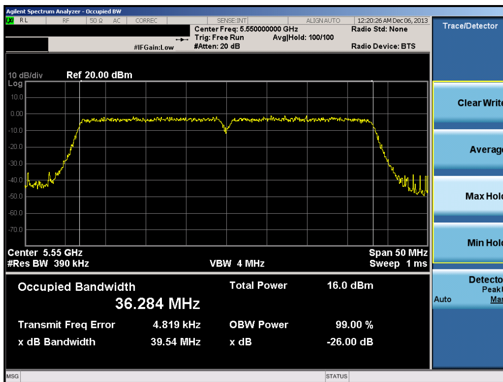
Plot 6-57. 26dB Bandwidth Plot (40MHz BW 802.11n (UNII Band 2C) – Ch. 110)
