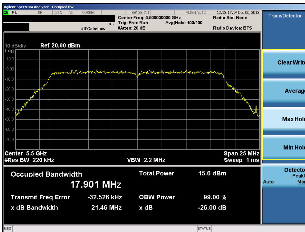
Plot 6-53. 26dB Bandwidth Plot (20MHz BW 802.11n (UNII Band 2C) – Ch. 100)
