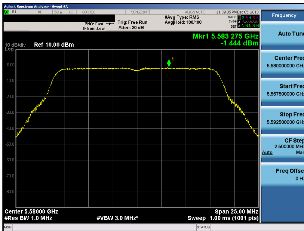
Plot 6-83. Peak Power Spectral Density Plot (802.11a (UNII Band 2C) – Ch. 116)
