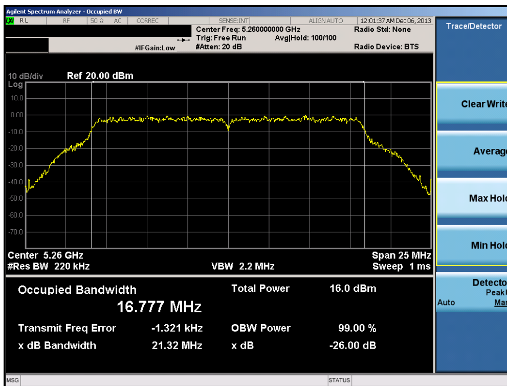
Plot 6-41. 26dB Bandwidth Plot (802.11a (UNII Band 2A) – Ch. 52)
