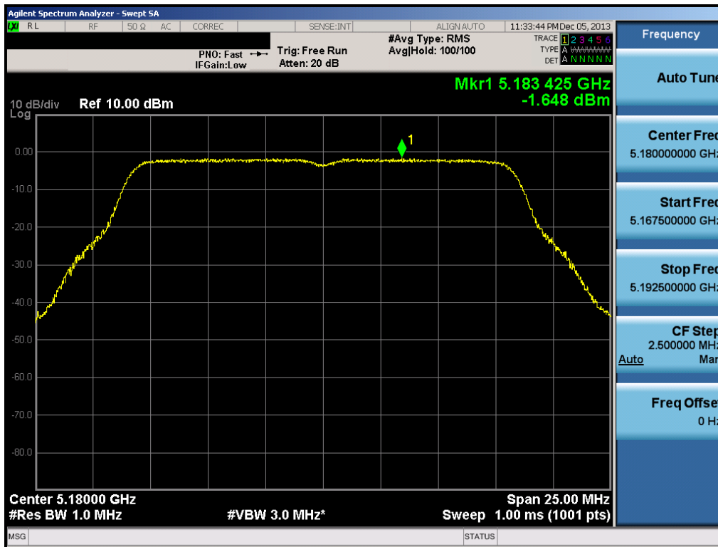
Plot 6-64. Peak Power Spectral Density Plot (802.11a (UNII Band 1) – Ch. 36)
