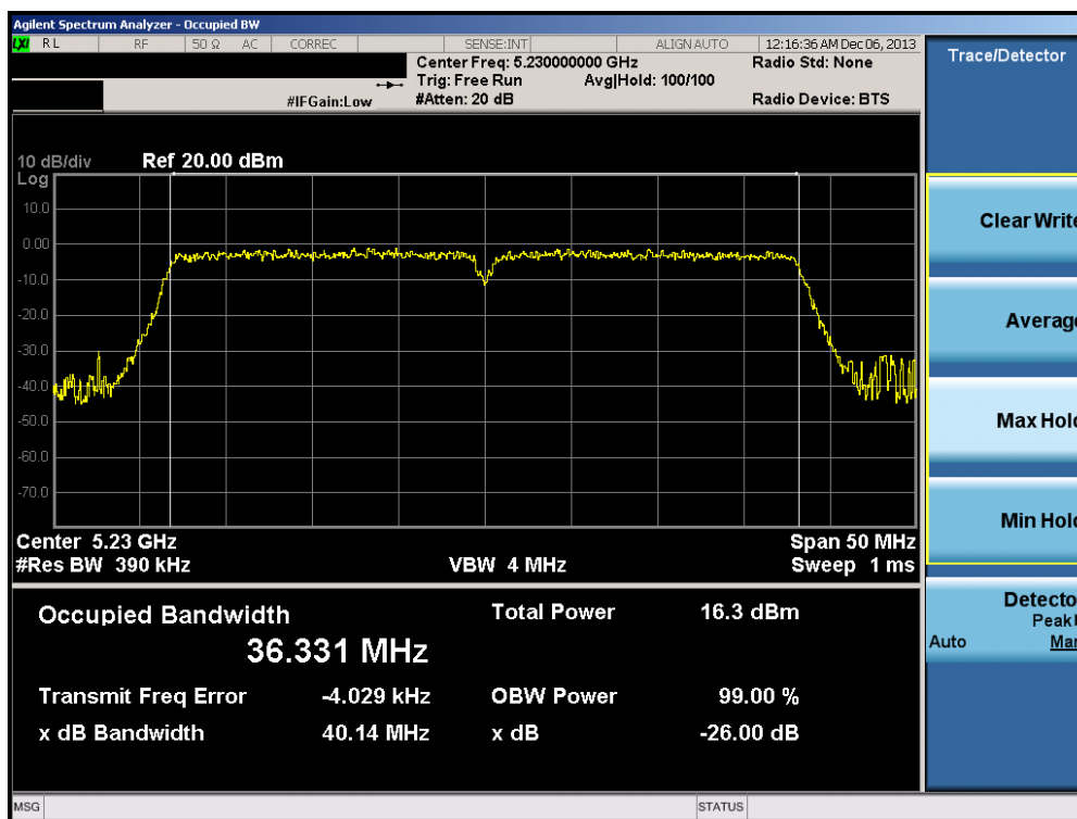
Plot 6-39. 26dB Bandwidth Plot (40MHz BW 802.11n (UNII Band 1) – Ch. 46)
