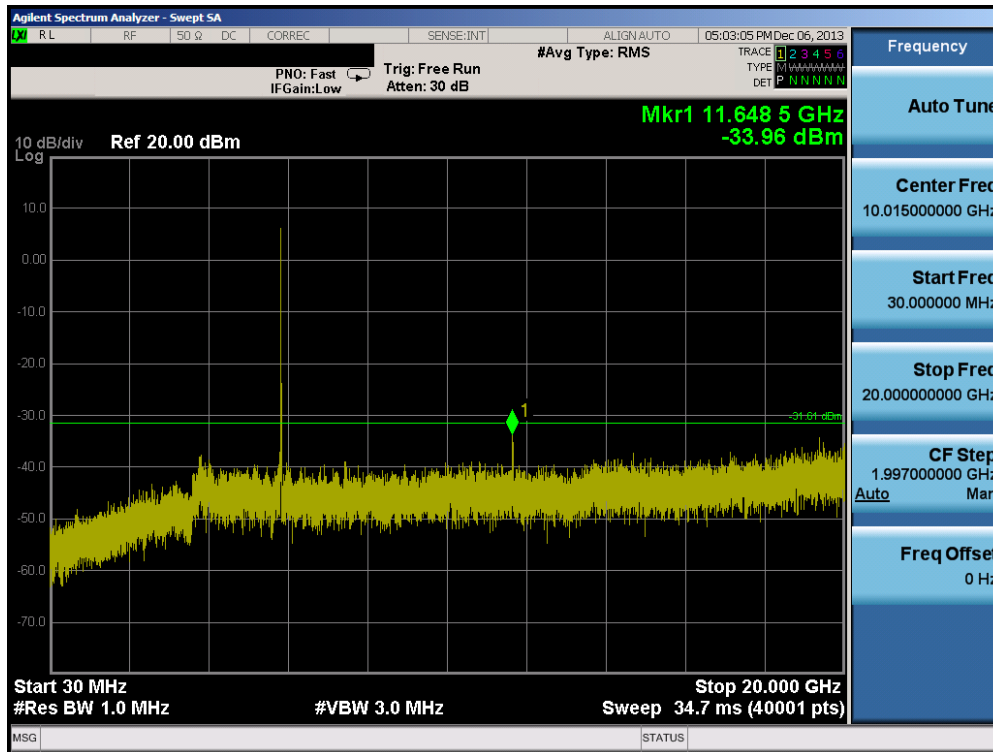
Plot 6-115. Conducted Spurious Plot (802.11a – Ch. 165)
