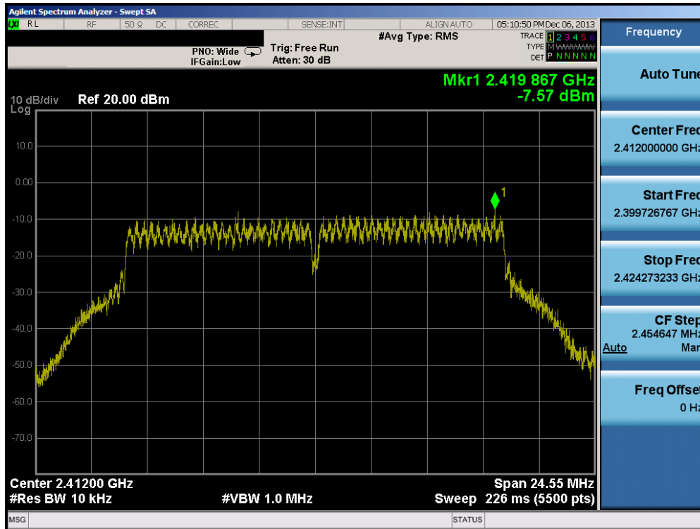
Plot 6-52. Power Spectral Density Plot (802.11g - Ch. 1)
