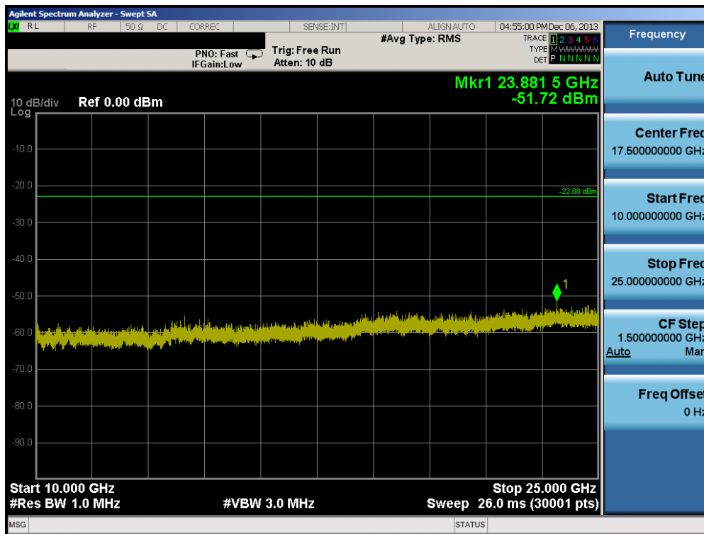
Plot 6-108. Conducted Spurious Plot (802.11g – Ch. 6)
