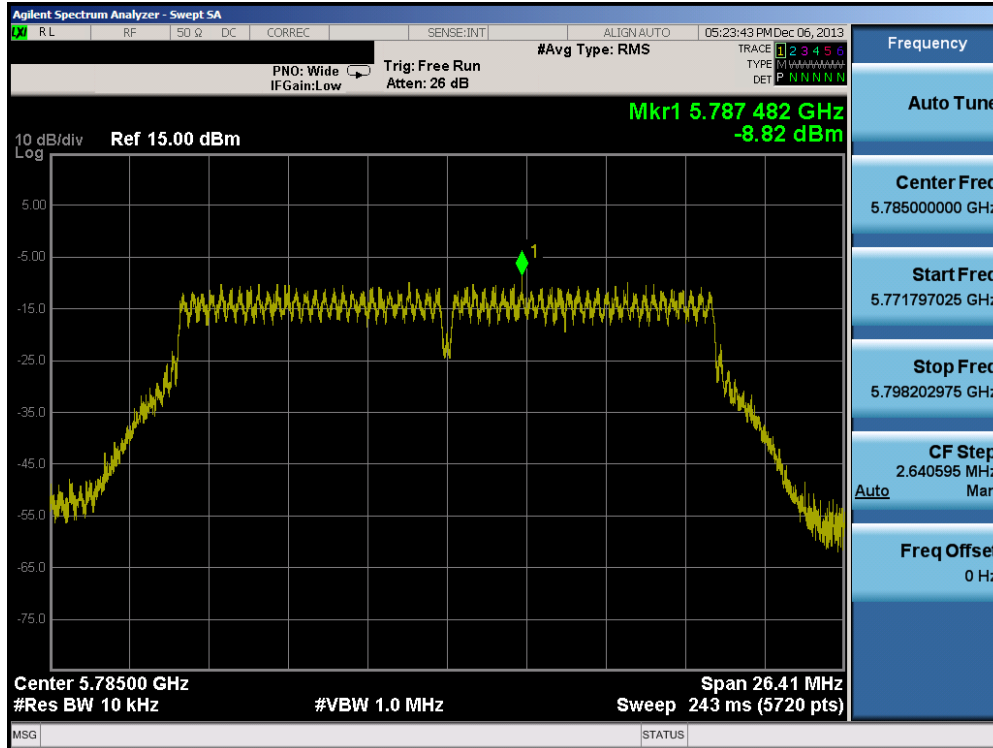
Plot 6-62. Power Spectral Density Plot (20MHz BW 802.11n (5.8GHz) – Ch. 157)
