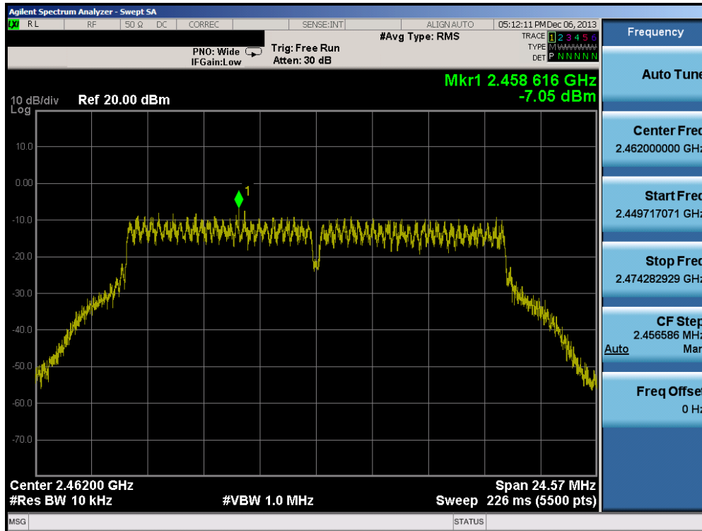
Plot 6-54. Power Spectral Density Plot (802.11g – Ch. 11)
