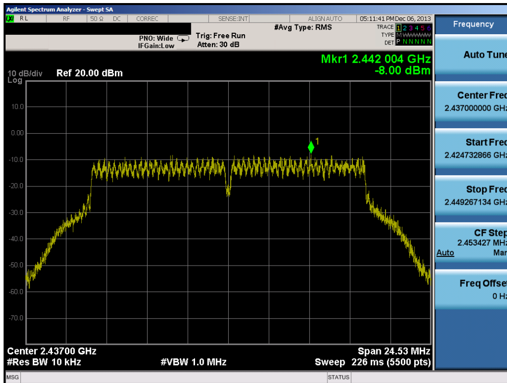
Plot 6-53. Power Spectral Density Plot (802.11g - Ch. 6)
