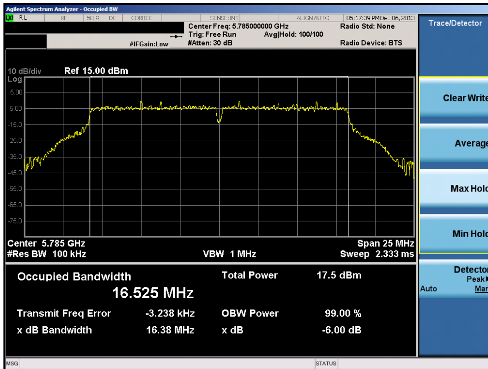
Plot 6-26. 6dB Bandwidth Plot (802.11a – Ch. 157)
