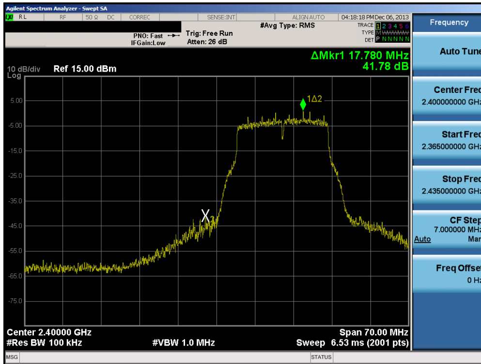
Plot 6-69. Band Edge Plot (802.11g- Ch. 1)
