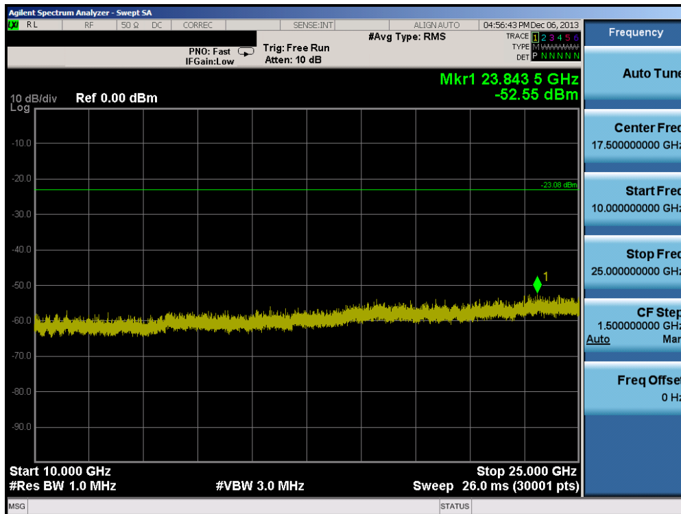
Plot 6-110. Conducted Spurious Plot (802.11g – Ch. 11)
