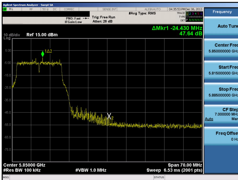
Plot 6-74. Band Edge Plot (802.11a – Ch. 165)
