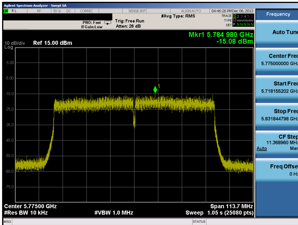
Plot 6-51. Power Spectral Density Plot (80MHz BW 802.11ac (5.8GHz) – Ch. 155)
