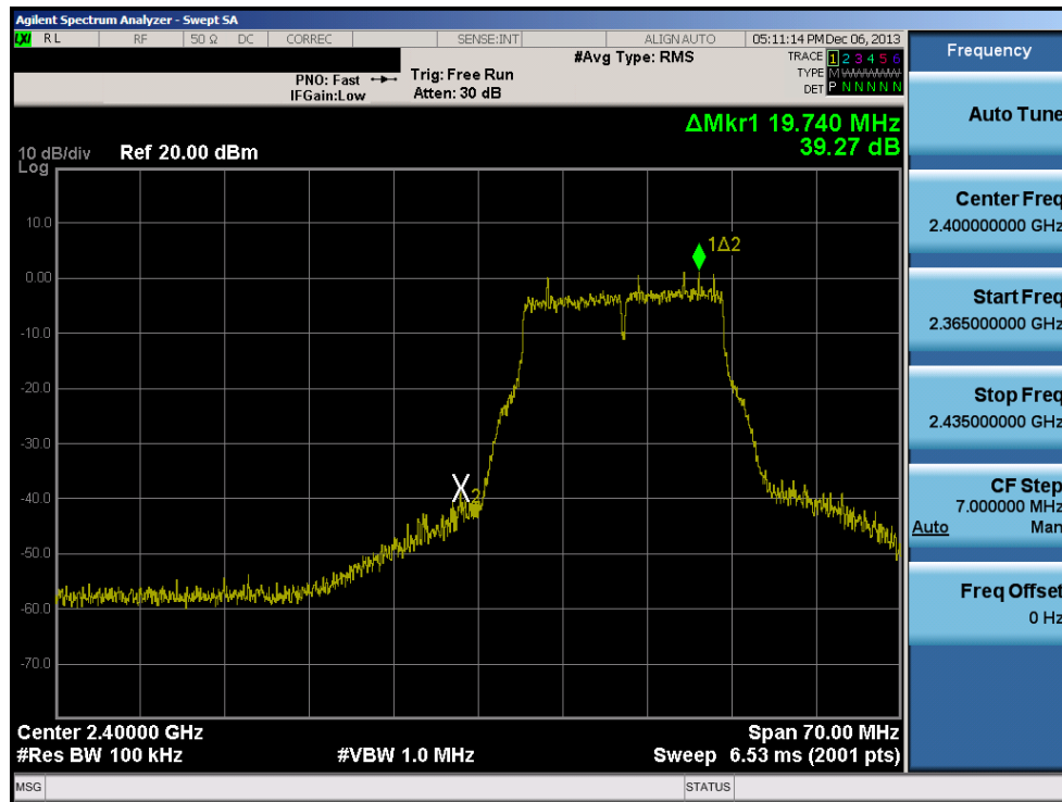
Plot 6-81. Band Edge Plot (802.11g– Ch. 1)
