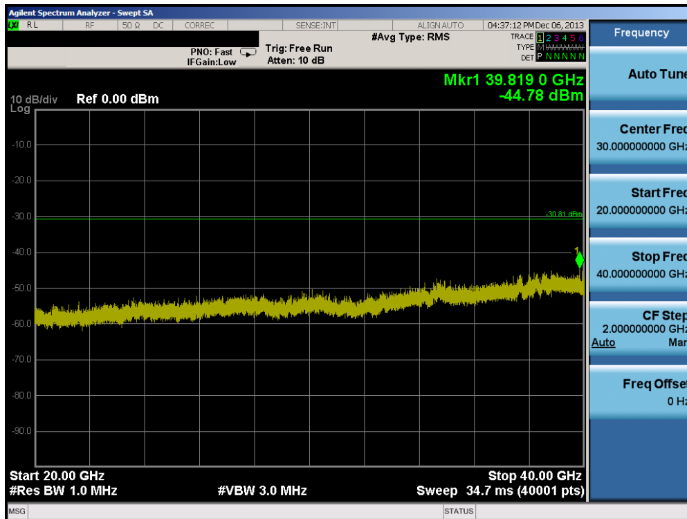
Plot 6-104. Conducted Spurious Plot (802.11a – Ch. 165)
