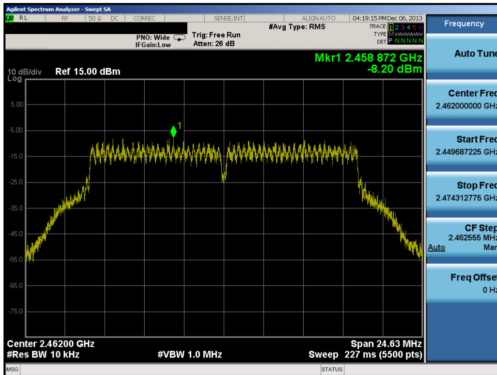
Plot 6-39. Power Spectral Density Plot (802.11g - Ch. 11)
