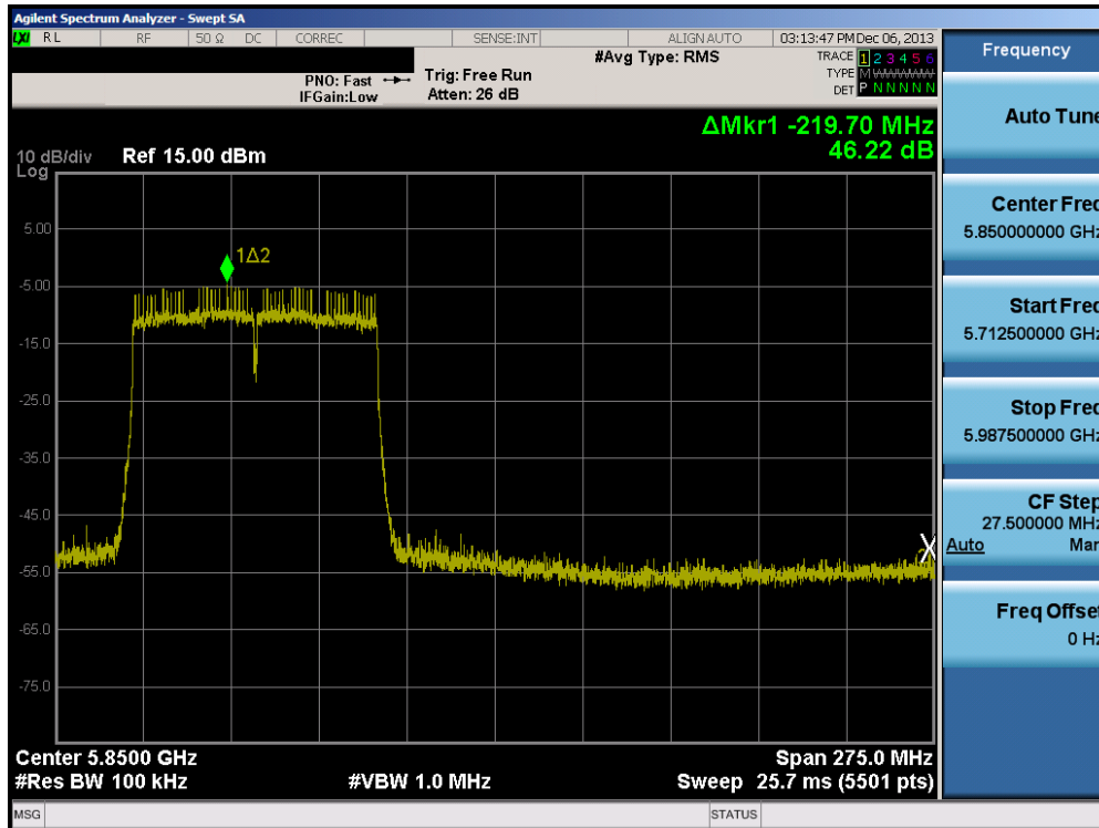
Plot 6-92. Band Edge Plot (80MHz BW 802.11ac (5.8GHz) – Ch. 155)
