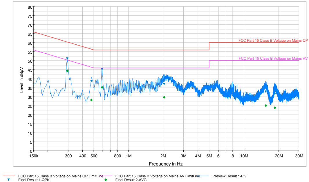
Plot 6-129. Line Conducted Plot with 802.11b (L1)
