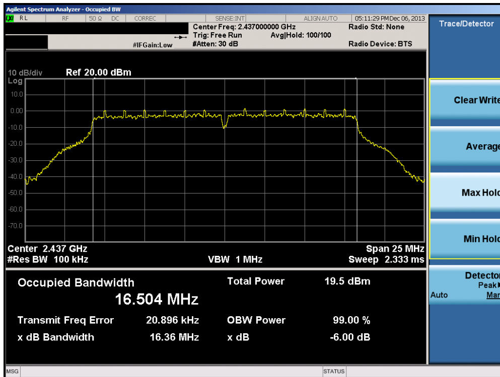
Plot 6-20. 6dB Bandwidth Plot (802.11g – Ch. 6)
