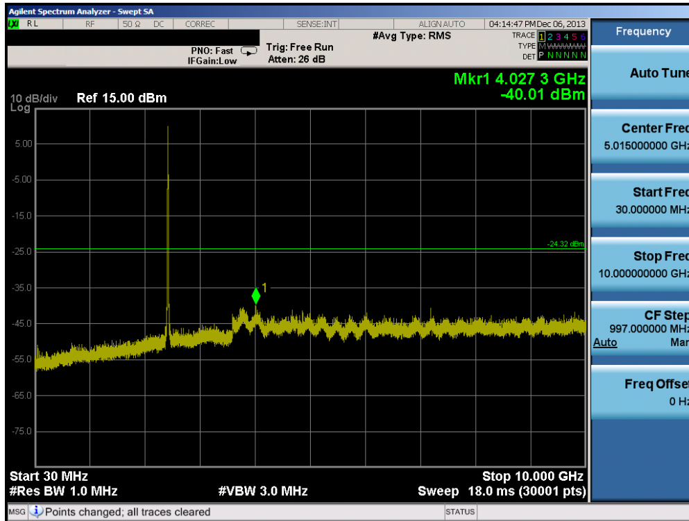
Plot 6-95. Conducted Spurious Plot (802.11b – Ch. 6)
