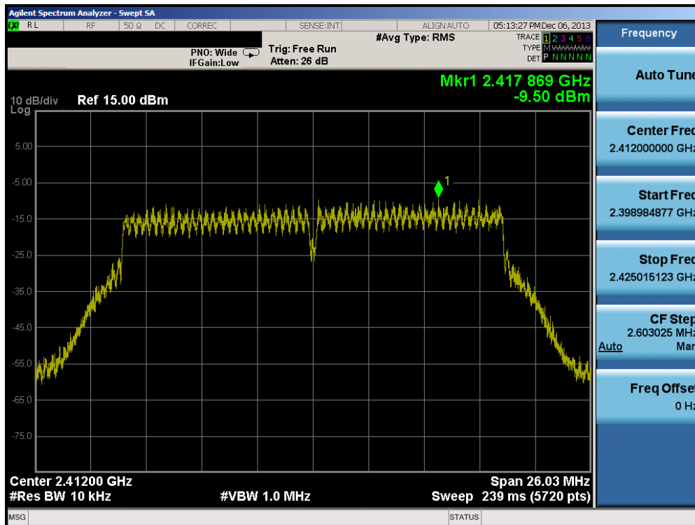
Plot 6-55. Power Spectral Density Plot (802.11n (2.4GHz) – Ch. 1)
