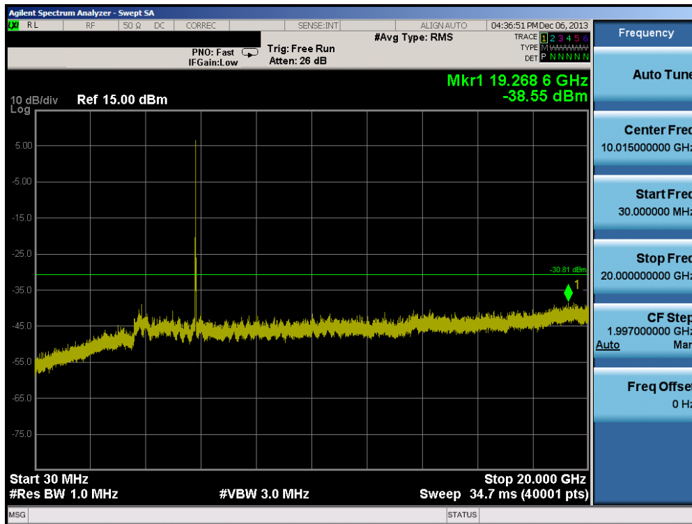
Plot 6-103. Conducted Spurious Plot (802.11a – Ch. 165)
