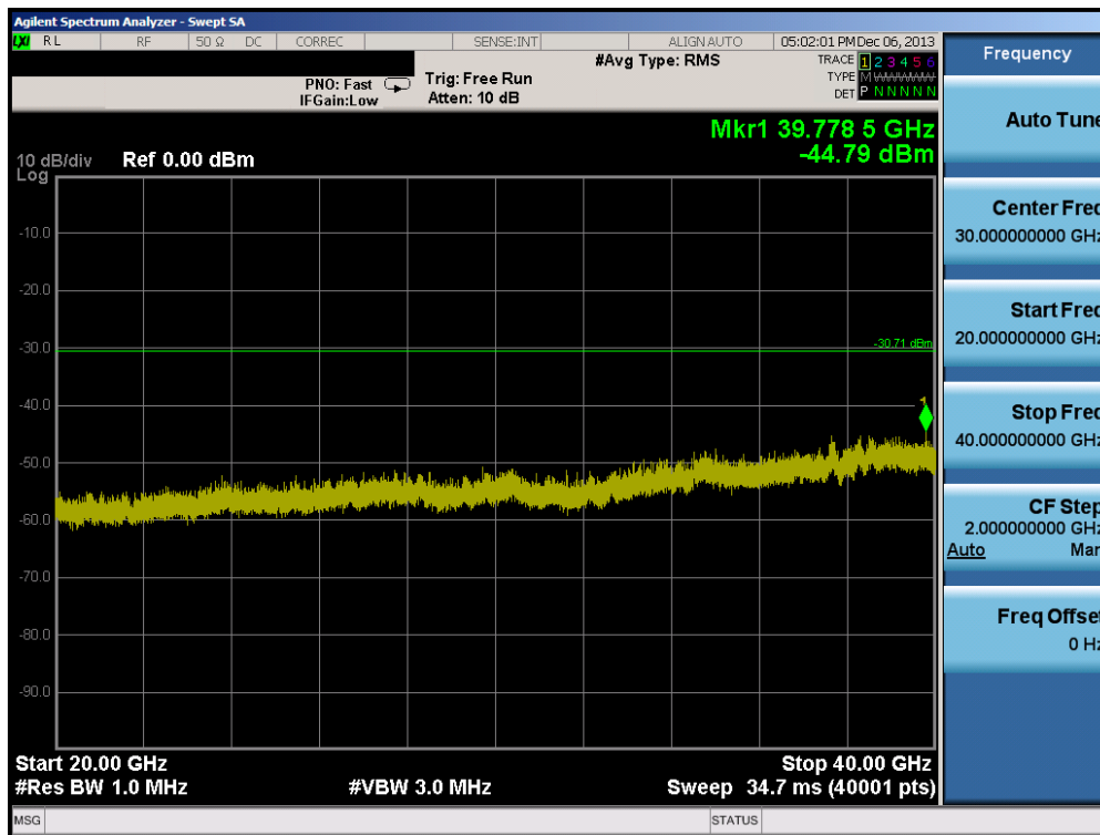
Plot 6-114. Conducted Spurious Plot (802.11a – Ch. 157)
