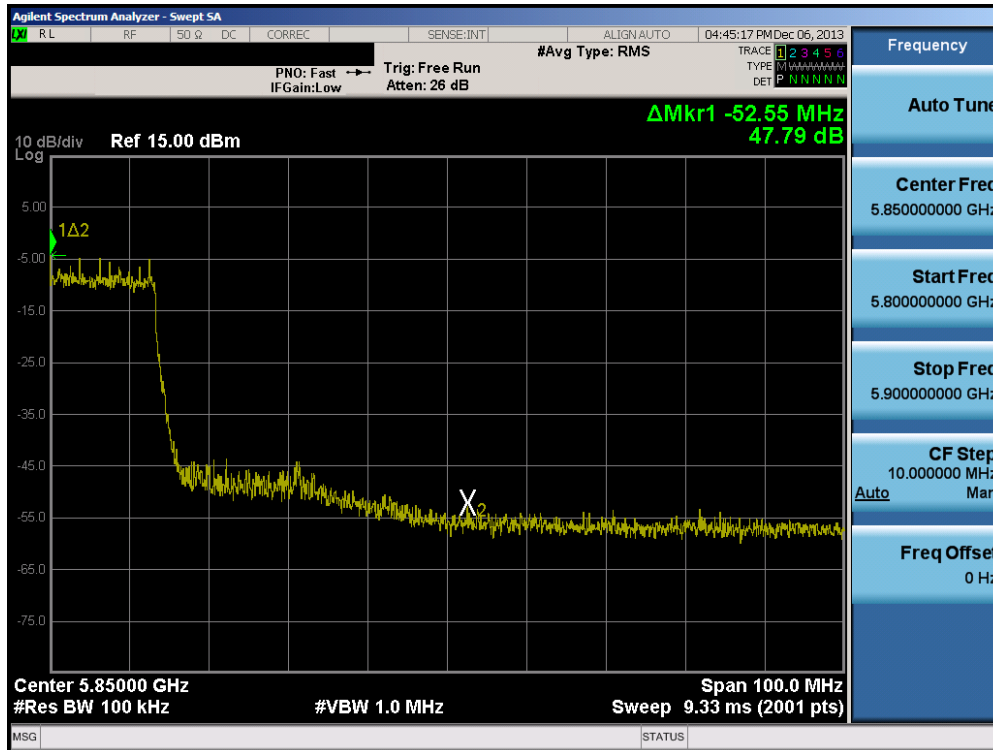
Plot 6-78. Band Edge Plot (40MHz BW 802.11n (5.8GHz) – Ch. 159)
