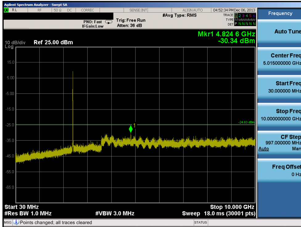
Plot 6-105. Conducted Spurious Plot (802.11g – Ch. 1)
