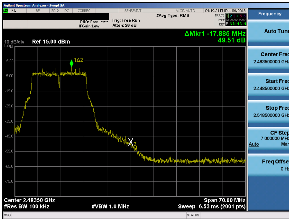
Plot 6-70. Band Edge Plot (802.11g - Ch. 11)
