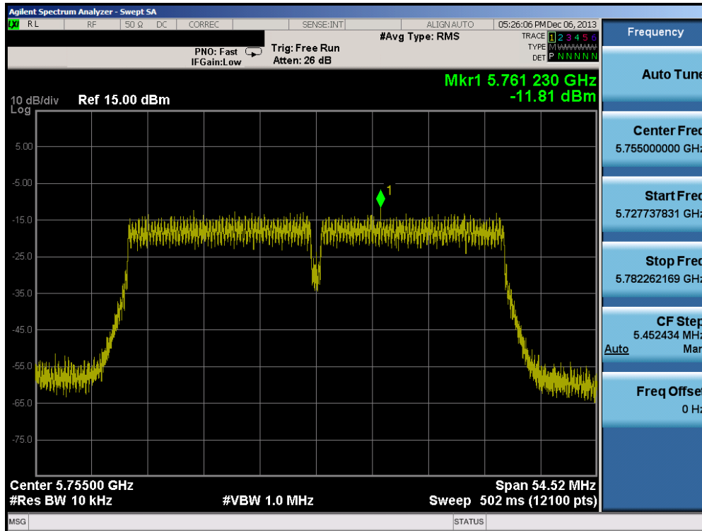
Plot 6-64. Power Spectral Density Plot (40MHz BW 802.11n (5.8GHz) – Ch. 151)
