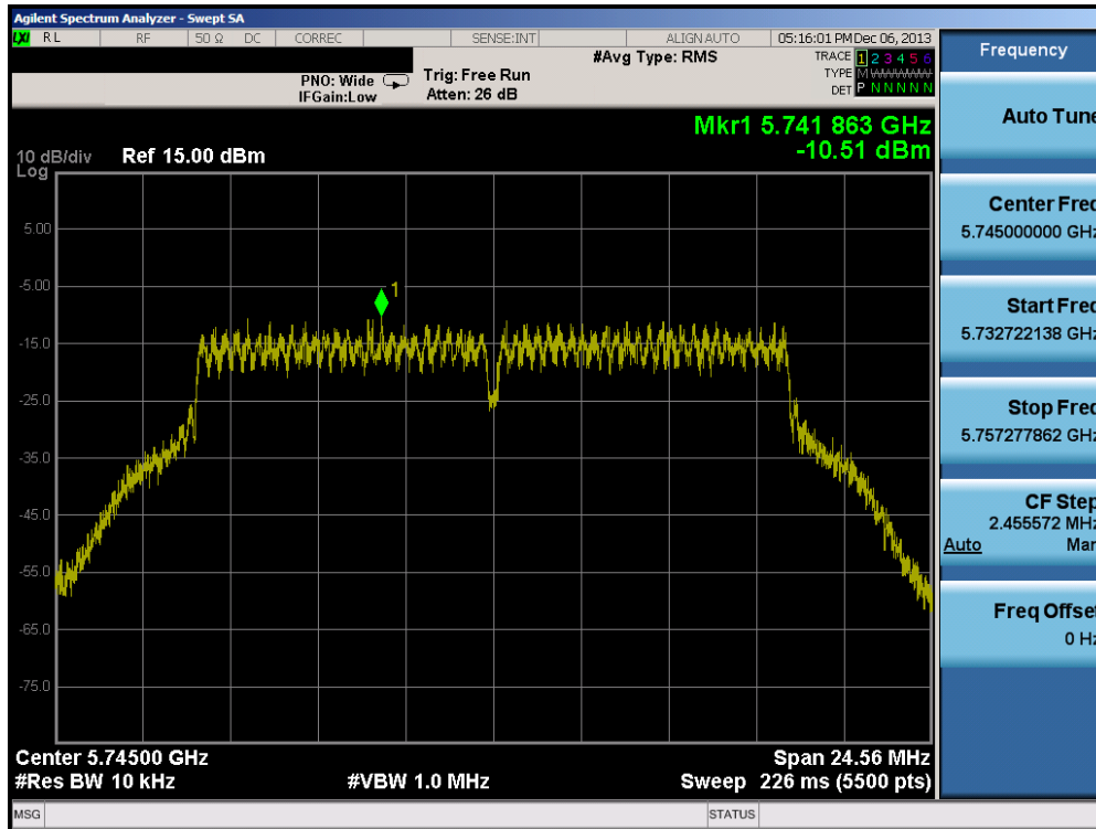
Plot 6-58. Power Spectral Density Plot (802.11a – Ch. 149)
