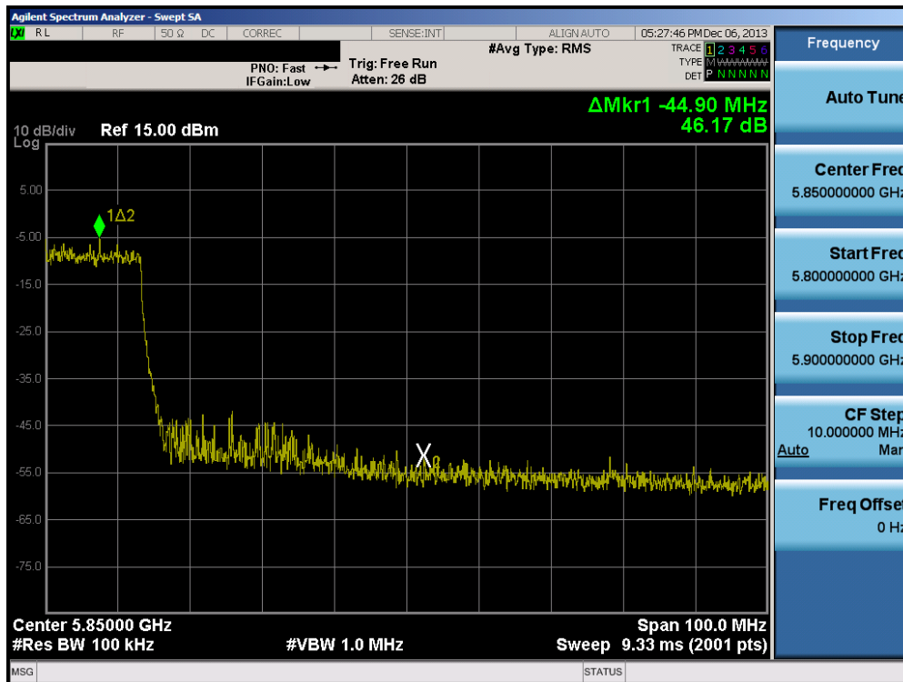
Plot 6-90. Band Edge Plot (40MHz BW 802.11n (5.8GHz) – Ch. 159)
