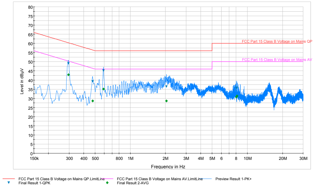
Plot 6-131. Line Conducted Plot with 802.11a (L1)
