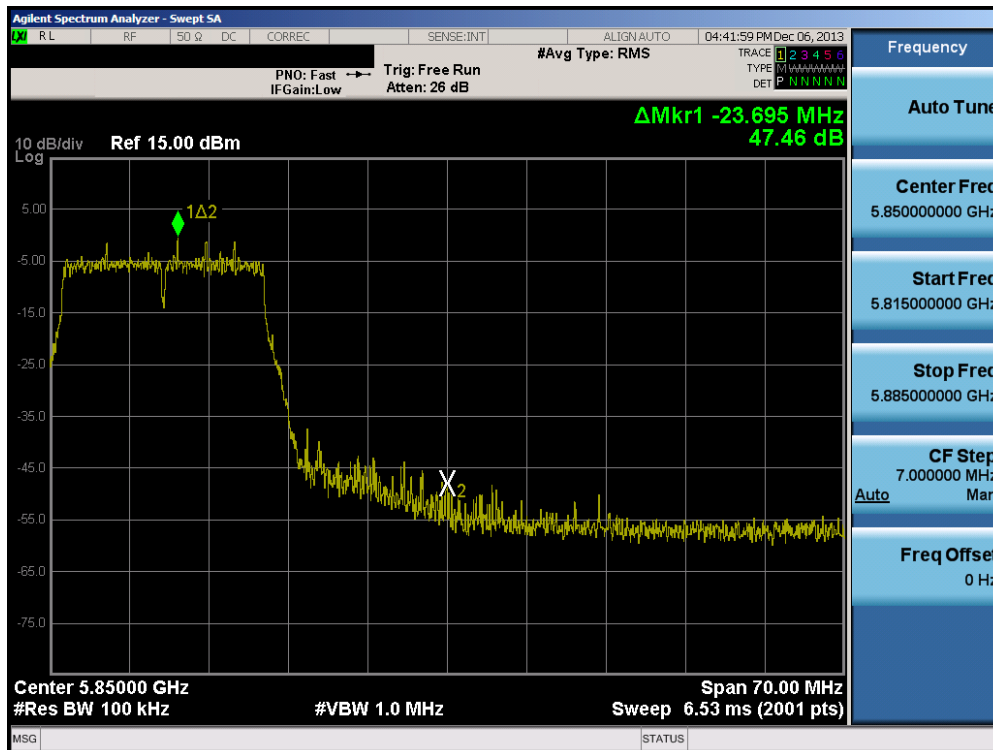
Plot 6-76. Band Edge Plot (20MHz BW 802.11n (5.8GHz) – Ch. 165)
