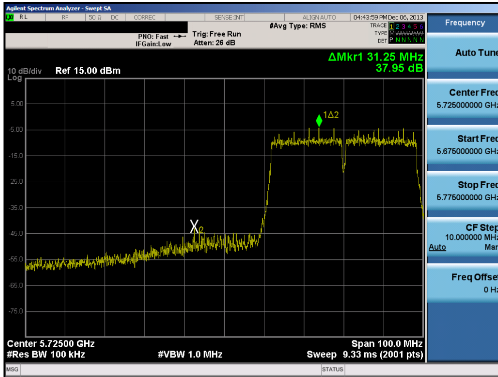
Plot 6-77. Band Edge Plot (40MHz BW 802.11n (5.8GHz) – Ch. 151)
