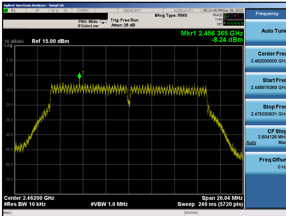
Plot 6-57. Power Spectral Density Plot (802.11n (2.4GHz) – Ch. 11)
