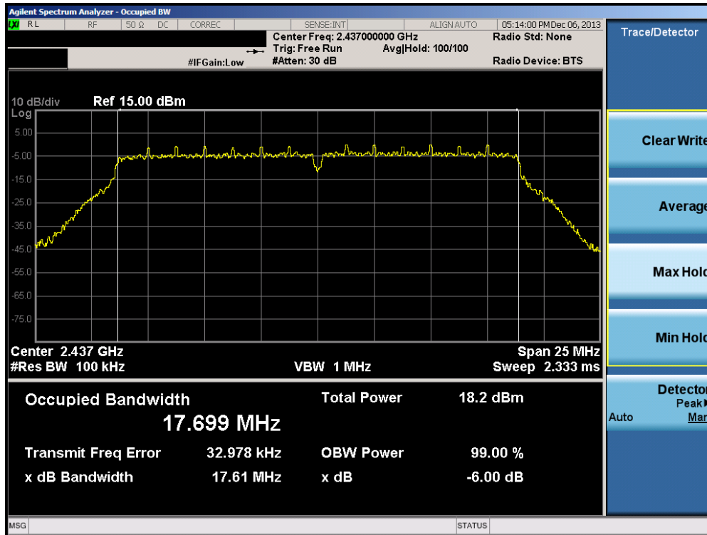
Plot 6-23. 6dB Bandwidth Plot (802.11n (2.4GHz) – Ch. 6)
