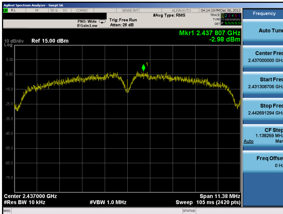
Plot 6-35. Power Spectral Density Plot (802.11g - Ch. 6)
