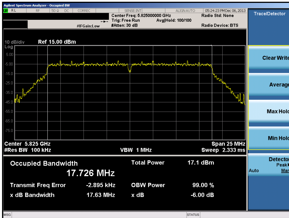
Plot 6-30. 6dB Bandwidth Plot (20MHz BW 802.11n (5.8GHz) – Ch. 165)
