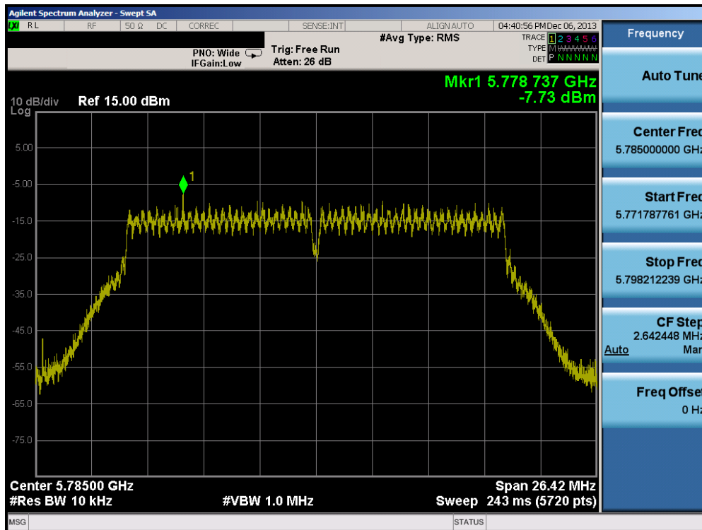
Plot 6-47. Power Spectral Density Plot (20MHz BW 802.11n (5.8GHz) – Ch. 157)
