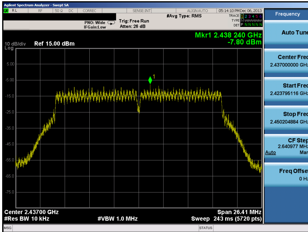
Plot 6-56. Power Spectral Density Plot (802.11n (2.4GHz) – Ch. 6)
