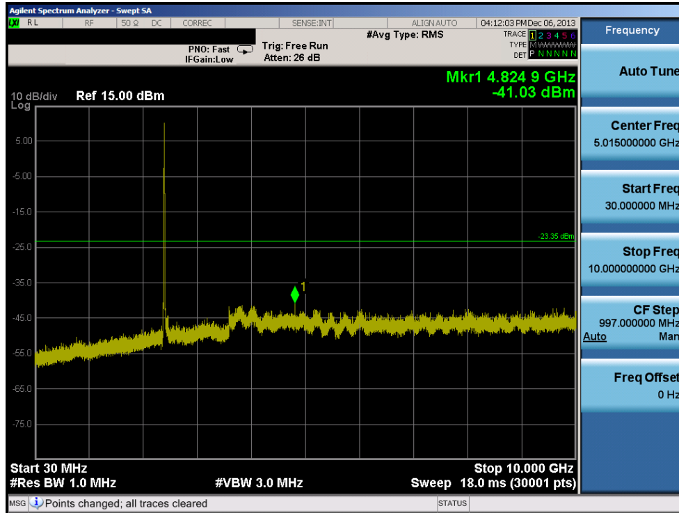
Plot 6-93. Conducted Spurious Plot (802.11b – Ch. 1)
