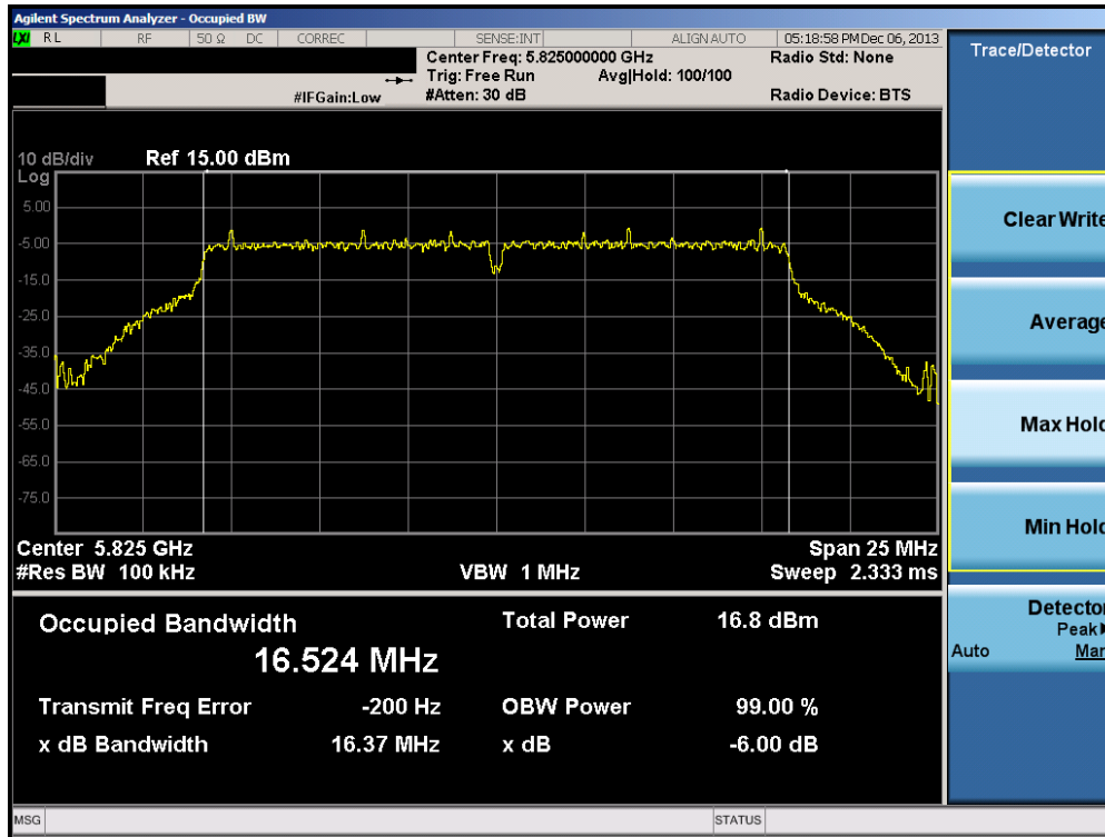
Plot 6-27. 6dB Bandwidth Plot (802.11a – Ch. 165)
