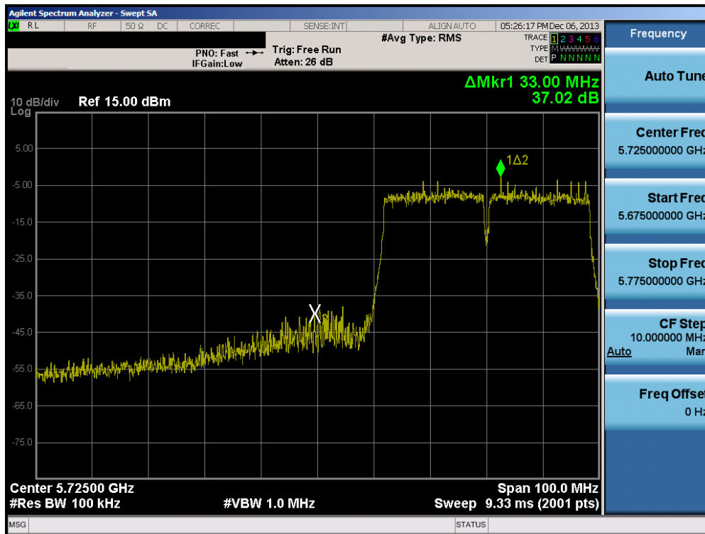
Plot 6-89. Band Edge Plot (40MHz BW 802.11n (5.8GHz) – Ch. 151)
