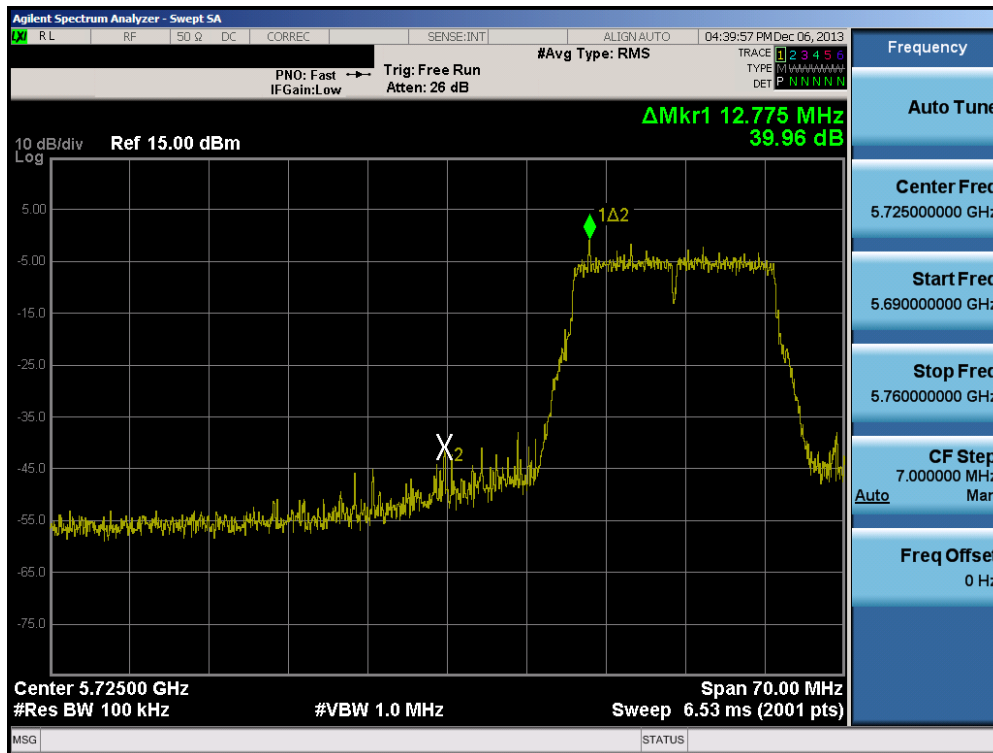
Plot 6-75. Band Edge Plot (20MHz BW 802.11n (5.8GHz) – Ch. 149)
