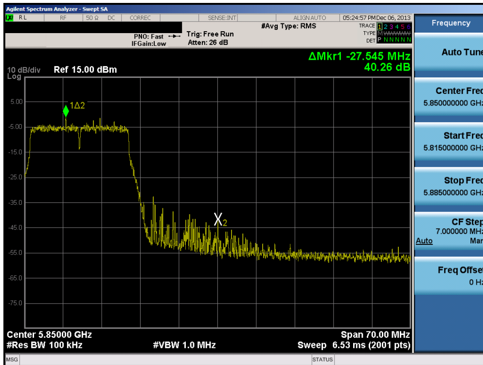
Plot 6-88. Band Edge Plot (20MHz BW 802.11n (5.8GHz) – Ch. 165)
