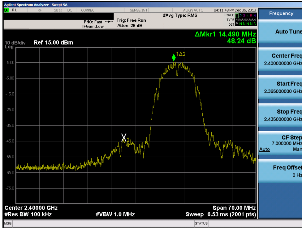
Plot 6-67. Band Edge Plot (802.11b– Ch. 1)
