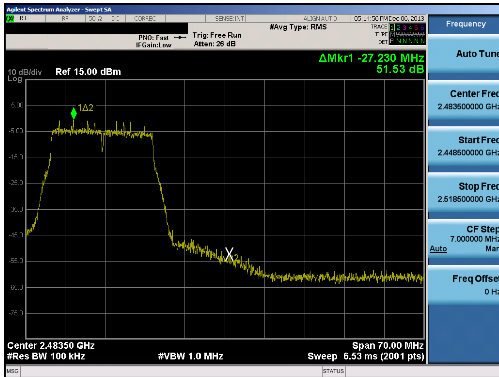
Plot 6-84. Band Edge Plot (802.11n (2.4GHz) – Ch. 11)
