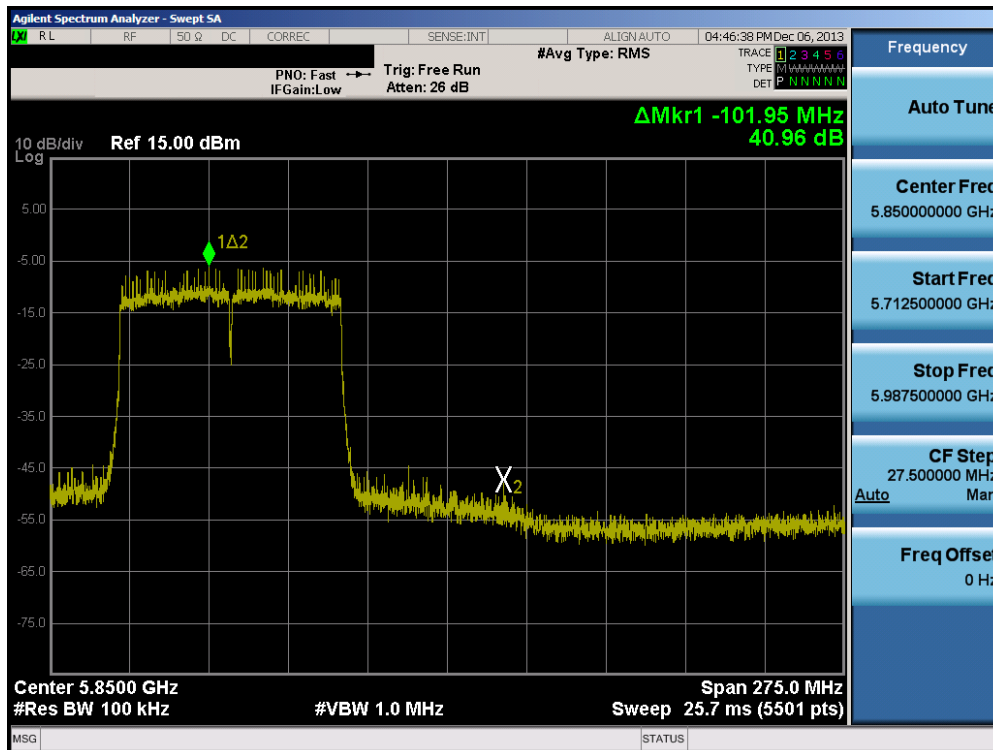
Plot 6-80. Band Edge Plot (80MHz BW 802.11ac (5.8GHz) – Ch. 155)
