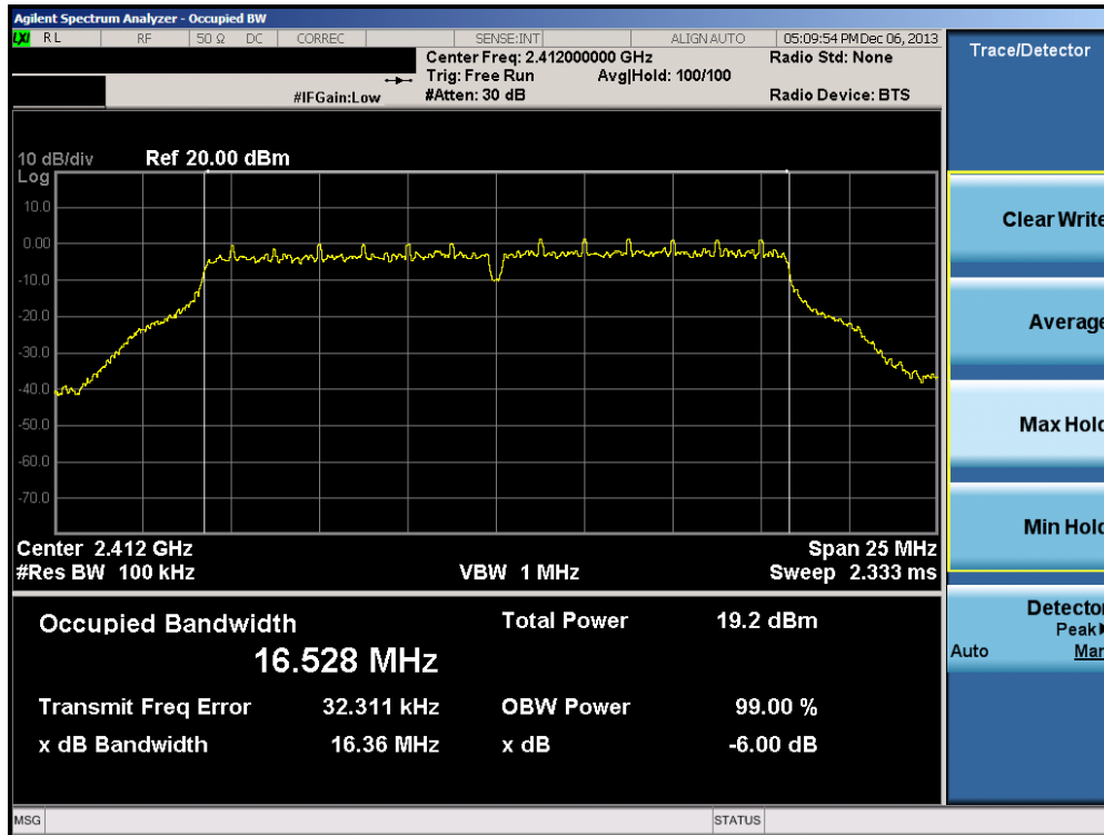
Plot 6-19. 6dB Bandwidth Plot (802.11g – Ch. 1)
