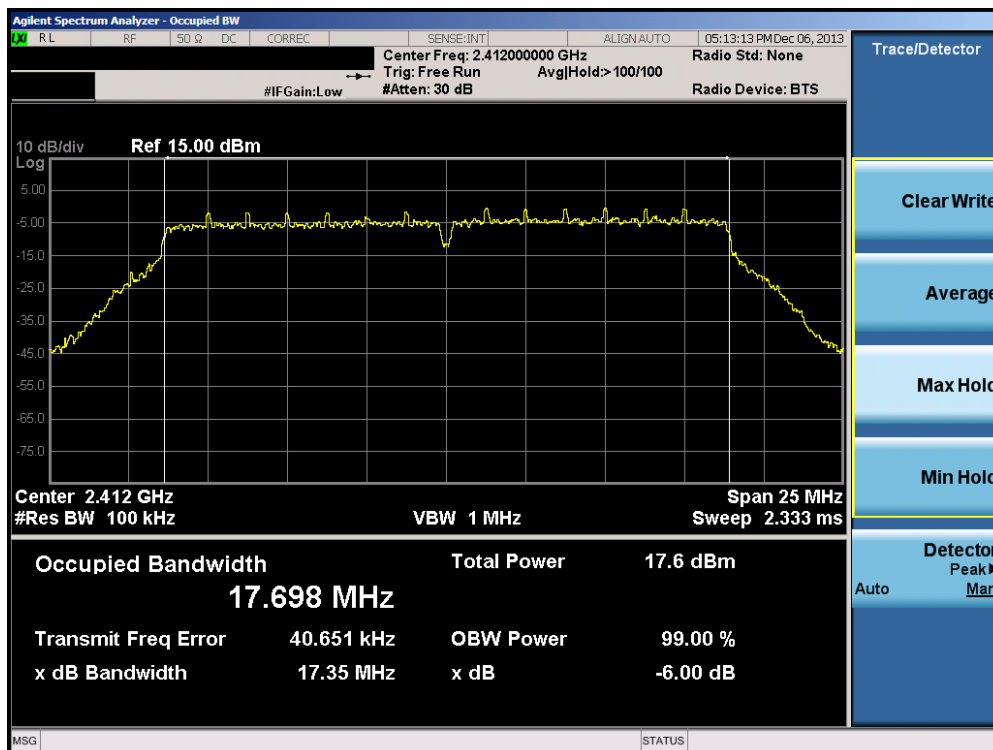
Plot 6-22. 6dB Bandwidth Plot (802.11n (2.4GHz) – Ch. 1)
