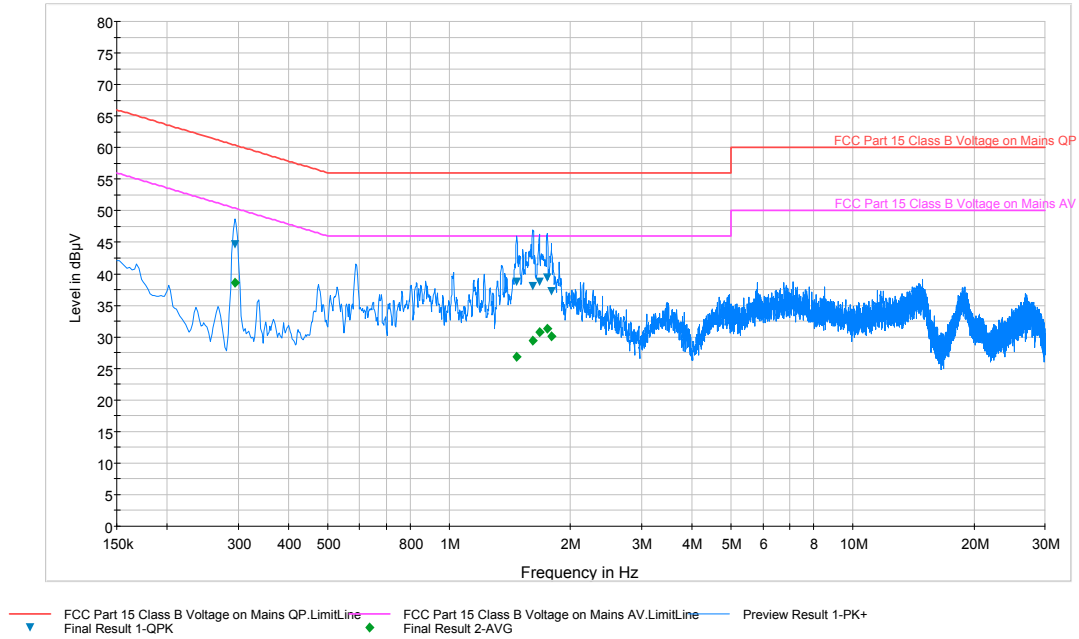
Plot 6-132. Line Conducted Plot with 802.11a (N)
