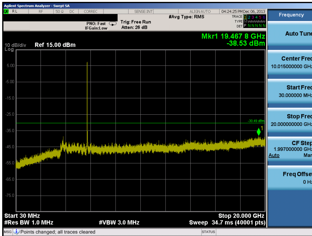
Plot 6-99. Conducted Spurious Plot (802.11a – Ch. 149)
