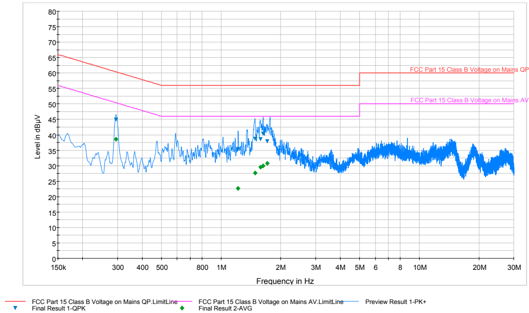
Plot 6-130. Line Conducted Plot with 802.11b (N)
