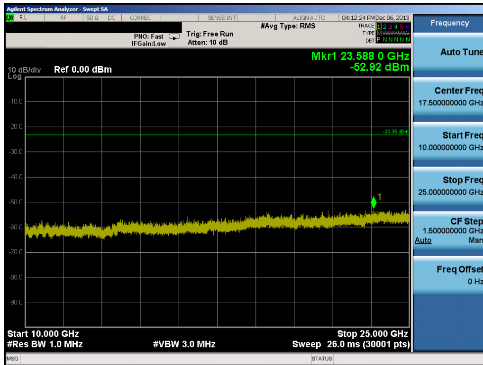
Plot 6-94. Conducted Spurious Plot (802.11b – Ch. 1)
