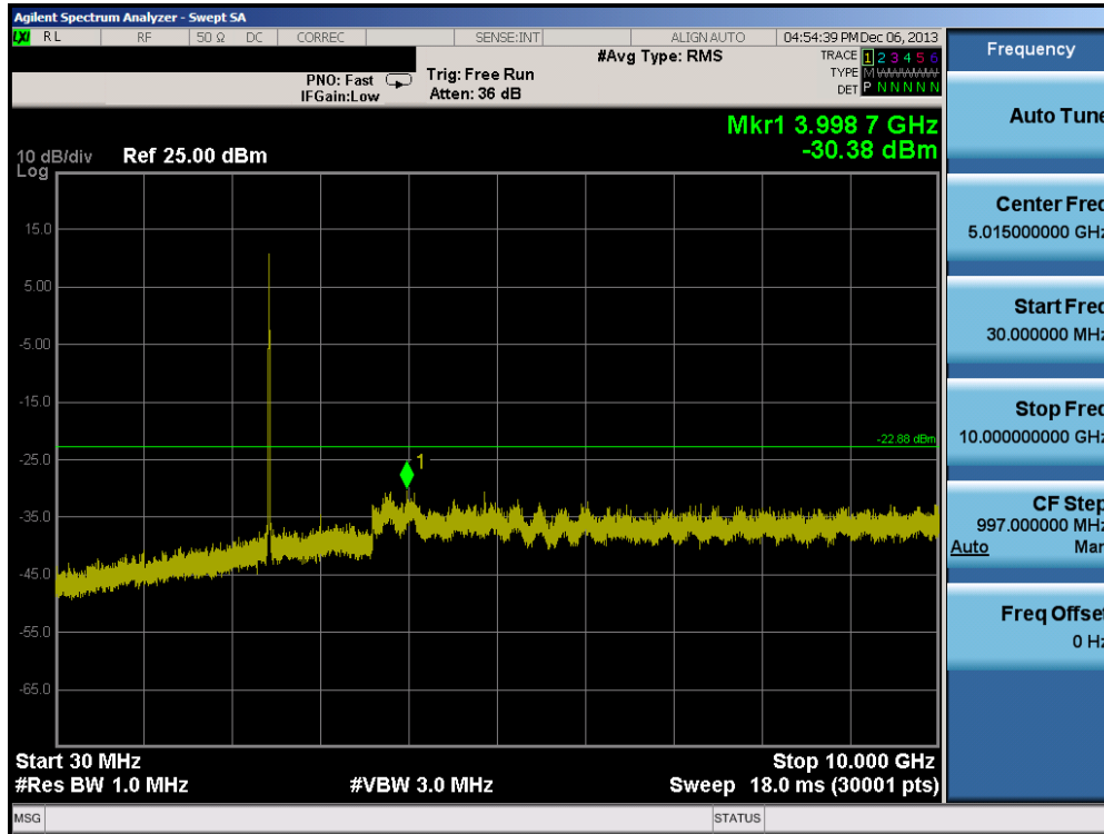
Plot 6-107. Conducted Spurious Plot (802.11g – Ch. 6)
