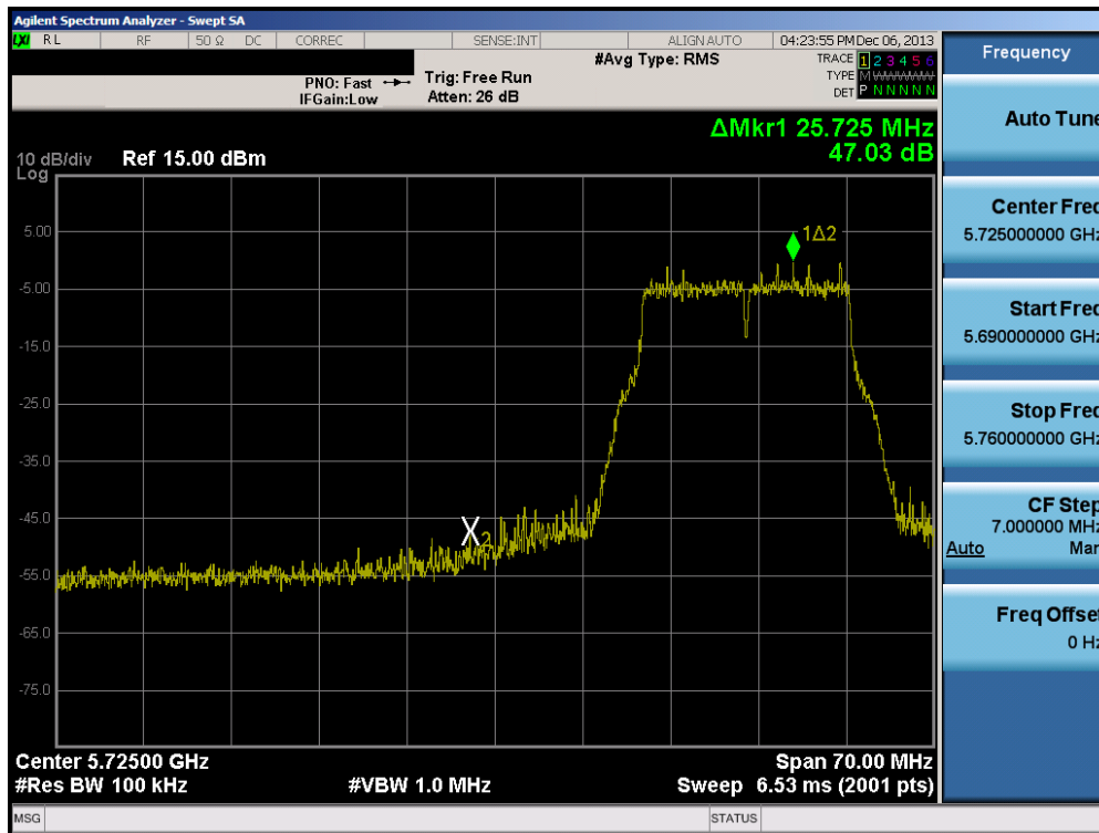
Plot 6-73. Band Edge Plot (802.11a – Ch. 149)
