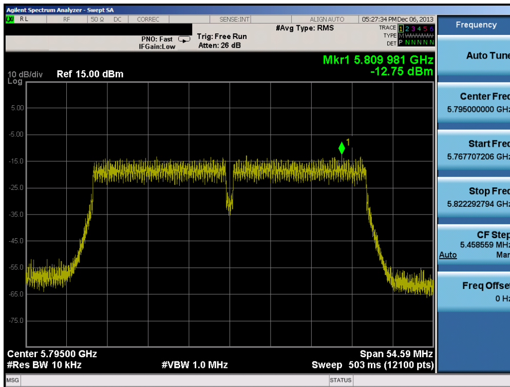
Plot 6-65. Power Spectral Density Plot (40MHz BW 802.11n (5.8GHz) – Ch. 159)
