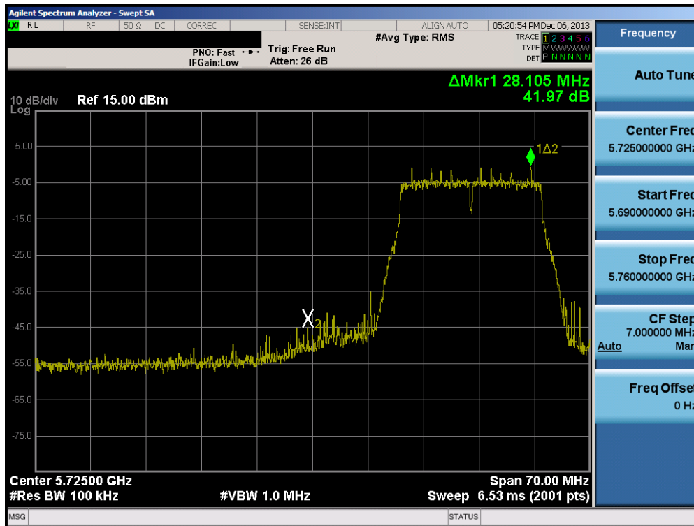
Plot 6-87. Band Edge Plot (20MHz BW 802.11n (5.8GHz) – Ch. 149)
