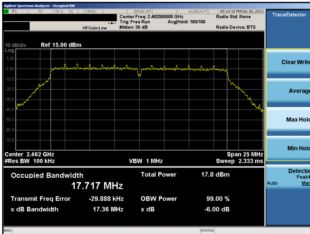
Plot 6-24. 6dB Bandwidth Plot (802.11n (2.4GHz) – Ch. 11)
