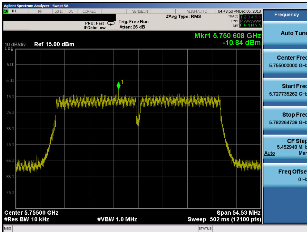
Plot 6-49. Power Spectral Density Plot (40MHz BW 802.11n (5.8GHz) – Ch. 151)
