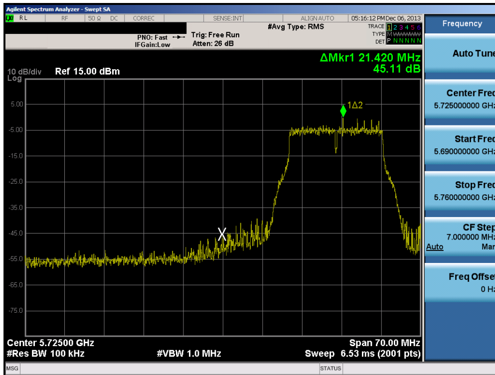
Plot 6-85. Band Edge Plot (802.11a – Ch. 149)
