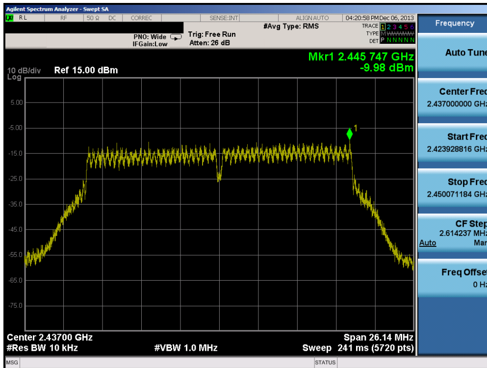
Plot 6-41. Power Spectral Density Plot (802.11n (2.4GHz) – Ch. 6)
