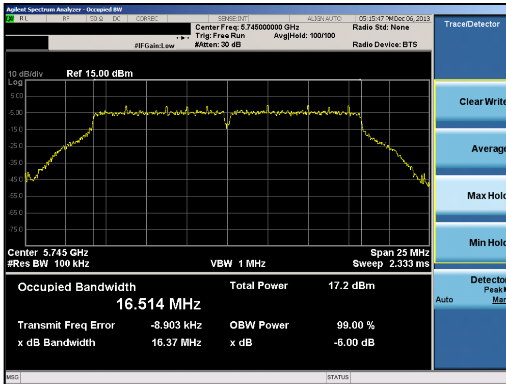
Plot 6-25. 6dB Bandwidth Plot (802.11a – Ch. 149)
