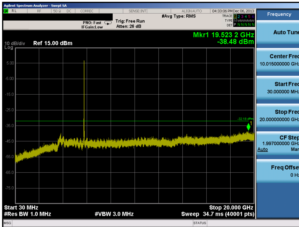
Plot 6-101. Conducted Spurious Plot (802.11a – Ch. 157)
