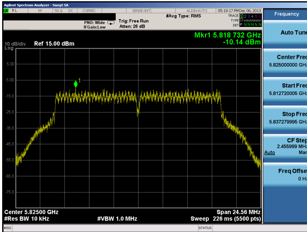
Plot 6-60. Power Spectral Density Plot (802.11a – Ch. 165)
