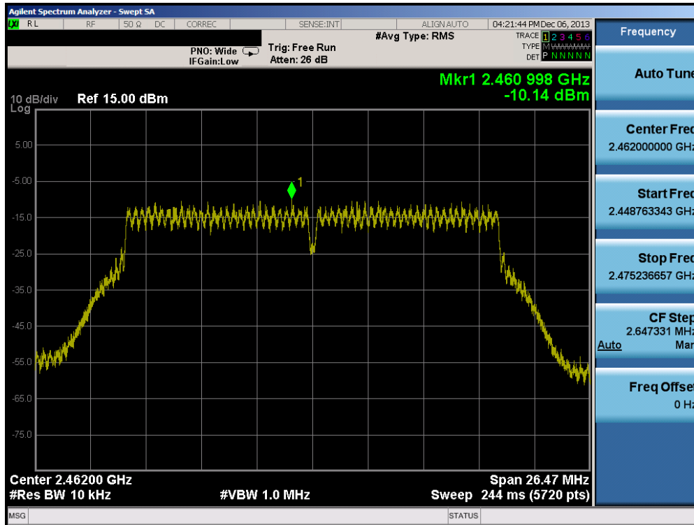
Plot 6-42. Power Spectral Density Plot (802.11n (2.4GHz) – Ch. 11)
