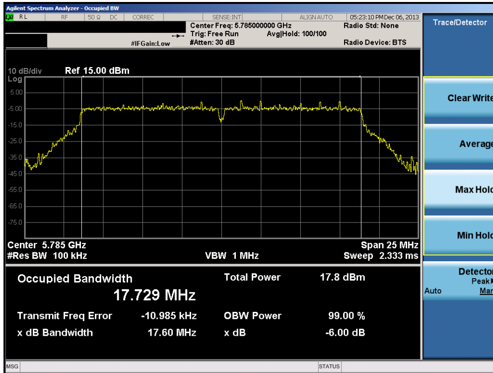
Plot 6-29. 6dB Bandwidth Plot (20MHz BW 802.11n (5.8GHz) – Ch. 157)
