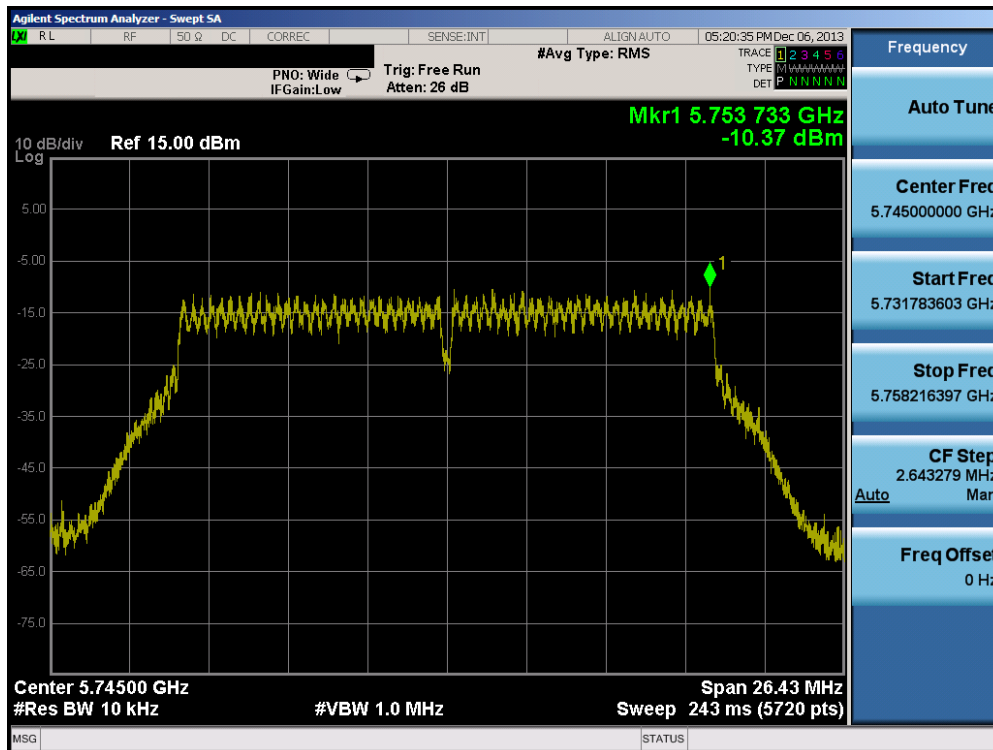
Plot 6-61. Power Spectral Density Plot (20MHz BW 802.11n (5.8GHz) – Ch. 149)
