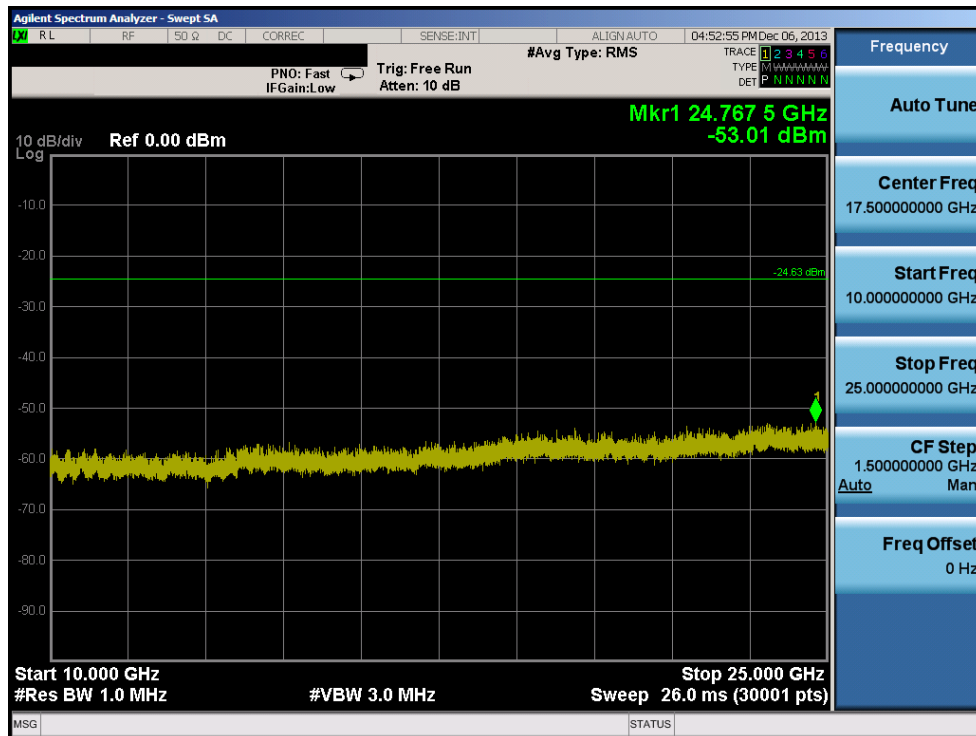
Plot 6-106. Conducted Spurious Plot (802.11g – Ch. 1)
