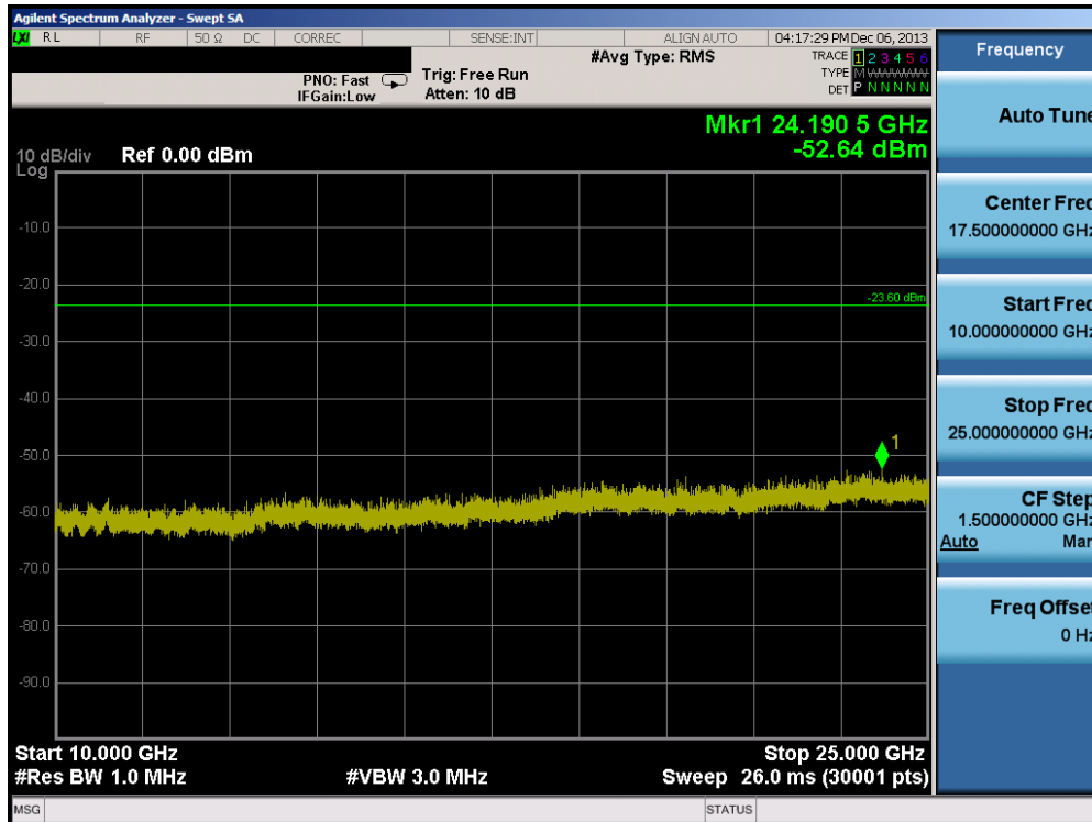
Plot 6-98. Conducted Spurious Plot (802.11b – Ch. 11)
