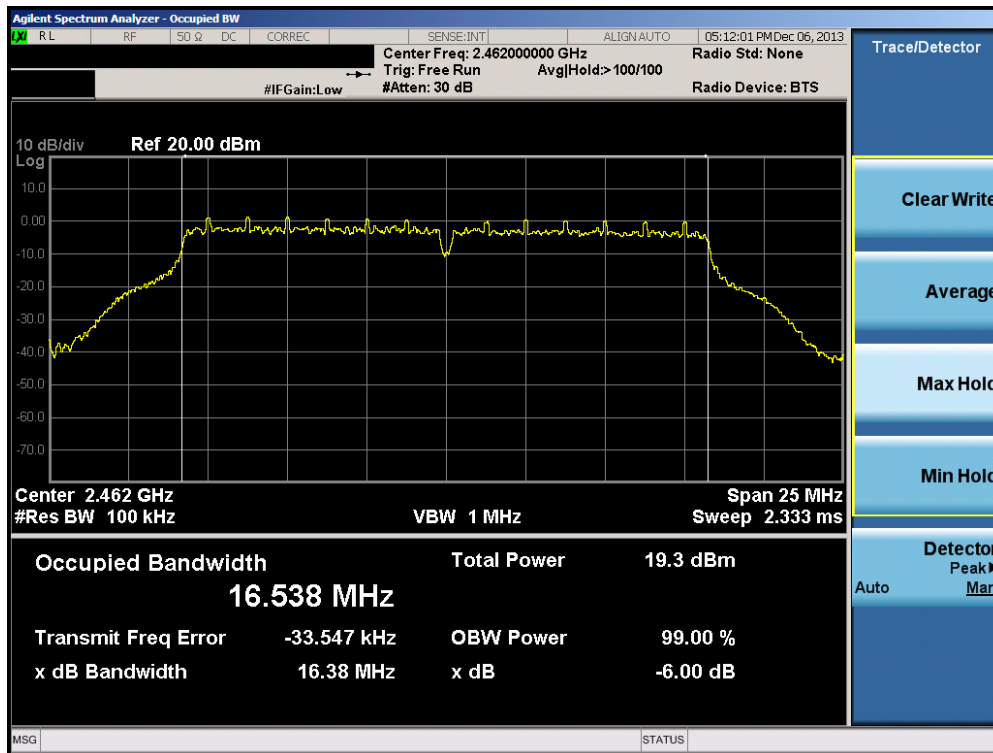
Plot 6-21. 6dB Bandwidth Plot (802.11g – Ch. 11)
