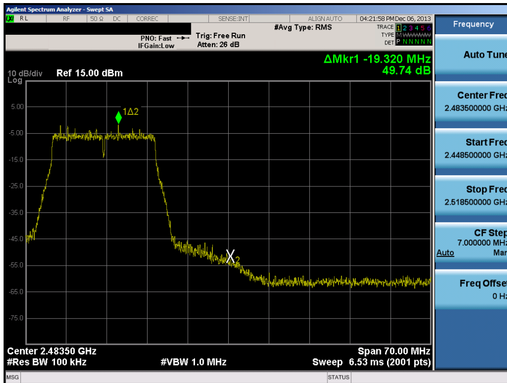
Plot 6-72. Band Edge Plot (802.11n (2.4GHz) – Ch. 11)
