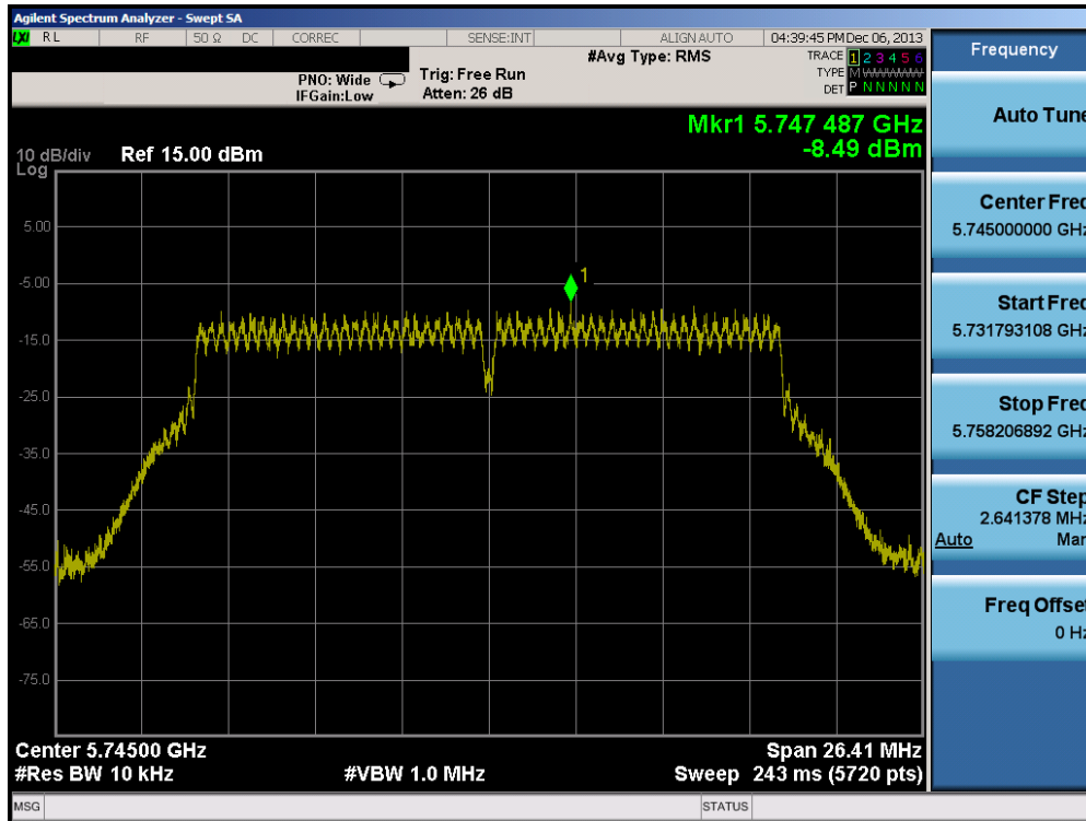
Plot 6-46. Power Spectral Density Plot (20MHz BW 802.11n (5.8GHz) – Ch. 149)
