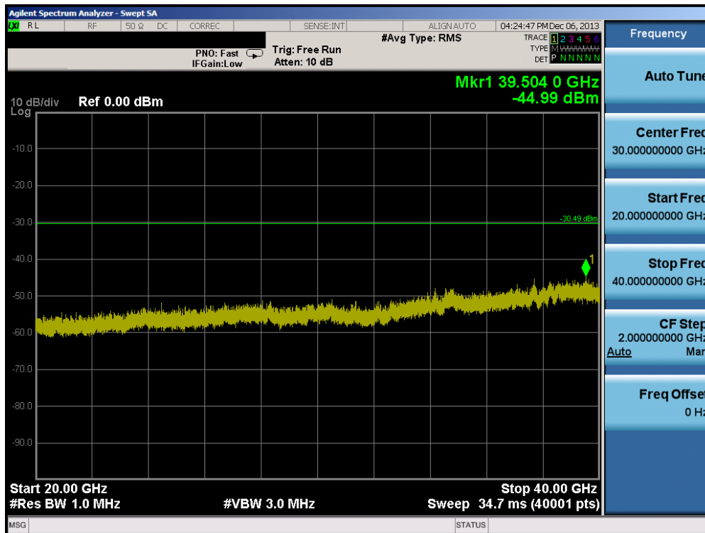
Plot 6-100. Conducted Spurious Plot (802.11a– Ch. 149)
