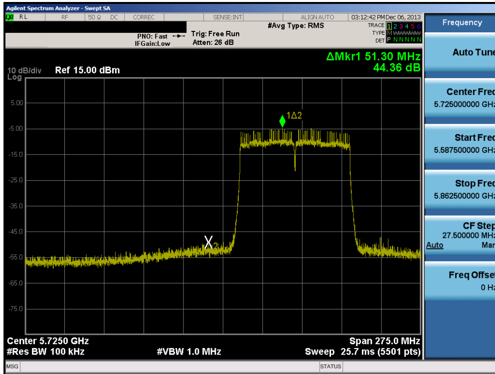
Plot 6-91. Band Edge Plot (80MHz BW 802.11ac (5.8GHz) – Ch. 155)
