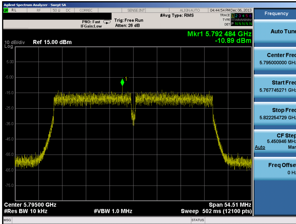
Plot 6-50. Power Spectral Density Plot (40MHz BW 802.11n (5.8GHz) – Ch. 159)
