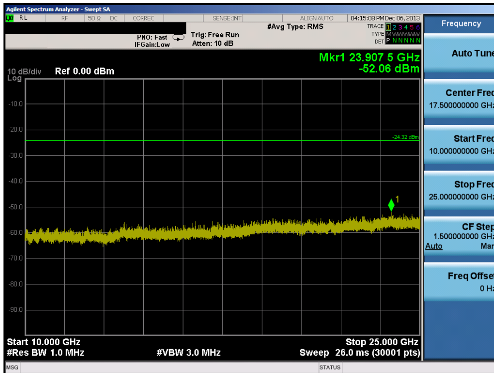
Plot 6-96. Conducted Spurious Plot (802.11b – Ch. 6)
