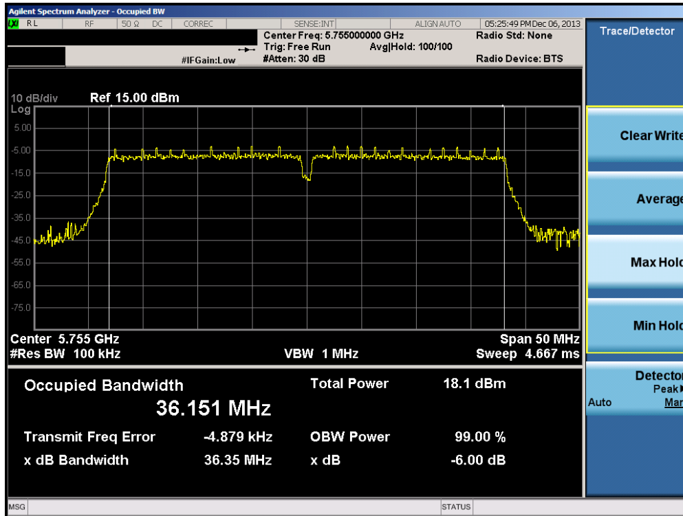
Plot 6-31. 6dB Bandwidth Plot (40MHz BW 802.11n (5.8GHz) – Ch. 151)
