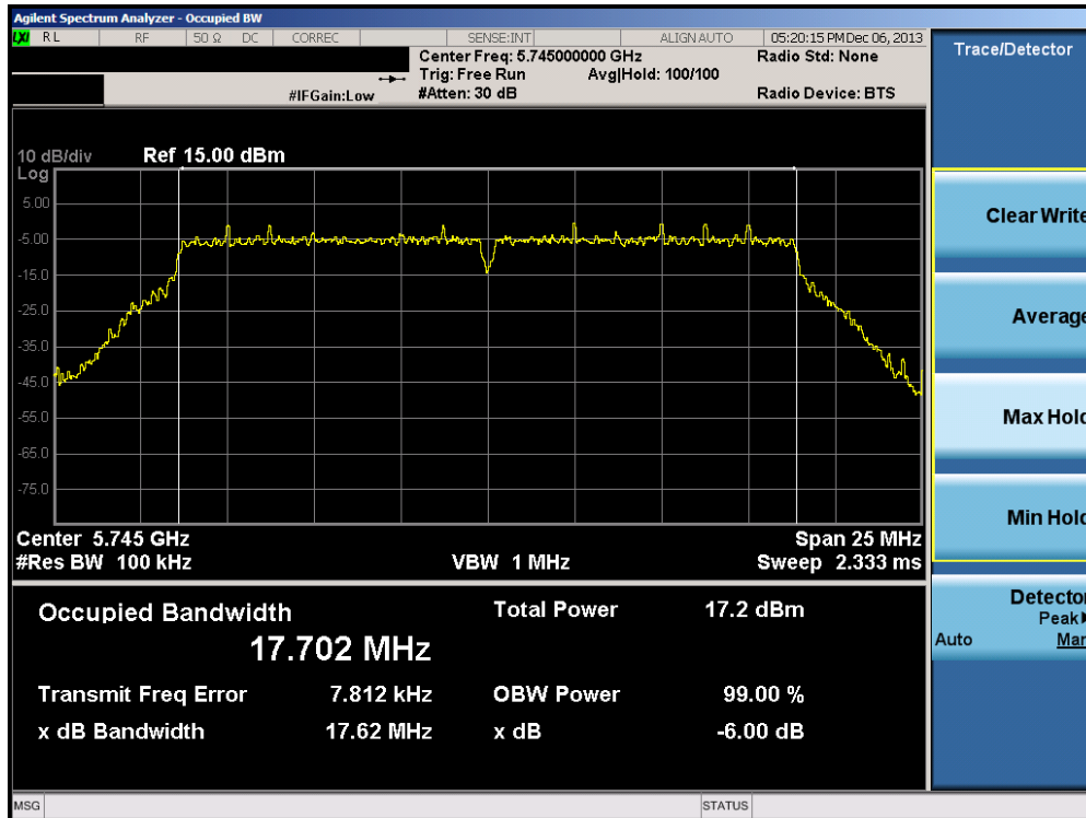
Plot 6-28. 6dB Bandwidth Plot (20MHz BW 802.11n (5.8GHz) – Ch. 149)
