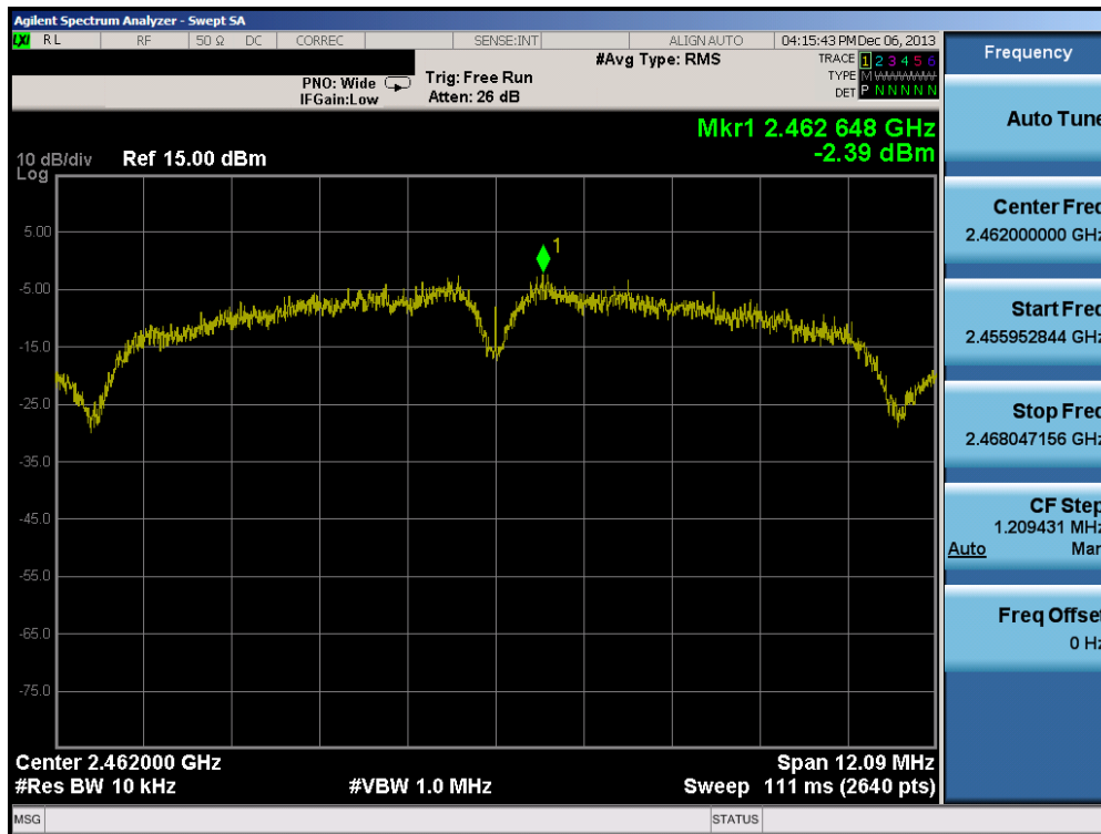
Plot 6-36. Power Spectral Density Plot (802.11b – Ch. 11)
