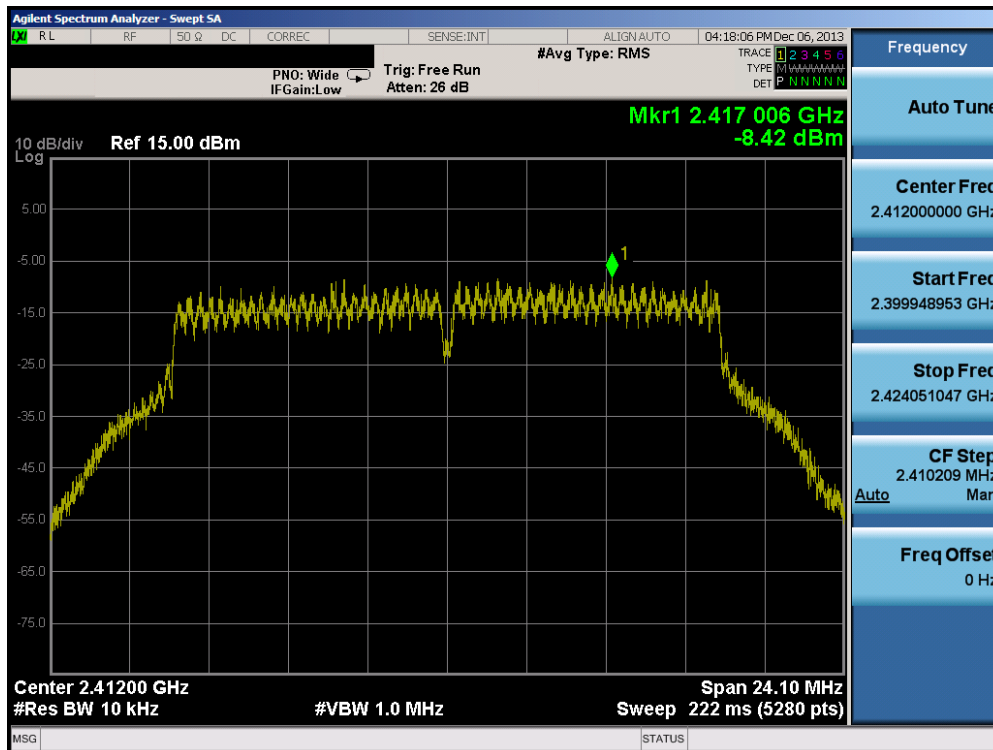
Plot 6-37. Power Spectral Density Plot (802.11g – Ch. 1)
