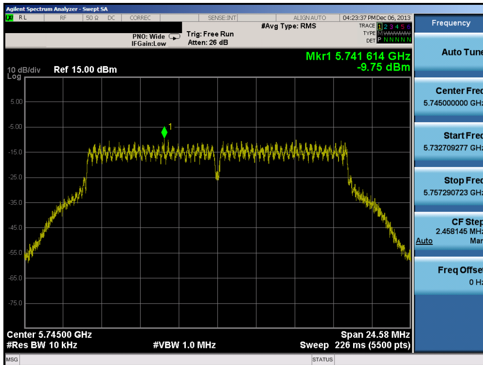
Plot 6-43. Power Spectral Density Plot (802.11a – Ch. 149)
