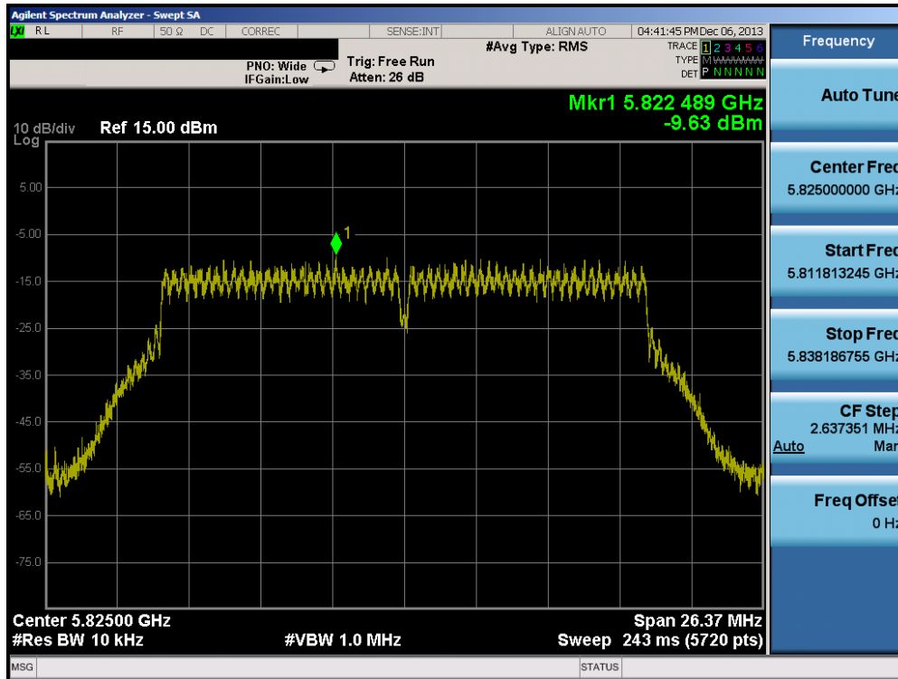
Plot 6-48. Power Spectral Density Plot (20MHz BW 802.11n (5.8GHz) – Ch. 165)
