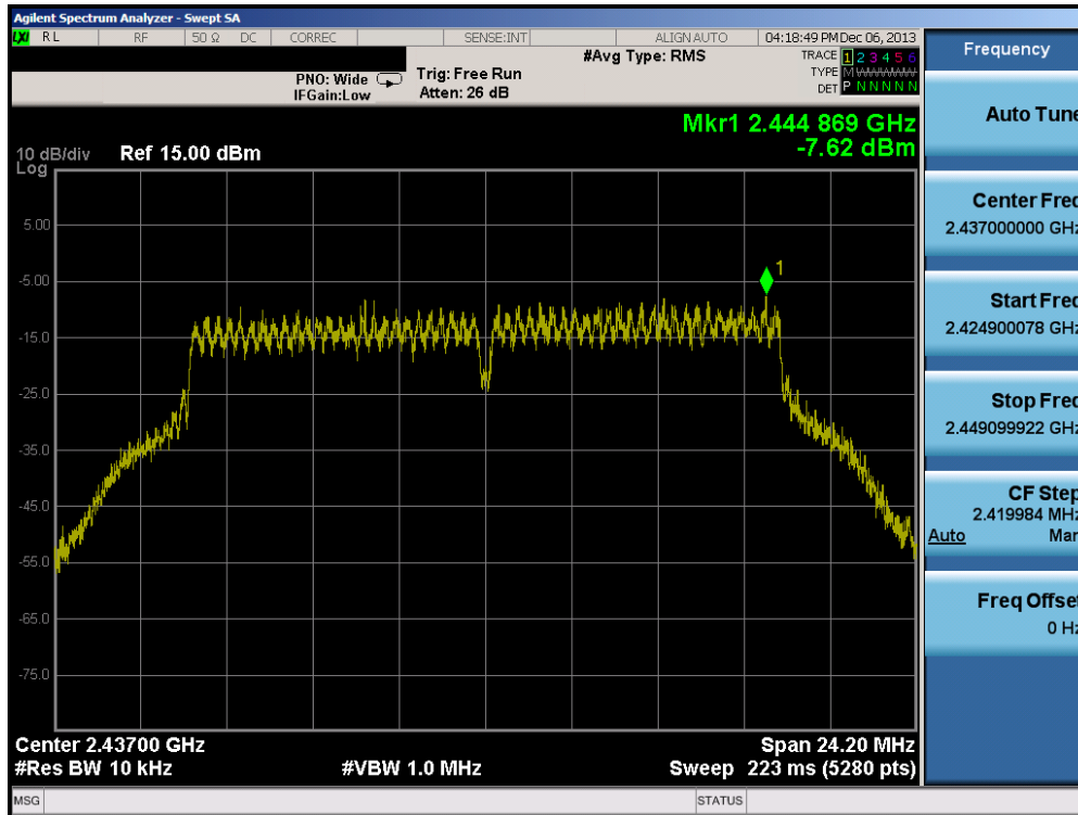
Plot 6-38. Power Spectral Density Plot (802.11g - Ch. 6)
