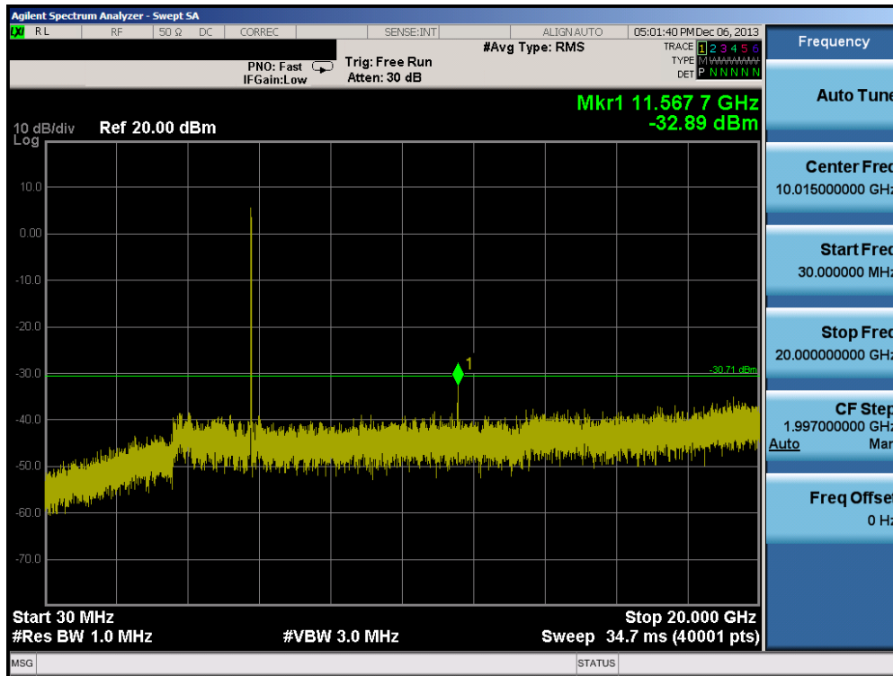
Plot 6-113. Conducted Spurious Plot (802.11a – Ch. 157)
