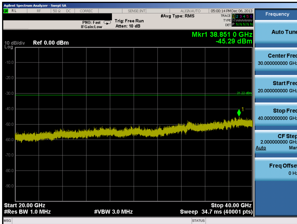
Plot 6-112. Conducted Spurious Plot (802.11a – Ch. 149)
