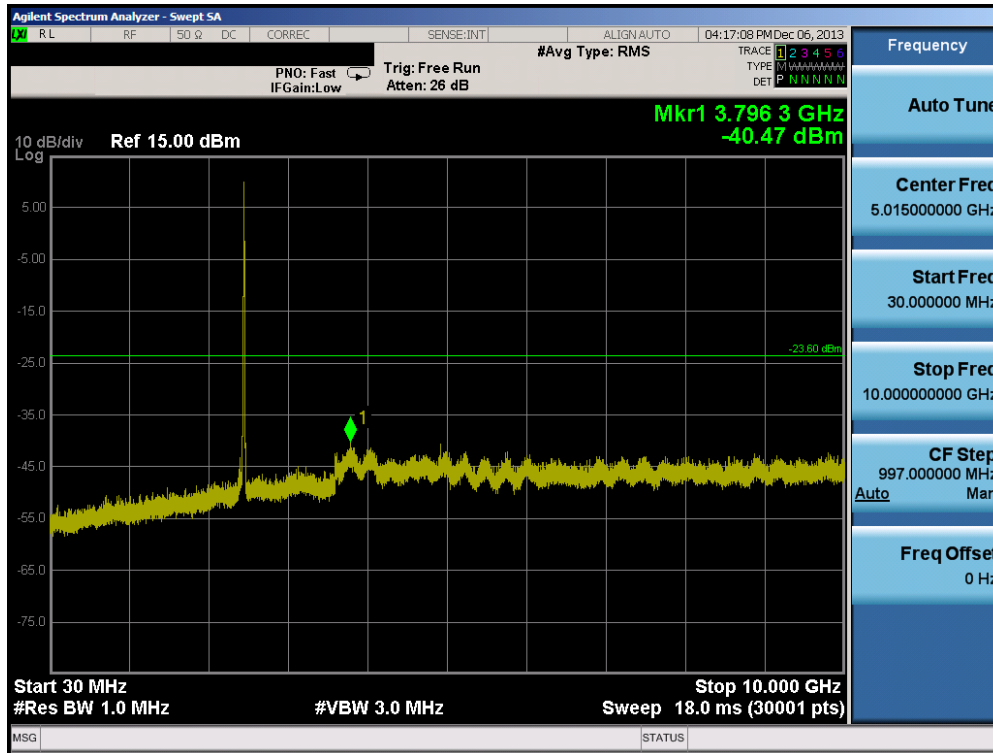
Plot 6-97. Conducted Spurious Plot (802.11b – Ch. 11)
