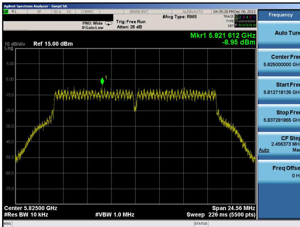
Plot 6-45. Power Spectral Density Plot (802.11a - Ch. 165)
