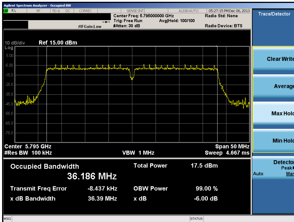
Plot 6-32. 6dB Bandwidth Plot (40MHz BW 802.11n (5.8GHz) – Ch. 159)
