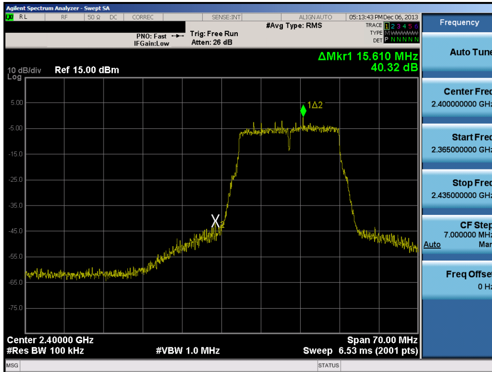
Plot 6-83. Band Edge Plot (802.11n (2.4GHz) – Ch. 1)
