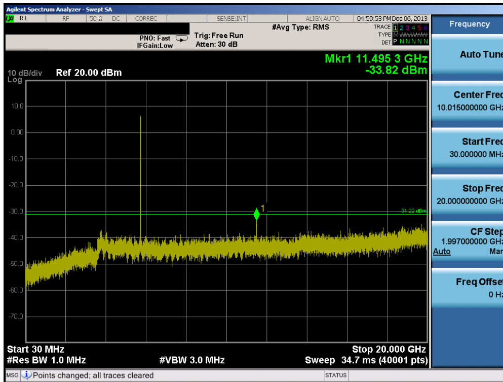
Plot 6-111. Conducted Spurious Plot (802.11a – Ch. 149)
