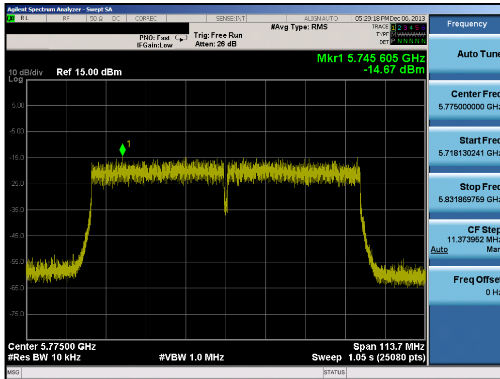
Plot 6-66. Power Spectral Density Plot (80MHz BW 802.11ac (5.8GHz) – Ch. 155)
