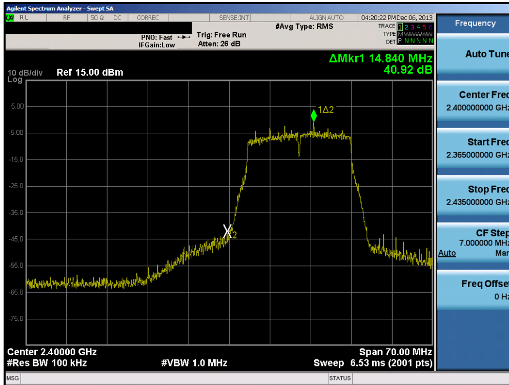
Plot 6-71. Band Edge Plot (802.11n (2.4GHz) – Ch. 1)
