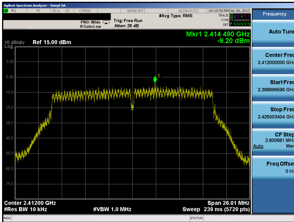
Plot 6-40. Power Spectral Density Plot (802.11n (2.4GHz) – Ch. 1)
