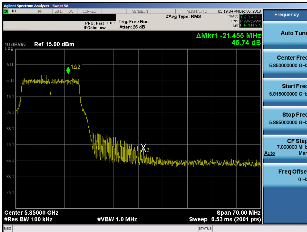
Plot 6-86. Band Edge Plot (802.11a – Ch. 165)
