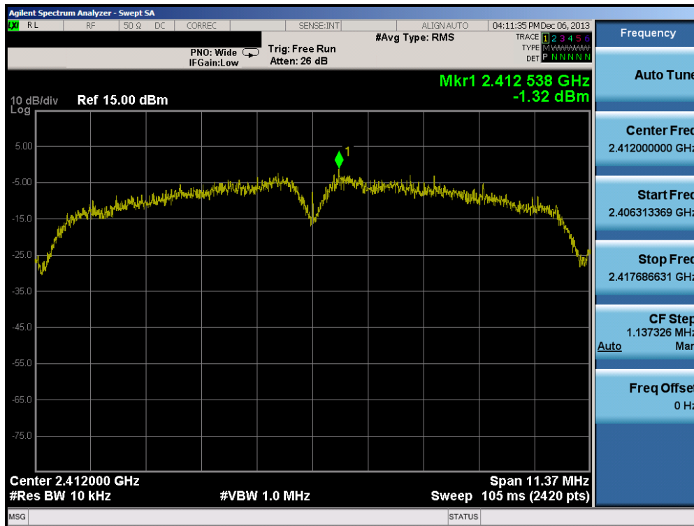
Plot 6-34. Power Spectral Density Plot (802.11b - Ch. 1)
