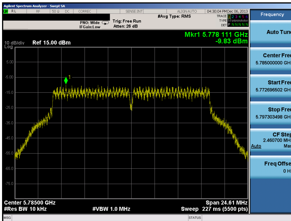
Plot 6-44. Power Spectral Density Plot (802.11a - Ch. 157)
