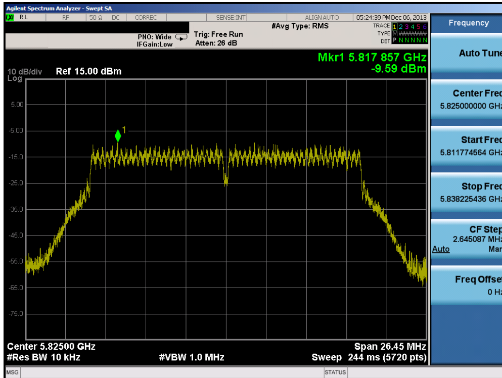
Plot 6-63. Power Spectral Density Plot (20MHz BW 802.11n (5.8GHz) – Ch. 165)
