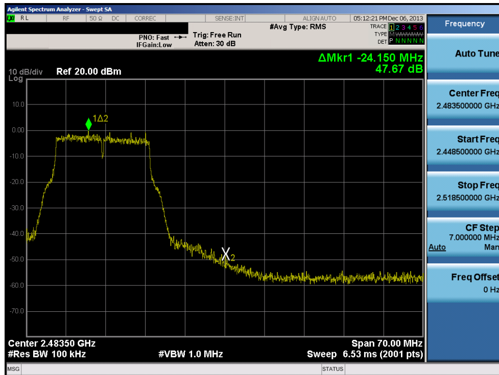
Plot 6-82. Band Edge Plot (802.11g – Ch. 11)
