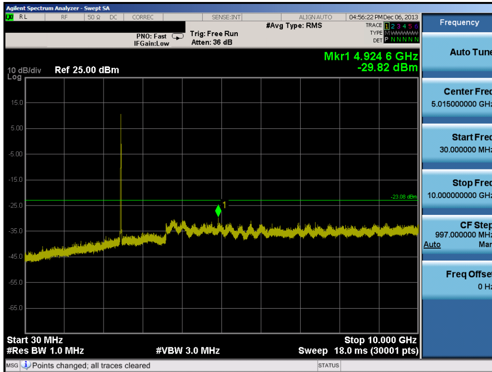
Plot 6-109. Conducted Spurious Plot (802.11g – Ch. 11)
