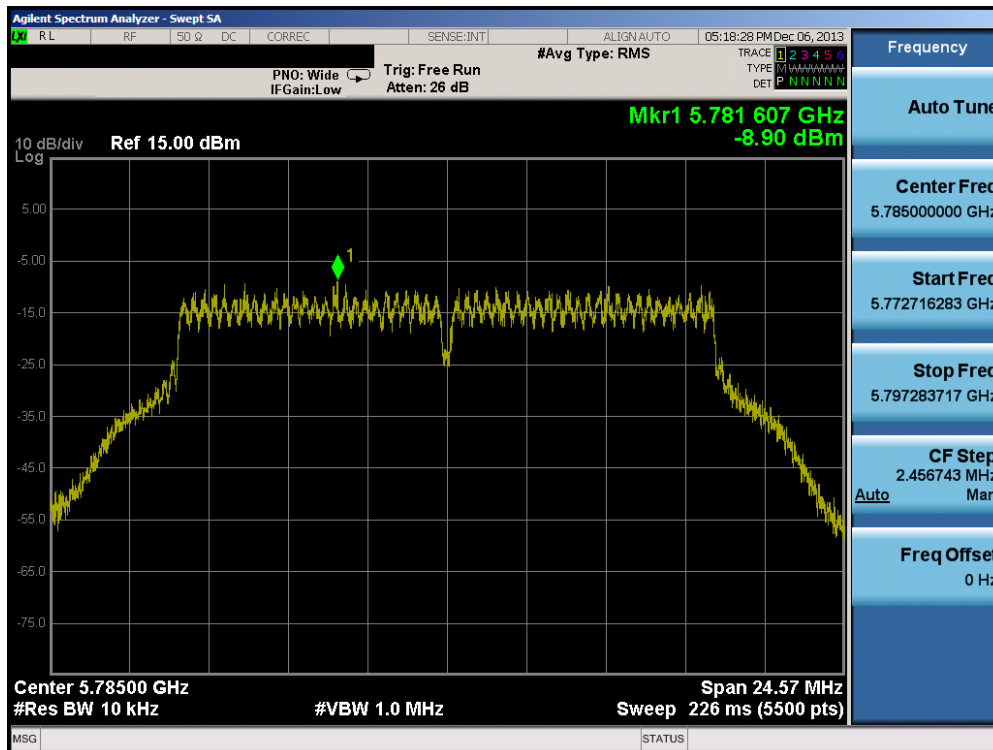
Plot 6-59. Power Spectral Density Plot (802.11a – Ch. 157)
