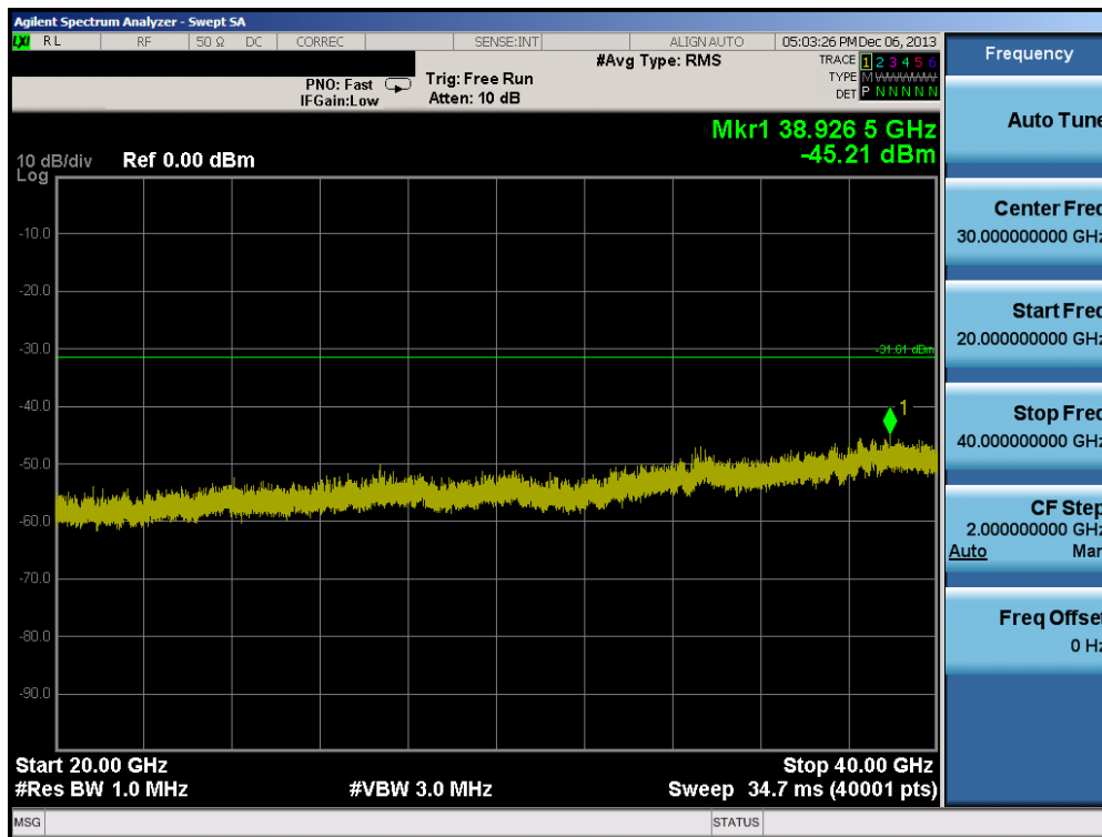
Plot 6-116. Conducted Spurious Plot (802.11a – Ch. 165)
