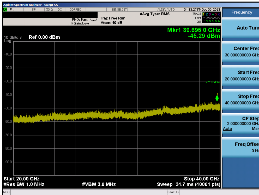
Plot 6-102. Conducted Spurious Plot (802.11a – Ch. 157)
