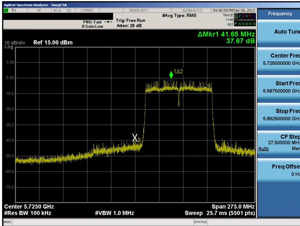
Plot 6-79. Band Edge Plot (80MHz BW 802.11ac (5.8GHz) – Ch. 155)
