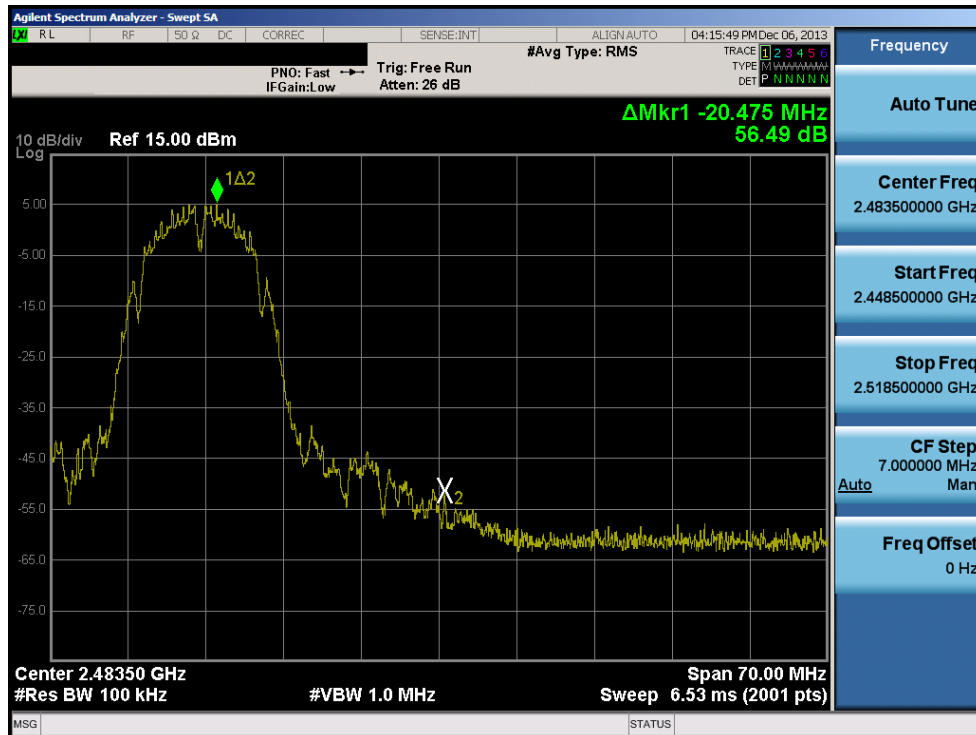
Plot 6-68. Band Edge Plot (802.11b – Ch. 11)
