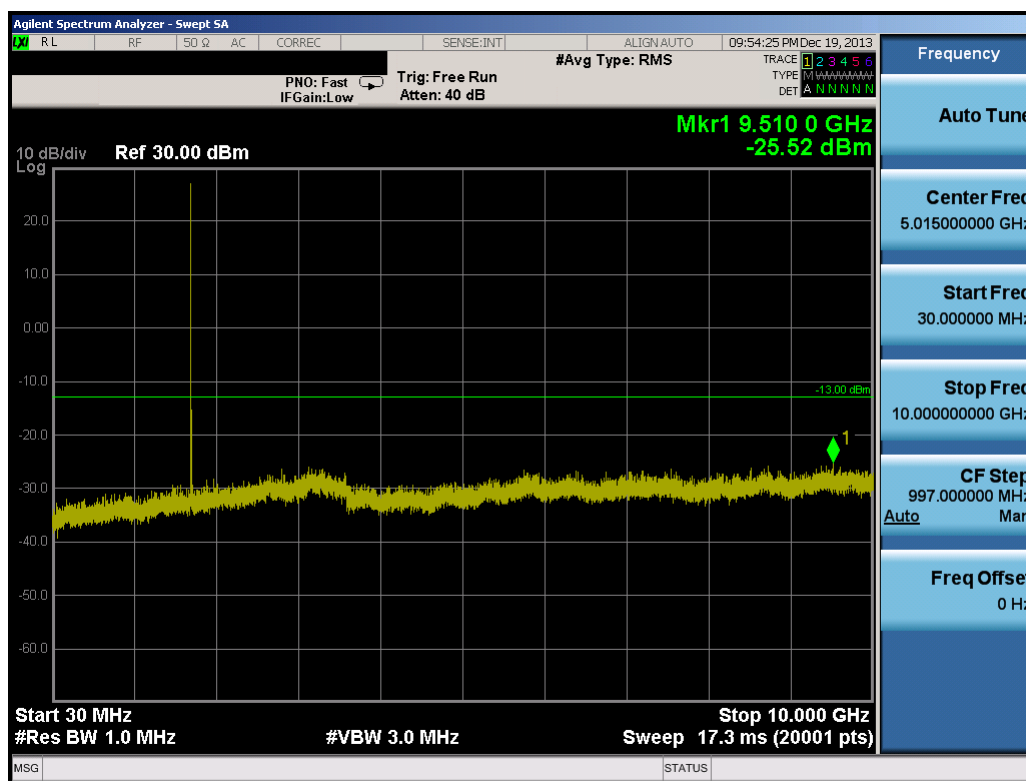
Plot 9-47. Conducted Spurious Plot (10.0MHz QPSK – RB Size 1, RB Offset 0– Low Channel)
