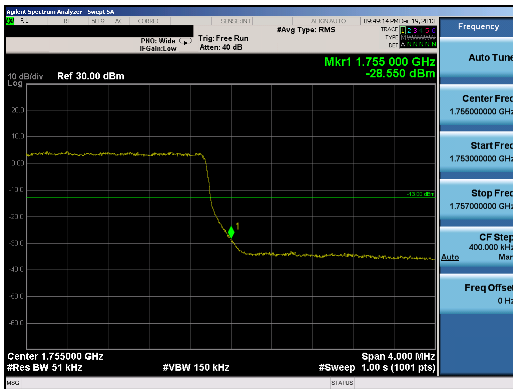
Plot 9-39. Upper Band Edge Plot (5.0MHz QPSK – RB Size 25)
