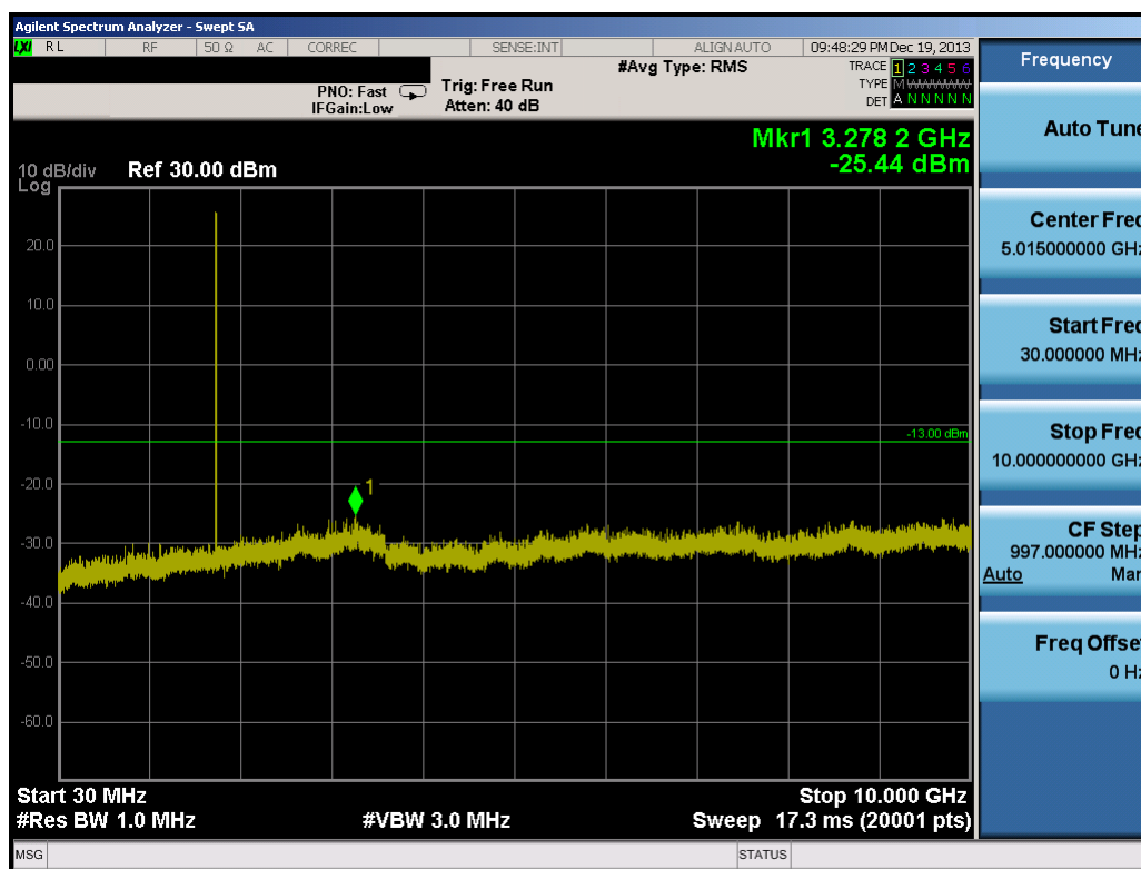
Plot 9-37. Conducted Spurious Plot (5.0MHz QPSK – RB Size 1, RB Offset 0 – High Channel)
