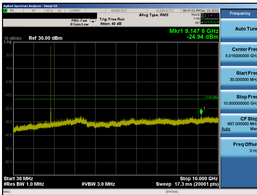
Plot 10-61. Conducted Spurious Plot (15.0MHz QPSK – RB Size 1, RB Offset 0 – Low Channel)
