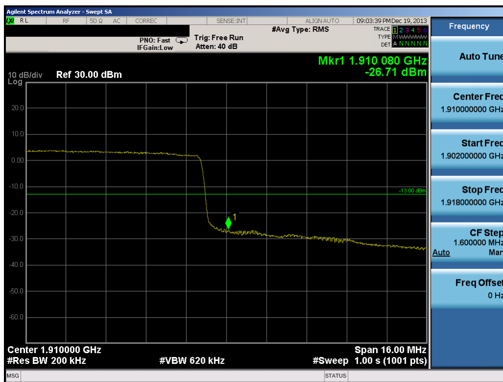
Plot 10-81. Upper Band Edge Plot (20.0MHz QPSK – RB Size 100)
