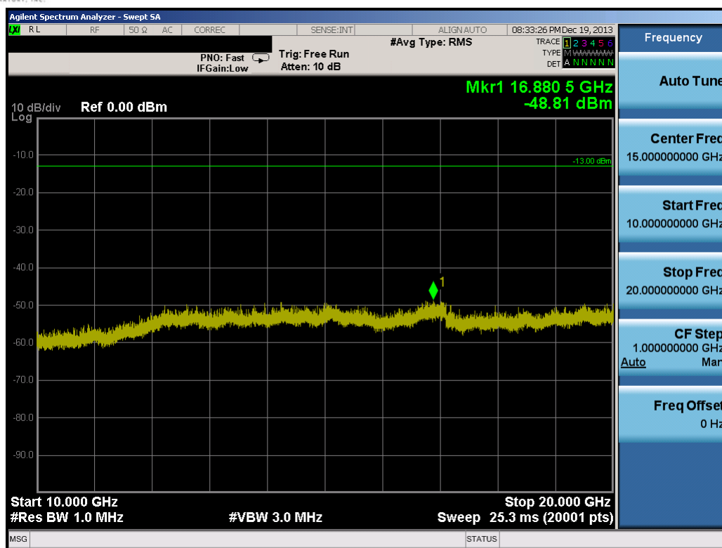
Plot 10-38. Conducted Spurious Plot (5.0MHz QPSK – RB Size 1, RB Offset 0 – High Channel)
