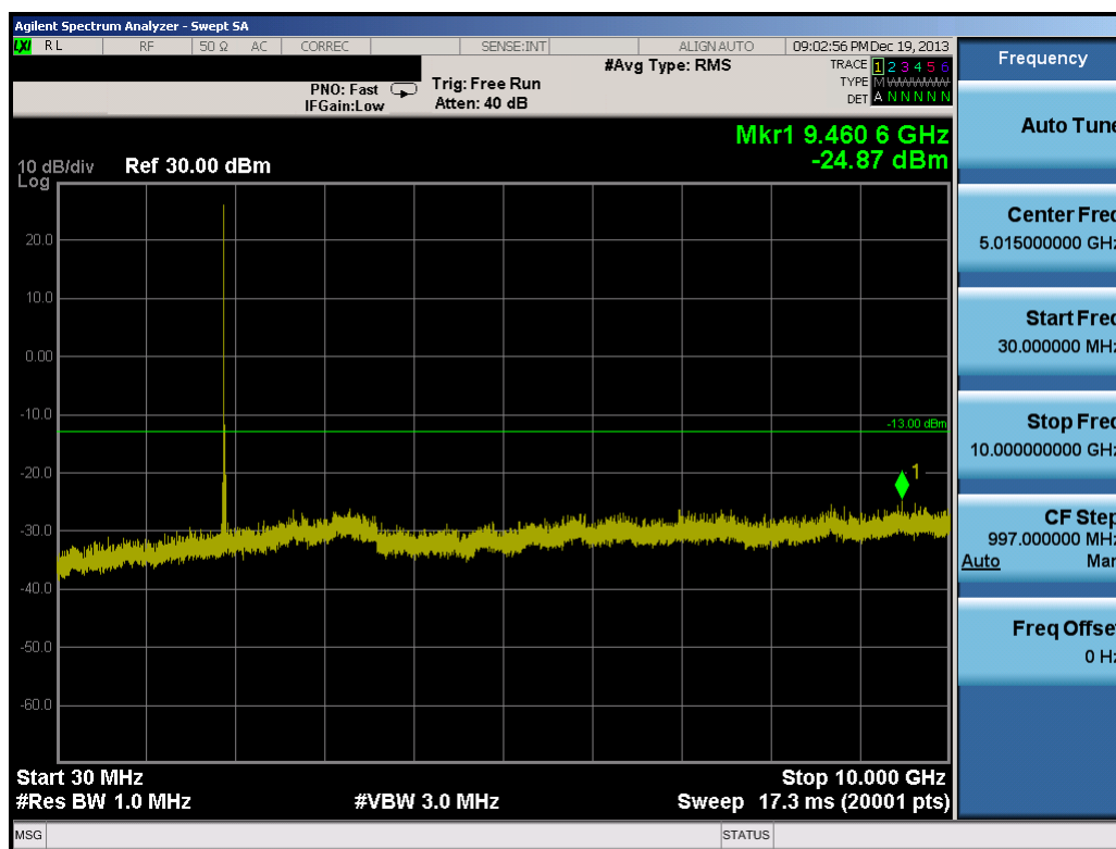
Plot 10-79. Conducted Spurious Plot (20.0MHz QPSK – RB Size 1, RB Offset 0 – High Channel)
