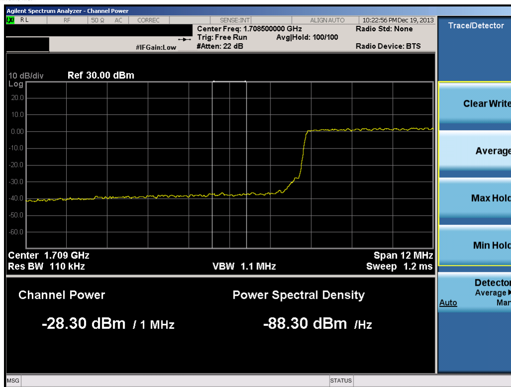
Plot 9-58. Lower Extended Band Edge Plot (15.0MHz QPSK – RB Size 75)
