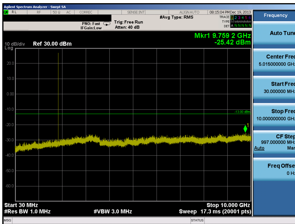
Plot 10-5. Conducted Spurious Plot (1.4MHz QPSK – RB Size 1, RB Offset 0 – Low Channel)
