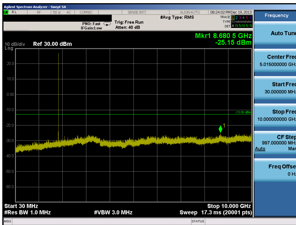
Plot 10-19. Conducted Spurious Plot (3.0MHz QPSK – RB Size 1, RB Offset 0 – Low Channel)
