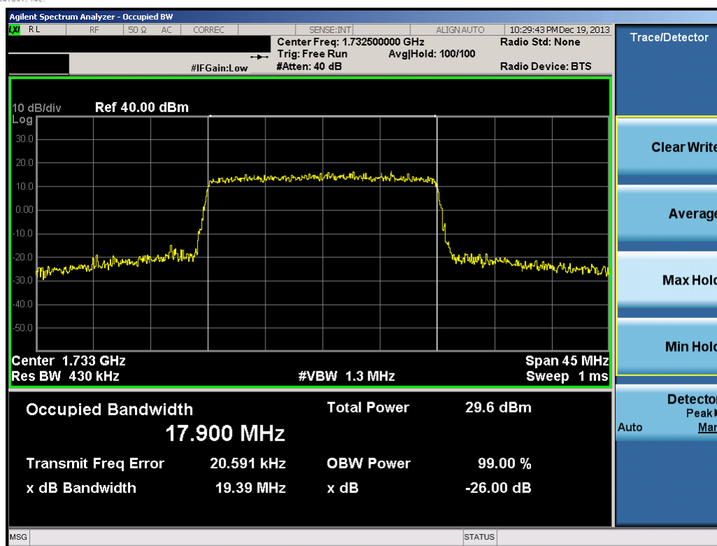
Plot 9-74. Occupied Bandwidth Plot (20.0MHz 16-QAM – RB Size 100)
