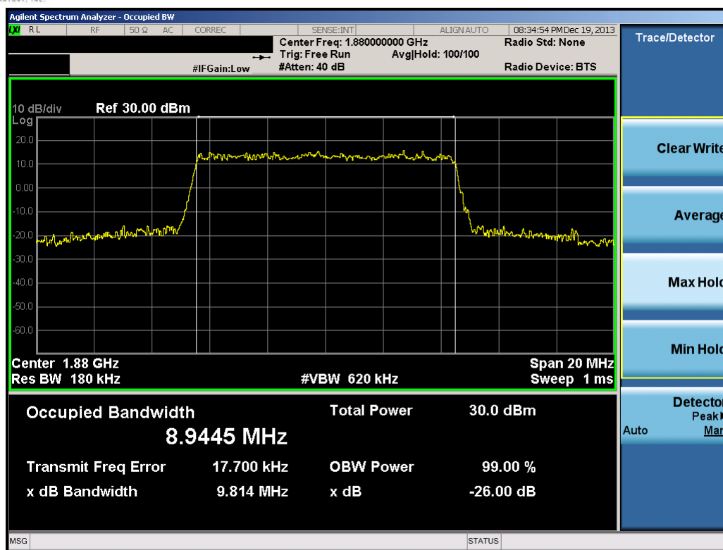
Plot 10-46. Occupied Bandwidth Plot (10.0MHz 16-QAM – RB Size 50)
