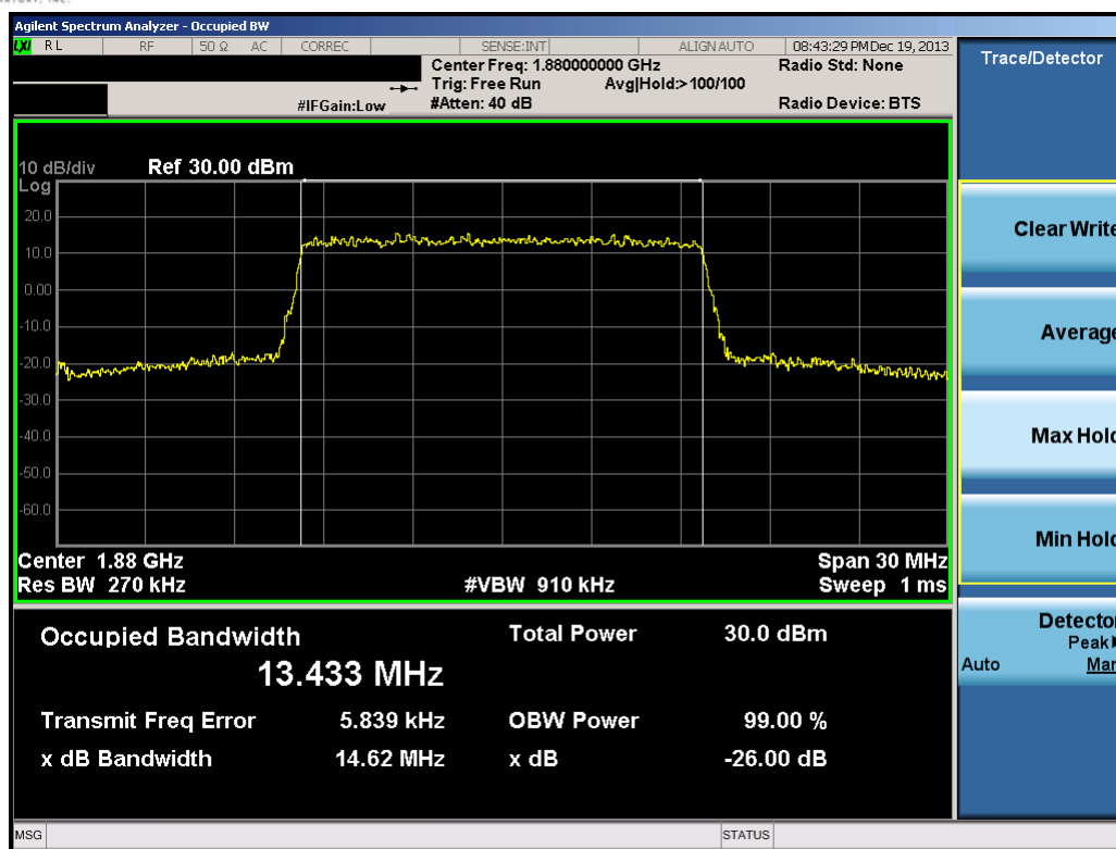
Plot 10-60. Occupied Bandwidth Plot (15.0MHz 16-QAM – RB Size 75)
