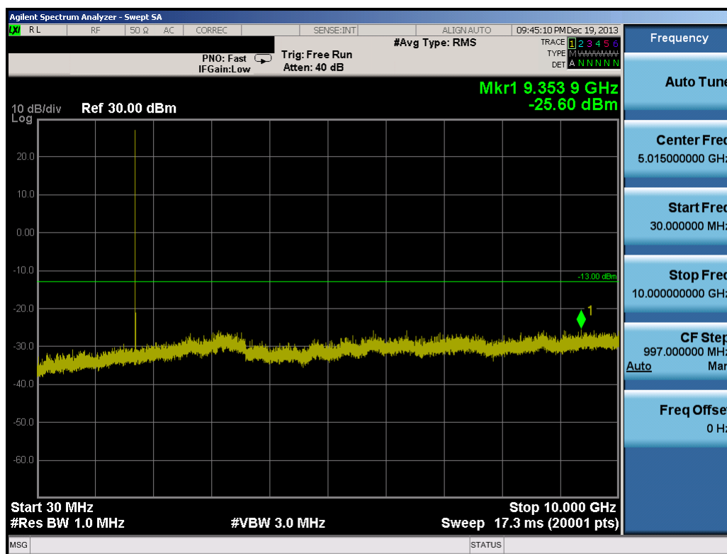
Plot 9-33. Conducted Spurious Plot (5.0MHz QPSK – RB Size 1, RB Offset 0 – Low Channel)
