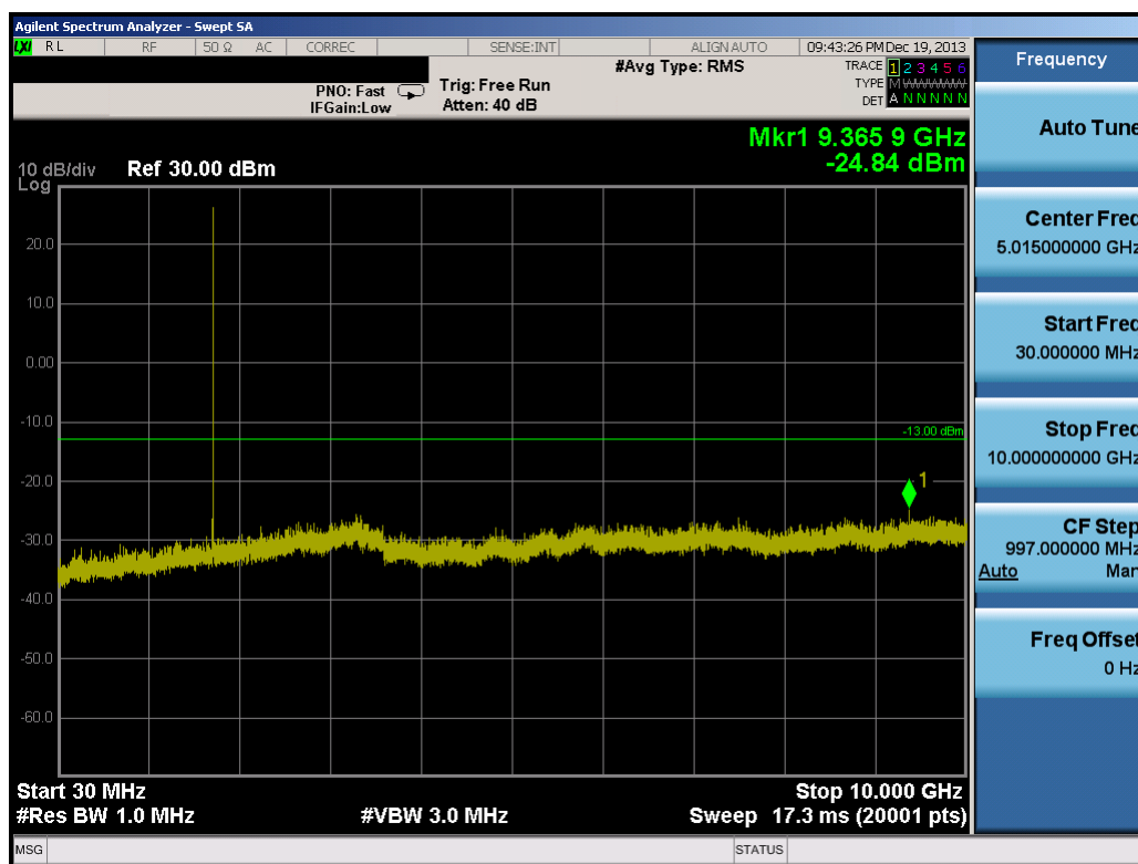
Plot 9-35. Conducted Spurious Plot (5.0MHz QPSK – RB Size 1, RB Offset 0 – Mid Channel)
