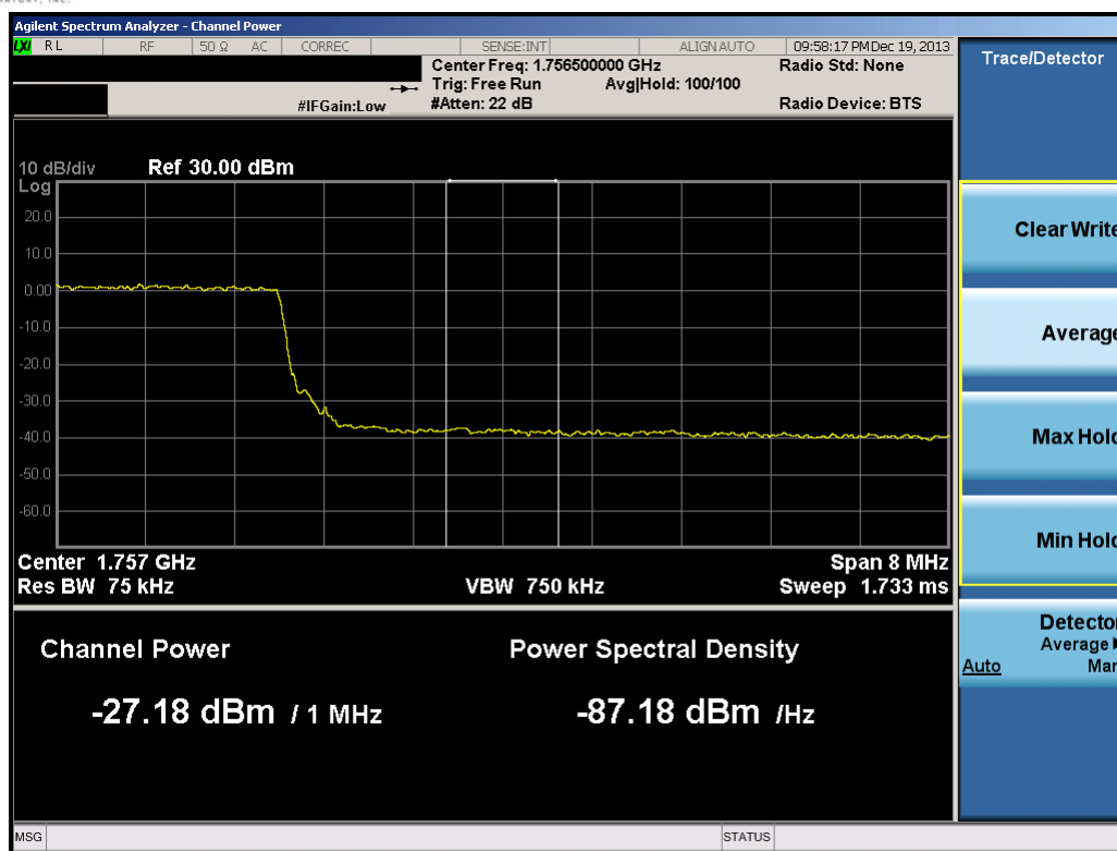
Plot 9-54. Upper Extended Band Edge Plot (10.0MHz QPSK – RB Size 50)
