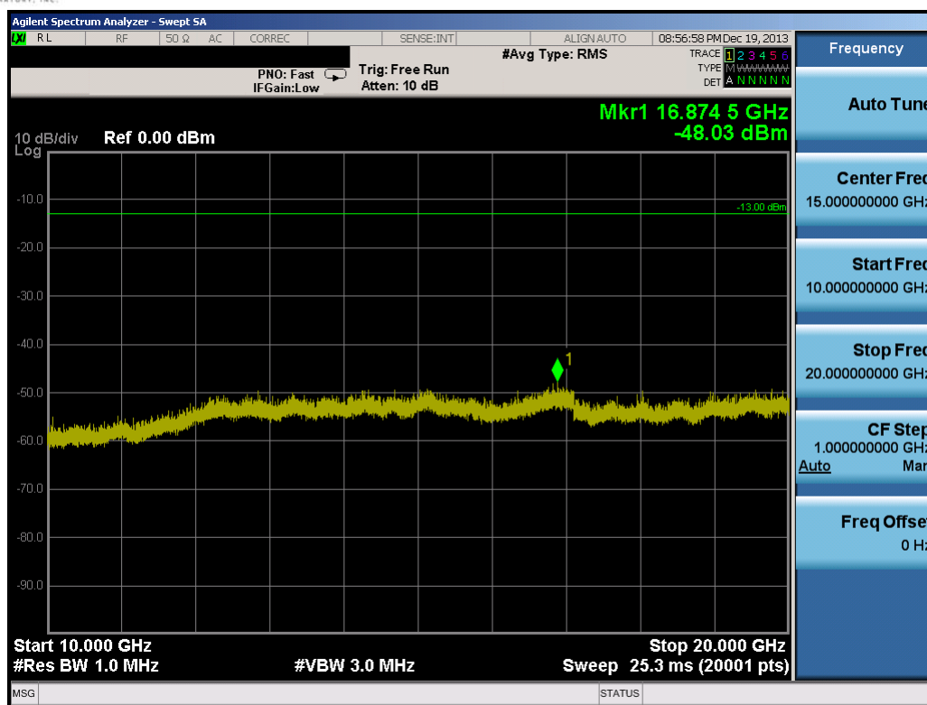
Plot 10-78. Conducted Spurious Plot (20.0MHz QPSK – RB Size 1, RB Offset 0 – Mid Channel)
