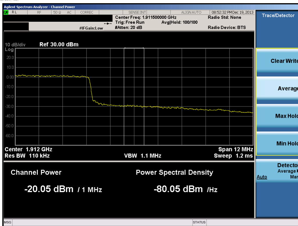
Plot 10-68. Upper Extended Band Edge Plot (15.0MHz QPSK – RB Size 75)
