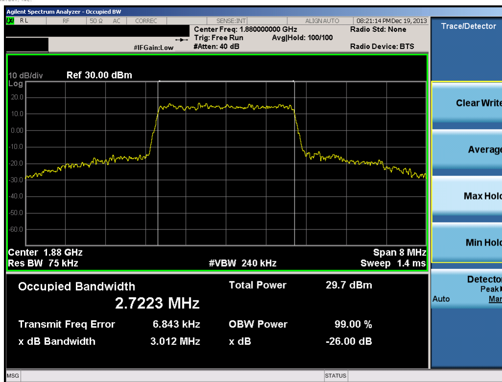
Plot 10-18. Occupied Bandwidth Plot (3.0MHz 16-QAM – RB Size 15)
