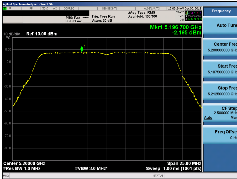
Plot 6-96. Peak Power Spectral Density Plot (20MHz BW 802.11n (UNII Band 1) – Ch. 40)
