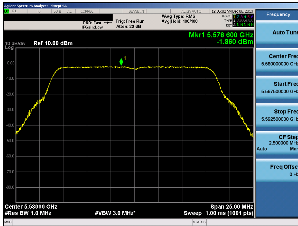
Plot 6-111. Peak Power Spectral Density Plot (802.11a (UNII Band 2C) – Ch. 116)
