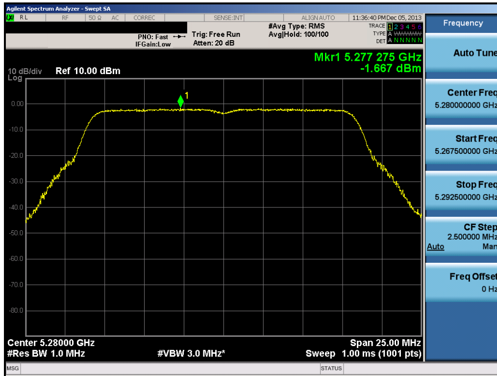
Plot 6-74. Peak Power Spectral Density Plot (802.11a (UNII Band 2A) – Ch. 56)
