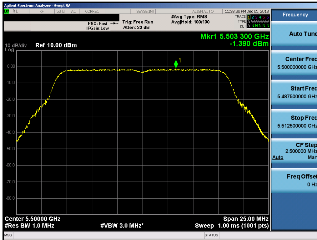
Plot 6-82. Peak Power Spectral Density Plot (802.11a (UNII Band 2C) – Ch. 100)
