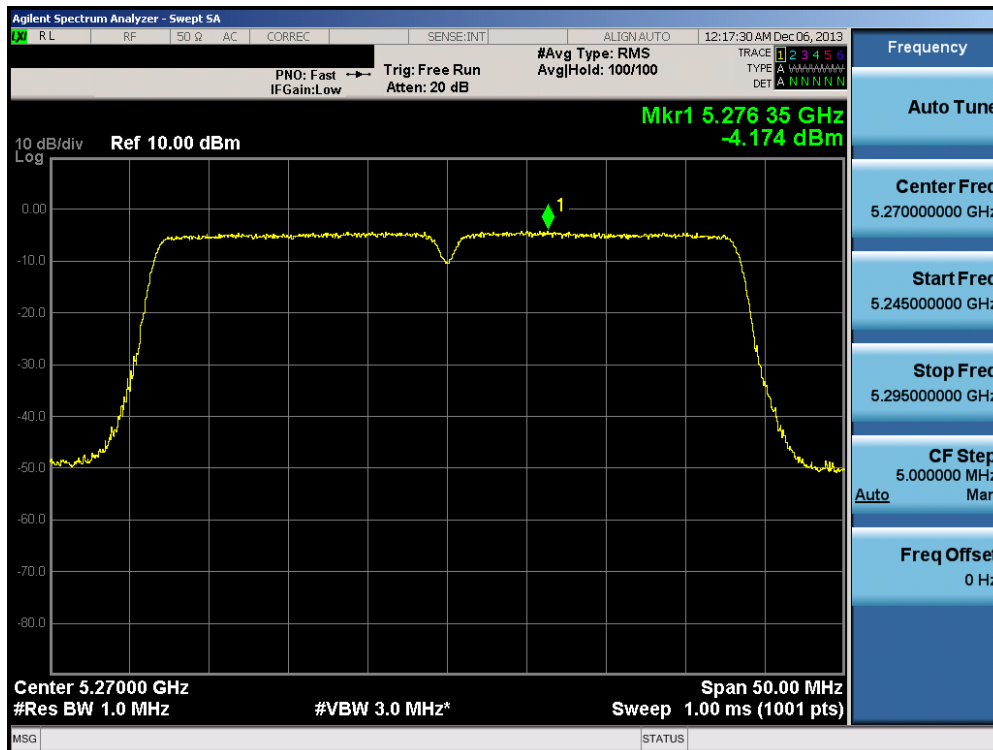
Plot 6-107. Peak Power Spectral Density Plot (40MHz BW 802.11n (UNII Band 2A) – Ch. 54)
