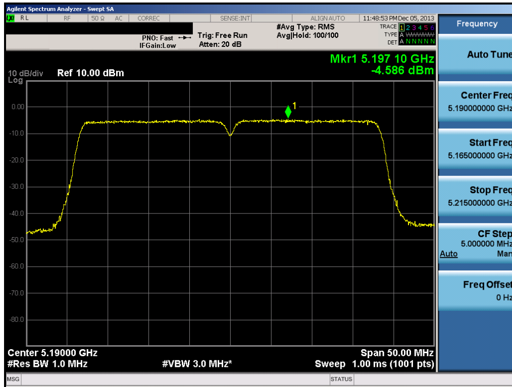
Plot 6-70. Peak Power Spectral Density Plot (40MHz BW 802.11n (UNII Band 1) – Ch. 38)
