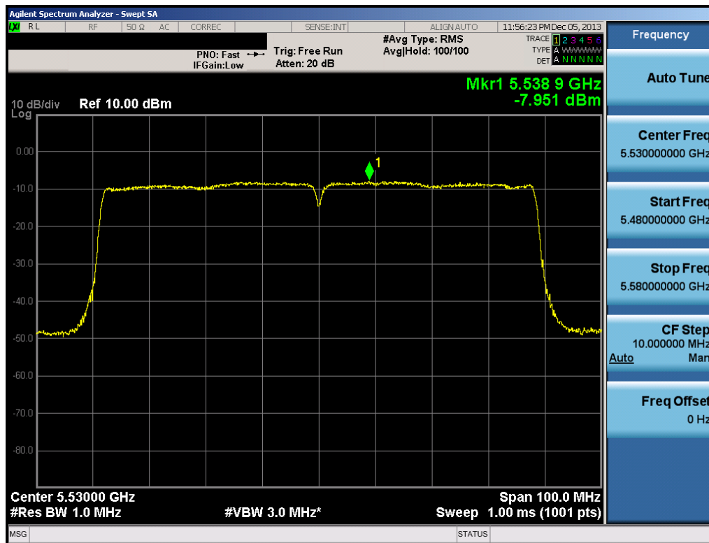
Plot 6-91. Peak Power Spectral Density Plot (80MHz BW 802.11ac (UNII Band 2C) – Ch. 106)
