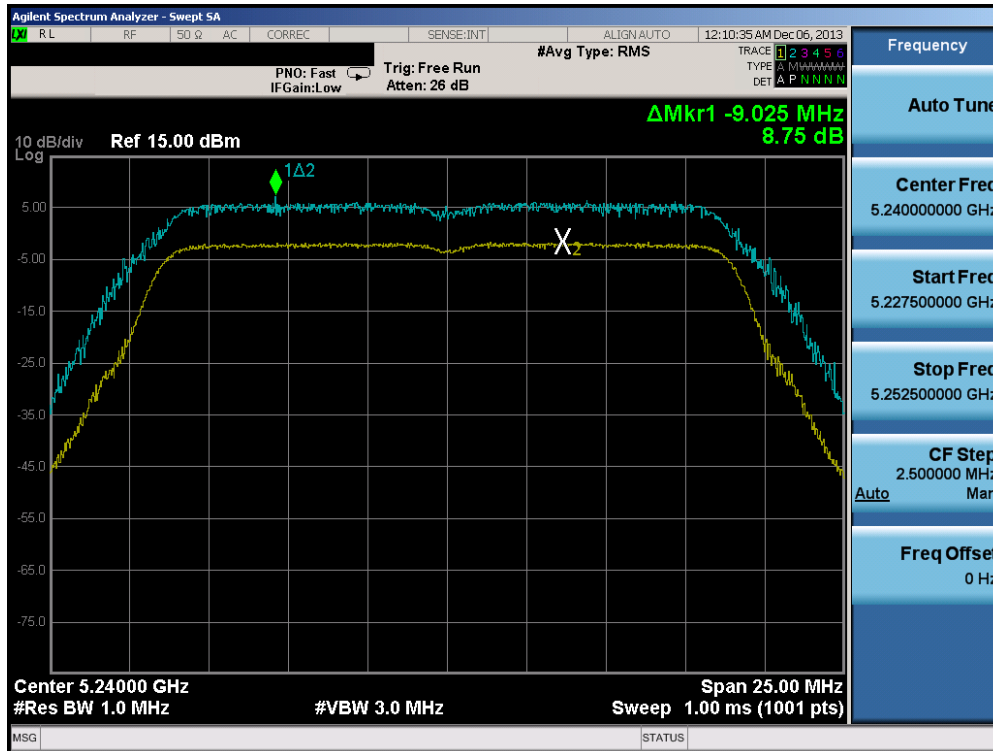
Plot 6-125. Peak Excursion Ratio Plot (20MHz BW 802.11n)
