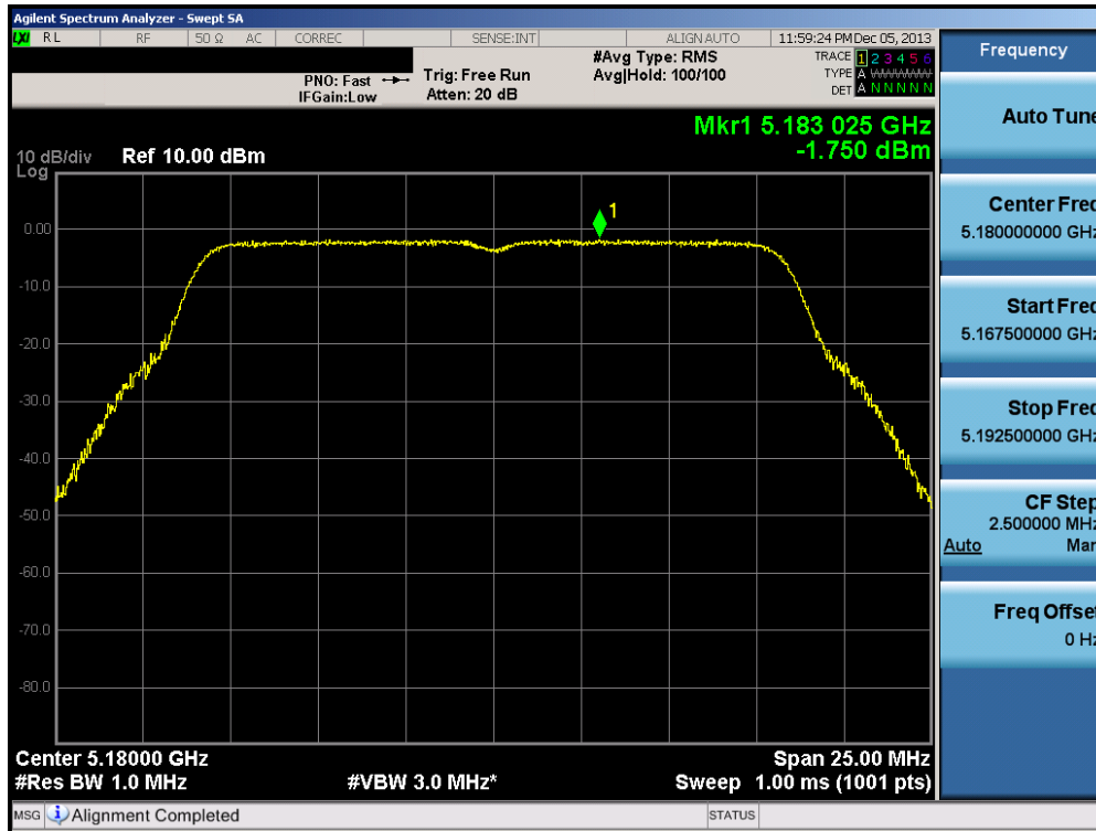
Plot 6-92. Peak Power Spectral Density Plot (802.11a (UNII Band 1) – Ch. 36)
