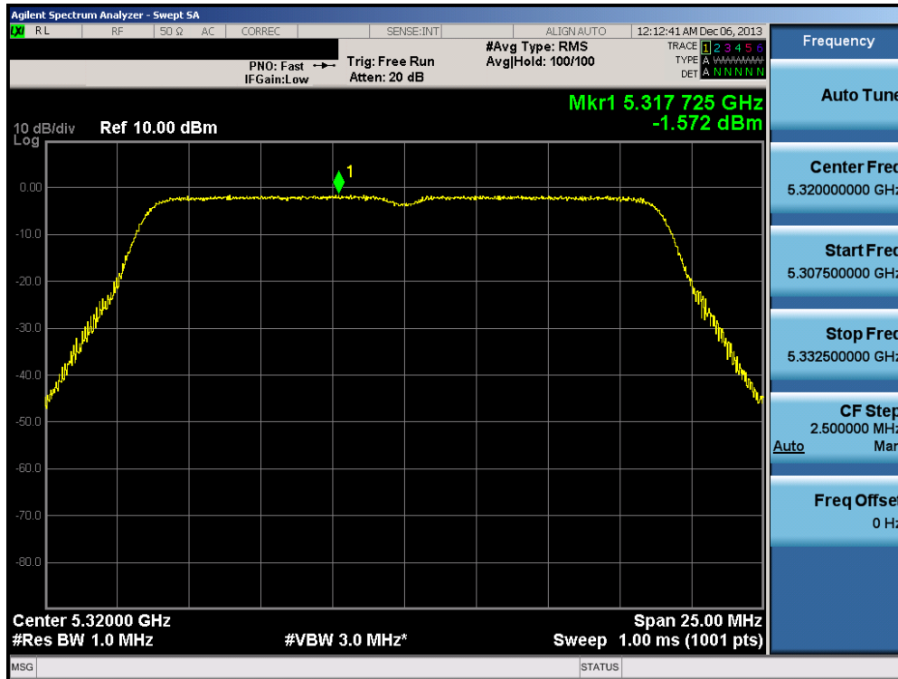
Plot 6-106. Peak Power Spectral Density Plot (20MHz BW 802.11n (UNII Band 2A) – Ch. 64)
