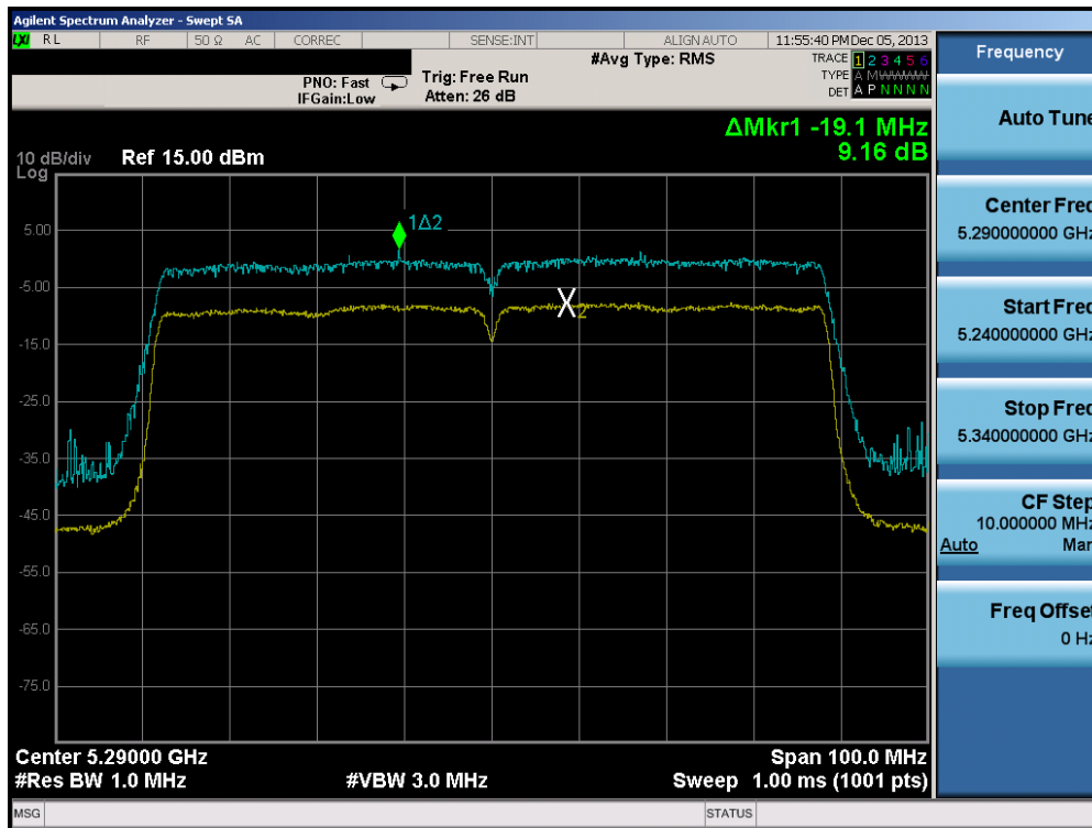
Plot 6-123. Peak Excursion Ratio Plot (80MHz BW 802.11ac)
