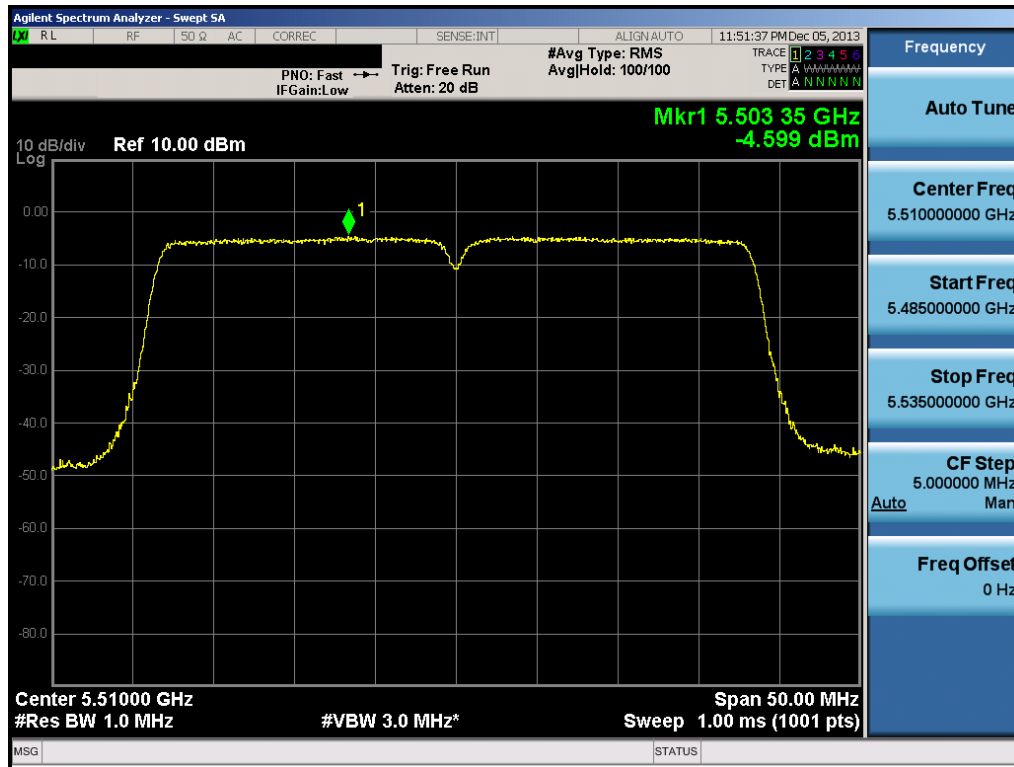
Plot 6-88. Peak Power Spectral Density Plot (40MHz BW 802.11n (UNII Band 2C) – Ch. 102)
