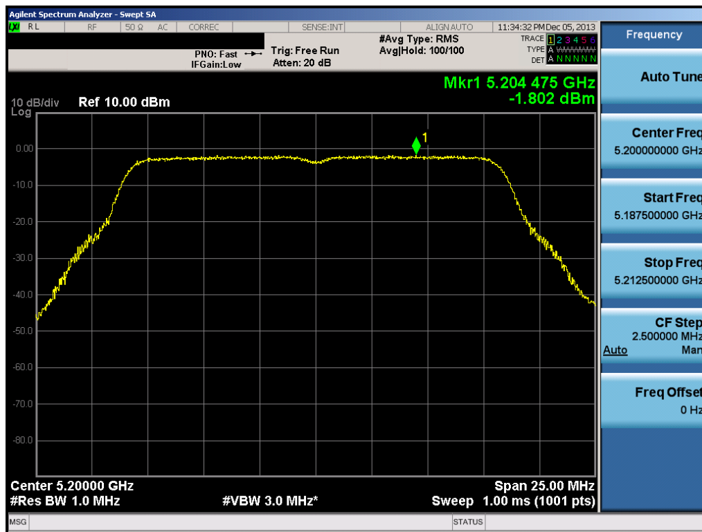
Plot 6-65. Peak Power Spectral Density Plot (802.11a (UNII Band 1) – Ch. 40)
