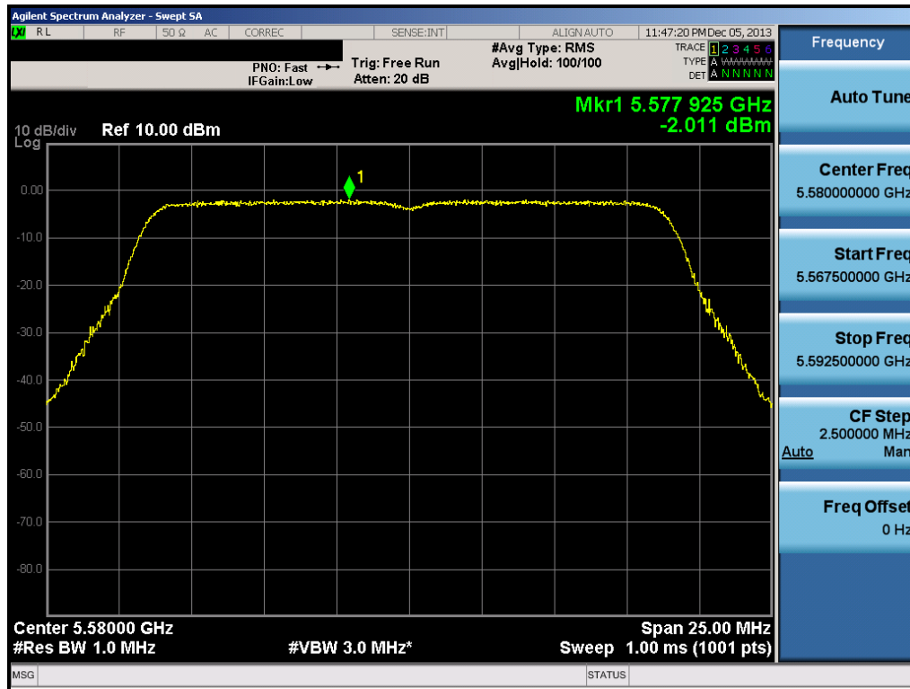
Plot 6-86. Peak Power Spectral Density Plot (20MHz BW 802.11n (UNII Band 2C) – Ch. 116)
