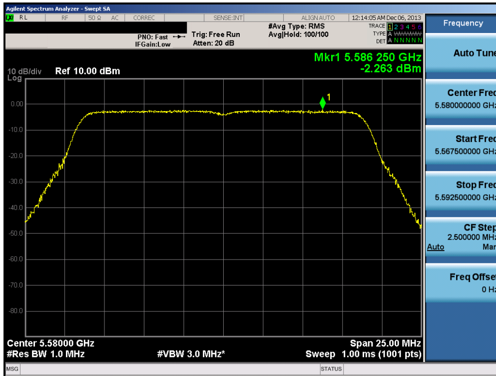
Plot 6-114. Peak Power Spectral Density Plot (20MHz BW 802.11n (UNII Band 2C) – Ch. 116)
