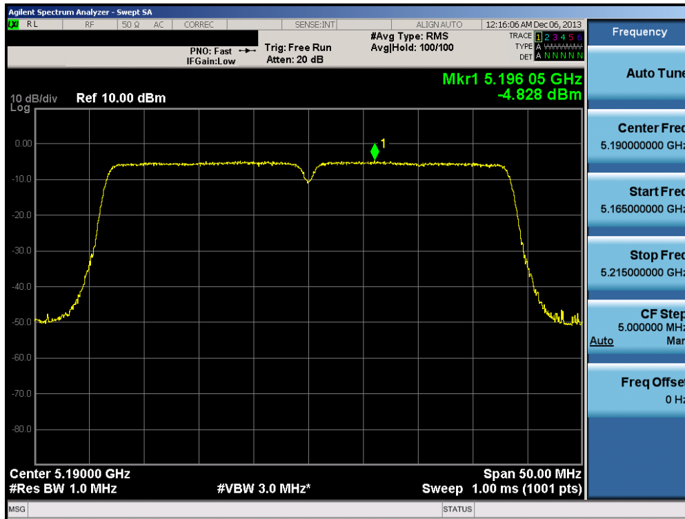
Plot 6-98. Peak Power Spectral Density Plot (40MHz BW 802.11n (UNII Band 1) – Ch. 38)
