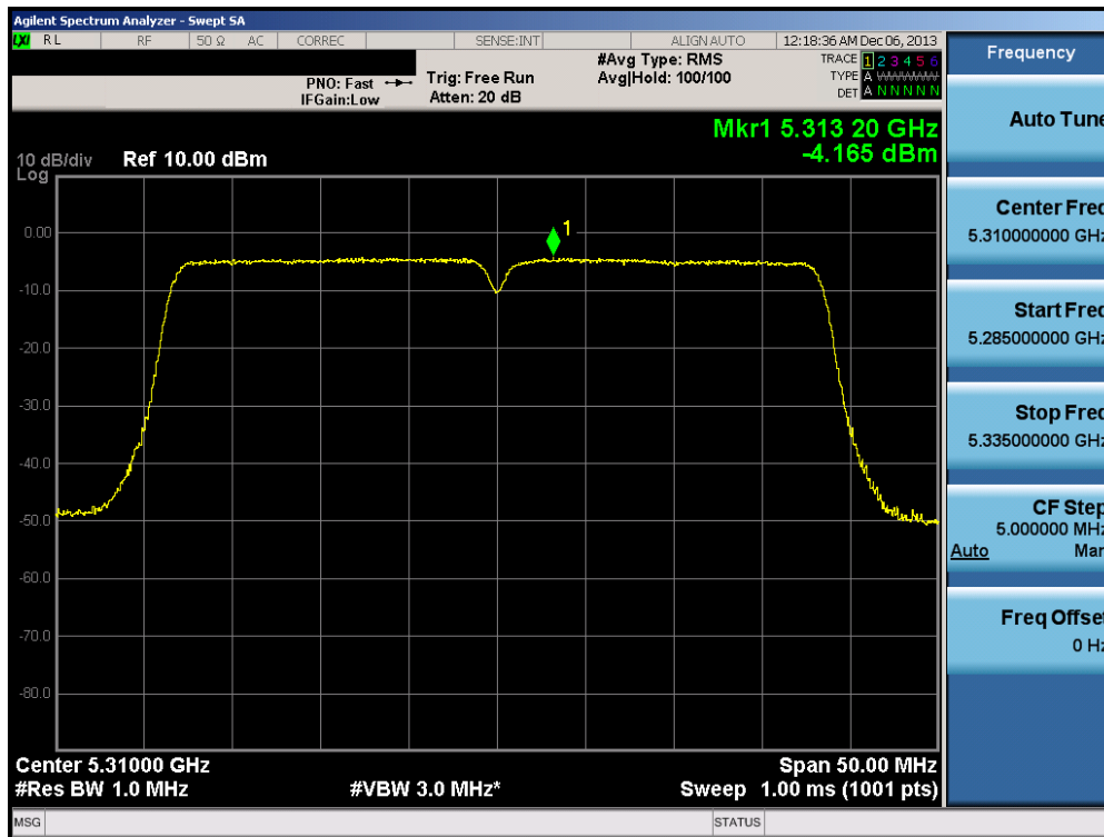
Plot 6-108. Peak Power Spectral Density Plot (40MHz BW 802.11n (UNII Band 2A) – Ch. 62)
