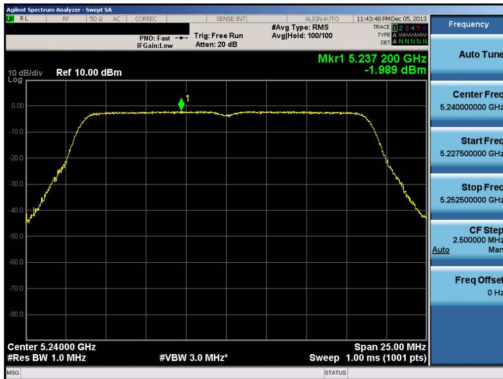
Plot 6-69. Peak Power Spectral Density Plot (20MHz BW 802.11n (UNII Band 1) – Ch. 48)
