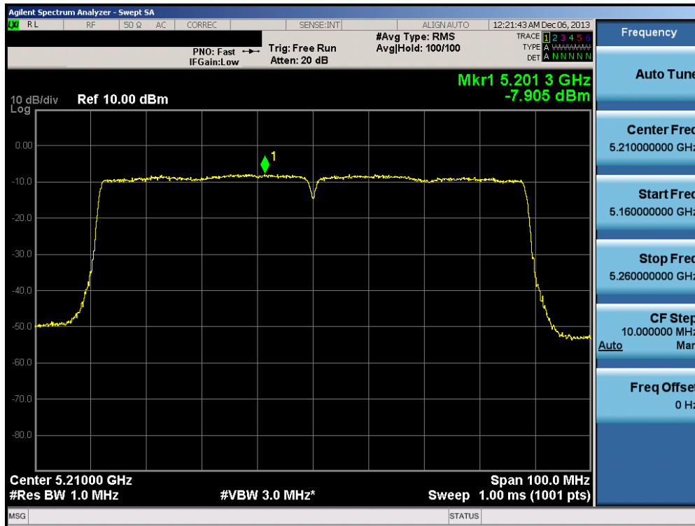
Plot 6-100. Peak Power Spectral Density Plot (80MHz BW 802.11ac (UNII Band 1) – Ch. 42)
