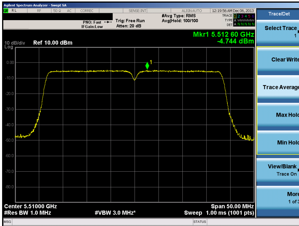
Plot 6-116. Peak Power Spectral Density Plot (40MHz BW 802.11n (UNII Band 2C) – Ch. 102)
