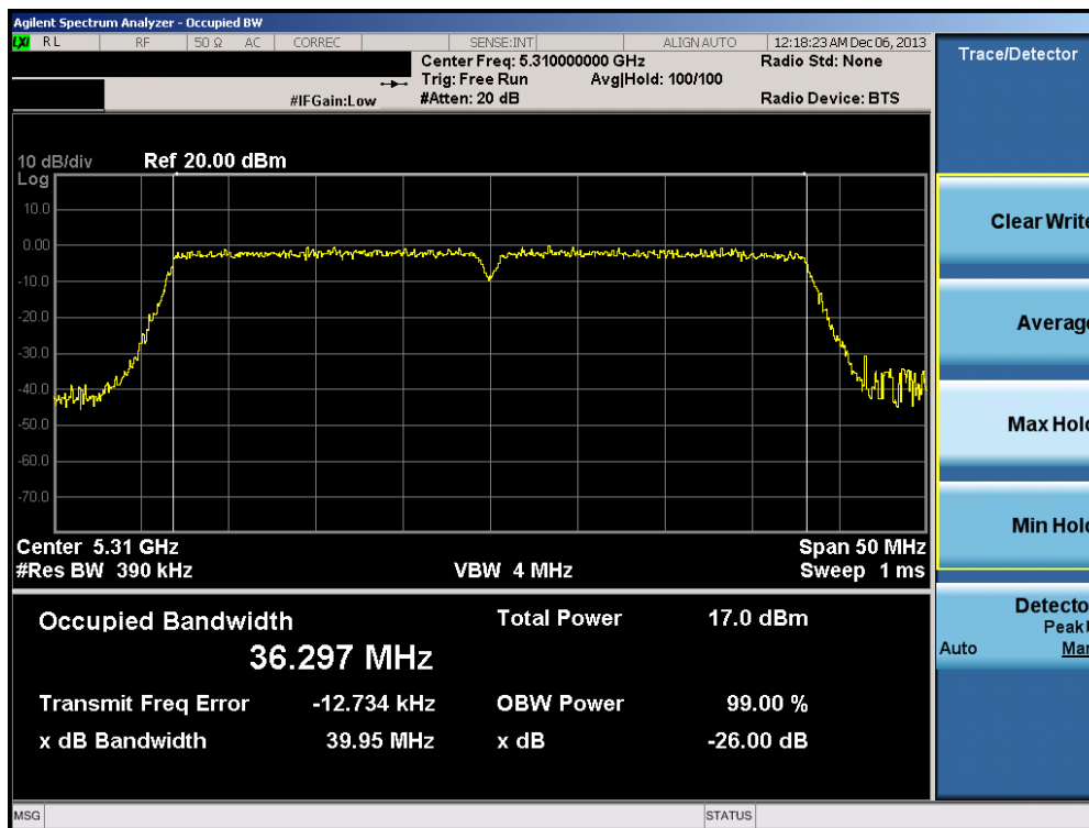
Plot 6-48. 26dB Bandwidth Plot (40MHz BW 802.11n (UNII Band 2A) – Ch. 62)
