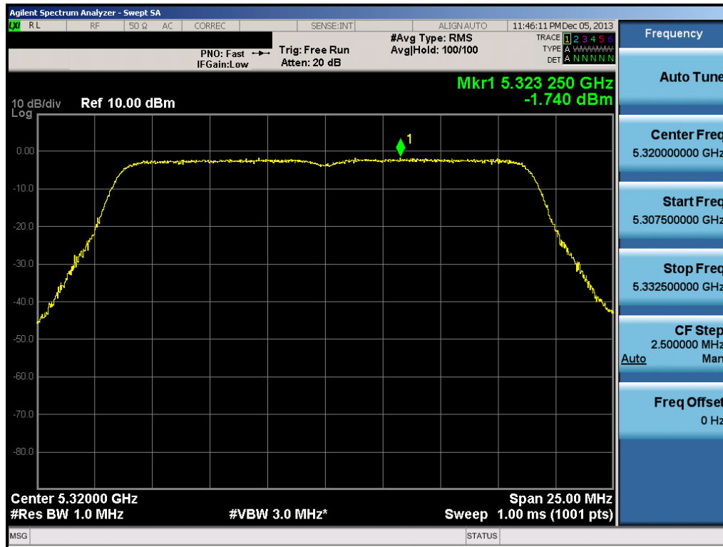
Plot 6-78. Peak Power Spectral Density Plot (20MHz BW 802.11n (UNII Band 2A) – Ch. 64)
