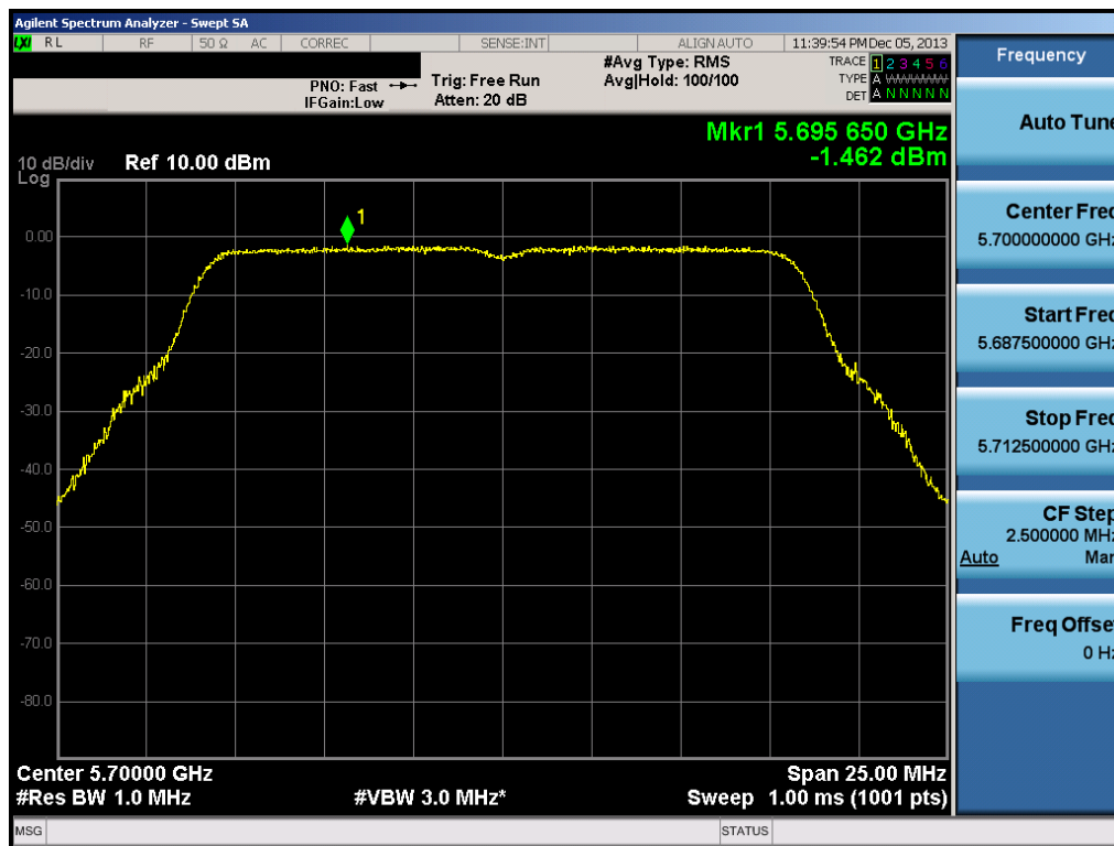
Plot 6-84. Peak Power Spectral Density Plot (802.11a (UNII Band 2C) – Ch. 140)
