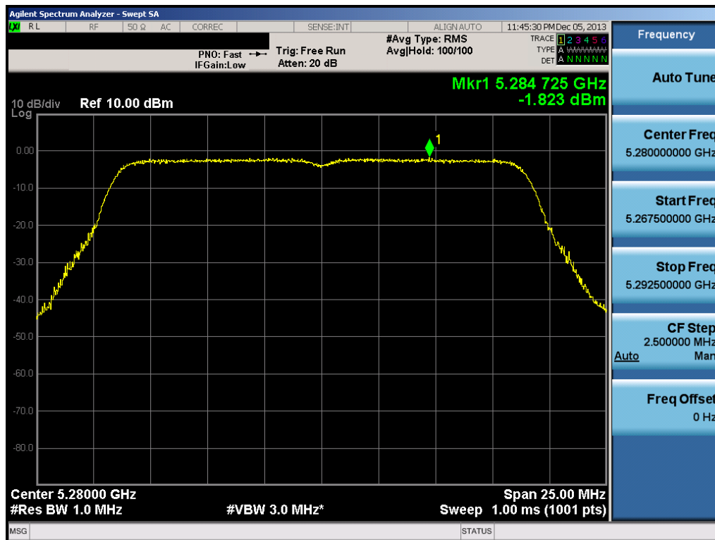
Plot 6-77. Peak Power Spectral Density Plot (20MHz BW 802.11n (UNII Band 2A) – Ch. 56)
