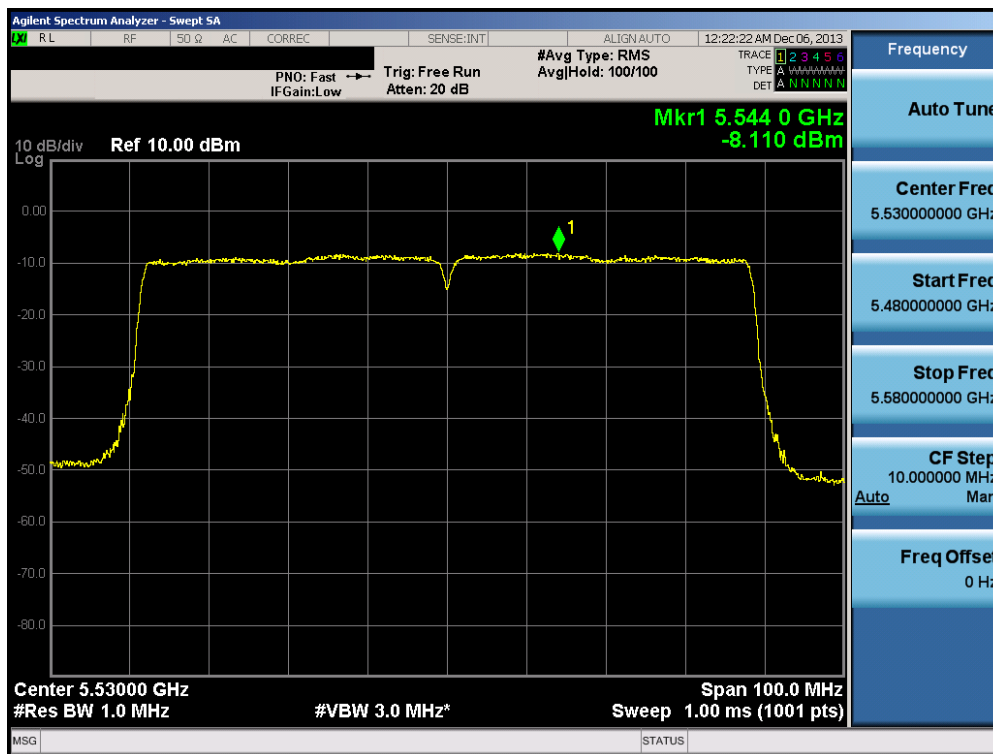
Plot 6-119. Peak Power Spectral Density Plot (80MHz BW 802.11ac (UNII Band 2C) – Ch. 106)
