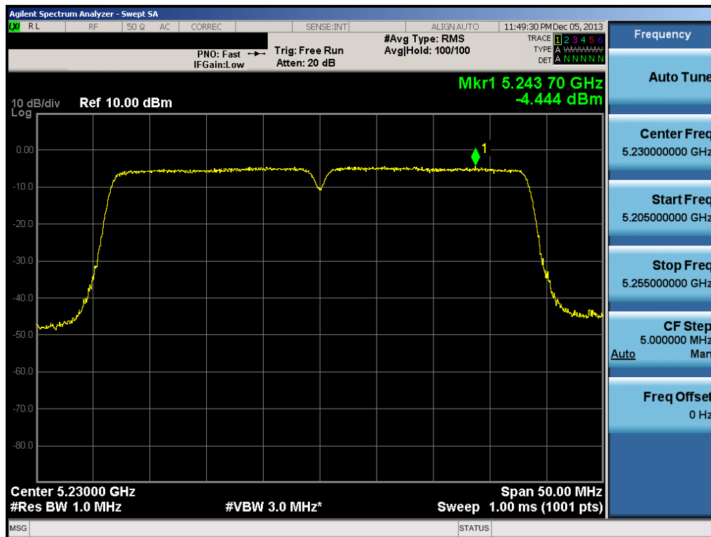
Plot 6-71. Peak Power Spectral Density Plot (40MHz BW 802.11n (UNII Band 1) – Ch. 46)
