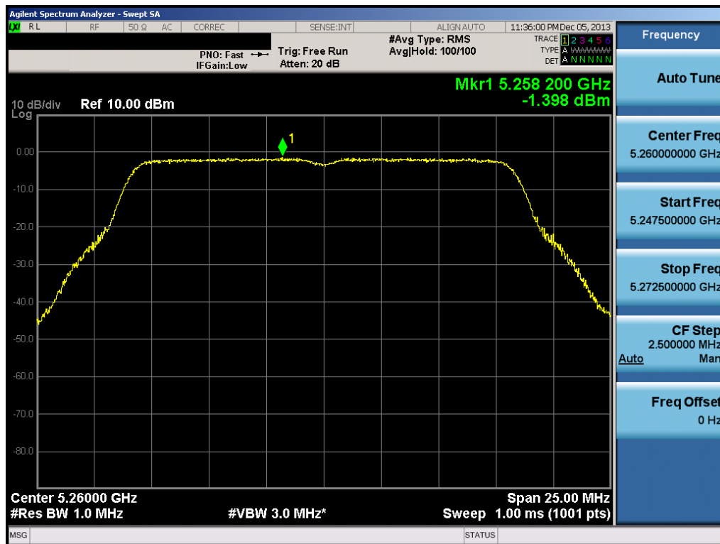
Plot 6-73. Peak Power Spectral Density Plot (802.11a (UNII Band 2A) – Ch. 52)
