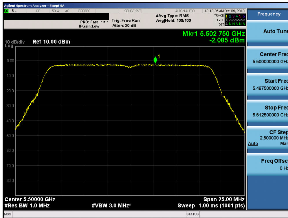
Plot 6-113. Peak Power Spectral Density Plot (20MHz BW 802.11n (UNII Band 2C) – Ch. 100)
