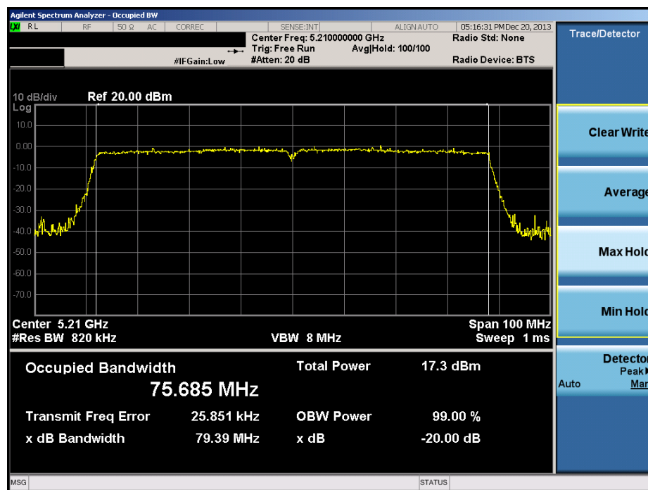
Plot 6-63. 20dB Bandwidth Plot (80MHz BW 802.11n (UNII Band 1) – Ch. 42)
