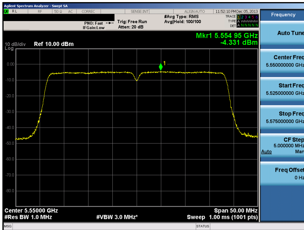
Plot 6-89. Peak Power Spectral Density Plot (40MHz BW 802.11n (UNII Band 2C) – Ch. 110)
