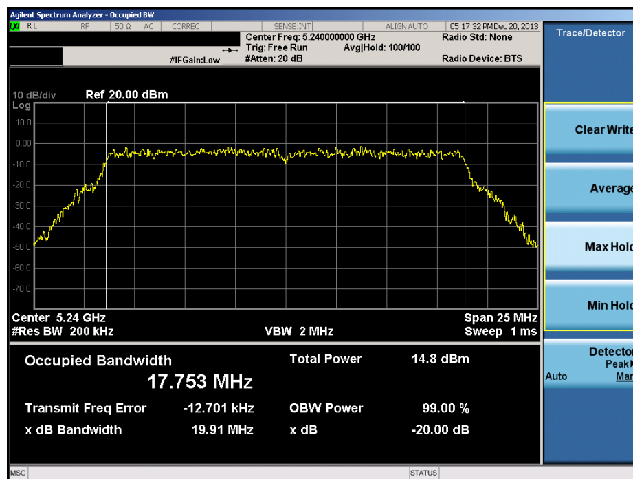
Plot 6-61. 20dB Bandwidth Plot (20MHz BW 802.11n (UNII Band 1) – Ch. 48)
