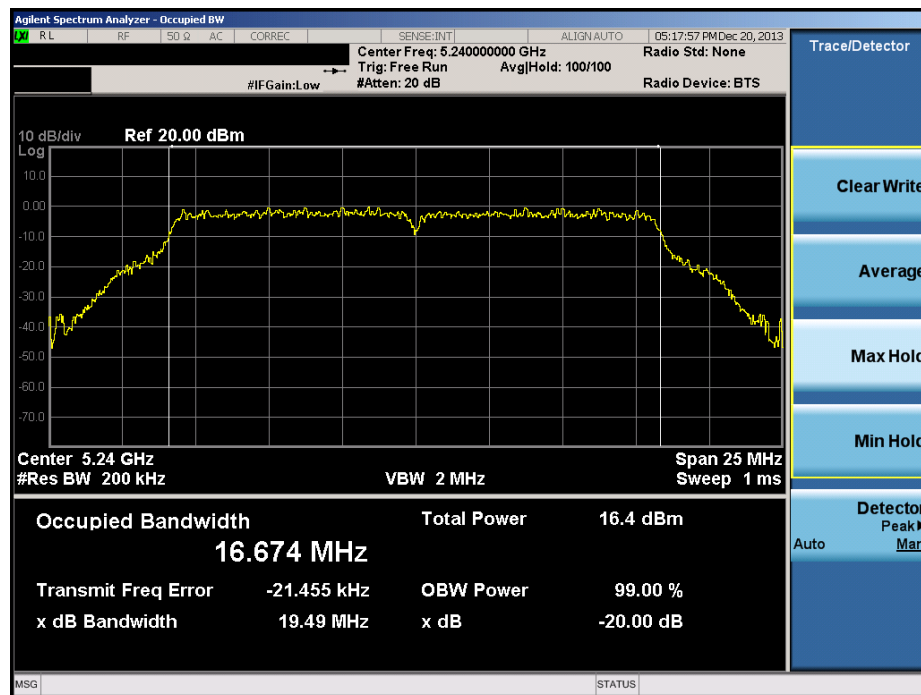
Plot 6-60. 20dB Bandwidth Plot (20MHz BW 802.11a (UNII Band 1) – Ch. 48)
