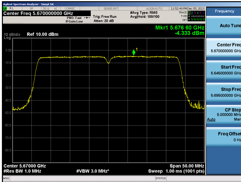
Plot 6-90. Peak Power Spectral Density Plot (40MHz BW 802.11n (UNII Band 2C) – Ch. 134)
