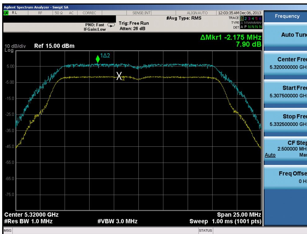
Plot 6-124. Peak Excursion Ratio Plot (802.11a)
