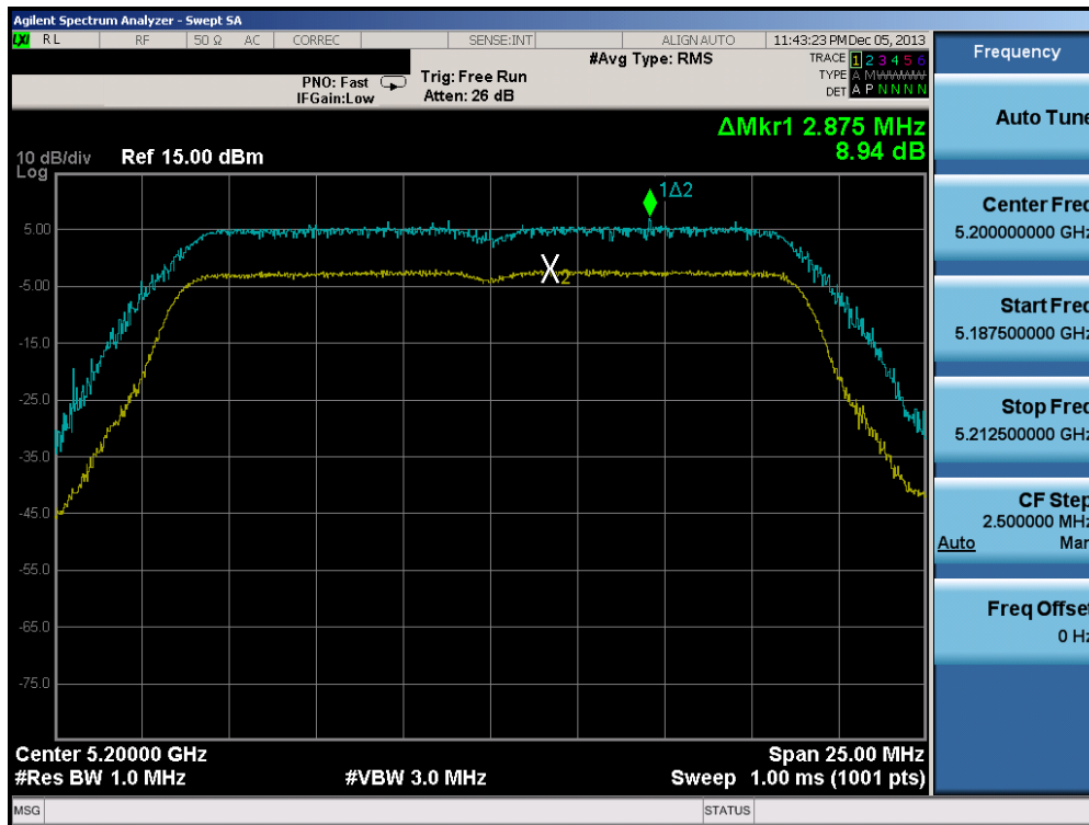
Plot 6-121. Peak Excursion Ratio Plot (20MHz BW 802.11n)
