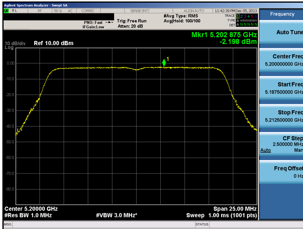
Plot 6-68. Peak Power Spectral Density Plot (20MHz BW 802.11n (UNII Band 1) – Ch. 40)
