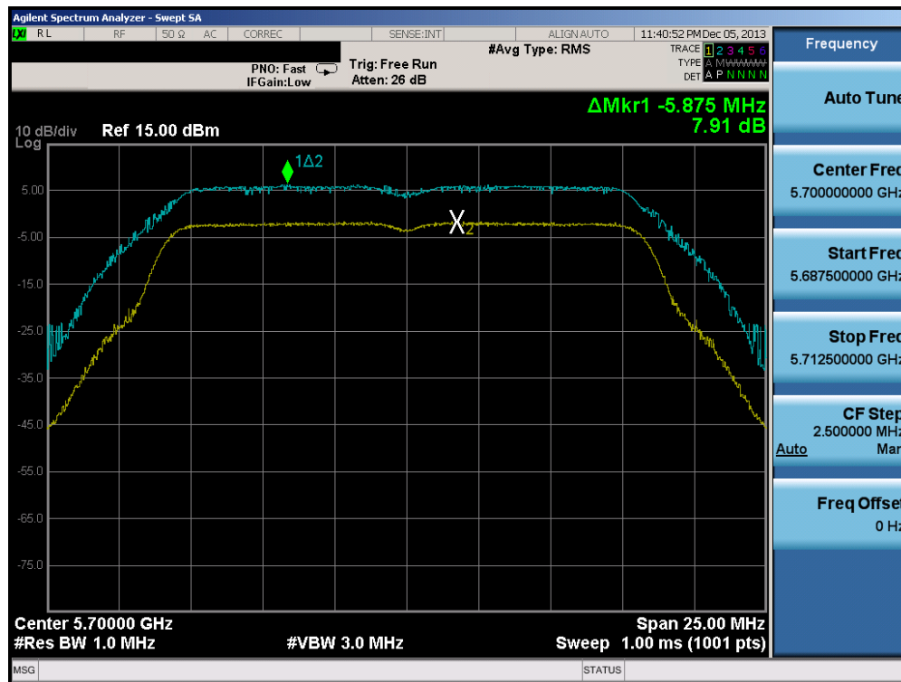
Plot 6-120. Peak Excursion Ratio Plot (802.11a)
