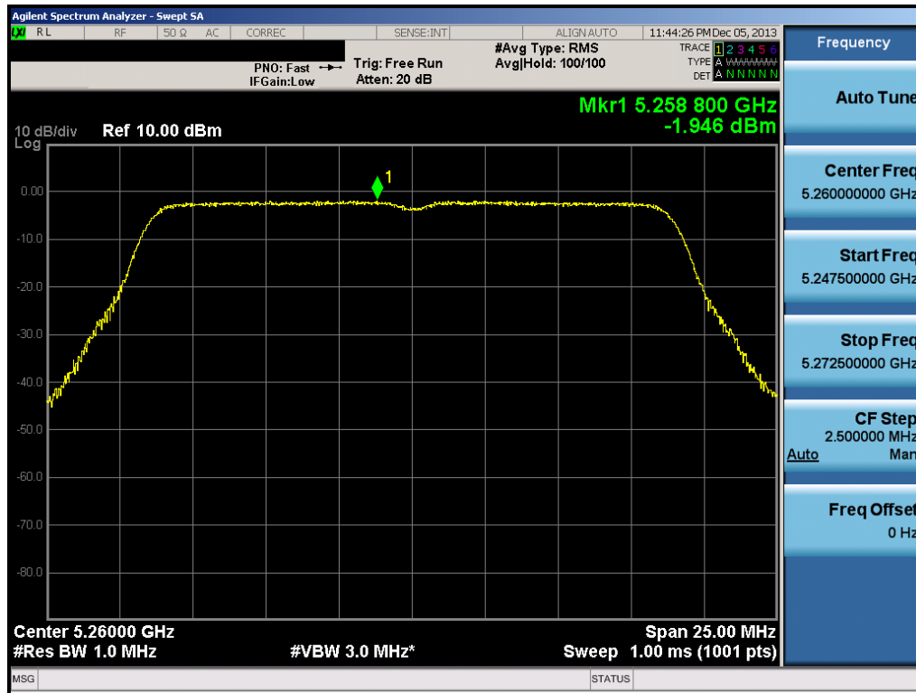
Plot 6-76. Peak Power Spectral Density Plot (20MHz BW 802.11n (UNII Band 2A) – Ch. 52)
