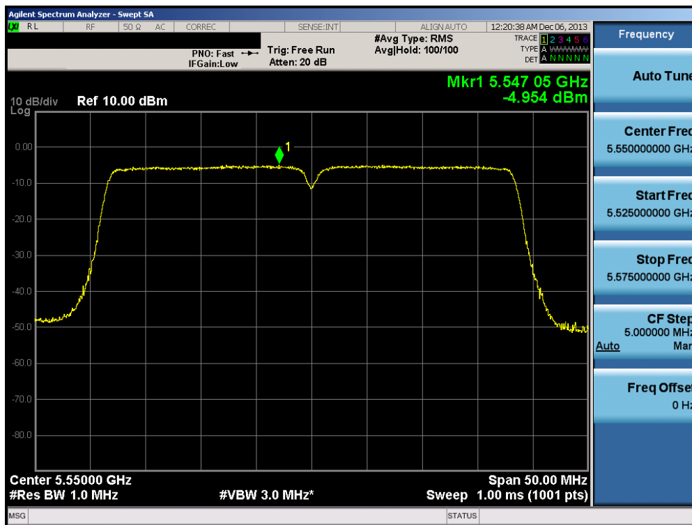
Plot 6-117. Peak Power Spectral Density Plot (40MHz BW 802.11n (UNII Band 2C) – Ch. 110)
