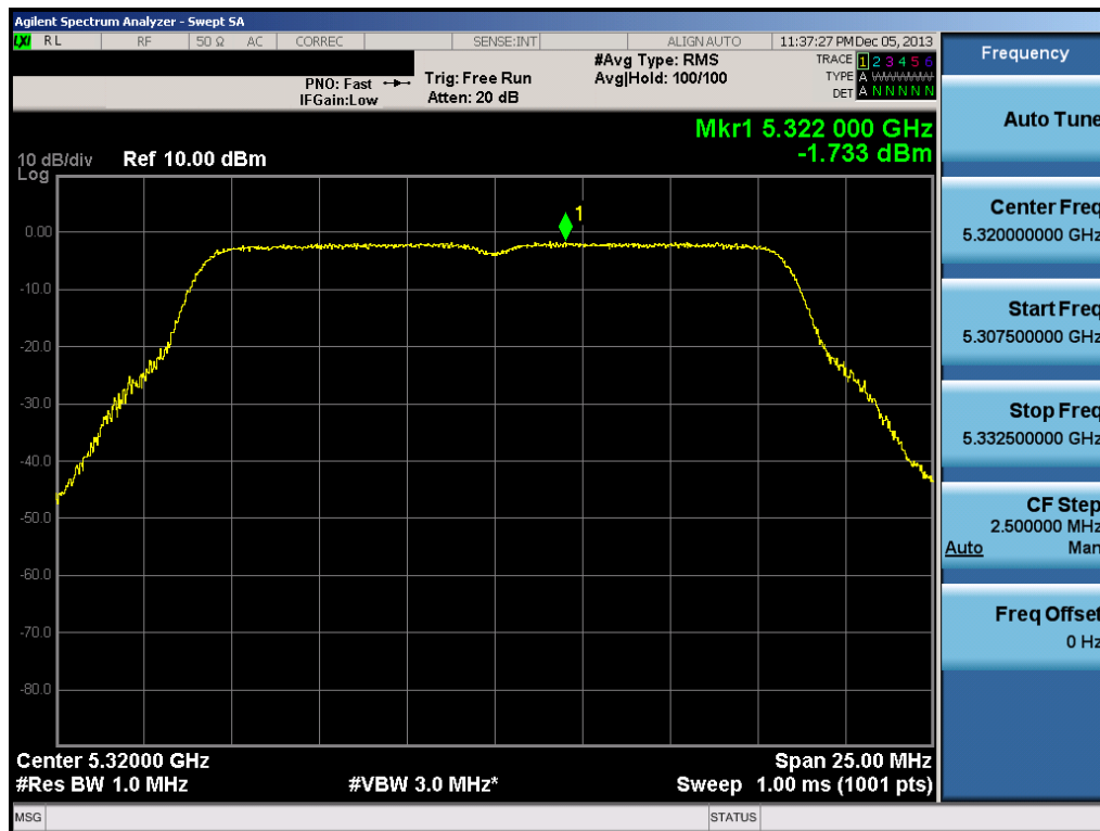
Plot 6-75. Peak Power Spectral Density Plot (802.11a (UNII Band 2A) – Ch. 64)
