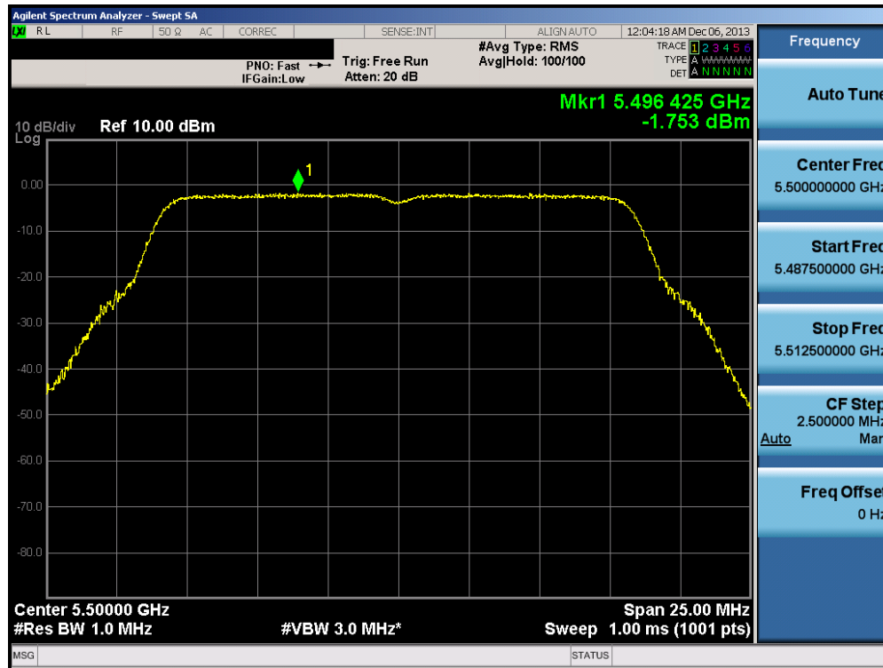
Plot 6-110. Peak Power Spectral Density Plot (802.11a (UNII Band 2C) – Ch. 100)
