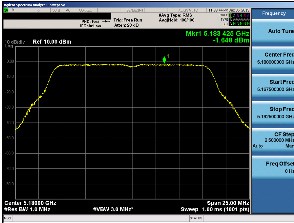
Plot 6-64. Peak Power Spectral Density Plot (802.11a (UNII Band 1) – Ch. 36)
