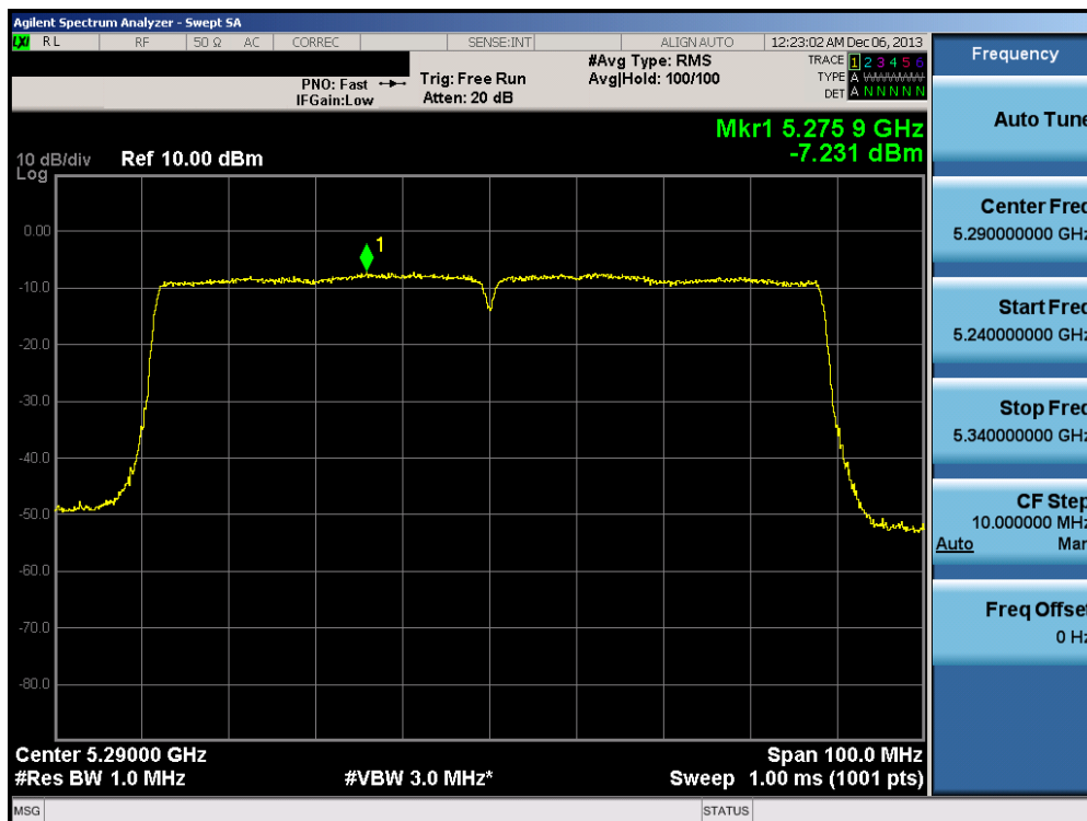
Plot 6-109. Peak Power Spectral Density Plot (80MHz BW 802.11ac (UNII Band 2A) – Ch. 58)
