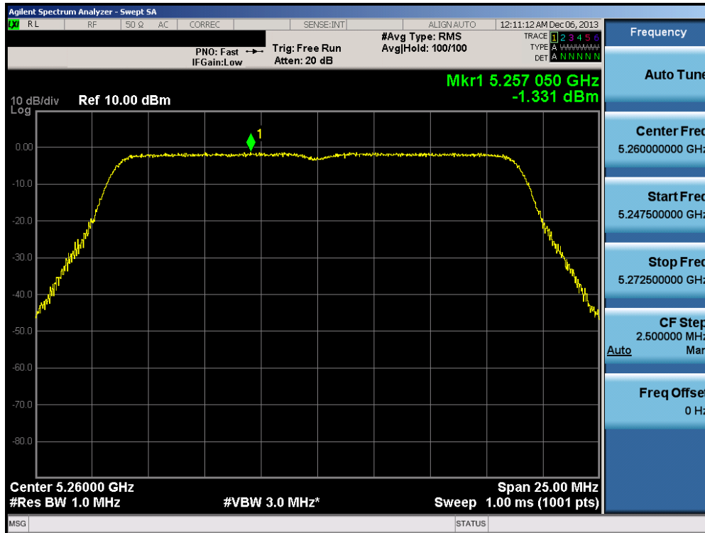
Plot 6-104. Peak Power Spectral Density Plot (20MHz BW 802.11n (UNII Band 2A) – Ch. 52)
