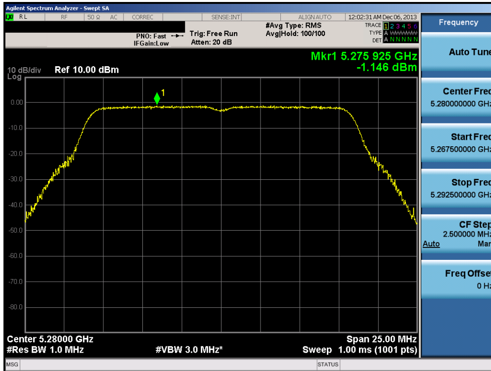
Plot 6-102. Peak Power Spectral Density Plot (802.11a (UNII Band 2A) – Ch. 56)
