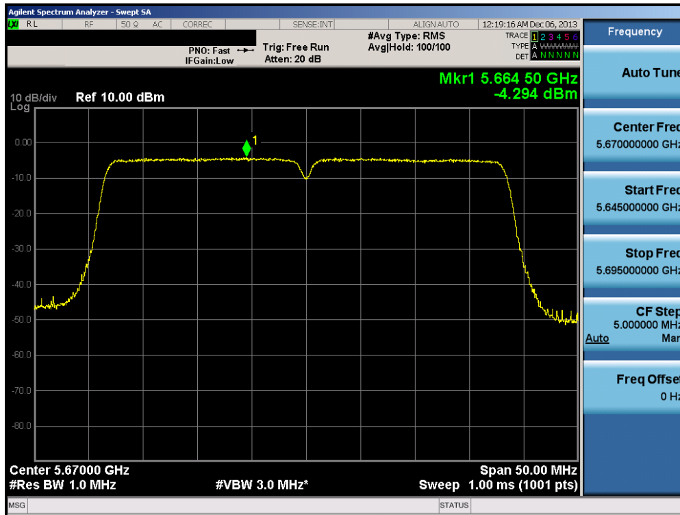
Plot 6-118. Peak Power Spectral Density Plot (40MHz BW 802.11n (UNII Band 2C) – Ch. 134)
