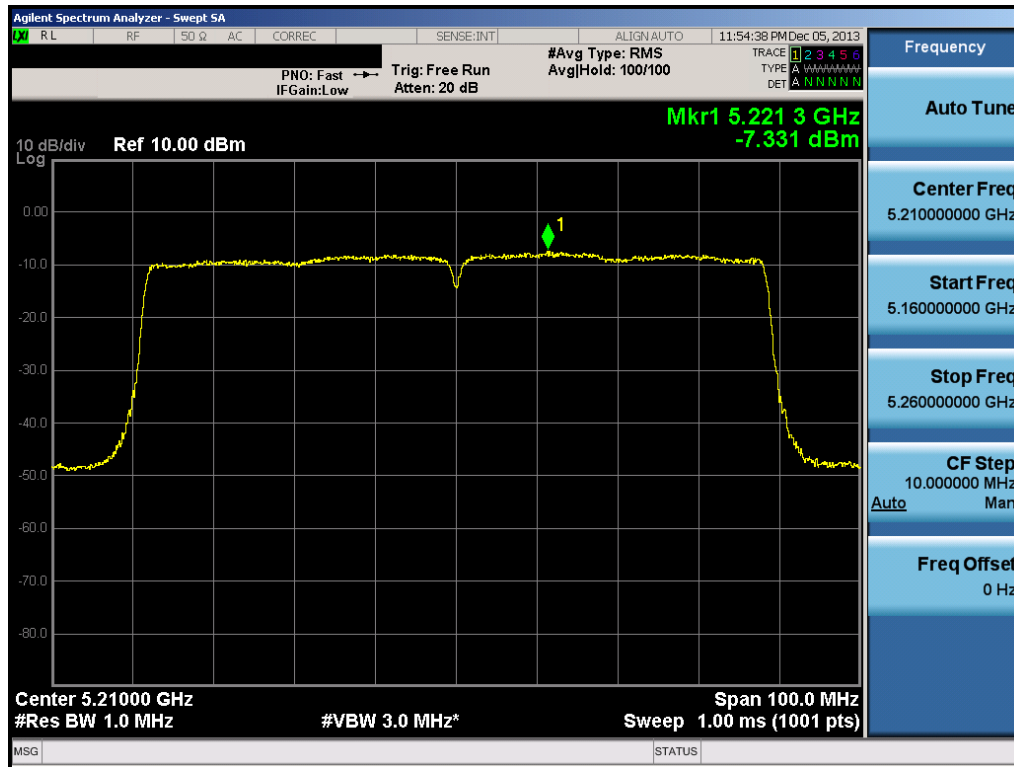
Plot 6-72. Peak Power Spectral Density Plot (80MHz BW 802.11ac (UNII Band 1) – Ch. 42)
