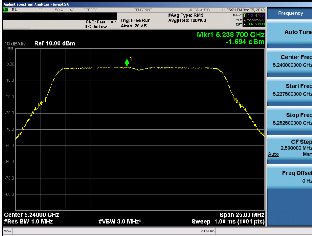
Plot 6-66. Peak Power Spectral Density Plot (802.11a (UNII Band 1) – Ch. 48)
