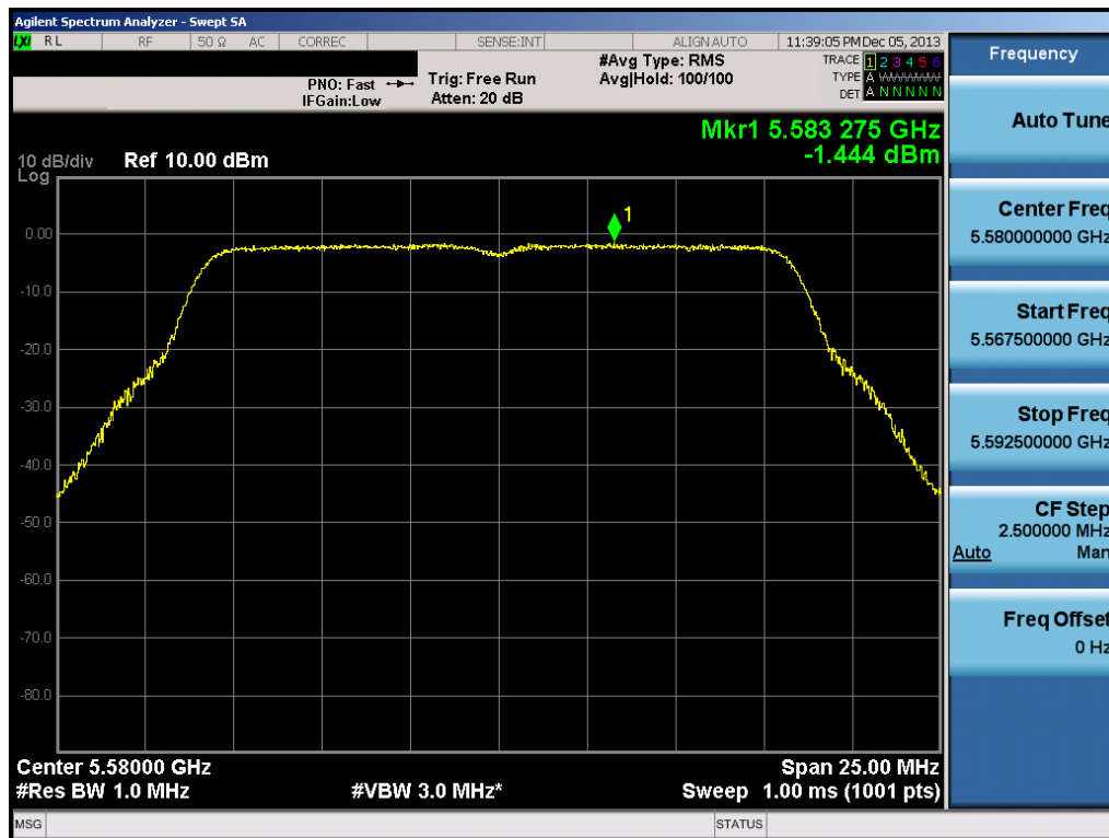
Plot 6-83. Peak Power Spectral Density Plot (802.11a (UNII Band 2C) – Ch. 116)
