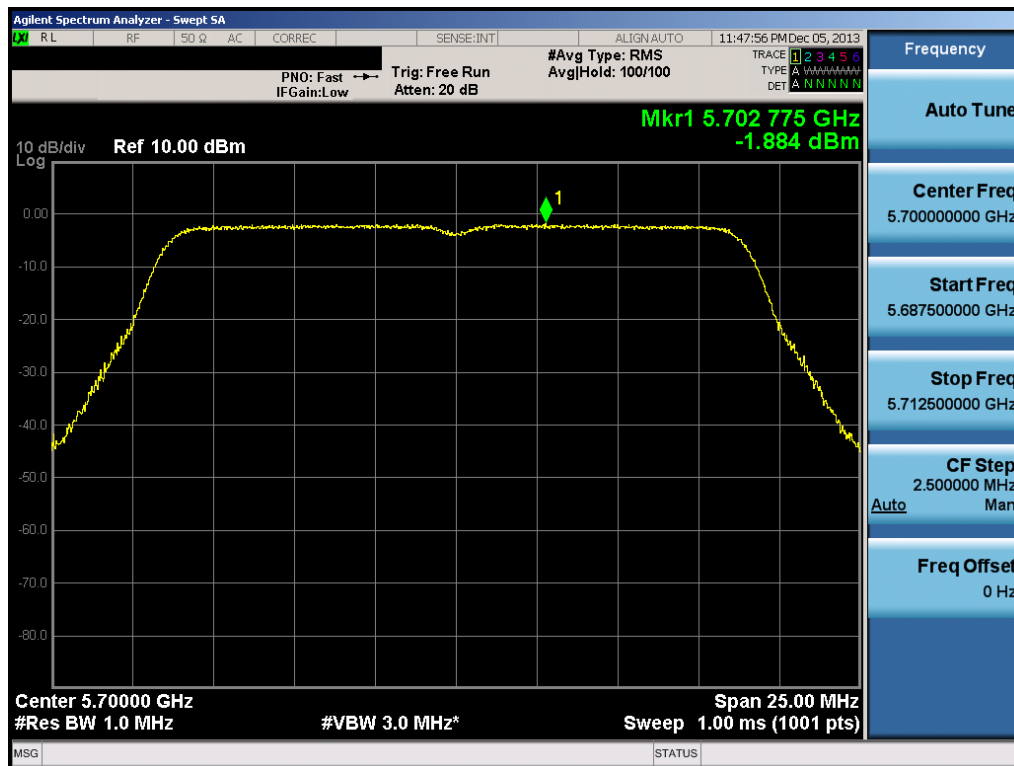
Plot 6-87. Peak Power Spectral Density Plot (20MHz BW 802.11n (UNII Band 2C) – Ch. 140)
