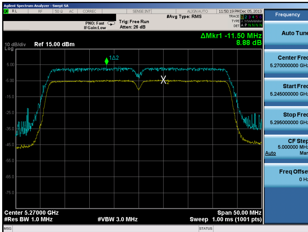
Plot 6-122. Peak Excursion Ratio Plot (40MHz BW 802.11n)
