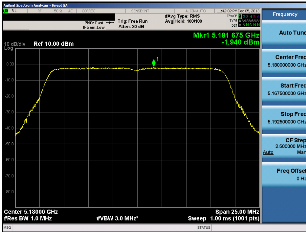
Plot 6-67. Peak Power Spectral Density Plot (20MHz BW 802.11n (UNII Band 1) – Ch. 36)
