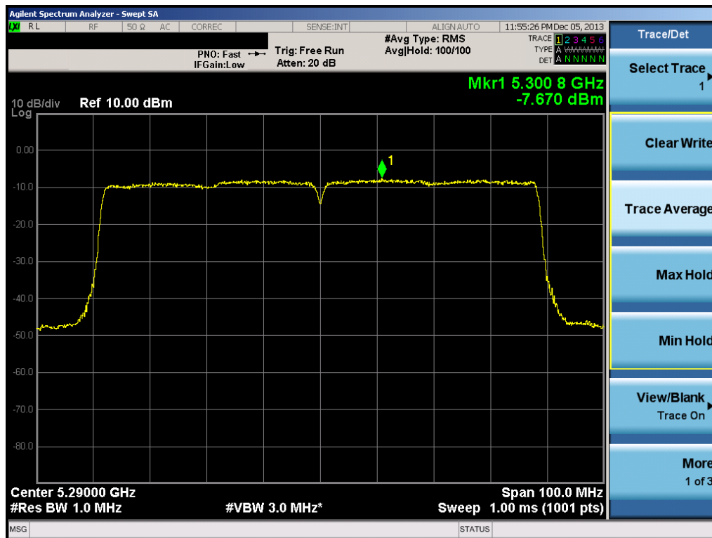
Plot 6-81. Peak Power Spectral Density Plot (80MHz BW 802.11ac (UNII Band 2A) – Ch. 58)
