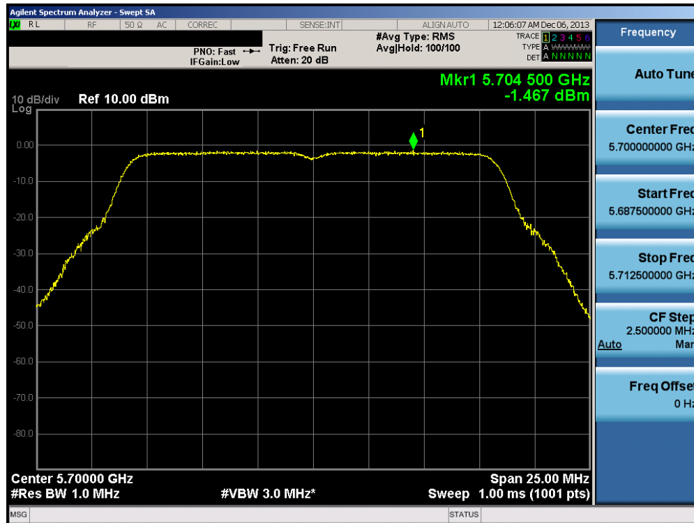
Plot 6-112. Peak Power Spectral Density Plot (802.11a (UNII Band 2C) – Ch. 140)
