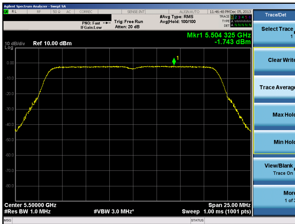
Plot 6-85. Peak Power Spectral Density Plot (20MHz BW 802.11n (UNII Band 2C) – Ch. 100)
