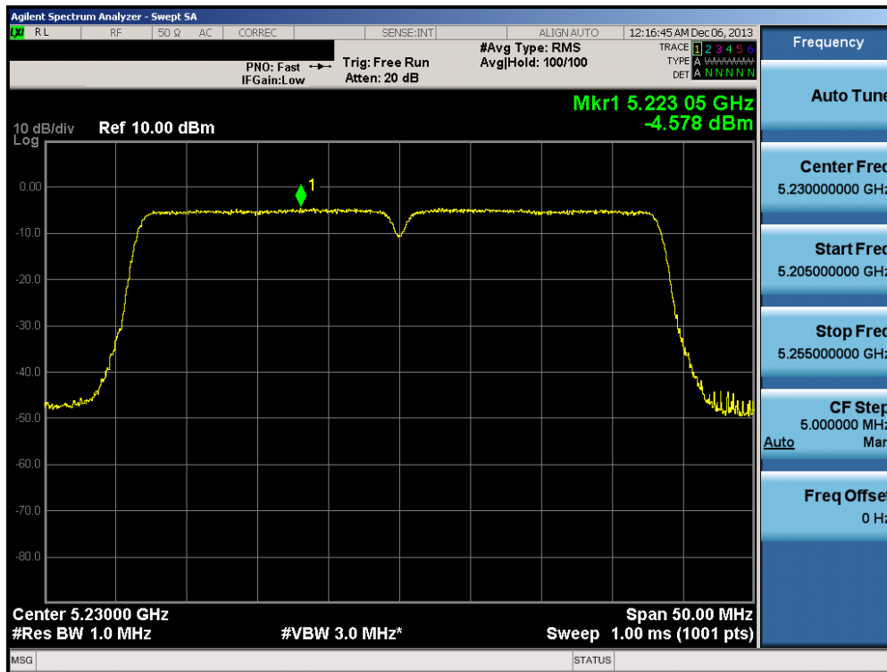
Plot 6-99. Peak Power Spectral Density Plot (40MHz BW 802.11n (UNII Band 1) – Ch. 46)
