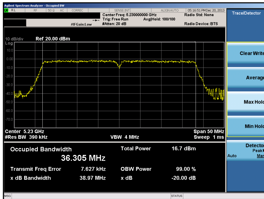
Plot 6-62. 20dB Bandwidth Plot (40MHz BW 802.11n (UNII Band 1) – Ch. 46)
