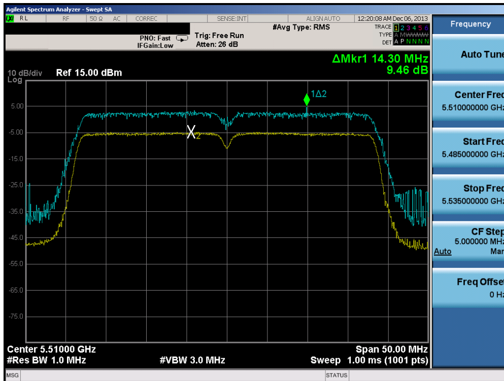
Plot 6-126. Peak Excursion Ratio Plot (40MHz BW 802.11n)
