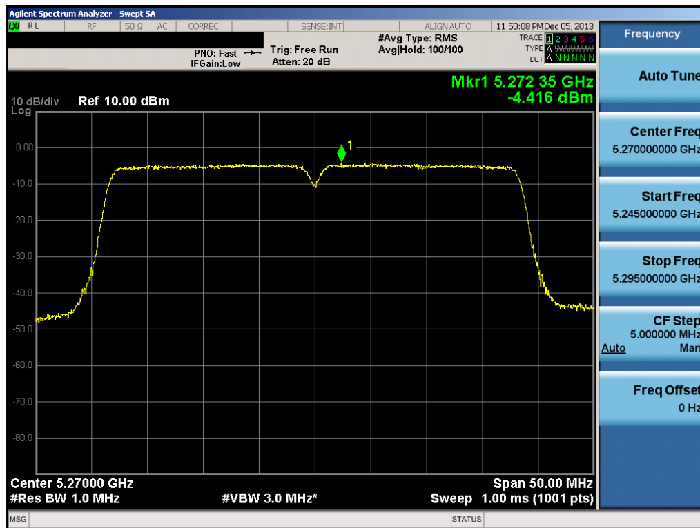
Plot 6-79. Peak Power Spectral Density Plot (40MHz BW 802.11n (UNII Band 2A) – Ch. 54)
