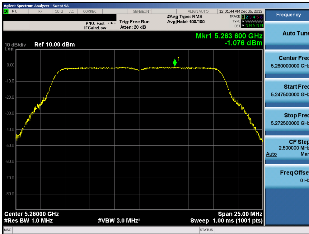
Plot 6-101. Peak Power Spectral Density Plot (802.11a (UNII Band 2A) – Ch. 52)
