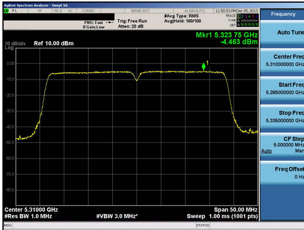
Plot 6-80. Peak Power Spectral Density Plot (40MHz BW 802.11n (UNII Band 2A) – Ch. 62)
