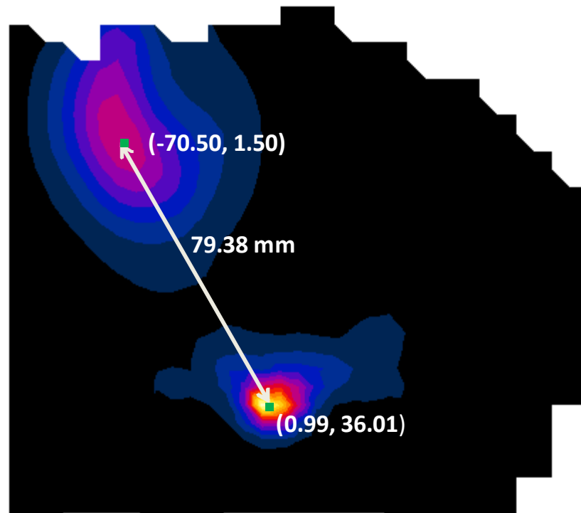
Figure 11-16 Peak SAR Locations of 5 GHz WLAN and GPRS 850 MHz
