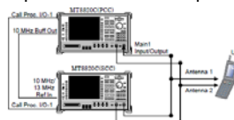
Figure 8-2 Power Measurement Setup
