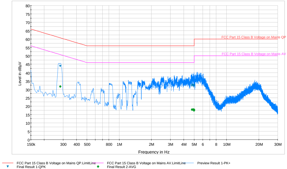
Plot 6-197. Line Conducted Plot with 802.11a UNII Band 2C (N)
