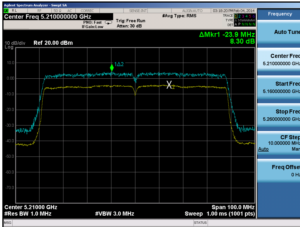
Plot 6-127. Peak Excursion Ratio Plot (80MHz BW 802.11ac)
