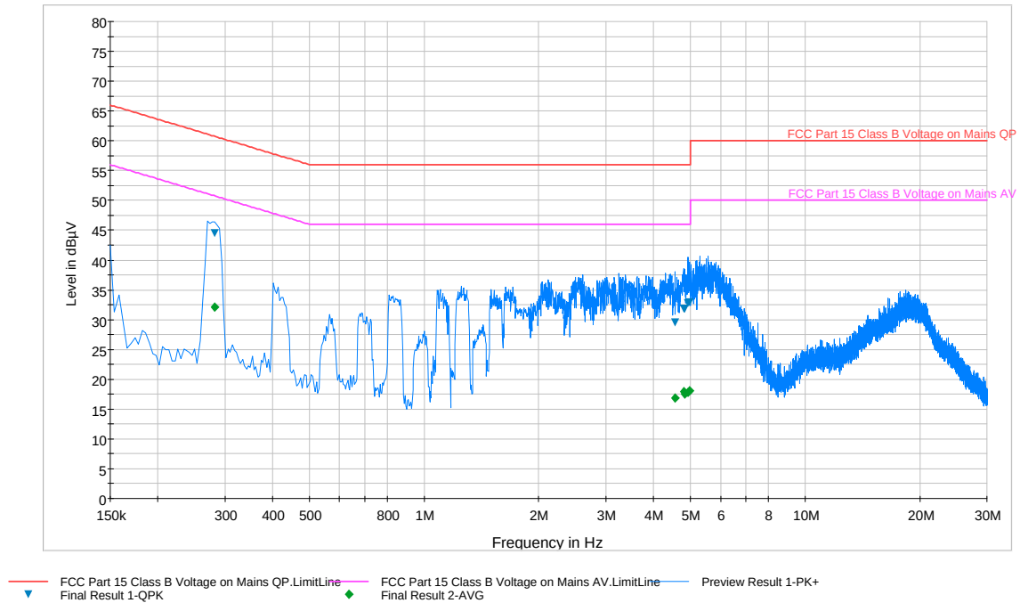
Plot 6-193. Line Conducted Plot with 802.11a UNII Band 1 (N)
