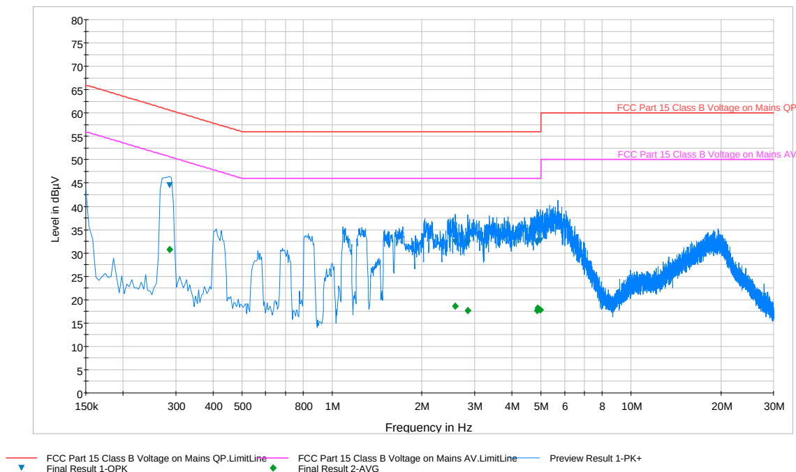
Plot 6-195. Line Conducted Plot with 802.11a UNII Band 2A (N)
