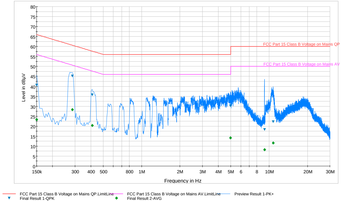
Plot 6-192. Line Conducted Plot with 802.11a UNII Band 1 (L1)
