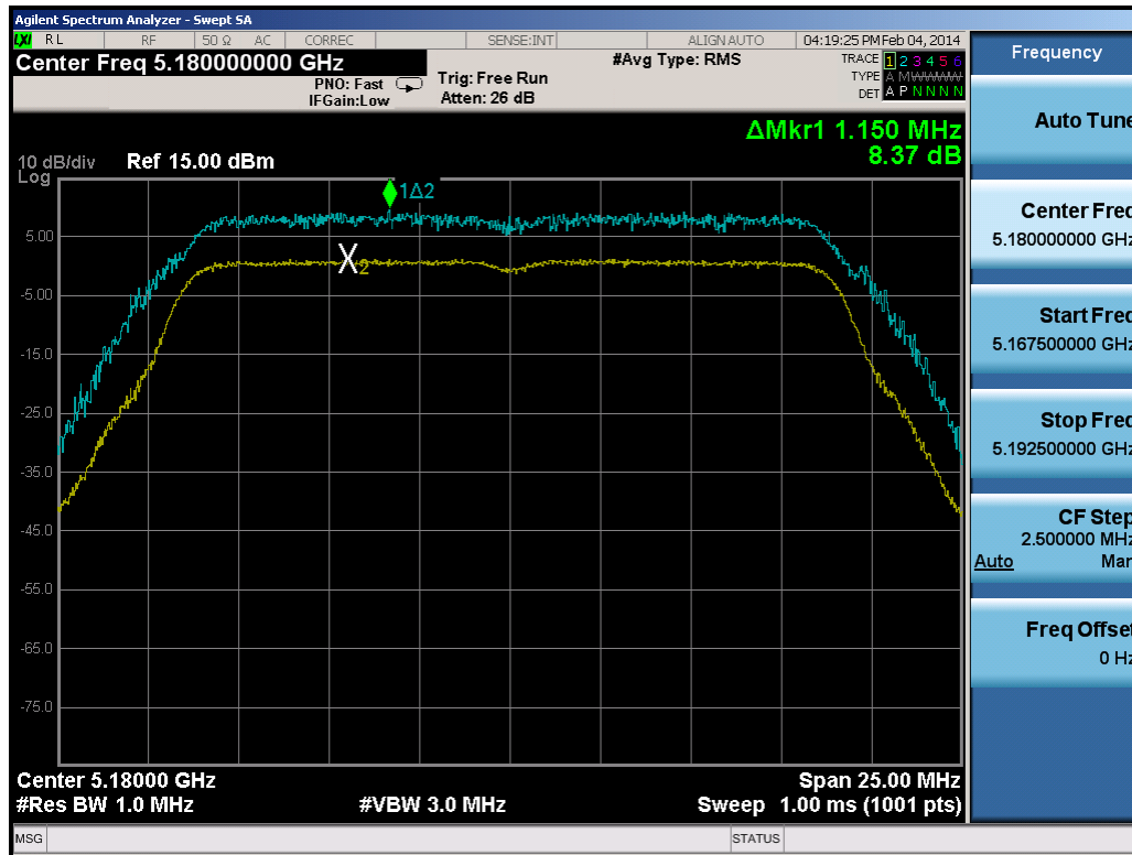
Plot 6-129. Peak Excursion Ratio Plot (20MHz BW 802.11n)
