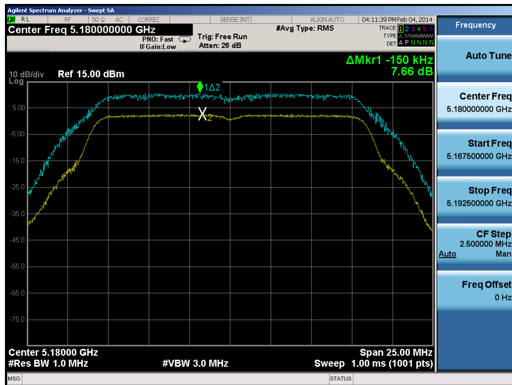
Plot 6-128. Peak Excursion Ratio Plot (802.11a)
