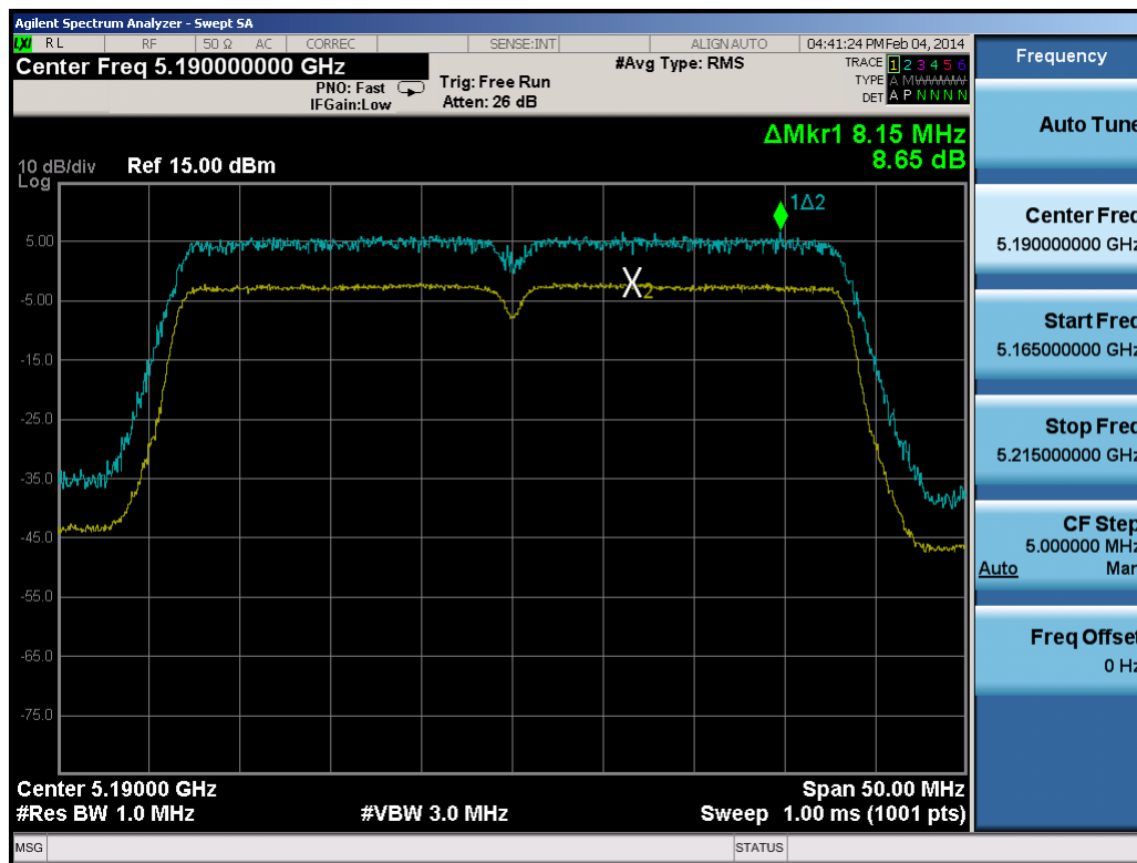
Plot 6-130. Peak Excursion Ratio Plot (40MHz BW 802.11n)
