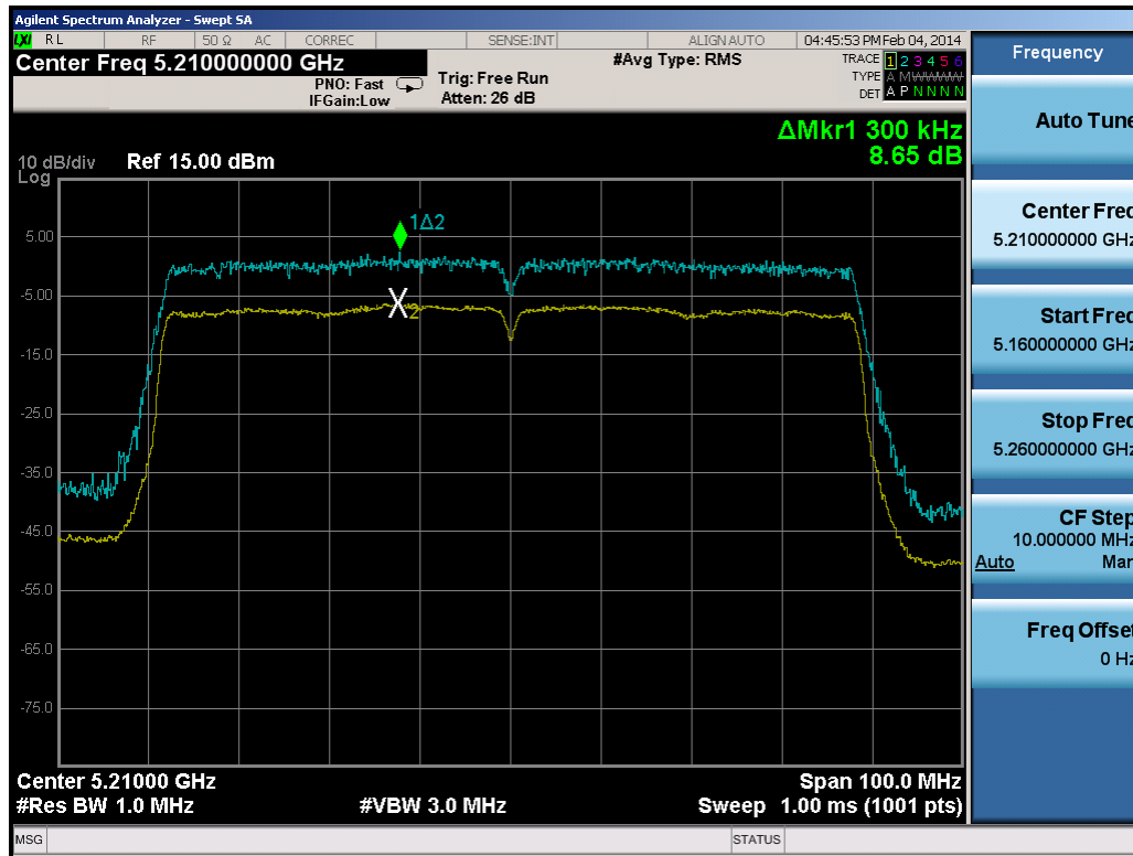
Plot 6-131. Peak Excursion Ratio Plot (80MHz BW 802.11ac)
