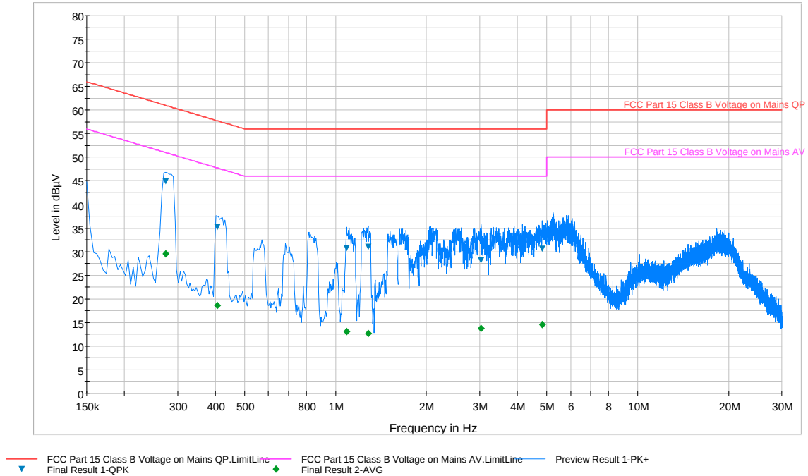
Plot 6-196. Line Conducted Plot with 802.11a UNII Band 2C (L1)
