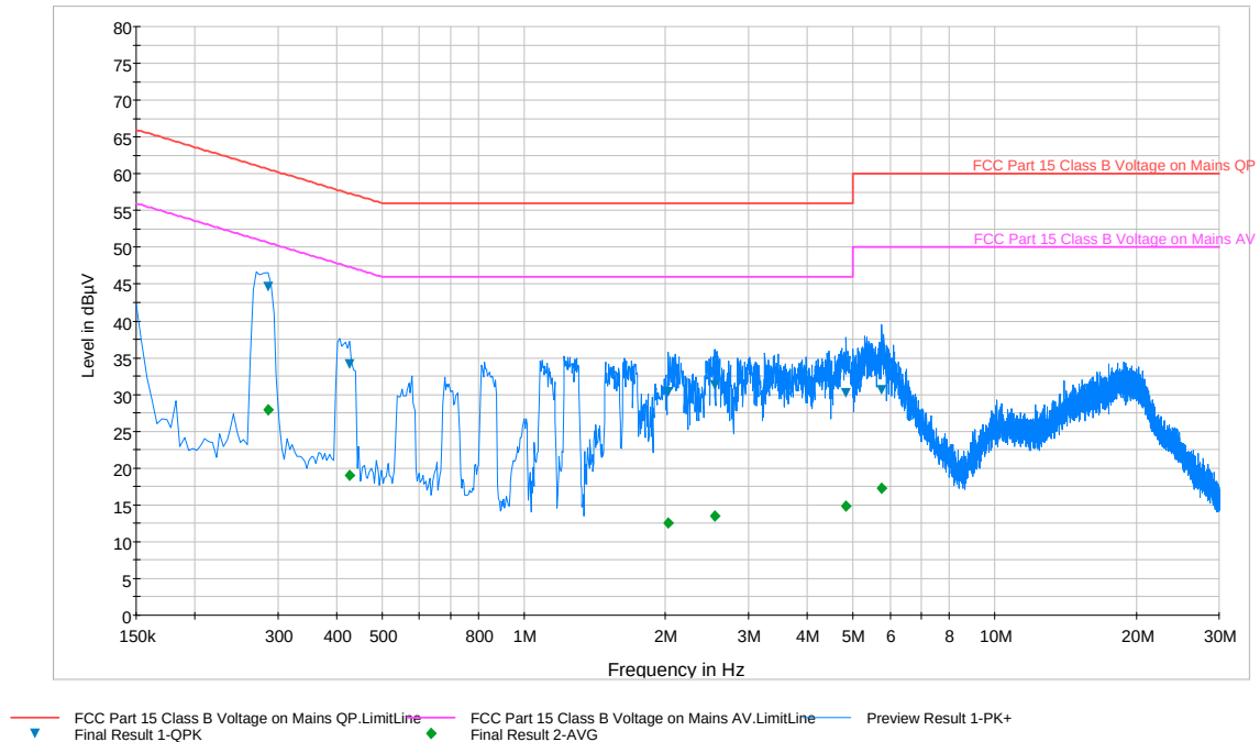
Plot 6-194. Line Conducted Plot with 802.11a UNII Band 2A (L1)
