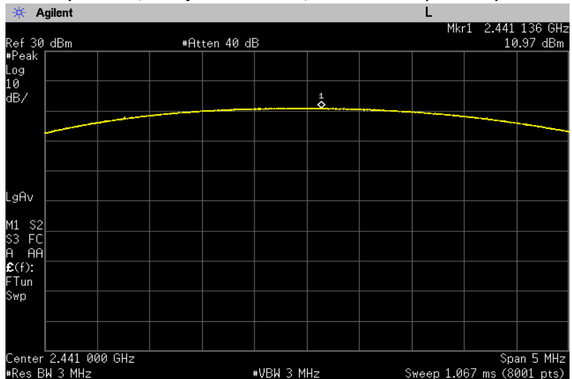
Peak Output Power, \pi/4 DQPSK modulation, Middle Channel (2441 MHz)
