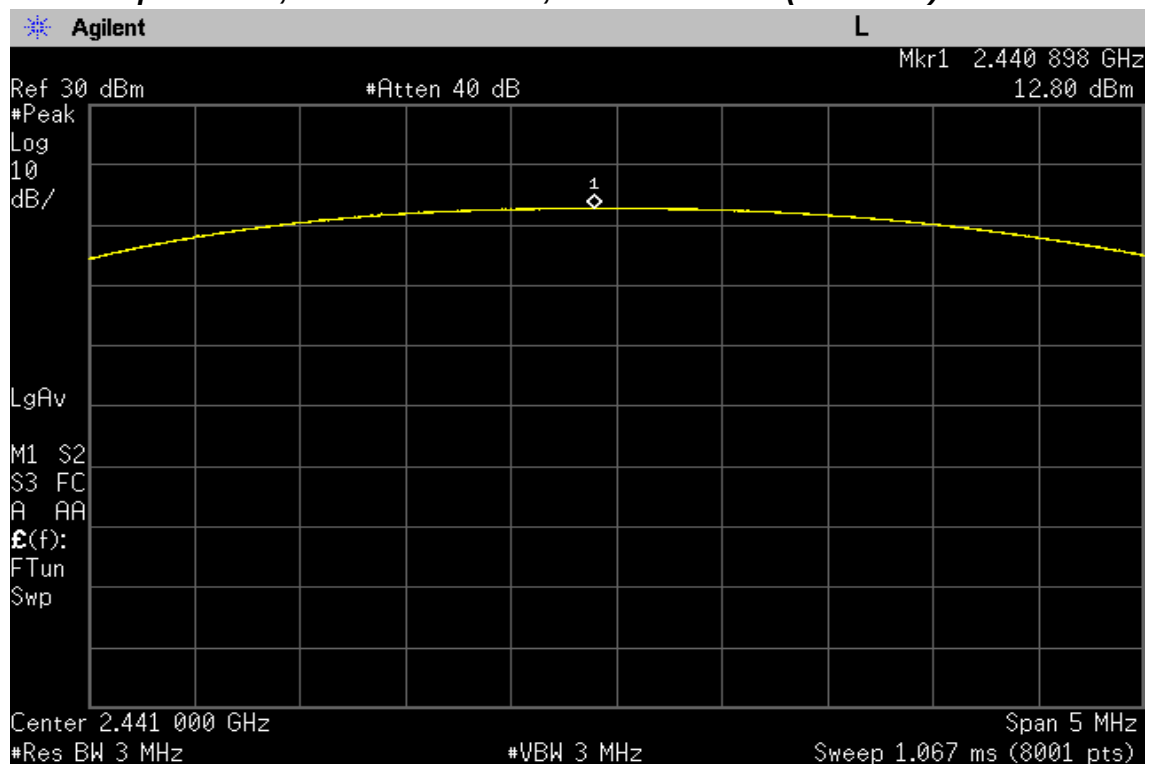
Peak Output Power, GFSK modulation, Middle Channel (2441 MHz)
