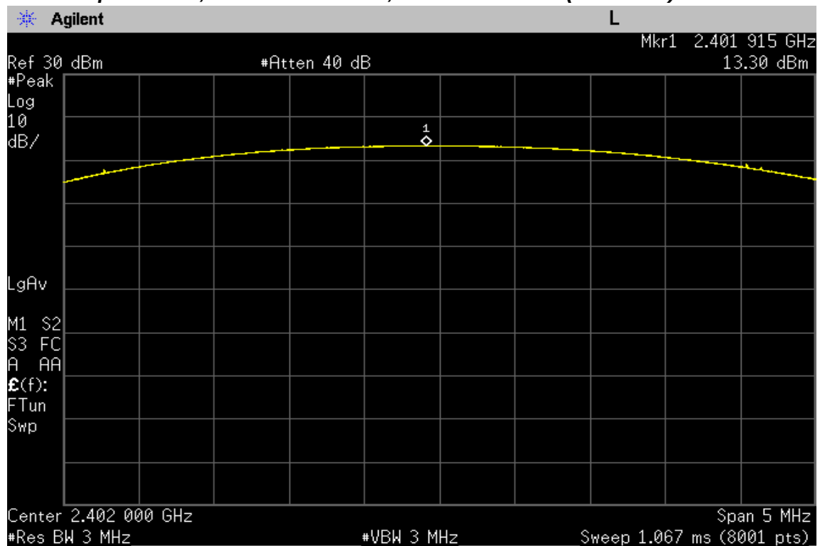
Peak Output Power, GFSK modulation, Lowest Channel (2402 MHz)
