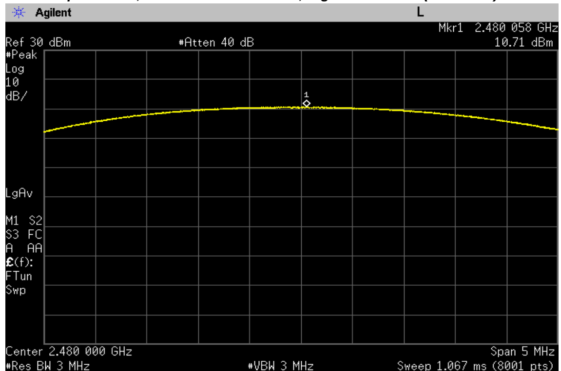
Peak Output Power, \pi/4 DQPSK modulation, Highest Channel (2480 MHz)
