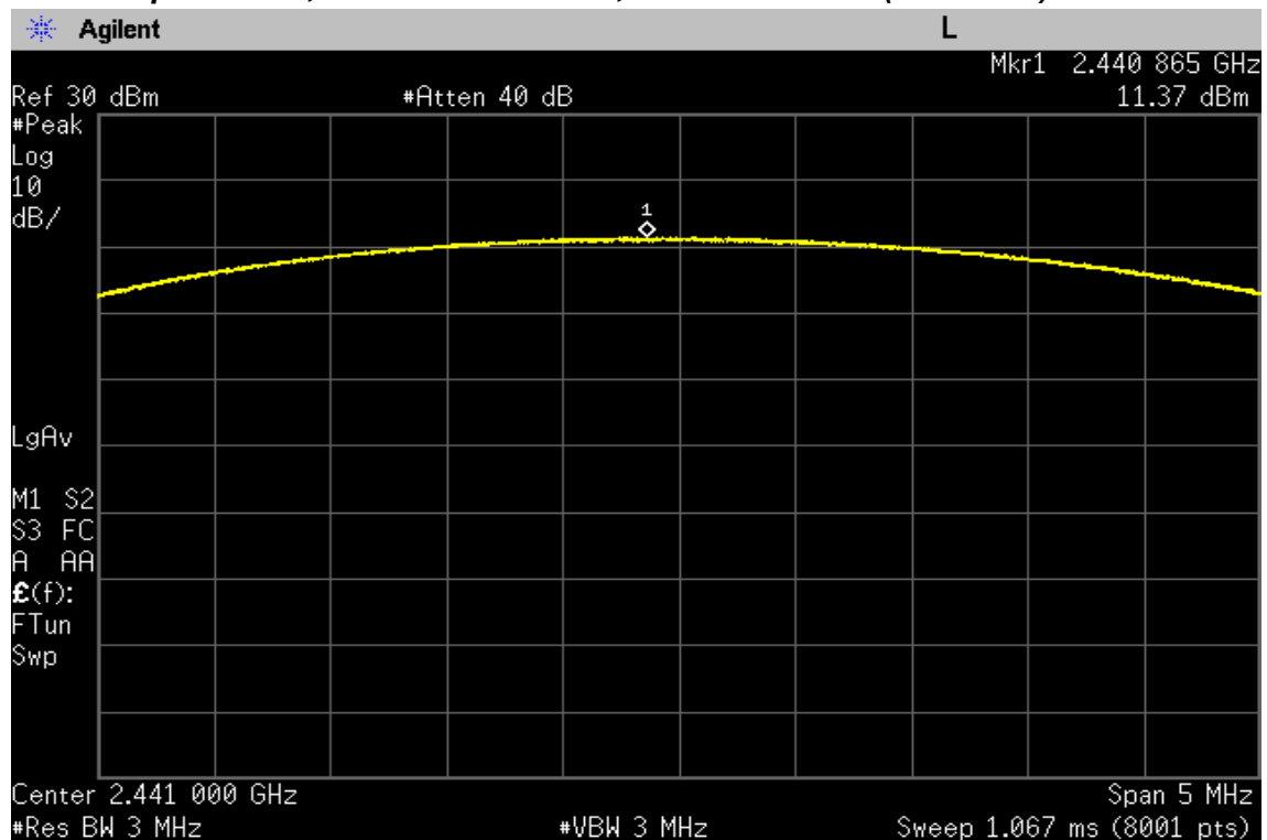
Peak Output Power, 8DPSK modulation, Middle Channel (2441 MHz)
