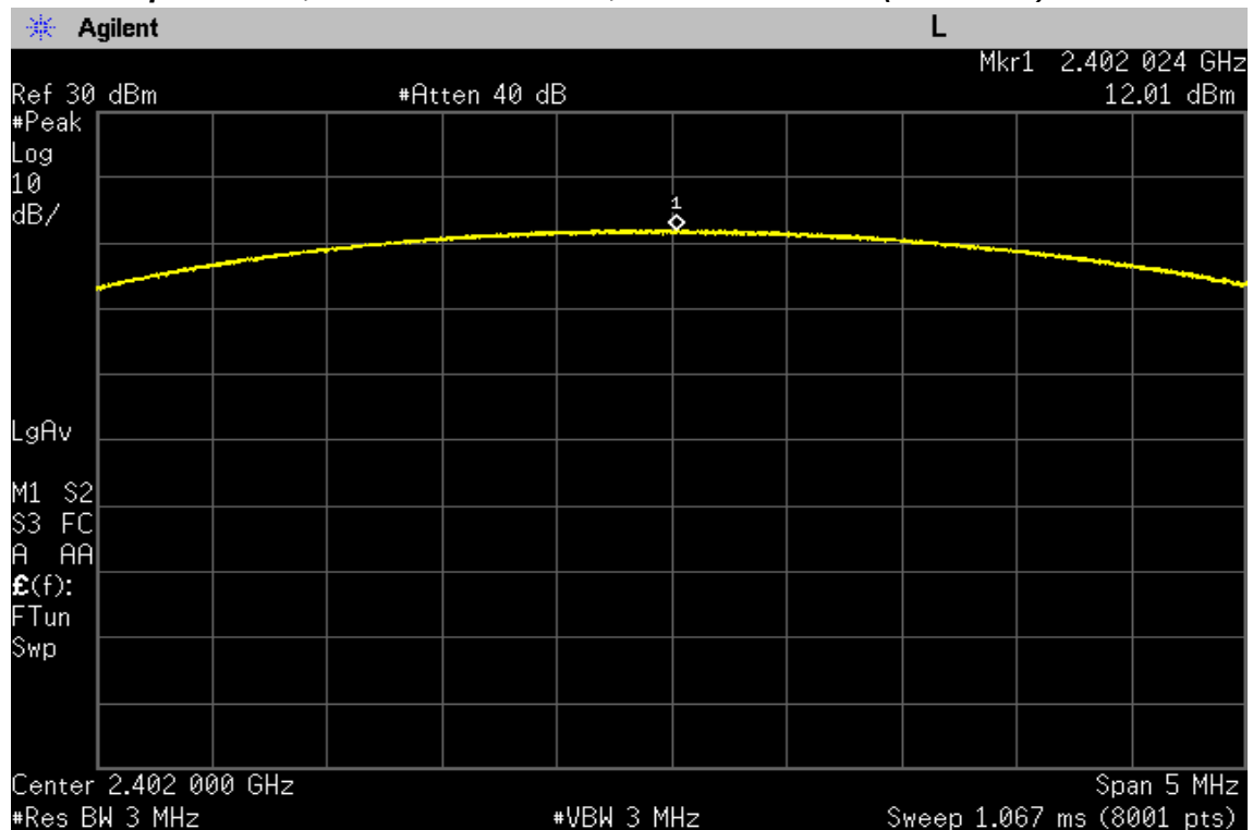
Peak Output Power, 8DPSK modulation, Lowest Channel (2402 MHz)
