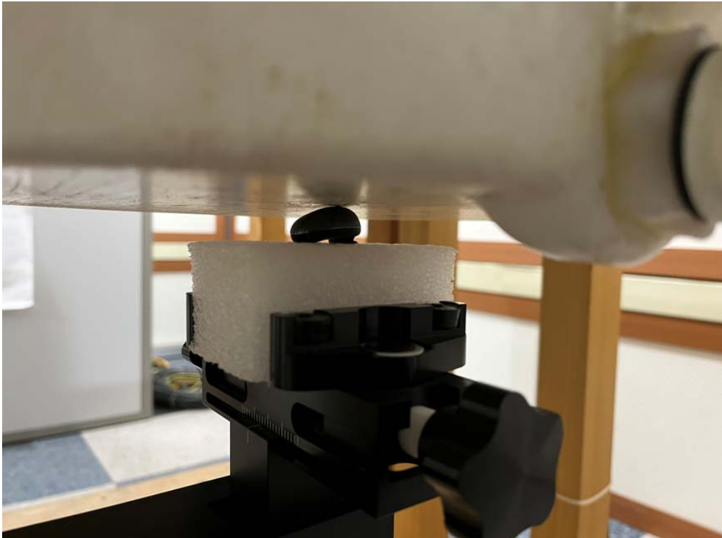
SAR Test Picture(Back), Test separation distance : 0 mm
