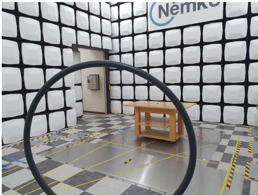
Radiated Test Picture(Rear)_Below 30MHz
