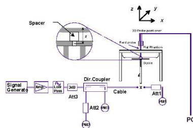
Figure 8-1 System Verification Setup Diagram
